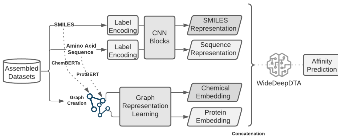
Figure 4.5. WideDeepDTA summarized.
