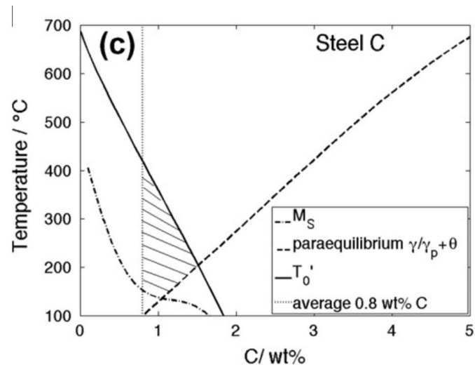
Figure 2.11. T-C diagram [33]
