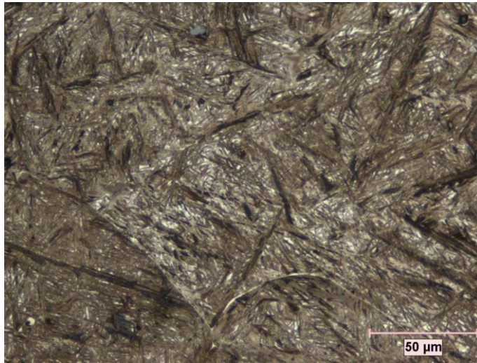
Figure 4.6. Optical Micrograph of Isothermally Heat-Treated Specimen at 170°C for 41 hours. The microstructure seems to be mostly bainite. There are small white areas which are most probably M/A islands.
