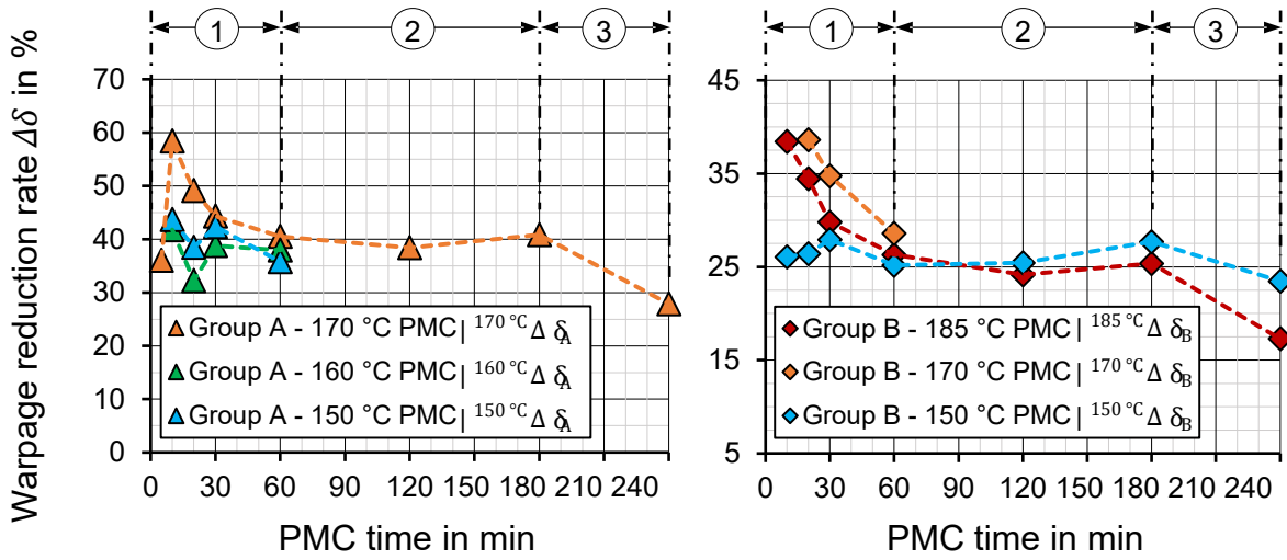
Figure 4.11: Intervals with different warpage reduction patterns
