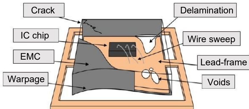
Figure 2.8: Schematic illustration for defect types in an encapsulant [5]
