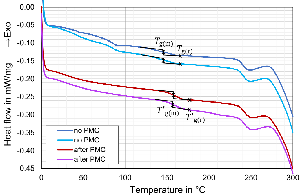
Figure 4.4: DSC curves of PCB substrate before and after 2 hours PMC at 185^\circ\text{C}
