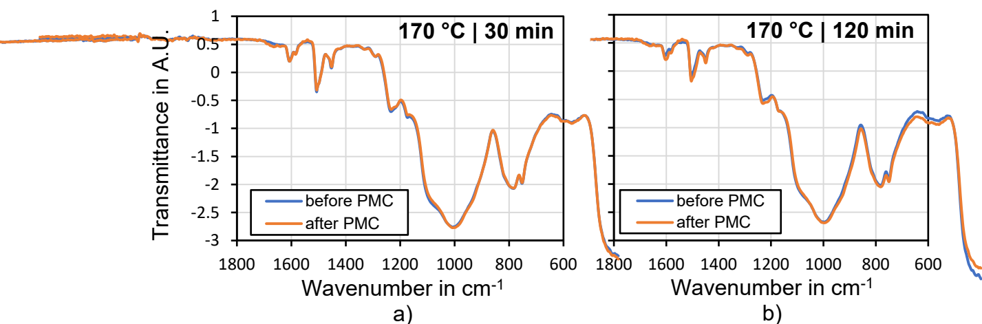
Figure 4.13: IR Spectra of EMC before and after PMC operations with a) 170\text{ }^{\circ}\text{C} and 30 min b) 170\text{ }^{\circ}\text{C} and 120 min
