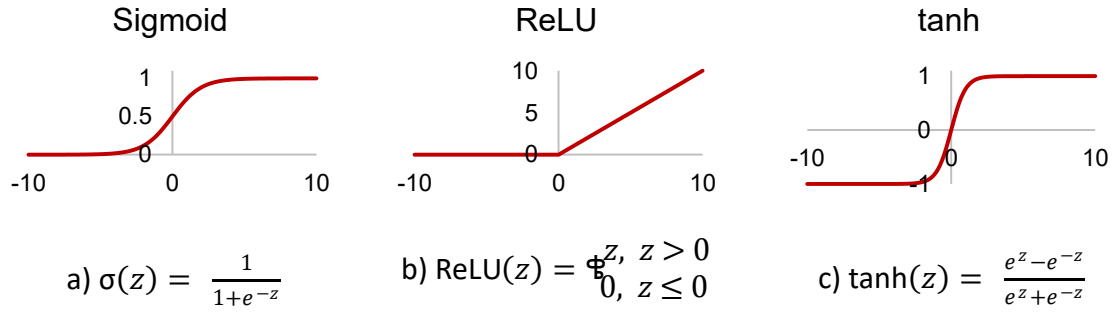
Figure 2.24: Commonly used activation functions a) sigmoid b) ReLU c) tanh [102]
