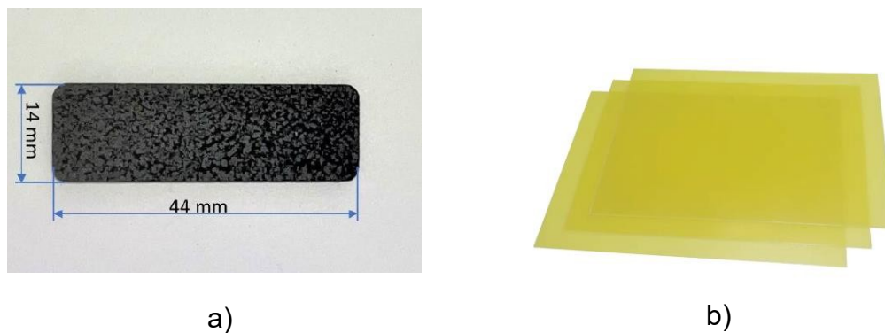
Figure 3.2: Main materials used in samples a) EMC granules pressed in sheet form b) PCB substrates without mounted electronics
