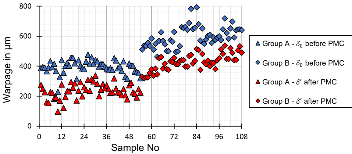
Figure 4.6: Measured warpage values of sample groups A and B
