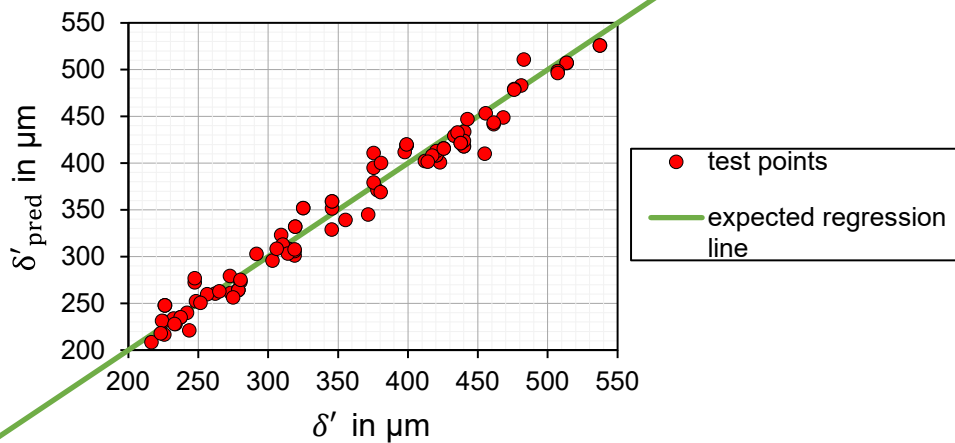
Figure 4.15: Comparison of measured and predicted final warpage values
