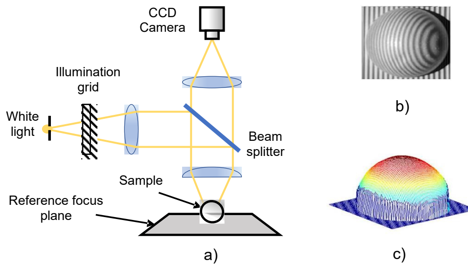
Figure 3.10: 3D Optical Profilometer a) schematic CGIS setup b) grid illuminated image c) 3D height map of the sample – adapted from [127,128]
