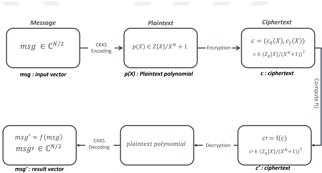
Figure 2.2 High level view of the CKKS scheme
