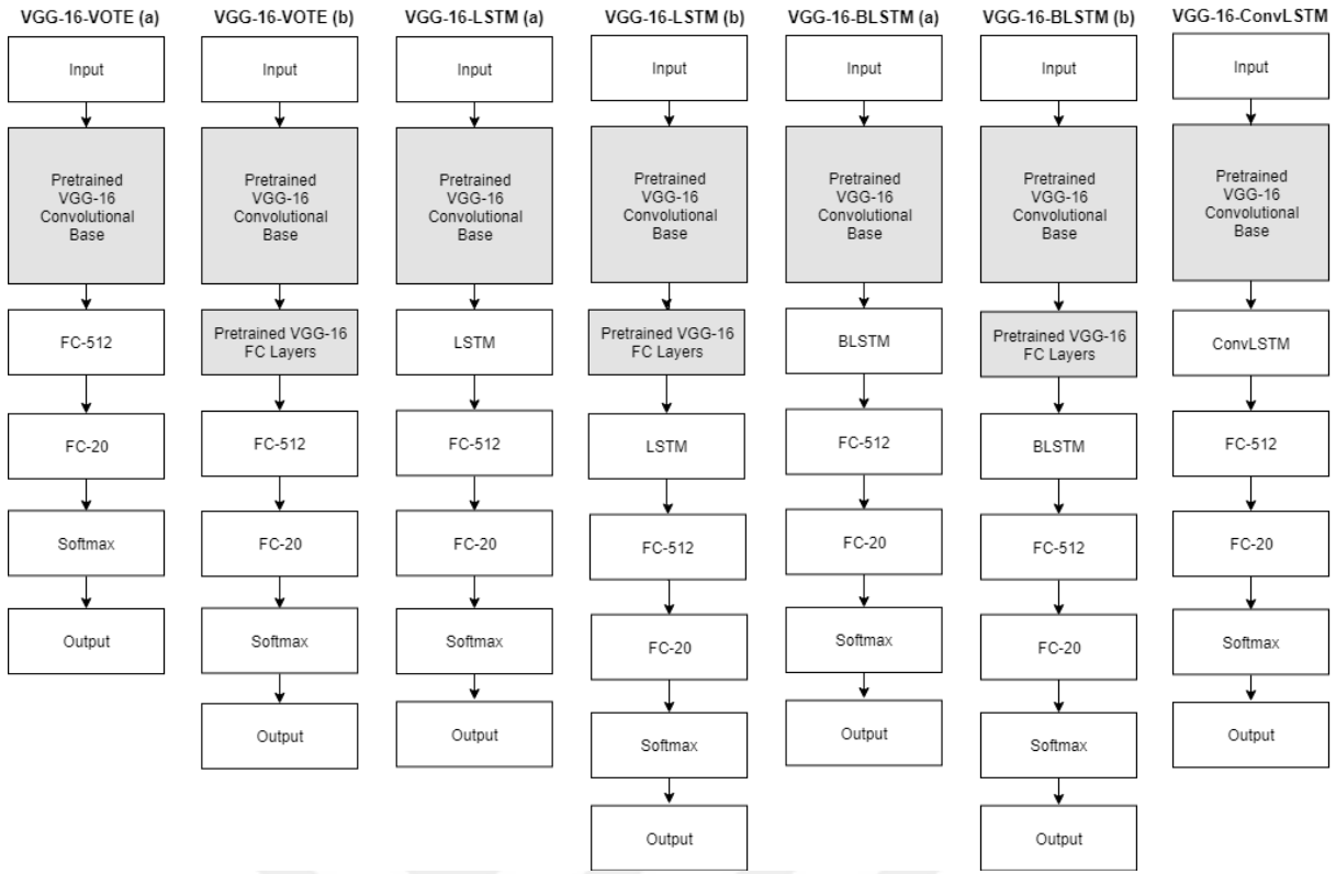
Figure 3.1: The architectures of networks used in the experiment VGG-16-VOTE(a) and VGG-16-VOTE(b) are designed as baseline methods using the pre-trained VGG-16 by [72].
