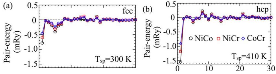
Figure 5.13 Real-space pair-interchange energies to 30 shells calculated at 1.15 T_{sp} for (a) fcc and (b) hcp NiCoCr from an inverse Fourier Transform of S_{\alpha\beta}^{(2)}(\mathbf{k}; T) from supplementary Fig. 10. S_{\alpha\beta}^{(2)}(\mathbf{R}_{0,i-j}; T = 1.15 T_{sp}) for Ni-Co is -0.8 mRy in fcc phase and -1.5 mRy in hcp phase for first shell, and zero for second shell; and only fcc has significant pair-interchange up to 7 th shell.
