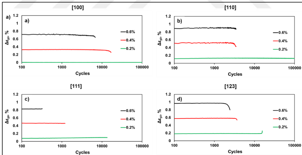
Figure 7.3 Cyclic plastic strain response of the \text{Fe}_{50}\text{Mn}_{30}\text{Co}_9\text{Cr}_9+2 at.% C single crystalline HEA at total strain amplitudes of \Delta\epsilon_t/2 = \pm 0.2\% , \Delta\epsilon_t/2 = \pm 0.4\% and \Delta\epsilon_t/2 = \pm 0.6\% for (a) [100], (b) [110], (c) [111] and (d) [123] orientation.
