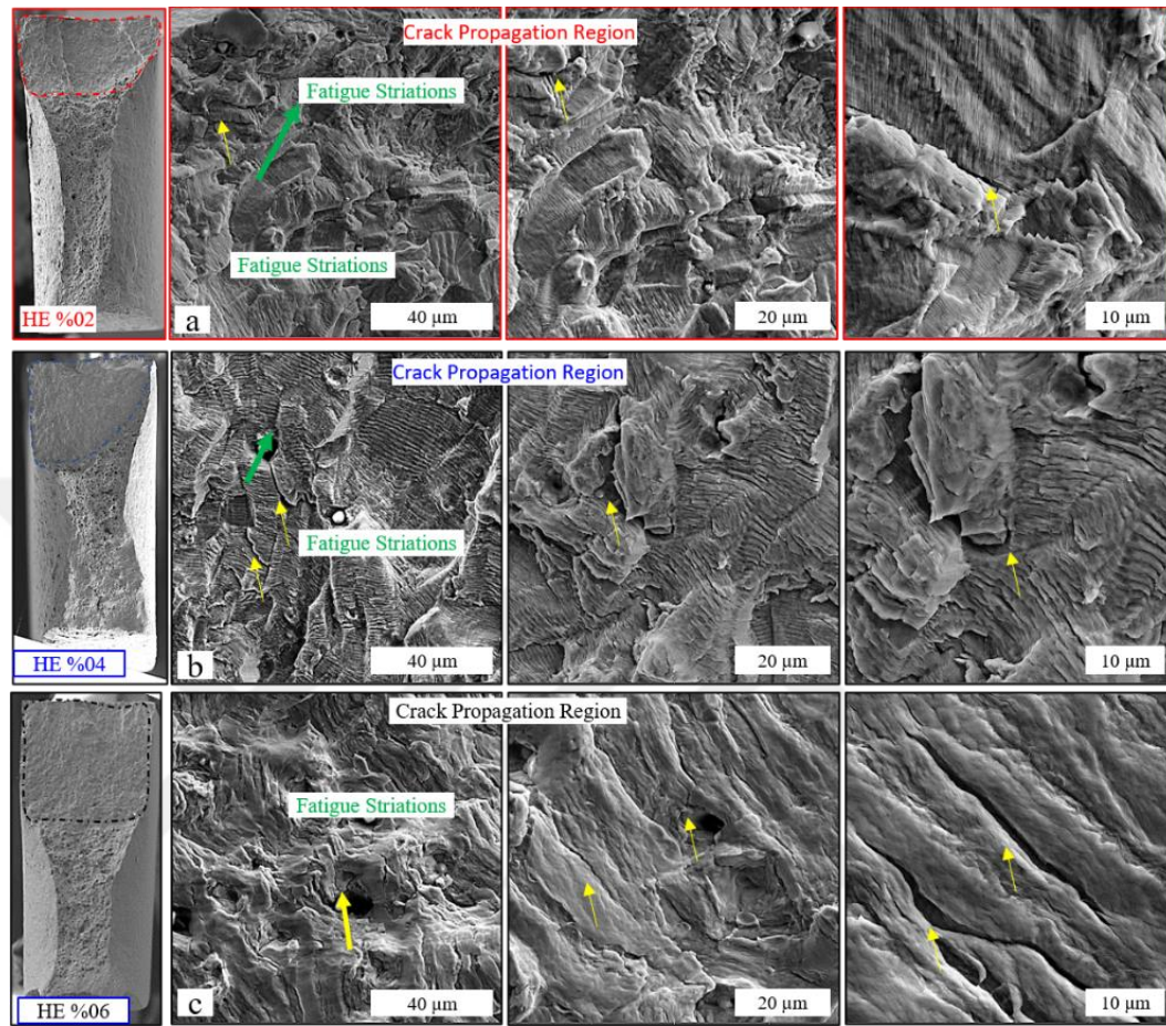
Figure 8.13 SEM images of the fracture features of the hot-extruded CoCrNiFeMn high entropy alloy within the crack propagation region after cyclic loading at different strain amplitudes (a) \Delta\epsilon/2 = \pm 0.2\% , (b) \Delta\epsilon/2 = \pm 0.4\% and (c) \Delta\epsilon/2 = \pm 0.6\% .
