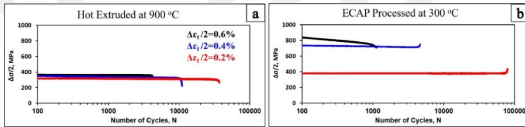
Figure 8.4 Cyclic deformation response of CoCrFeMnNi high entropy alloy in Hot-Extruded (a) and ECAP (b) conditions at the total strain amplitudes of \Delta\epsilon_t/2 = \pm 0.2\% , \Delta\epsilon_t/2 = \pm 0.4\% and \Delta\epsilon_t/2 = \pm 0.6\% .
