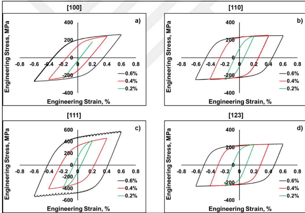
Figure 7.4 Half-life hysteresis loops of the \text{Fe}_{50}\text{Mn}_{30}\text{Co}_9\text{Cr}_9+2 at.% C single crystalline HEA at total strain amplitudes of \Delta\epsilon_t/2 = \pm 0.2\% , \Delta\epsilon_t/2 = \pm 0.4\% and \Delta\epsilon_t/2 = \pm 0.6\% for (a) [100], (b) [110], (c) [111] and (d) [123] orientation.
