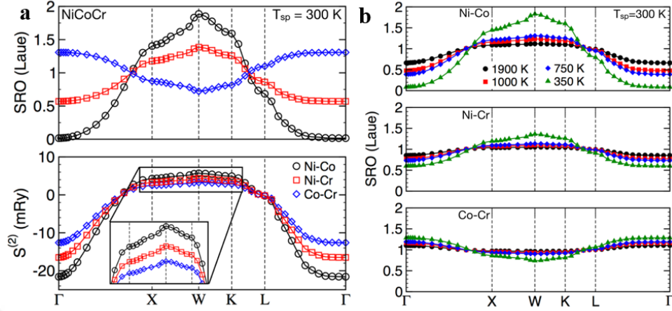
Figure 5.12 (a) For fcc NiCoCr, Warren-Cowley SRO parameters \alpha_{\alpha\beta}(\mathbf{k}; T) [Laue] and pair-interchange energies S_{\alpha\beta}^{(2)}(\mathbf{k}; T) [mRy] calculated at T = 1.15T_{sp} and plotted along high-symmetry directions in the Brillouin zone. The theoretical spinodal decomposition temperature is T_{sp} = 300 K. Maximal SRO is found for Ni-Co pairs at W = (1 \frac{1}{2} 0) . (b) Temperature-dependence of the SRO pairs – see also Fig. 5 – shows Ni-Co pairs persist with temperature.
