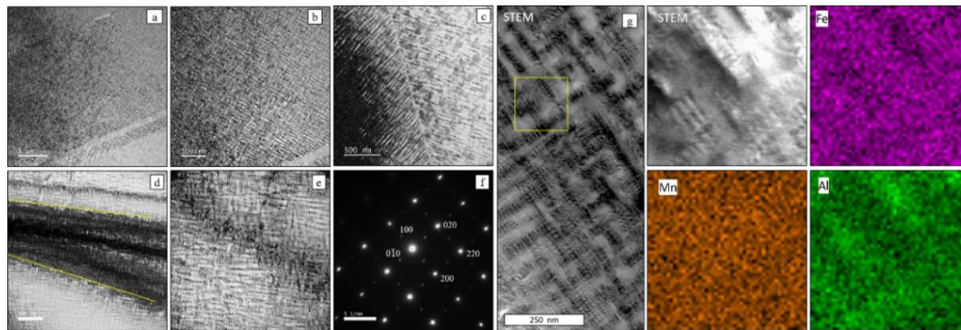
Figure 6.17 (a–e) Transmission electron microscopy (TEM) bright-field images showing \kappa -carbide distribution, (f) corresponding diffraction pattern of (e), (g) the TEM EDSX maps showing the Kappa carbide being Al rich.
