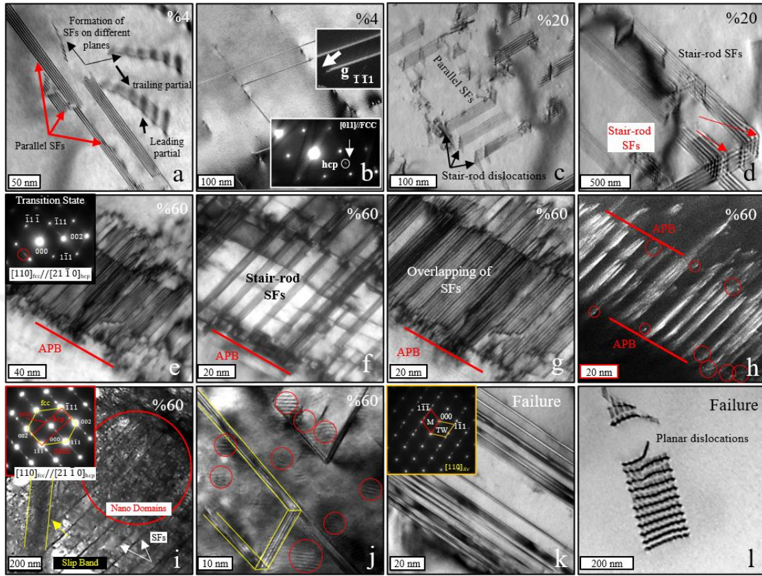
Figure 5.6 Bright-field and dark-field TEM micrographs with corresponding selected-area diffraction patterns (SADPs) demonstrating major deformation mechanisms of the [110]-oriented as-quenched single-crystalline NiCoCr strained to different levels under tension at room temperature (RT). (a) Formation of parallel stacking faults (SFs) on different {111} planes, causing nucleation of widely extended stacking faults (SFs) and precursors to \epsilon -martensite thin plate formation at 4% strain. The extended coplanar Shockley partials and SFs lead to formation of (b) \epsilon -martensite hcp plates at 4% strain, insets : diffraction patterns and dark-field image, (c) the nucleation of the stair-rod type SFs at 20% strain, (d) a well-developed stair-rod SF at 20% strain, (e) high density SFs at 60% strain, representing an anti-phase boundary with a corresponding SADP that indicates a transition state, (f-g) the same region (e) taken with a different tilting angle and showing stair-rod stacking faults in the same region, and (h) dark filed image taken from diffuse intensity on the SADP inset (e) marked with red circle, (i) nano domains at % 60 strain, proving the occurrence of the hexagonal D0_{19} structure with the corresponding SADP inset, (j) higher magnification of nano domains, (k) nanotwins bundle with corresponding diffraction pattern inset, and (l) planar slip localization at failure.
