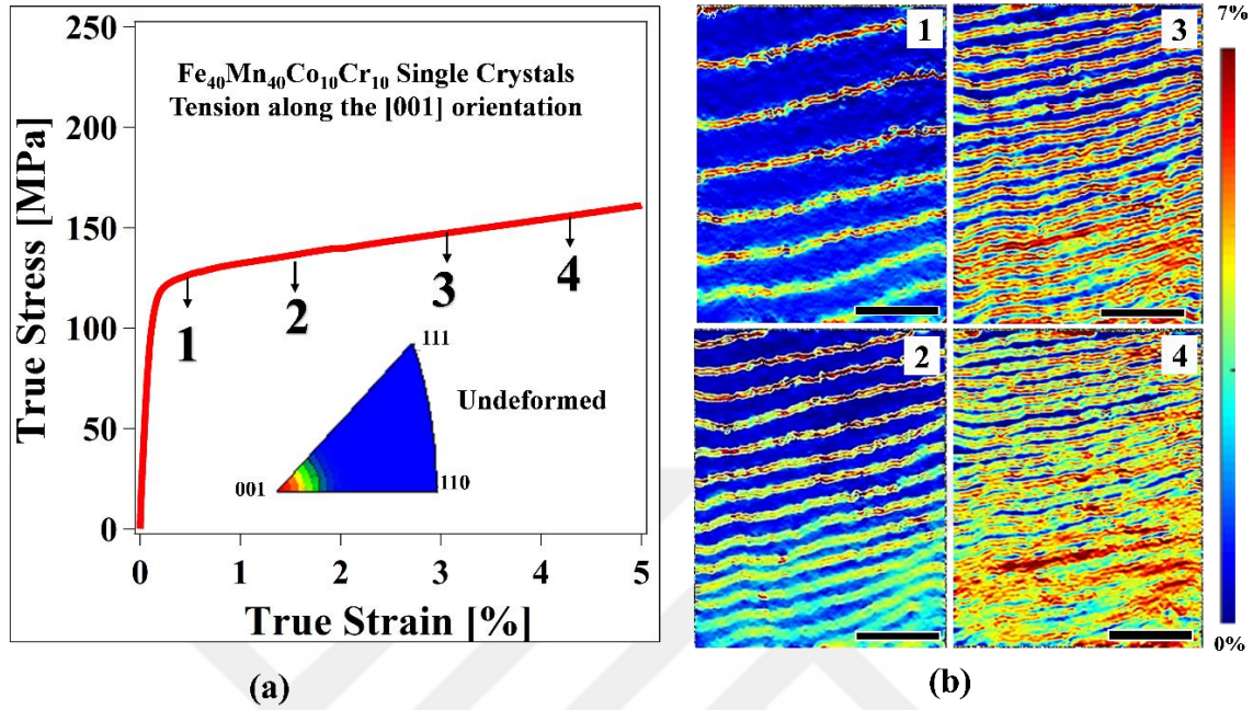
Figure 4.4 (a) The room temperature tensile stress-strain response of the [001] single crystals of Fe 40 Mn 40 Co 10 Cr 10 deformed up to 5% strain. Inverse pole figures demonstrate the initial orientation of the sample (b) In-situ DIC images show the normal ( \epsilon_{yy} ) strain maps at four different strain levels (1, 2, 3, and 4) marked in (a). Each scale bar represents a length of 1 mm.
