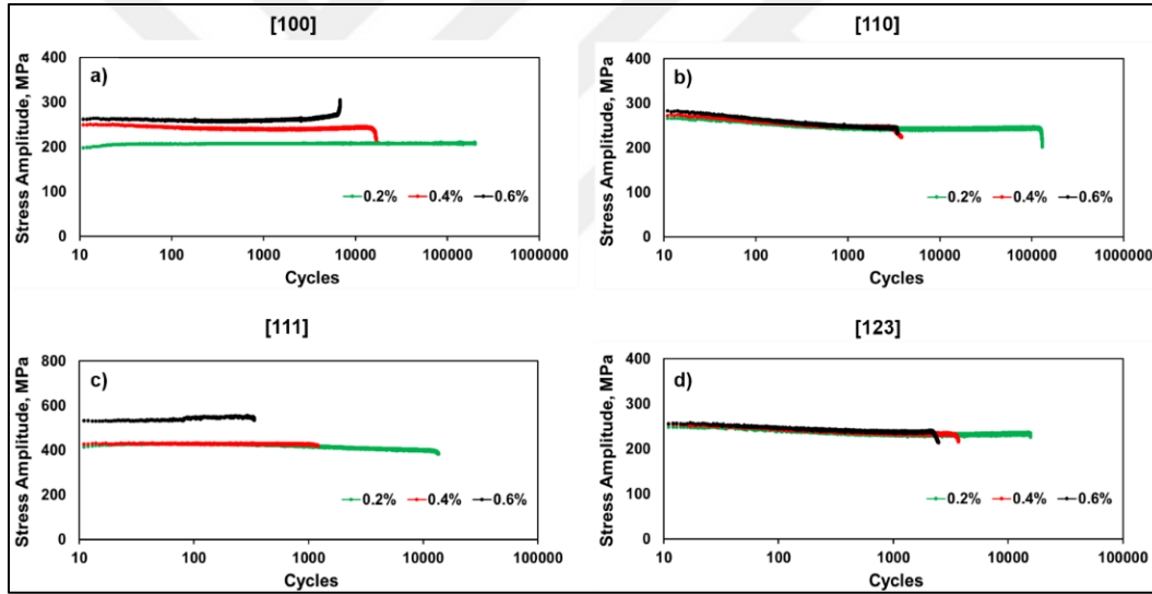
Figure 7.2 Cyclic deformation response of the Fe 50 Mn 30 Co 9 Cr 9+2 at.% C single crystalline HEA at total strain amplitudes of \Delta\epsilon_t/2 = \pm 0.2\% , \Delta\epsilon_t/2 = \pm 0.4\% and \Delta\epsilon_t/2 = \pm 0.6\% for (a) [100], (b) [110], (c) [111] and (d) [123] orientation.
