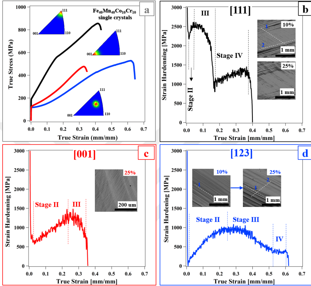
Figure 4.1 (a) The room temperature true stress - true strain tension responses of the [111], [001]- and [123]-oriented single crystals of the Fe 40 Mn 40 Co 10 Cr 10 HEA. Inverse pole figures show the initial loading directions for three orientations, measured using EBSD. The evolution of \theta ( d\sigma/d\epsilon ), with true strain for the (b) [111], (c) [001] and (d) [123]-oriented crystals. Optical microscopy insets provide the surface relieves at different strain levels indicated. The stages of deformation were also marked for each orientation.
