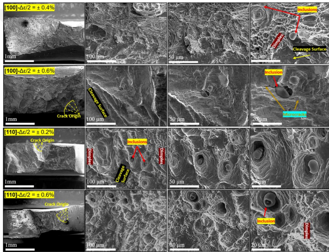
Figure 7.12 Fracture surfaces of Fe 50 Mn 30 Co 9 Cr 9 + 2 at.% C high entropy alloy in single crystals fatigued at different strain amplitudes. Higher magnifications of fracture are displayed to the right.
