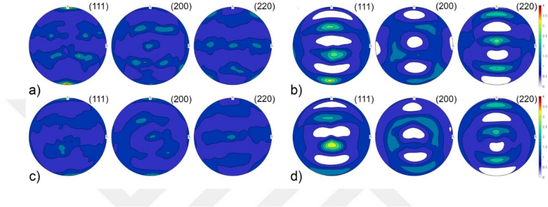
Figure 8.16 Pole figures of the main planes for the CoCrNiFeMn high entropy alloy samples (a) the plane perpendicular to the extrusion directions of the HE sample, (b) the plane perpendicular to the longitudinal direction of the ECAP sample. The same pole figures on the same planes after LCF testing at \Delta\epsilon/2 = \pm 0.6\% for (c) the HE sample, (d) the ECAP sample.
