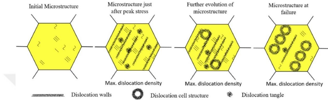
Figure 8.9 Schematic illustration of the formation of the cell structures in CoCrNiFeMn high entropy alloy under push-pull low-cycle fatigue loading.
