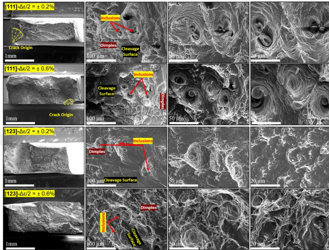
Figure 7.13 Fracture surfaces of [111] and [123] oriented single crystalline \text{Fe}_{50}\text{Mn}_{30}\text{Co}_9\text{Cr}_9 + 2 \text{ at.}\% \text{ C} HEAs fatigued at different strain amplitudes. Higher magnifications of fracture are displayed to the right.
