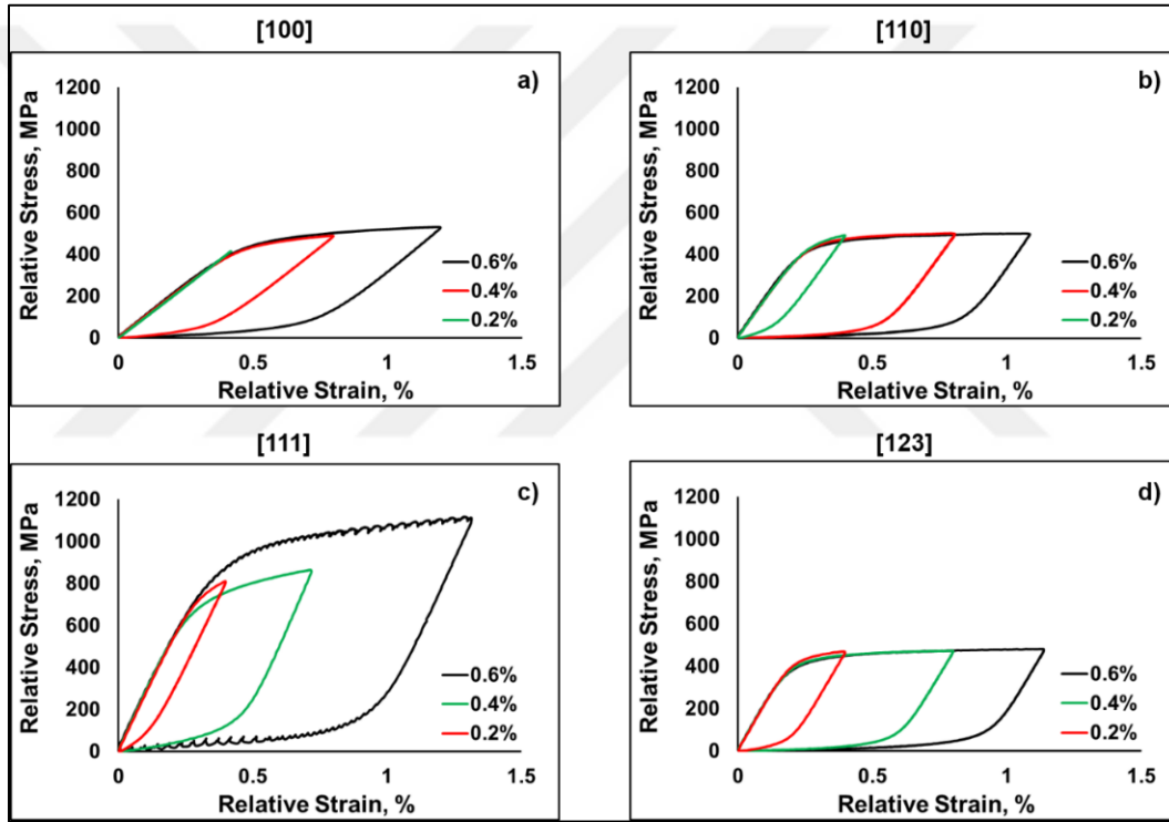
Figure 7.5 Half-life hysteresis loops of the \text{Fe}_{50}\text{Mn}_{30}\text{Co}_9\text{Cr}_9+2 \text{ at.}\% \text{ C} single crystalline HEA at total strain amplitudes of \Delta\epsilon_t/2 = \pm 0.2\% , \Delta\epsilon_t/2 = \pm 0.4\% and \Delta\epsilon_t/2 = \pm 0.6\% for (a) [100], (b) [110], (c) [111] and (d) [123] orientation plotted in relative coordinates of stress and strain.
