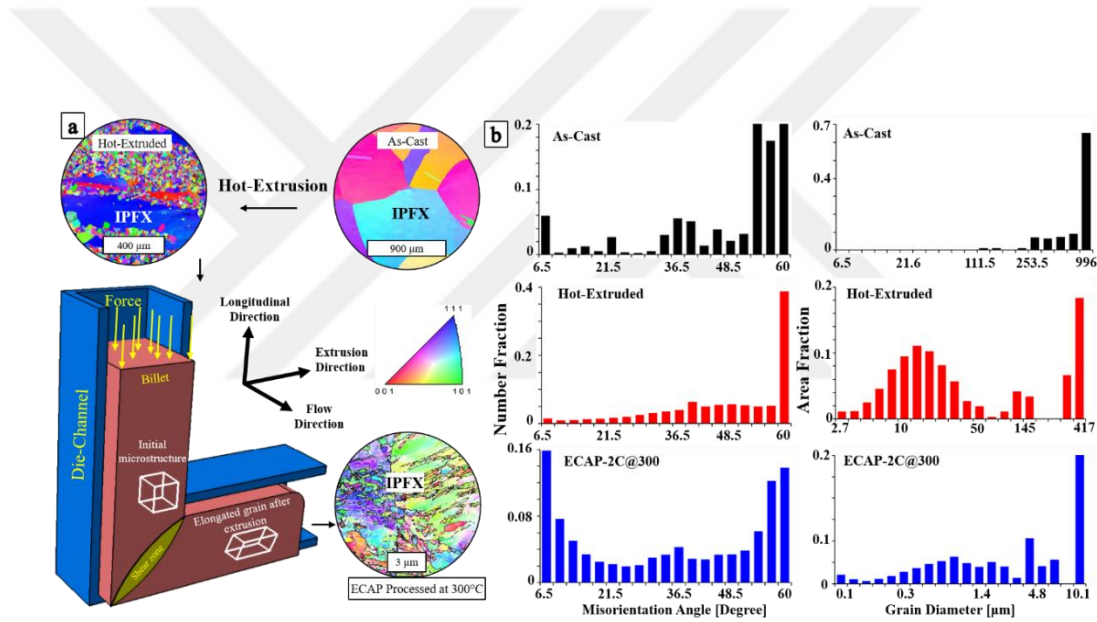
Figure 8.1 (a) Schematic of the ECAP processing depicting the relevant directions of the billet after the process, and orientation mapping, obtained through electron back scatter diffraction (EBSD) imaging, of CoCrFeMnNi high entropy alloy, (b) the histograms of the grain boundary misorientation angles and grain diameters of the EBSD micrographs shown in (a).
