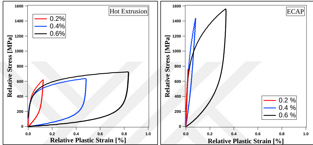
Figure 8.7 Half-life hysteresis loops of CoCrFeMnNi high entropy alloy in Hot-Extruded (a) and ECAP (b) conditions plotted in relative coordinates for the different total strain amplitudes of \Delta\epsilon/2 = \pm 0.2\% , \Delta\epsilon/2 = \pm 0.4\% and \Delta\epsilon/2 = \pm 0.6\% .
