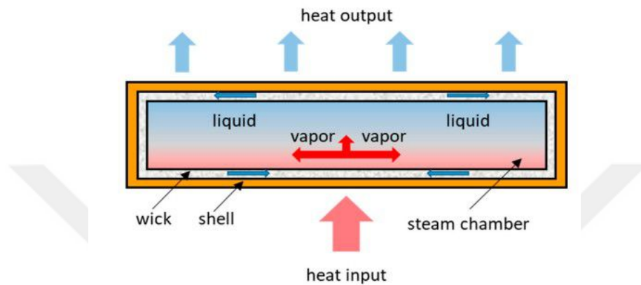
Figure 1.2: Vapor chamber scheme and working cycle [8]
