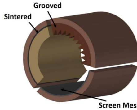
(a) Sintered, grooved and screen mesh wick structures [24]
