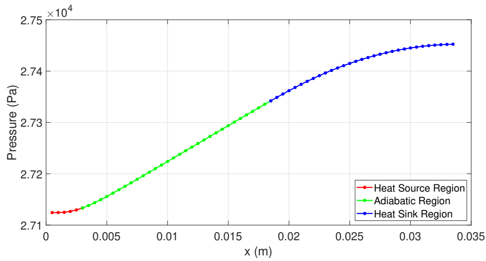
Figure 3.12: Pressure distribution plot
