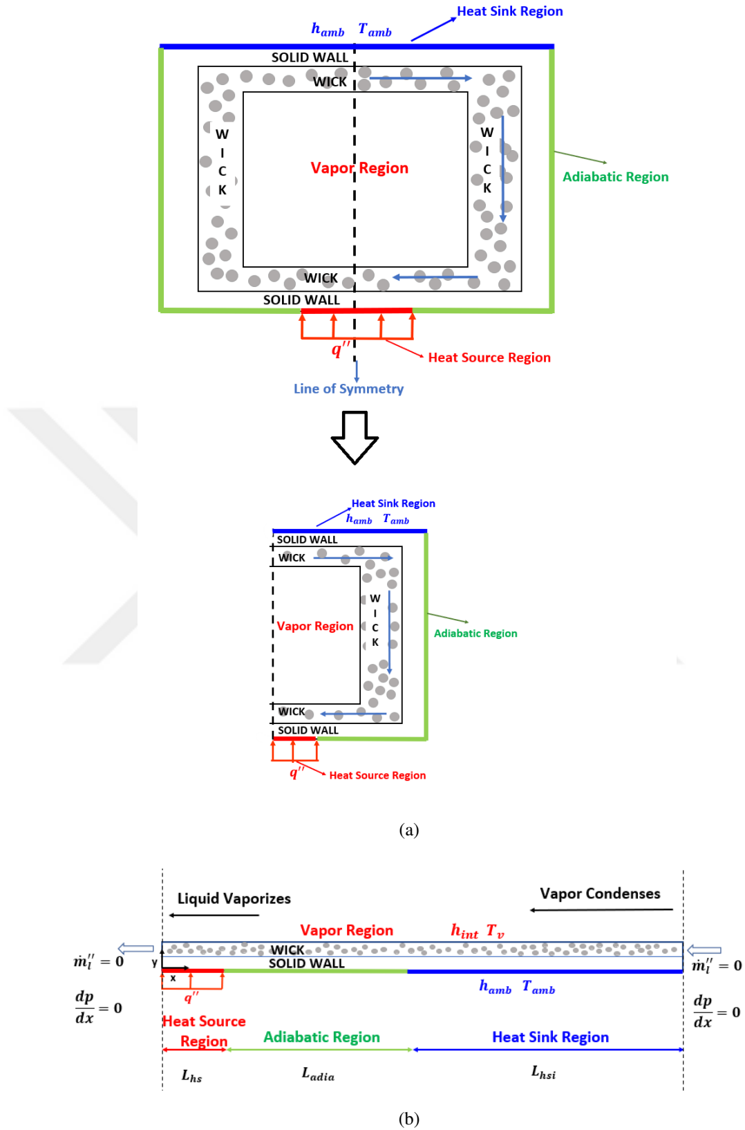
Figure 3.1: Schematic diagram of the vapor chamber
