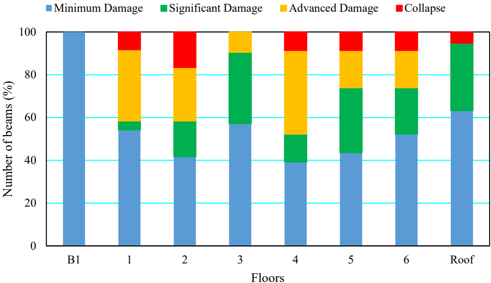
Figure 4.13 As-built building beam assessment for +X direction.
