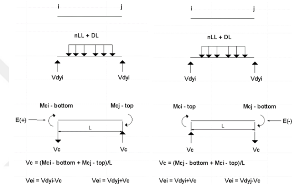
Figure 4.6 Shear demand calculation at the end of the beams.
