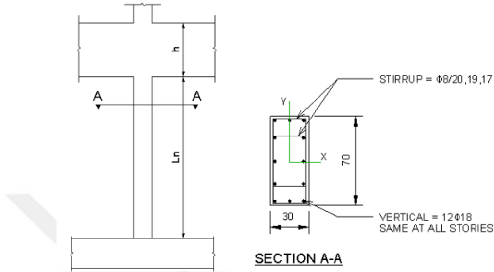
Figure 4.9 Elevation and section of column S19 (dimensions in cm).
