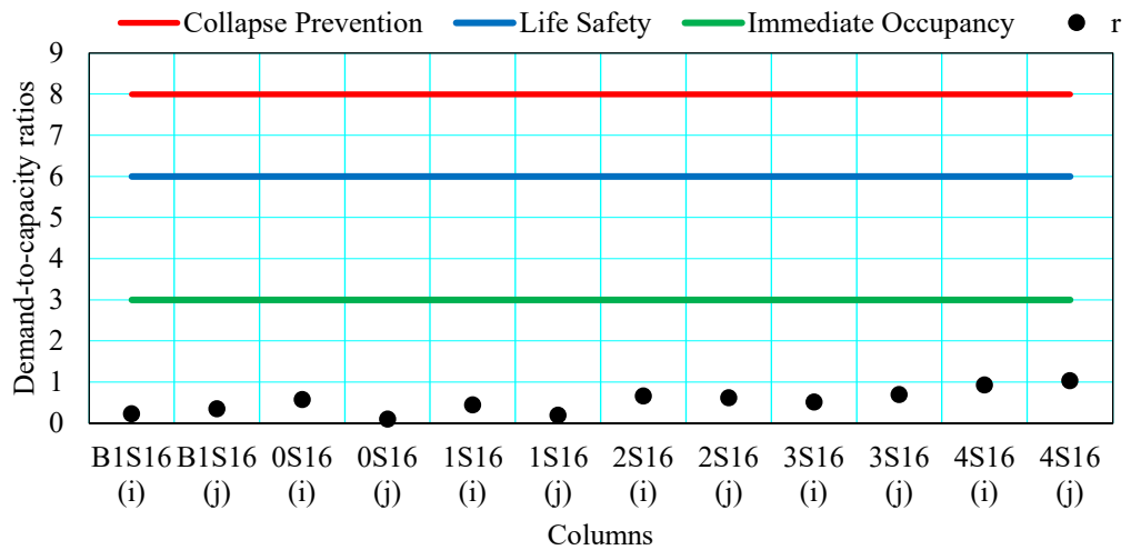
Figure 4.22 Demand-to-capacity ratio for column S16 of the post-retrofit building.
