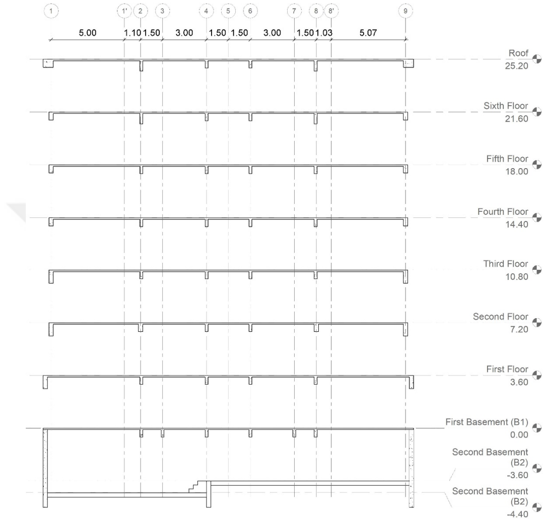
Figure 3.2 Building section A-A (see Figure 3.3; dimensions in m).
