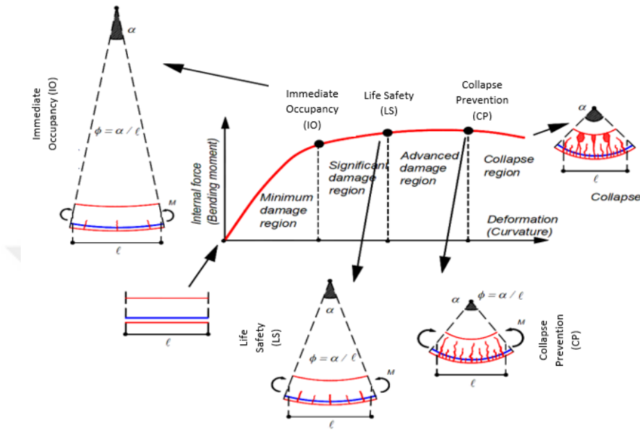
Figure 4.5 Damage states for ductile members [Celep 2014].
