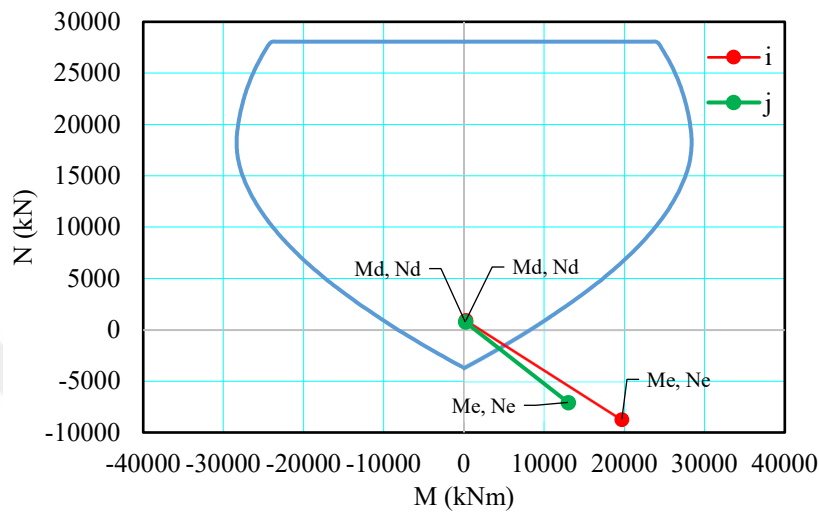
Figure 4.23 Demand-to-capacity ratio calculation for column PB11' on the second floor.
