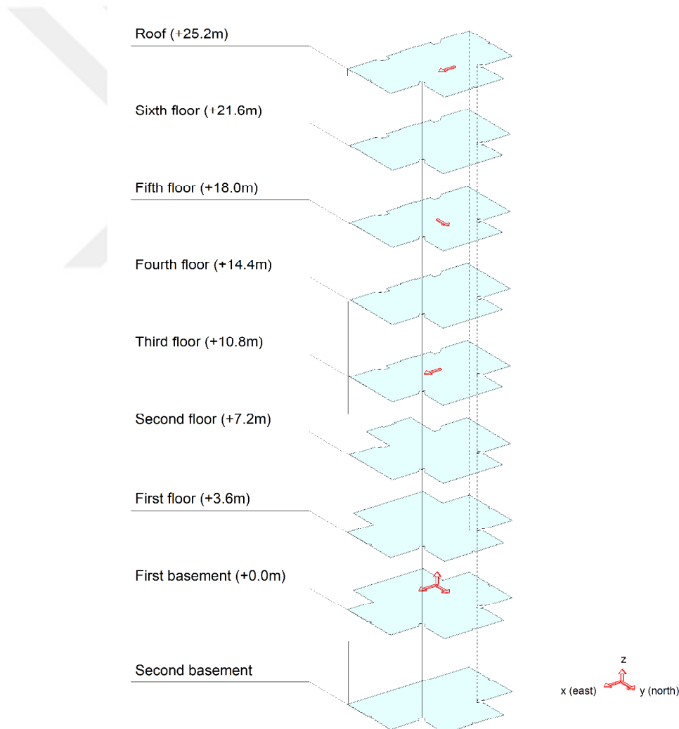
Figure 3.10 Instrumentation scheme for the as-built building.
