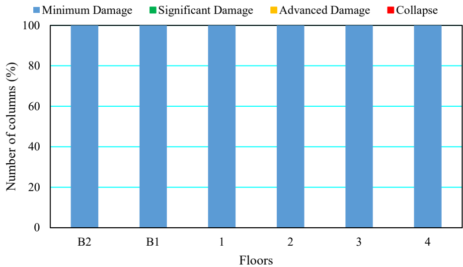
Figure 4.28 Post-retrofit building column assessment for +X direction.
