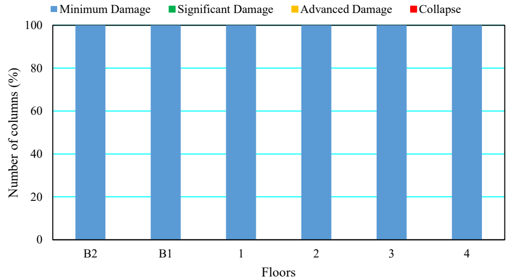
Figure 4.27 Post-retrofit building column assessment for +Y direction.
