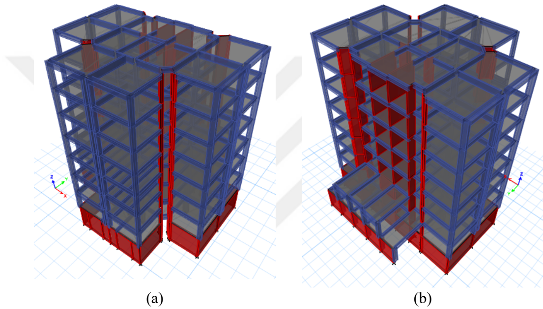
Figure 3.13 3-D views of the finite element model of the as-built building from (a) SE and (b) NW corners.
