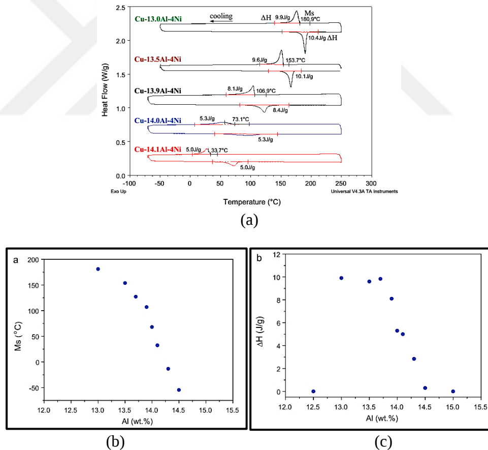
Figure 2.5. The characteristics of transformation temperatures are (a) Heating and cooling curves, the effect of weight percentage of Al on the (b) martensite transformation temperature, and (c) enthalpy of the transformation [71].
