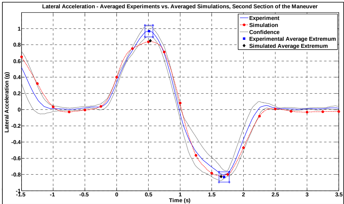
Figure 4.34 Lateral Acceleration EDZ vs. Averaged Simulation – The Second Move
