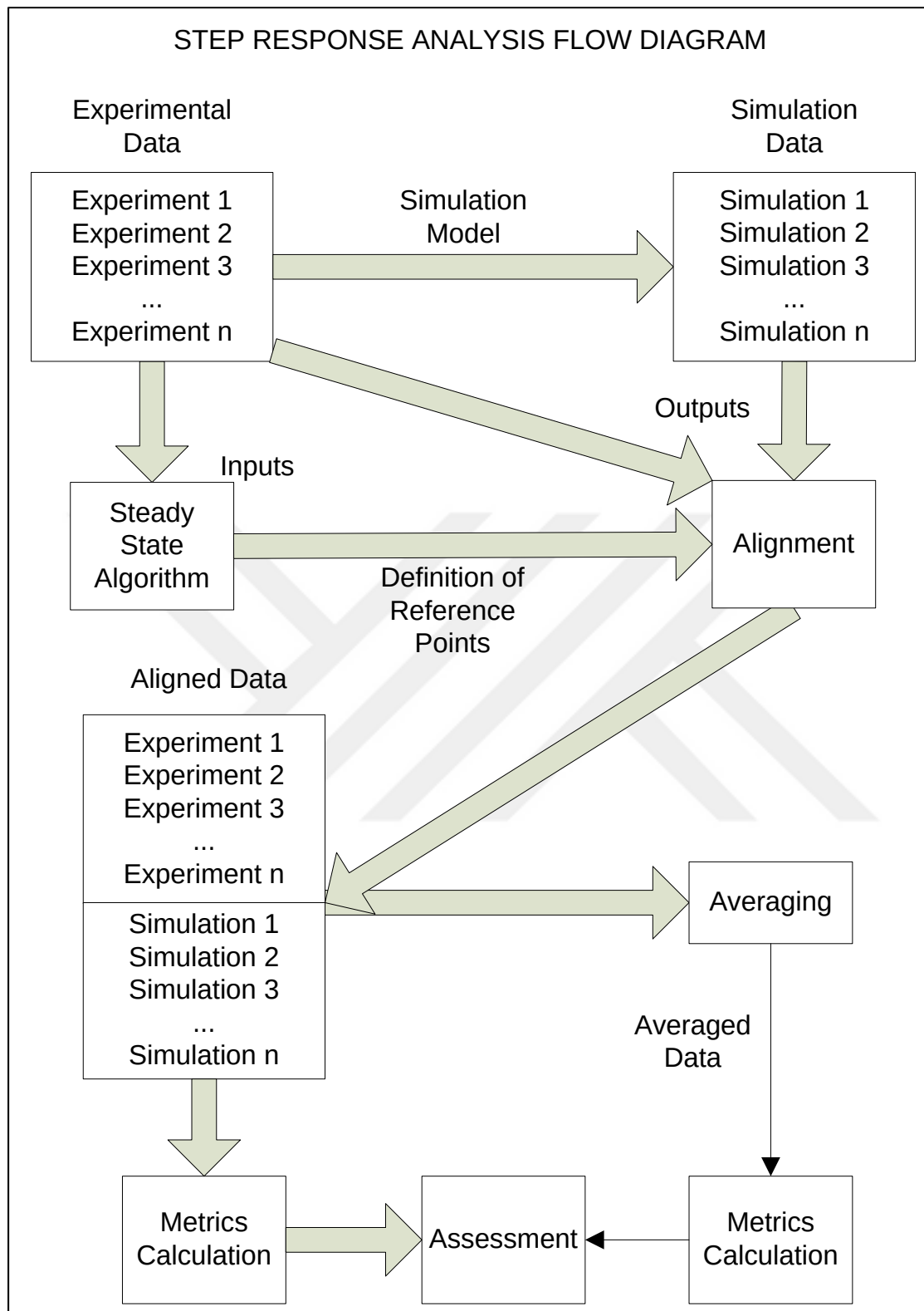
Figure 4.8 Step Response Analysis Methodology
