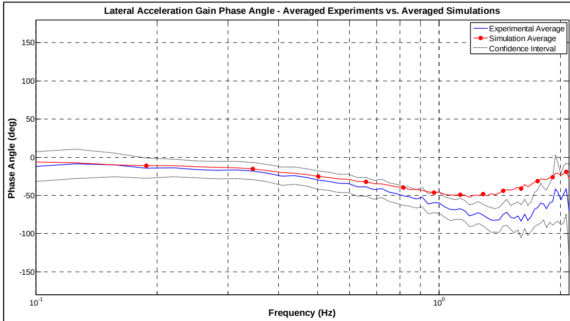
Figure 4.17 Lateral Acceleration Phase Angle
