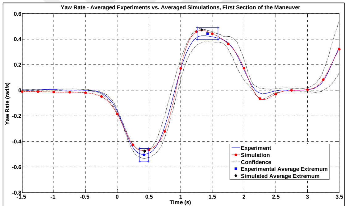
Figure 4.35 Yaw Rate EDZ vs. Averaged Simulation – The First Move
