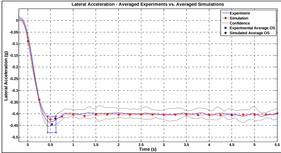
Figure 4.9 Lateral Acceleration EDZ vs. Averaged Simulation
