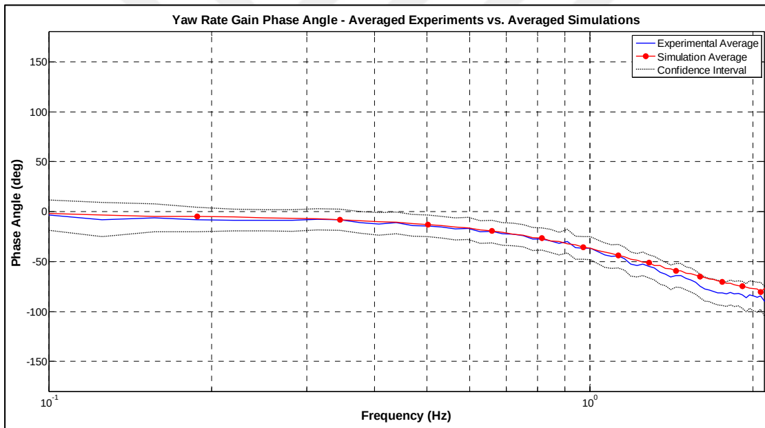
Figure 4.18 Yaw Rate Phase Angle
