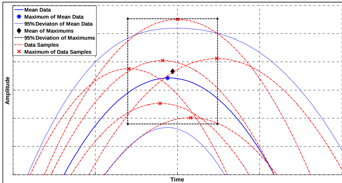
Figure 4.7 Graphical Explanation of MVW Concept: The extremum (and the deviations) obtained by averaging the signals, is not equal to the average (and the deviation) of the extrema of the signals.
