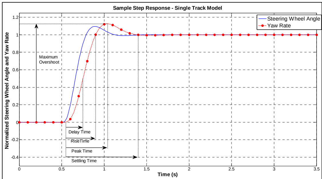
Figure 4.4 Sample Yaw Rate Step Response (Single Track Model Simulation)
