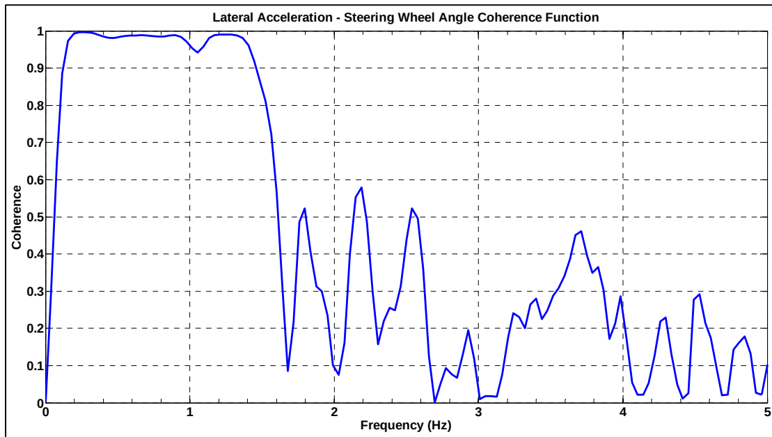
Figure 4.13 Sample Coherence Function of the Lateral Acceleration
