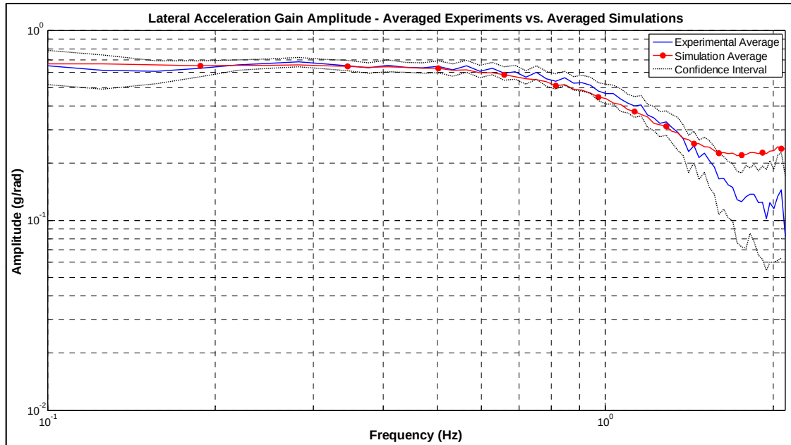
Figure 4.15 Lateral Acceleration Response Gain
