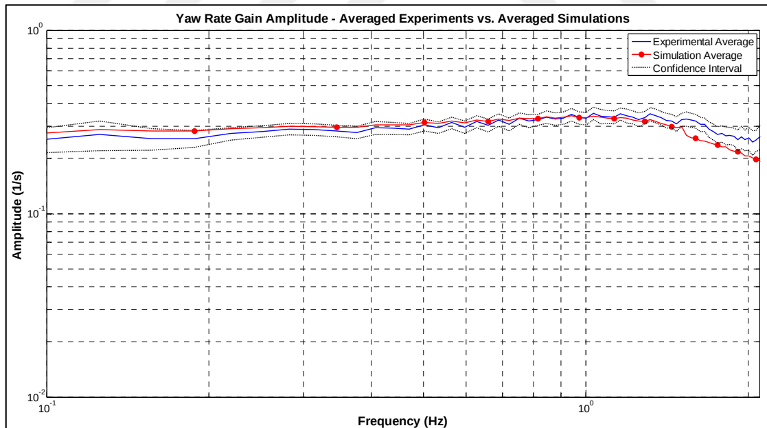
Figure 4.16 Yaw Rate Response Gain
