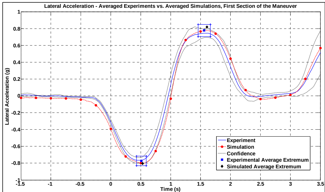
Figure 4.33 Lateral Acceleration EDZ vs. Averaged Simulation – The First Move
