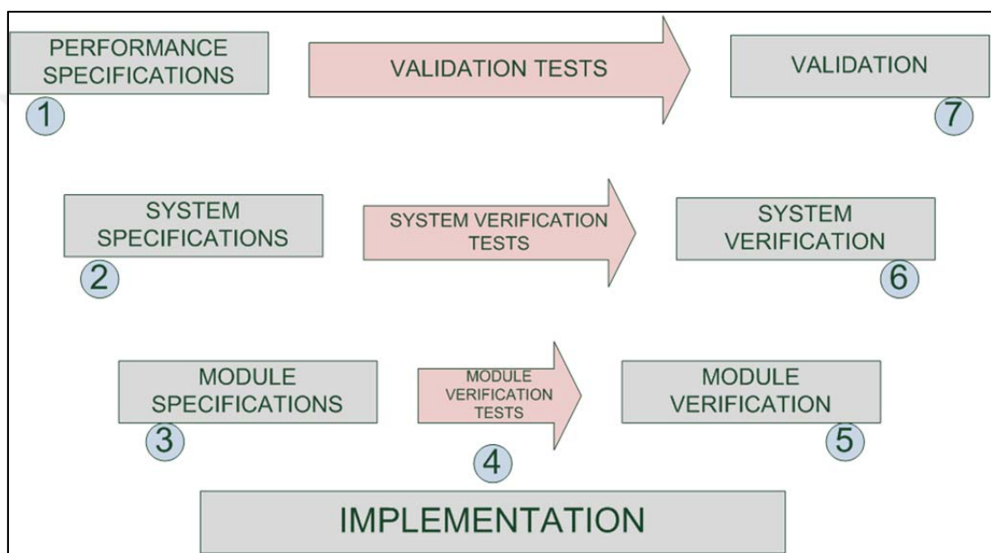
Figure 3.4 The V-Model
