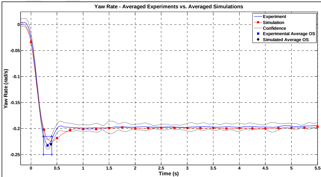
Figure 4.10 Yaw Rate EDZ vs. Averaged Simulation
