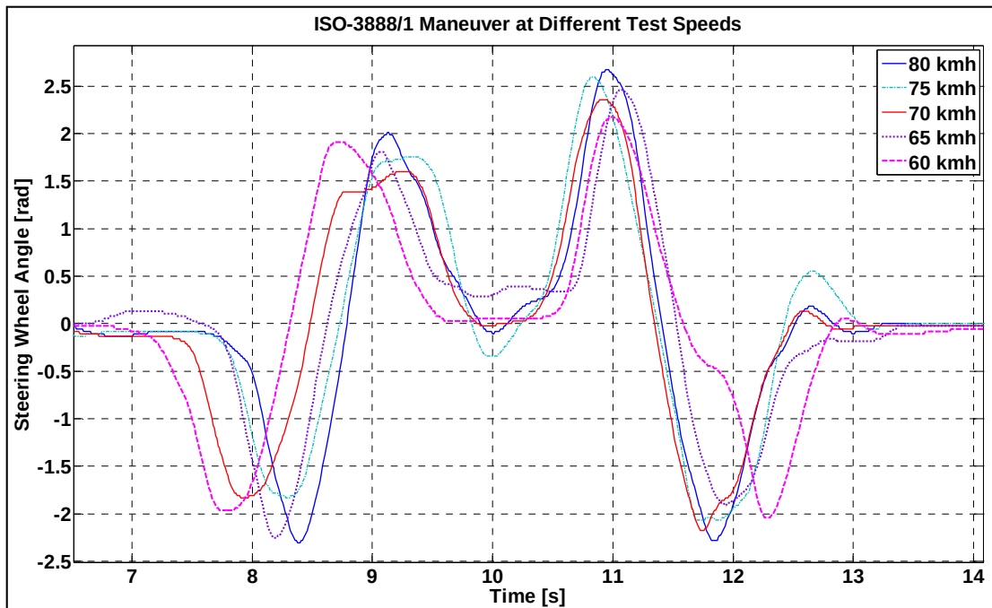
Figure 4.19 Time histories of double lane change maneuver for different test speeds
