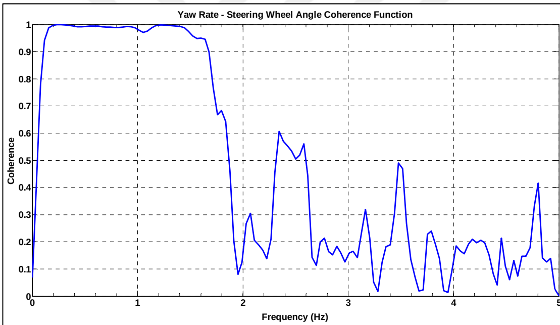
Figure 4.14 Sample Coherence Function of the Yaw Rate
