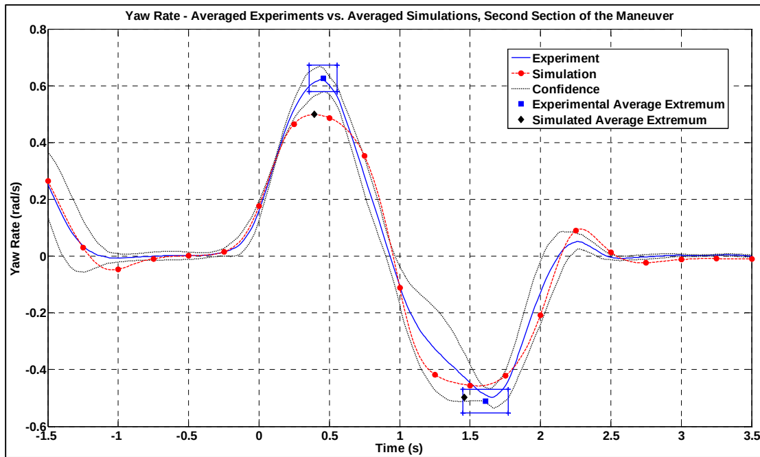
Figure 4.36 Yaw Rate EDZ vs. Averaged Simulation – The Second Move
