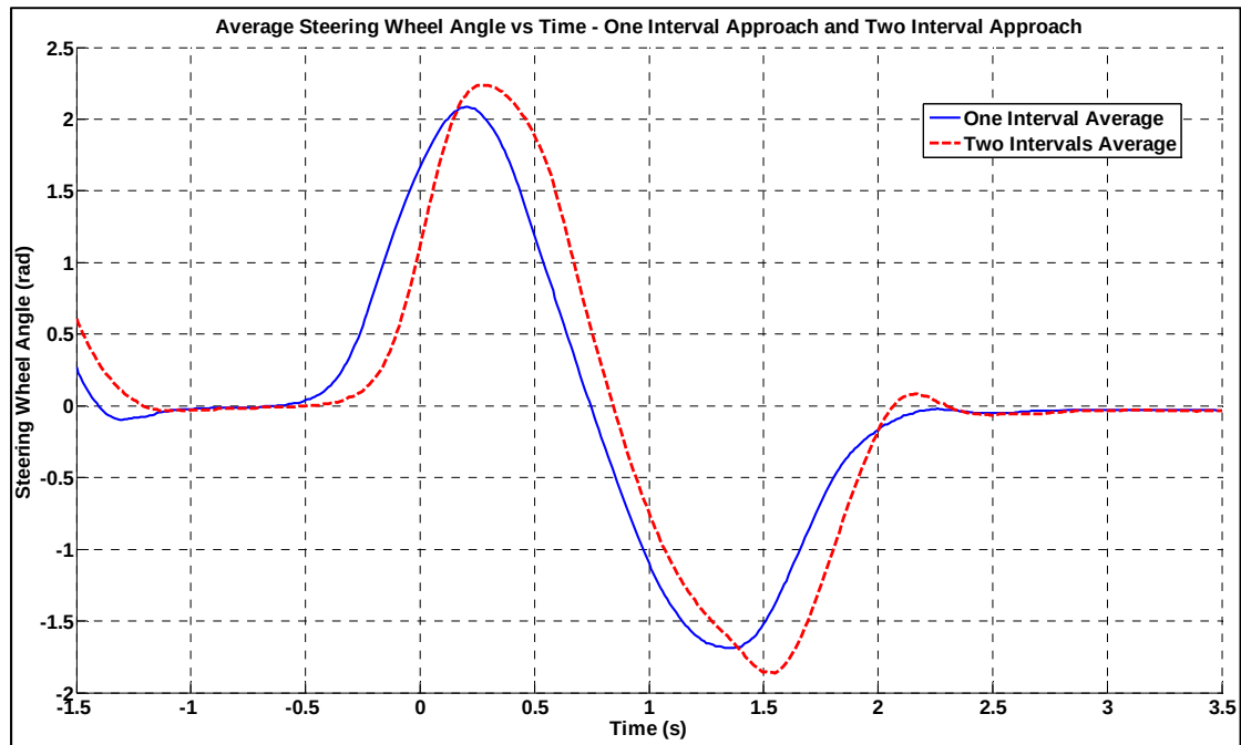
Figure 4.32 Comparison of Average Steering Wheel Angles
