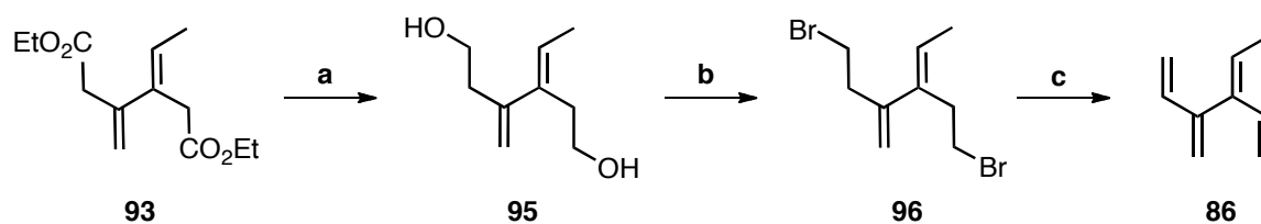
Scheme 1.27: Preparation of 4-( E )-methyl [4]dendralene 86 . Reagents and conditions: (a) \text{LiAlH}_4 (2.0 mol equiv), \text{Et}_2\text{O} , 0 °C, 30 min, then rt, overnight, 97%; (b) NBS (2.0 mol equiv), \text{PPh}_3 (2.0 mol equiv), \text{CH}_2\text{Cl}_2 , -78 °C to rt, overnight, 40%; (c) DBU (6.4 mol equiv), DMSO, rt, 50 mmHg, 15 min, then 15 mmHg, 2 h, 60%.
