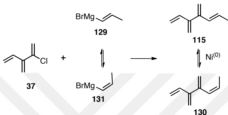
Scheme 1.41: Possible routes to the formation of 1-( E )-methyl [4]dendralene 115 and 1-( Z )-methyl [4]dendralene 130 .
