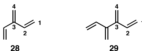
Figure 1.3: [3]dendralene 28 and [4]dendralene 29 .
