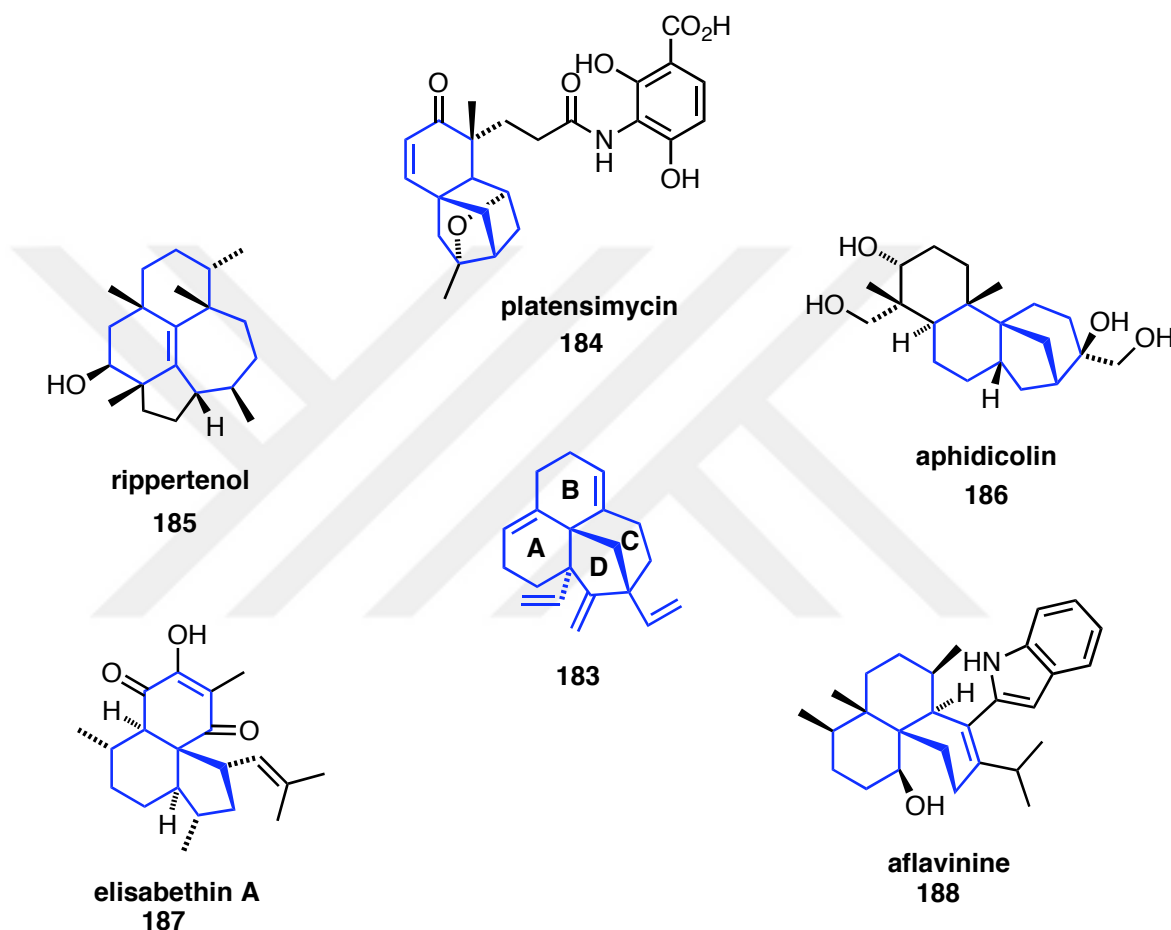
Figure 2.3: Tetracycline 183 and structurally related natural products.
