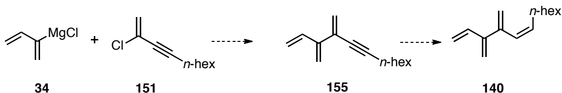
Scheme 1.53: New approach to 1-(Z)-hexyl [4]dendralene 140 .
