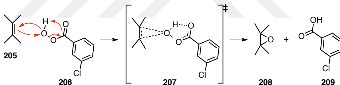
Scheme 2.13: Epoxidation of an alkene 205 using m -CPBA 206 . 5
