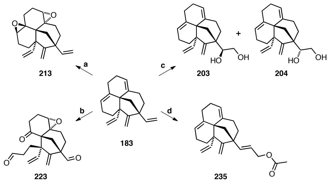
Scheme 2.24: Summary of manipulation of tetracycle 183 . (a) DMDO in acetone (2 mol equiv), rt, 2 h, 37% 213 ( bis -epoxide) and 9% ( mono -epoxides); (b) O 3 (excess), CH 2 Cl 2 , 15 min, –78 °C, then PPh 3 (6 mol equiv), –78 °C to 0 °C, 30 min, 8%; (c) OsO 4 (4.1% in H 2 O solution) (0.04 mol equiv), THF/H 2 O/ t -BuOH (5:1:1 ratio), rt, 4 days, in the dark, 30%; (d) ( Z )-but-2-ene-1,4-diyl diacetate (4 mol equiv), Grubbs II catalyst (0.2 mol equiv), CH 2 Cl 2 , 60 °C, 24 h, 13%.
