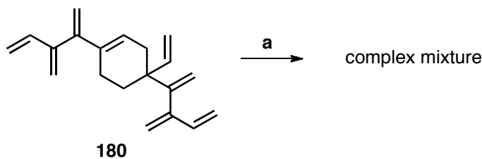
Scheme 2.4: Heat treatment of the major dimer 180 . Reagents and conditions: (a) PhCl, BHT, reflux, 24 h.
