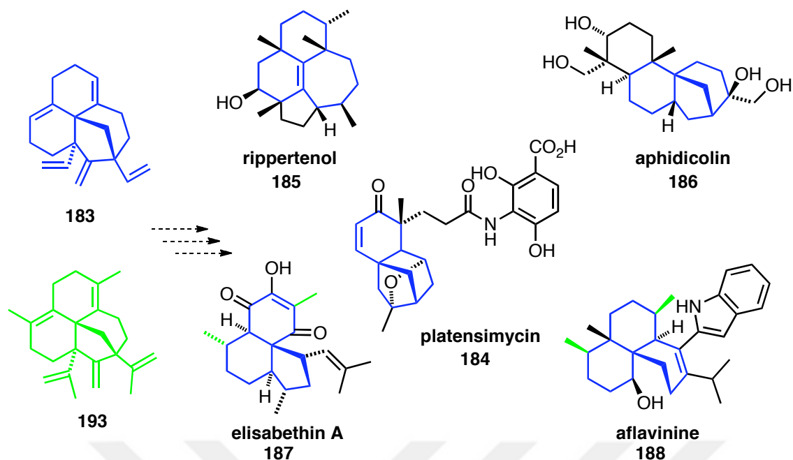
Figure 2.6: Tetracycle 183 , tetracycle 193 and structurally related natural products.
