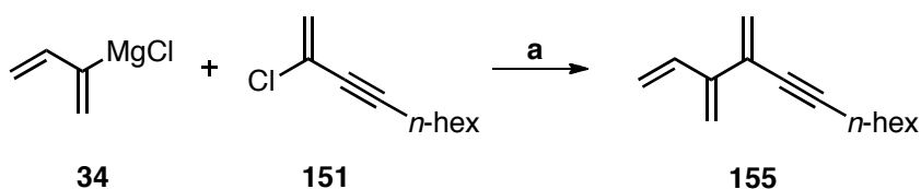
Scheme 1.55: Synthesis C2 alkynyl substituted [3]dendralene 155 . Reagents and conditions: (a) Grignard reagent (3 mol equiv), \text{PPh}_3 (0.05 mol equiv), \text{Ni(dppp)Cl}_2 (0.05 mol equiv), THF, -15\text{ }^\circ\text{C} to 0\text{ }^\circ\text{C} , 2.5 h, 63%.
