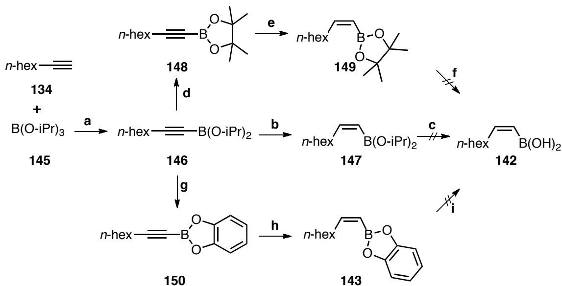
Scheme 1.51: Hydrogenation-based methods towards (Z)- boronic acid 142 . Reagents and conditions: (a) n -BuLi (1.5 M, 1.00 mol equiv), Et 2 O, −78 °C, 30 min, then B(O- i -Pr) 3 (1.00 mol equiv), −78 °C, 2 h, then, HCl (2 M in Et 2 O, 1.03 mol equiv), 94%; (b) Lindlar catalyst, H 2 (ca. 1 mol equiv), pyridine, 1,4-dioxane, in the dark, rt, 1.5 h, without purification; (c) H 2 O, 1h, rt, 11% (over two steps); (d) Pinacol (1.05 mol equiv), Et 2 O, 4 h, rt, 100%; (e) Lindlar catalyst, H 2 (ca. 1 mol equiv), pyridine, pentane, in the dark, rt, 30 min, 87% ( E : Z ratio 20:80); (f) H 2 O, rt, 2 h, no deprotection; (g) Catechol (1.00 mol equiv), Et 2 O, rt, 4 h, 85% (without purification); (h) Lindlar catalyst, H 2 (ca. 1 mol equiv), pyridine, pentane, in the dark, rt, 3.5 h, 22%; (i) H 2 O, rt, 3 h, no deprotection.
