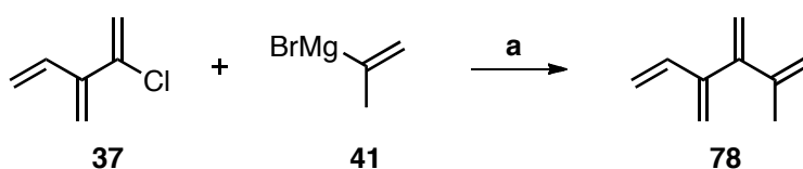
Scheme 1.22: Synthesis of 2-methyl [4]dendralene 78 . Reagents and conditions: (a) Isopropenyl magnesium bromide (1.5 mol equiv), Ni(dppp)Cl 2 (0.040 mol equiv), THF, 0 °C to rt, overnight, 29%.
