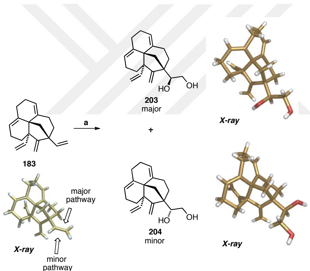
Scheme 2.12: Dihydroxylation reaction of tetracycle 183 and single X-ray crystal structures of the dihydroxylation products 203 and 204 . Reagents and conditions: (a) \text{OsO}_4 (0.04 mol equiv), NMO (2 mol equiv), THF/ \text{H}_2\text{O} / t -BuOH (5:1:1 ratio), rt, 4 days, in the dark, 30%, 203:204 ( ca. 70:30 ratio).
