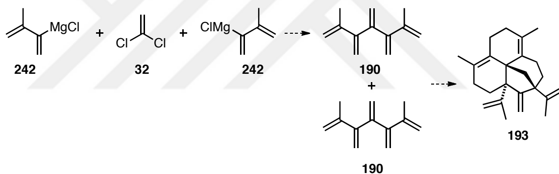
Scheme 2.9: Proposed synthesis of tetracycle 193 .
