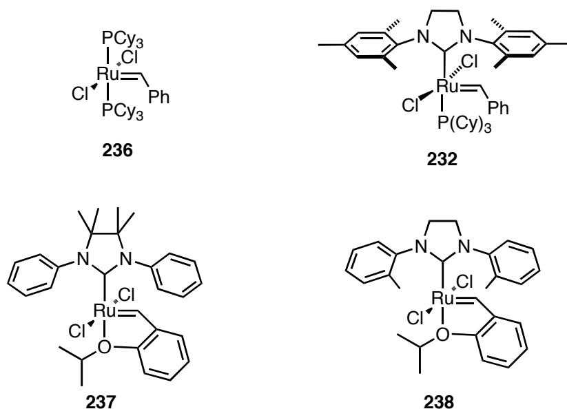
Figure 2.14: Candidate catalysts for the alkene cross-metathesis. 100
