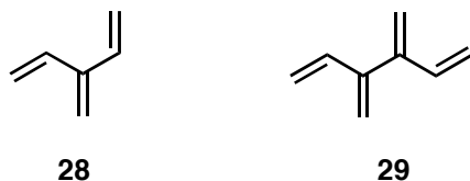
Figure 1.2: [3]dendralene 28 and [4]dendralene 29 .
