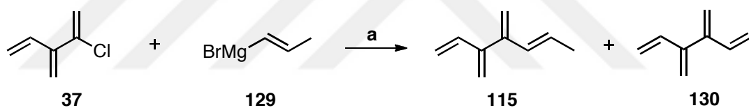
Scheme 1.64: An attempt to synthesise 1-( E )-methyl [4]dendralene 115 . Reagents and conditions: (a) Grignard reagent (1.3 mol equiv), Ni(dppp)Cl 2 (0.10 mol equiv), PPh 3 (0.20 mol equiv), THF, 0 °C to rt, 5 h, (ratios 115 : 130 , 45:55).
