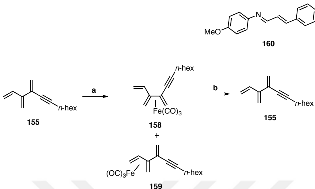
Scheme 1.57: Complexation of C2 alkynyl substituted [3]dendralene 155 with iron tricarbonyl and decomplexation with CAN. Reagents and conditions: (a) \text{Fe}_2(\text{CO})_9 (1.8 mol equiv), aza catalyst 160 (0.35 mol equiv), 1,2-dimethoxyethane, THF, in the dark, 60 °C, 40 h, 158:159 , 30% and 13%, isolated, respectively; (b) CAN (2 mol equiv), acetone, methanol, 0 °C, 30 min, then more CAN (2 mol equiv), 0 °C, 5 min, clean product by ^1\text{H} NMR.
