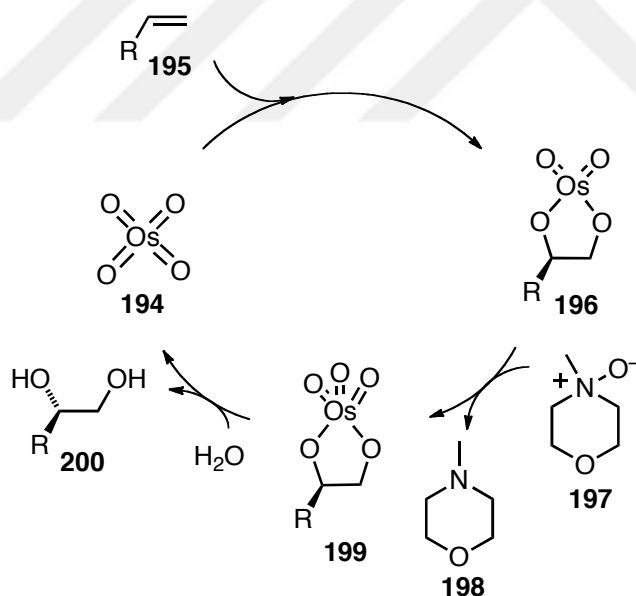
Scheme 2.11: Mechanism of dihydroxylation of an alkene using catalytic amounts of \text{OsO}_4 194 with NMO 197 co-oxidant. 84
