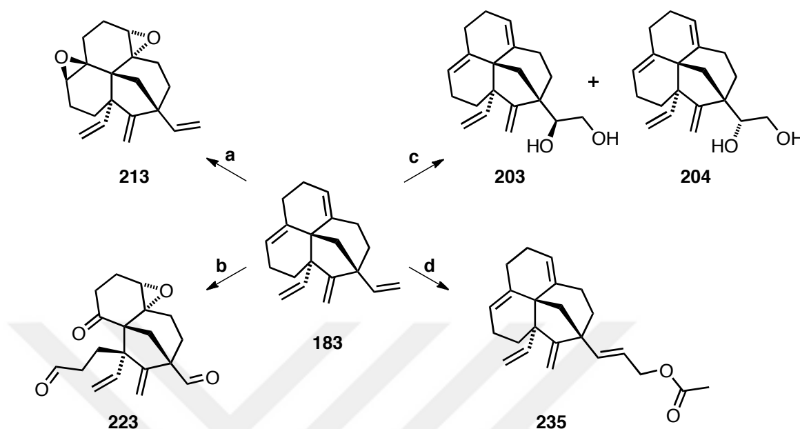
Scheme 2.34: Summary of manipulation of tetracycle 183 . (a) DMDO in acetone (2 mol equiv), rt, 2 h, 37% 213 ( bis -epoxide) and 9% ( mono -epoxides); (b) O_3 (excess), CH_2Cl_2 , 15 min, -78\text{ }^\circ\text{C} , then PPh_3 (6 mol equiv), -78\text{ }^\circ\text{C} to 0\text{ }^\circ\text{C} , 30 min, 8%; (c) OsO_4 (4.1% in H_2O solution) (0.04 mol equiv), THF/ H_2O / t -BuOH (5:1:1 ratio), rt, 4 days, in the dark, 30%; (d) (Z) -But-2-ene-1,4-diyl diacetate (4 mol equiv), Grubbs II catalyst (0.2 mol equiv), CH_2Cl_2 , 60\text{ }^\circ\text{C} , 24 h, 13%.
