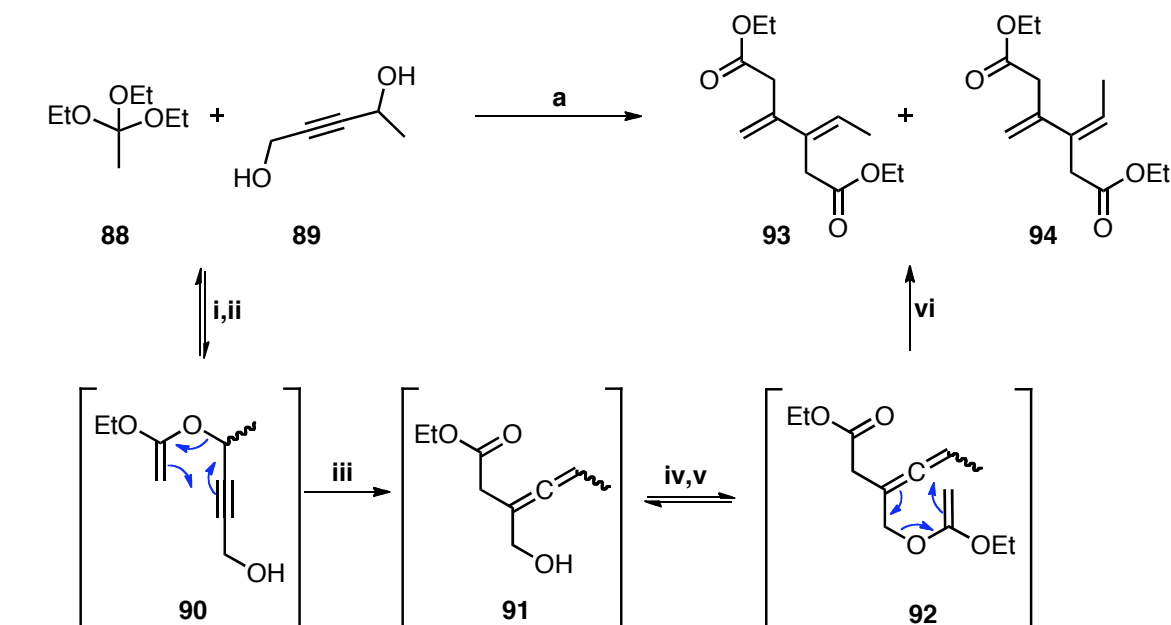
Scheme 1.26: Preparation of E - and Z - diesters 93 and 94 . 35 Reagents and conditions: (a) \text{CH}_3\text{C}(\text{OEt})_3 (9.1 mol equiv), \text{C}_2\text{H}_5\text{CO}_2\text{H} , DMF, 180 °C, 300 W microwave irradiation, 25 min, 73% (ratio E - to Z - isomer 93 and 94 , respectively 47:53); i) acetal exchange step ii) elimination step iii) [3,3]-sigmatropic rearrangement step iv) acetal exchange step v) elimination step vi) [3,3]-sigmatropic rearrangement step.
