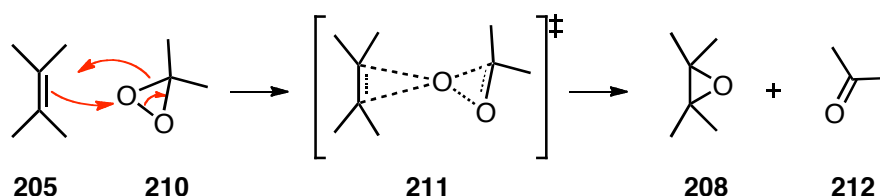
Scheme 2.14: Epoxidation of an alkene 205 using DMDO 210 . 91
