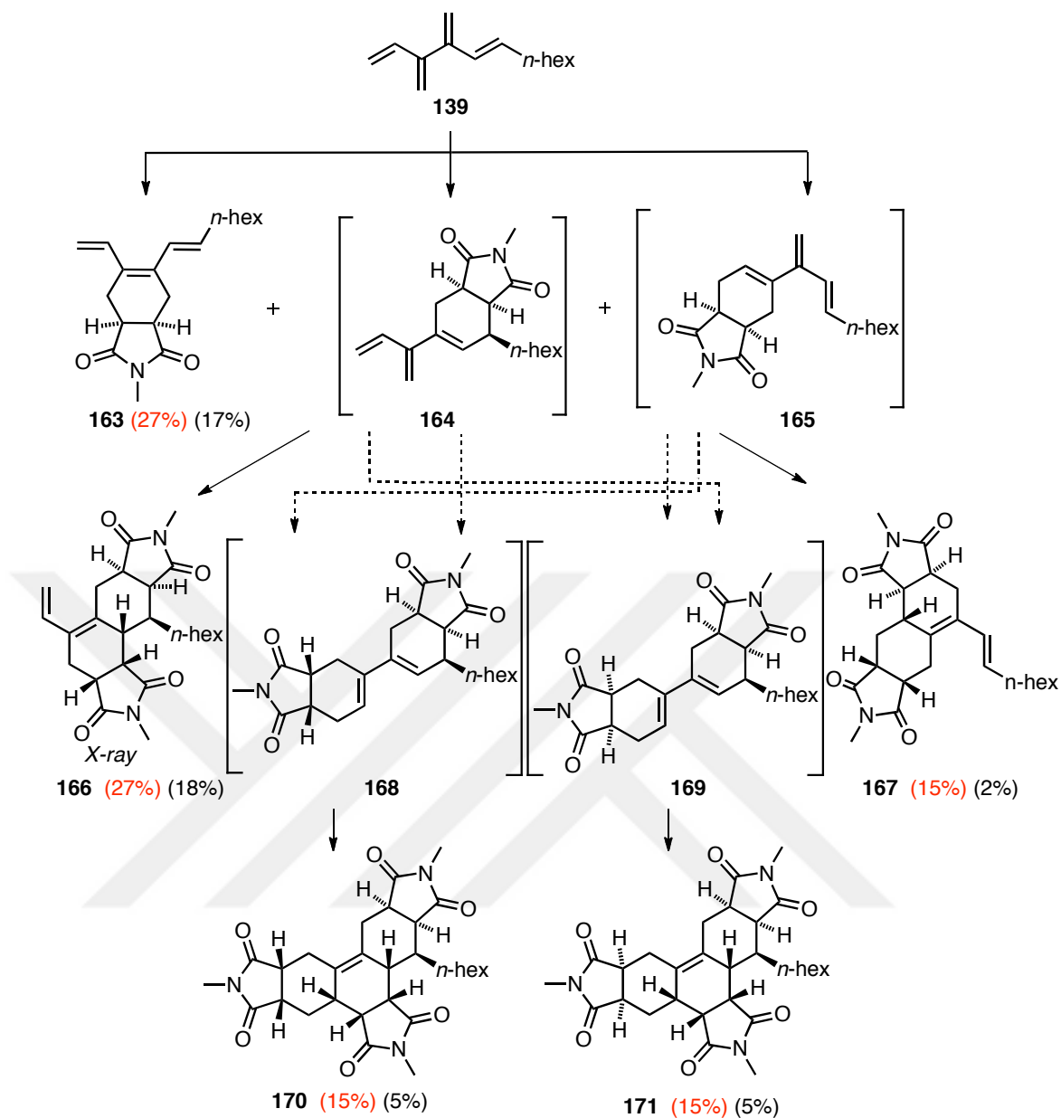
Scheme 1.61: The Diels-Alder reaction between 1-(E)-hexyl [4]dendralene 139 and an excess of NMM 49 . Reagents and conditions: (a) NMM (3 mol equiv), \text{CDCl}_3 , rt, 1 day. Crude product ratios in red text, isolated yields in black text.
