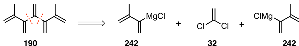
Scheme 2.25: Retrosynthetic analysis of dimethyl substituted [5]dendralene 190 .
