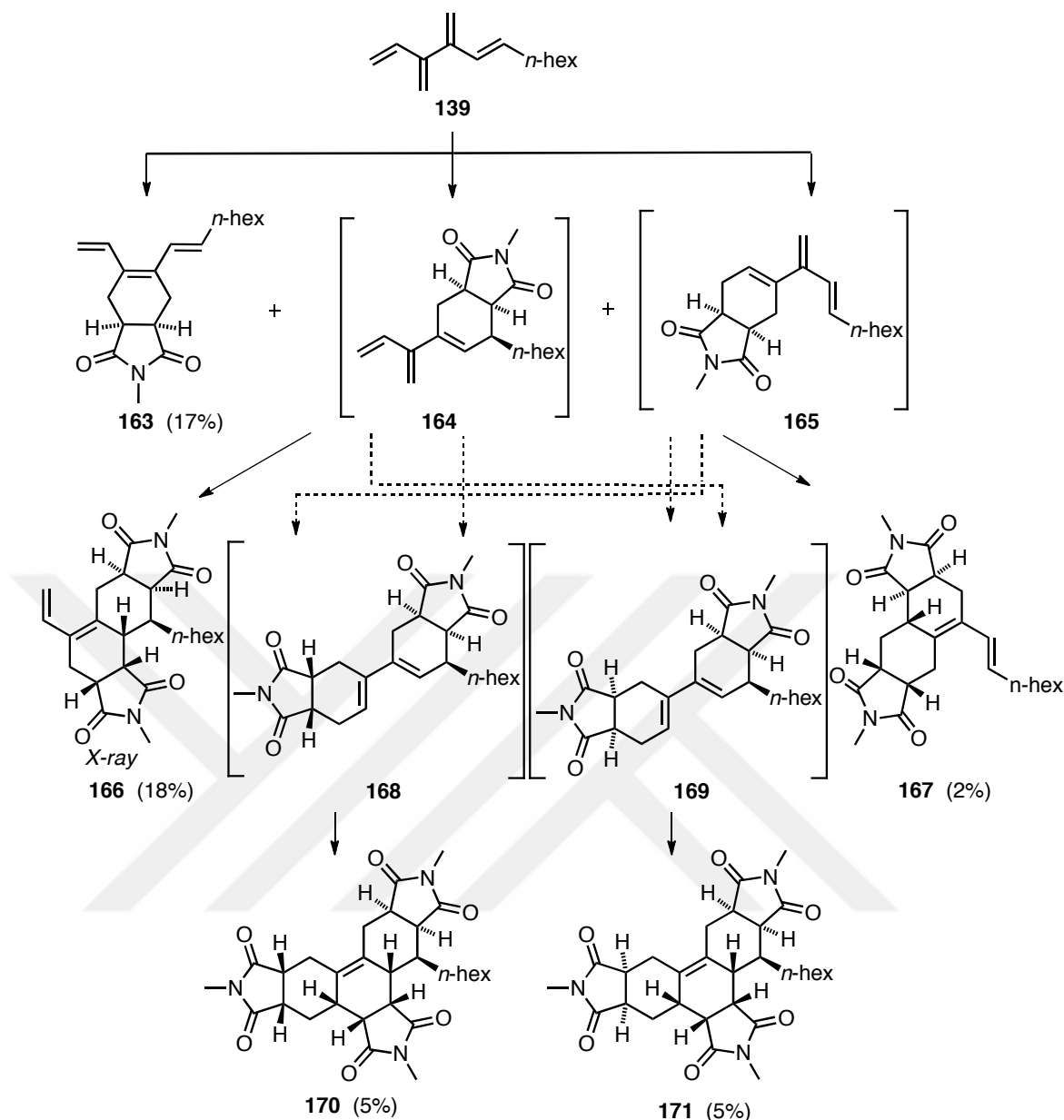
Scheme 1.68: The Diels-Alder reaction between 1-( E )-hexyl [4]dendralene 139 and an excess of NMM 49 . Reagents and conditions: (a) NMM (3 mol equiv), CDCl 3 , rt, 1 day. Isolated yields shown.
