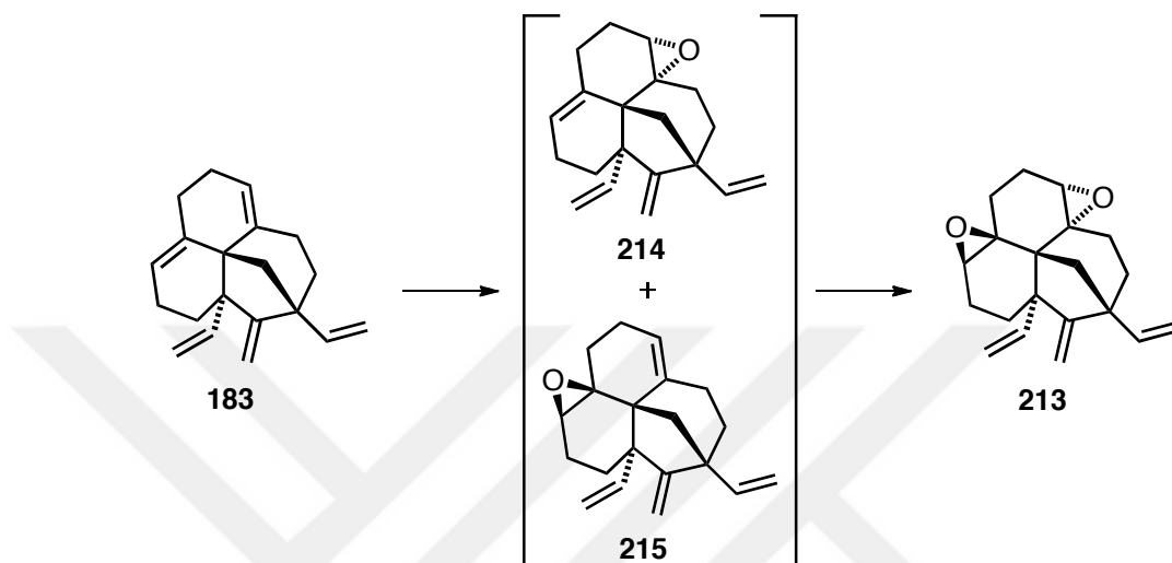
Scheme 2.16: Proposed structures of mono -epoxides 214 and 215 .
