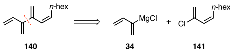
Scheme 1.48: Retrosynthetic analysis of 1-( Z )-hexyl [4]dendralene 140 .
