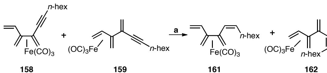
Scheme 1.58: Reduction of iron tricarbonyl protected mixture ( 158:159 , 2:1 ratio). Reagents and conditions: (a) \text{H}_2 , Lindlar catalyst, pentane, in the dark, rt, 6 h, 65% (impure).
