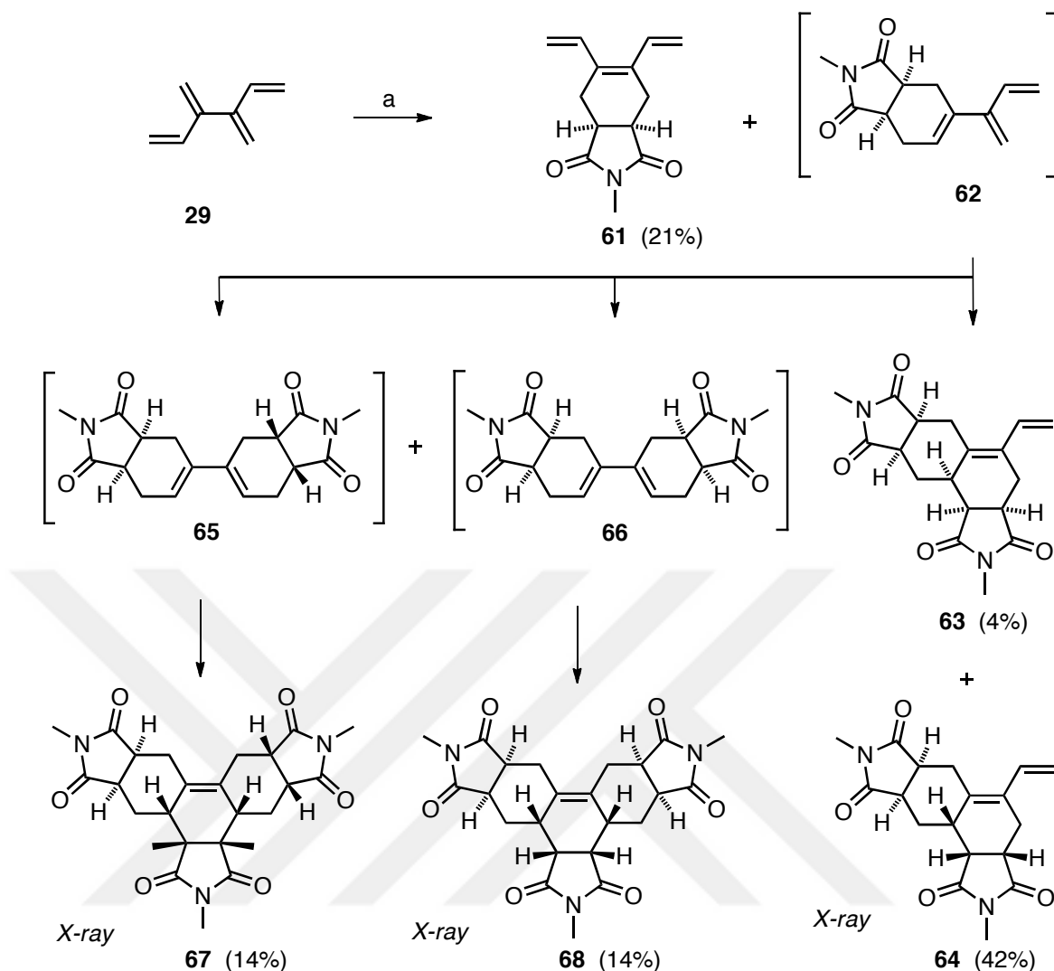
Scheme 1.17: Reactions between [4]dendralene 29 and NMM 49 under kinetically controlled conditions at room temperature. Reagents and conditions: (a) NMM (2.5 mol equiv), rt, 16 h, 95%.
