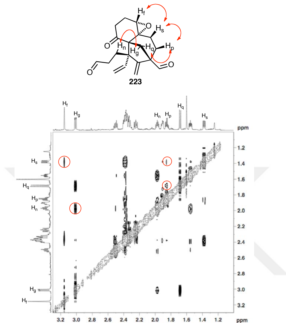
Figure 2.10: NOESY spectrum of the compound 223 . nOe cross-peaks highlighted in red are associated with the spatial correlations indicated by red arrows.
