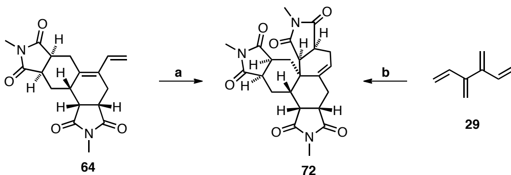
Scheme 1.20: The efficient preparation of tris -adduct 72 . Reagents and conditions: (a) NMM (3.6 mol equiv), \text{CH}_2\text{Cl}_2 , 19 kbar, 70 °C, 2 h, then rt, 4 days, 84%; (b) NMM (9.5 mol equiv), \text{CH}_2\text{Cl}_2 , 19 kbar, 70 °C, 2 h, then rt, 4 days, 34%.
