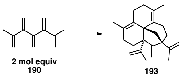
Scheme 2.38: Formation of tetracycle 193 from dimethyl substituted [5]dendralene 190 .
