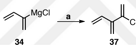
Scheme 1.33: Improved synthesis of 2-chloro [3]dendralene 37 . Reagents and conditions: (a) 1,1-dichloroethylene (7.6 mol equiv), Ni(dppe)Cl_2 (0.013 mol equiv), -20\text{ }^{\circ}C , 13 h, 85%.
