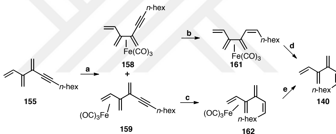
Scheme 1.59: Summary of the hydrogenation approach to 1-(Z)-hexyl [4]dendralene 140 via iron tricarbonyl protected substrates. Reagents and conditions: (a) \text{Fe}_2(\text{CO})_9 (1.8 mol equiv), aza catalyst (0.35 mol equiv), 1,2-dimethoxyethane, THF, in the dark, 60 °C, 40 h, 158:159 , 30% and 13%, respectively; (b) \text{H}_2 , Lindlar catalyst, pentane, in the dark, rt, 6 h, 82% (impure); (c) \text{H}_2 , Lindlar catalyst, pyridine, pentane, in the dark, rt, 14 h, 45% (impure); (d) CAN (2 mol equiv), acetone, methanol, 0 °C, 5 min (impure); (e) CAN (2 mol equiv), acetone, methanol, 0 °C, 1 h, then more CAN (2 mol equiv), 0 °C, 15 min (impure).
