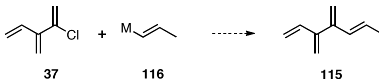
Scheme 1.32: Preparation of 1-(E)-methyl [4]dendralene 115 from 2-chloro [3]dendralene 37 using transition metal catalysis ( M = B(OR)_2 or MgBr ).
