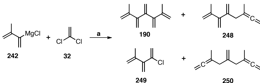
Scheme 2.30: Towards the synthesis of dimethyl substituted [5]dendralene 190 . Reagents and conditions: (a) (3-Methylbuta-1,3-dien-2-yl)magnesium chloride (3.0 mol equiv), 1,1-dichloroethylene (1.0 mol equiv), \text{PPh}_3 (0.050 mol equiv), \text{Ni(dppp)Cl}_2 (0.025 mol equiv), 15 °C to rt, 45 h.
