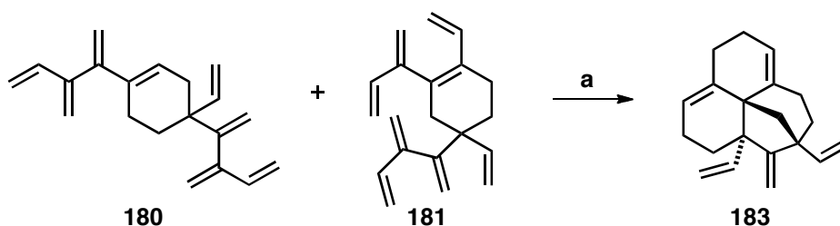
Scheme 2.5: Synthesis of tetracycle 183 from a mixture of Diels-Alder dimers of [5]dendralene 176 . Reagents and conditions: (a) A ca. 60:40 mixture of 180 and 181 , PhCl, BHT, reflux, 24 h, 7% or mesitylene, reflux, 4.5 h, 10%.
