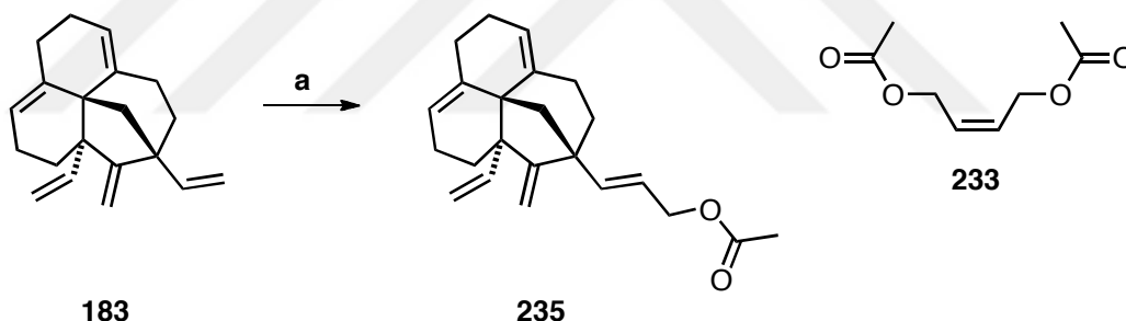
Scheme 2.23: Cross-metathesis reaction of tetracycle 183 . Reagents and conditions: (a) ( Z )-but-2-ene-1,4-diyl diacetate (4 mol equiv), Grubbs II catalyst (0.2 mol equiv), CH 2 Cl 2 , 60 °C, sealed tube, 24 h, 13% (34% based on recovered starting material).
