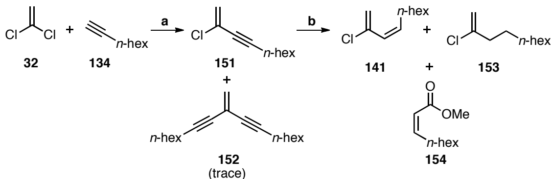
Scheme 1.52: An attempt to prepare 141 . Reagents and conditions: (a) 1,1-dichloroethylene (1.5 mol equiv), Pd(PPh 3 ) 4 (0.030 mol equiv), toluene, seal tube, rt, 25 min, then 1-octyne (1 mol equiv), n -BuNH 2 (1.5 mol equiv), CuI (0.030 mol equiv), 40 °C, 8 h, 63%; (b) H 2 , 5%Pd on BaSO 4 , quinoline, methanol, rt, 72 h, 14% (ratio 141 : 153 , 19:1) and 11% 154 .
