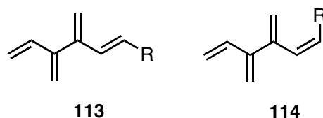
Figure 1.14: 1-( E )- and ( Z )-alkyl substituted [4]dendralenes 113 and 114 .
