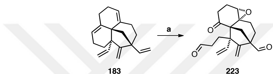
Scheme 2.18: Ozonolysis reaction of tetracycle 183 . Reagents and conditions: (a) \text{O}_3 (excess), \text{CH}_2\text{Cl}_2 , 15 min, -78\text{ }^{\circ}\text{C} , then \text{PPh}_3 (6 mol equiv), -78\text{ }^{\circ}\text{C} to 0\text{ }^{\circ}\text{C} , 30 min, 8%.
