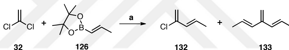
Scheme 1.43: Towards the preparation of 1-( E )-methyl-3-chloro-butadiene 132 . Reagents and conditions: (a) 1,1-dichloroethylene (1.2 mol equiv), Pd(PPh 3 ) 4 (0.020 mol equiv), Ag 2 CO 3 (2.0 mol equiv), THF, various temperature, 6 h, only starting material; (b) 1,1-dichloroethylene (1.0 mol equiv), Pd(dppf)Cl 2 (0.050 mol equiv), NaOH (2.0 mol equiv), sealed tube, THF, various temperatures, 8 h.
