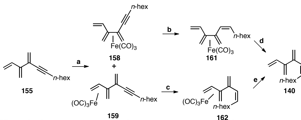
Scheme 1.67: Summary of the hydrogenation approach to 1-(Z)-hexyl [4]dendralene 140 via iron tricarbonyl protected substrates. Reagents and conditions: (a) \text{Fe}_2(\text{CO})_9 (1.8 mol equiv), aza catalyst (0.35 mol equiv), 1,2-dimethoxyethane, THF, in the dark, 60 °C, 40 h, 158:159 , 30% and 13%, respectively; (b) \text{H}_2 , Lindlar catalyst, pentane, in the dark, rt, 6 h, 82% (impure); (c) \text{H}_2 , Lindlar catalyst, pyridine, pentane, in the dark, rt, 14 h, 45% (impure); (d) CAN (2 mol equiv), acetone, methanol, 0 °C, 5 min (impure); (e) CAN (2 mol equiv), acetone, methanol, 0 °C, 1 h, then more CAN (2 mol equiv), 0 °C, 15 min (impure).
