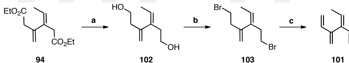
Scheme 1.29: Preparation of 4-( Z )-methyl [4]dendralene 101 . Reagents and conditions: (a) \text{LiAlH}_4 (2.0 mol equiv), \text{Et}_2\text{O} , 0 °C, 30 min, then rt, overnight, 91%; (b) NBS (2.0 mol equiv), \text{PPh}_3 (2.0 mol equiv), \text{CH}_2\text{Cl}_2 , -78 °C to rt, overnight, 84%; (c) DBU (6.4 mol equiv), DMSO, rt, 50 mmHg, 15 min, then 15 mmHg, 2 h, 77%.
