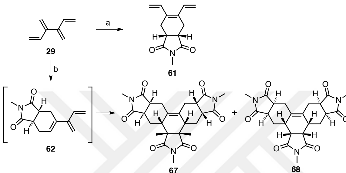
Scheme 1.21: Controlling the cycloaddition site selectivity with Lewis acid catalysts. Reagents and conditions: (a) NMM. \text{MeAlCl}_2 complex (2 mol equiv), toluene, -78^\circ\text{C} , 30 min to rt, 20 min, 77%; (b) NMM. 2\text{MeAlCl}_2 complex (3 mol equiv), \text{CH}_2\text{Cl}_2 , -78^\circ\text{C} , 2 h then rt, 20 min, ( 67 : 68 , 37% and 34% respectively).
