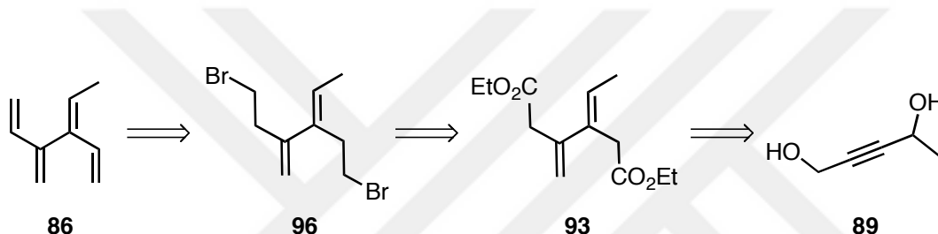
Scheme 1.25: Retrosynthesis of 4-( E )-methyl [4]dendralene 86 .
