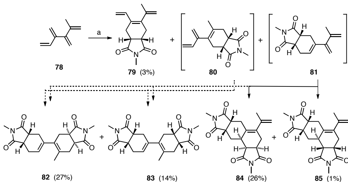
Scheme 1.23: Diels-Alder reaction of 2-methyl [4]dendralene 78 with NMM 49 . Reagents and conditions: (a) NMM (3 mol equiv), CH 2 Cl 2 , rt, 14 h, 71%.
