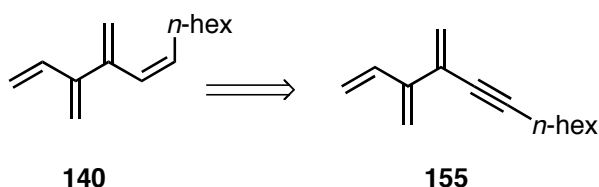
Scheme 1.62: Retrosynthetic analysis of 1-( Z )-hexyl [4]dendralene 140 .
