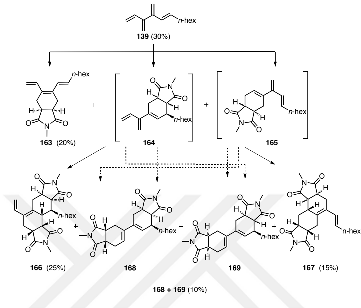
Scheme 1.60: The Diels-Alder reaction between 1-( E )-hexyl [4]dendralene 139 and one molar equivalent of NMM 49 . Reagents and conditions: (a) NMM (1 mol equiv), CDCl 3 , rt, 117 hours. Yields estimated from the crude 1 H NMR spectrum.
