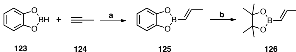
Scheme 1.37: Synthesis of pinacol boronate ester 126 . Reagents and conditions: (a) Propyne (ca. 1.3 mol equiv), -78\text{ }^{\circ}\text{C} to 70\text{ }^{\circ}\text{C} , THF, 12 h, 58%; (b) Pinacol (1.0 mol equiv), \text{Et}_2\text{O} , rt, 3 h, 63%.
