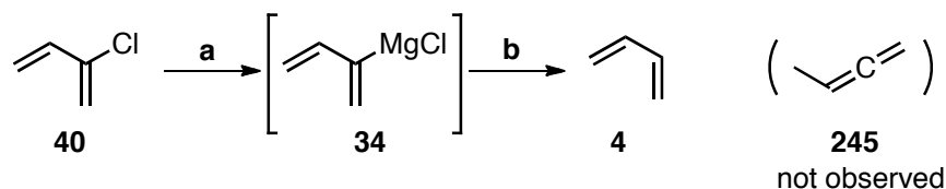
Scheme 2.28: The formation of Grignard 34 reagent and its protonolysis product. Reagents and conditions: (a) Magnesium turnings (1.6 mol equiv), \text{BrC}_2\text{H}_4\text{Br} (0.30 mol equiv), \text{ZnBr}_2 (0.010 mol equiv), THF, reflux, 2 h, 76%. (b) Quenched with water and diluted with \text{CDCl}_3 . Also see. 103
