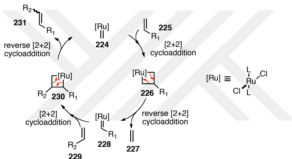
Scheme 2.22: Mechanism of a ruthenium-catalysed alkene cross-metathesis reaction. 99
