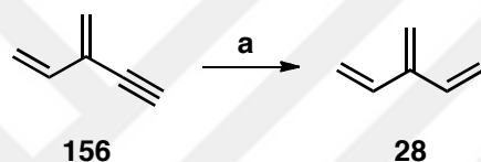
Scheme 1.54: Hopf's synthesis of [3]dendralene 28 . Reagents and conditions: (a) \text{H}_2 , Lindlar catalyst, 60%.
