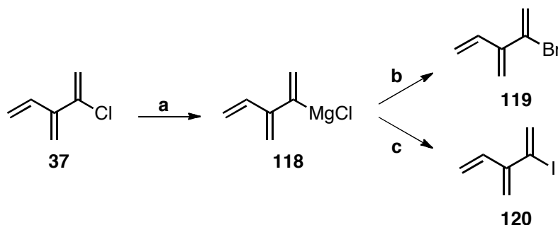
Scheme 1.34: Preparation of 2-bromo [3]dendralene 119 and 2-iodo [3]dendralene 120 . Reagents and conditions: (a) Magnesium powder (2.9 mol equiv), \text{BrC}_2\text{H}_4\text{Br} (0.70 mol equiv), \text{ZnBr}_2 (0.030 mol equiv), THF, reflux, 30 min, 36%; (b) NBS (3.0 mol equiv), THF, -78^\circ\text{C} to rt, 2.5 h, 13%; (c) \text{I}_2 (3.0 mol equiv), \text{Et}_2\text{O} , -78^\circ\text{C} to rt, 2.5 h, 30%.
