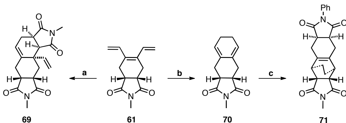
Scheme 1.19: Further transformation of internal mono -adduct product 61 . Reagents and conditions: (a) NMM (2 mol equiv), \text{CH}_2\text{Cl}_2 , rt, 19 kbar, overnight, 69%; (b) toluene, BHT, reflux, 18 h, 72%; (c) NPM (3 mol equiv), BHT, reflux, toluene, 18 h, 70% (yield from 61 , in two steps).
