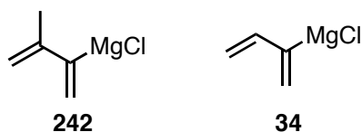
Figure 2.17: Grignard reagents 242 and 34 for the formation of dimethyl substituted [5]dendralene 190 and [5]dendralene 176 , respectively.
