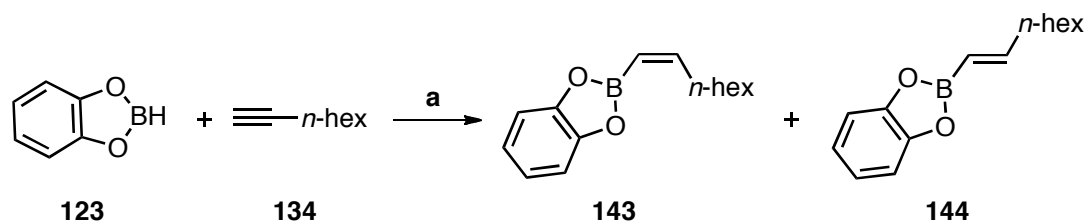
Scheme 1.50: An rhodium catalysed attempt to prepare (Z)-catechol boronate 143 . Reagents and conditions: (a) [\text{Rh}(\text{cod})\text{Cl}]_2 (0.015 mol equiv), \text{PCy}_3 (0.060 mol equiv), \text{Et}_3\text{N} (1.0 mol equiv), rt, 30 min, then 1-octyne (1.2 mol equiv), rt, 2 h, 10% yield, ( 143 : 144 , 1:2 ratio).
