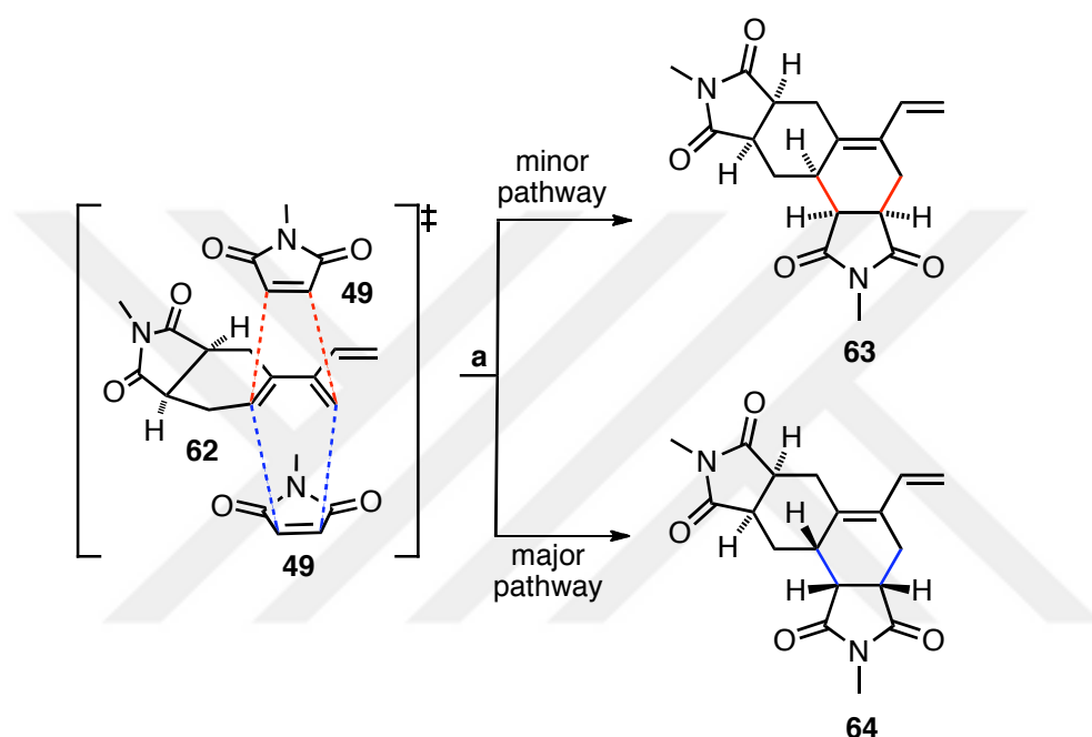
Scheme 1.18: Two possible addition of NMM 49 to mono -adduct 62 and bis -adducts 63 and 64 . Reagents and conditions: (a) NMM (2.5 mol equiv), 16 h, rt ( 4:5 ratio, 4%, 42% respectively).
