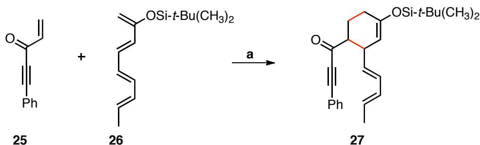
Scheme 1.7: Site selectivity in the intermolecular Diels-Alder reaction between a dienophile 25 and a multiple diene 26 . Reagents and conditions: (a) CCl 4 , reflux, 55%.
