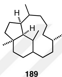
Figure 2.4: Trinervitane carbon skeleton 189 .
