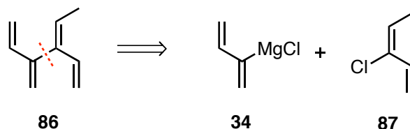
Scheme 1.24: Retrosynthesis of 4-( E )-methyl [4]dendralene 86 .
