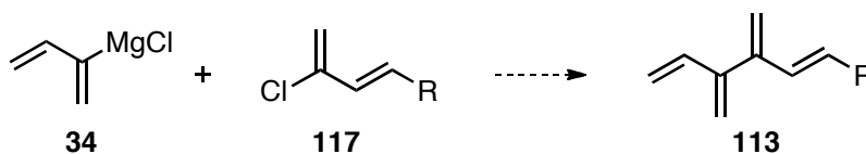
Scheme 1.42: Preparation of 1-( E )-alkyl substituted [4]dendralene 113 from Grignard reagent 34 and coupling partner 117 . (R=Me, n -hex).
