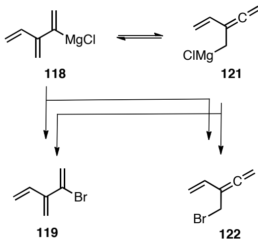
Scheme 1.35: Possible relationships between 118 and 121 . Reagents and conditions: (a) NBS (3 mol equiv), THF, -78^\circ\text{C} , 1.5 h then to rt, 1 h, 28%, (ratio of 119 : 122 , 45:55, isolated ratio).
