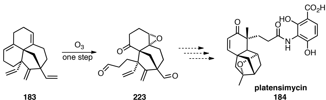
Scheme 2.37: From tetracycle 183 to platensimycin 184 .
