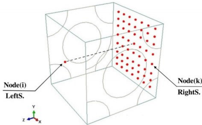
Figure 4.6: Schematic of a matching pair of nodes on opposite faces of an RVE [82]
