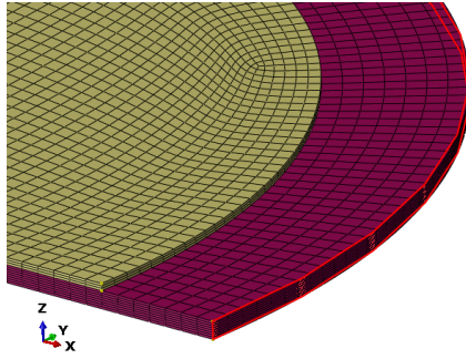
(a) Heterogeneous Macro-Scale Model
