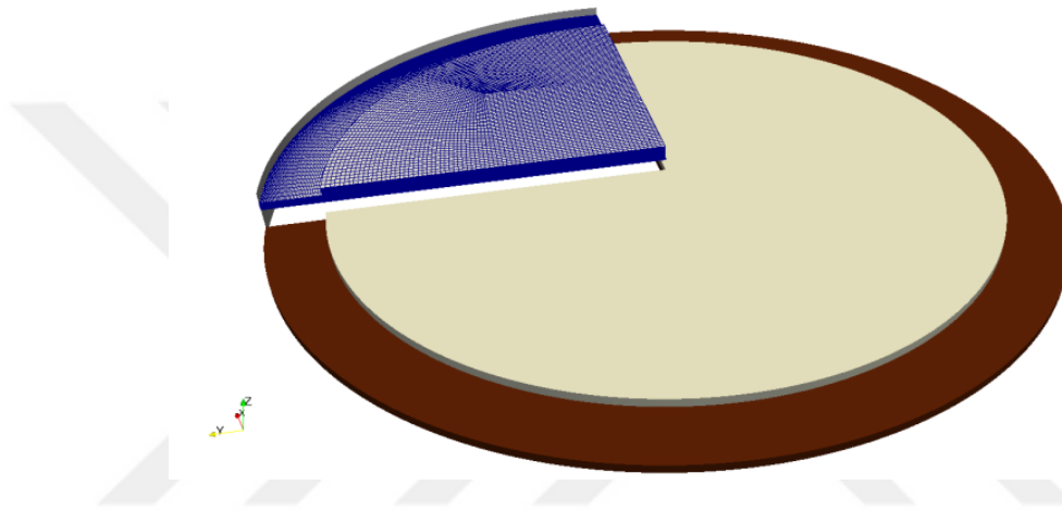
Figure 5.17: Full scale of macroscale model and its quarter computational domain [97]
