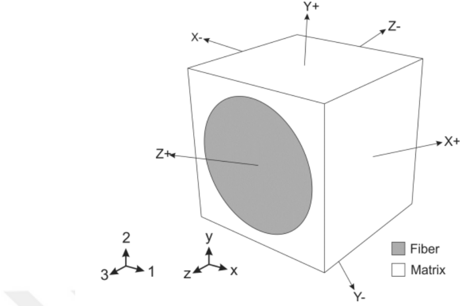
Figure 4.7: Part and Surface Designations in a Representative Volume Element [94]
