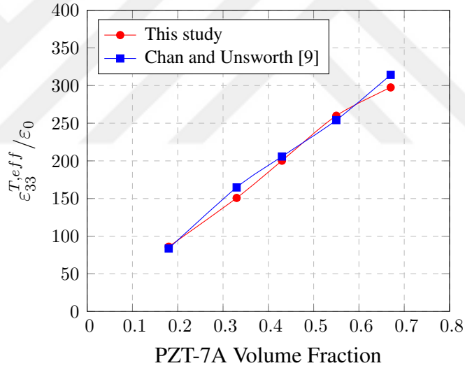
Figure 5.15: \epsilon_{33}^{T,eff} / \epsilon_0 vs. PZT-7A volume fraction ( d_{33} = 167 \times 10^{-12} \text{ m/V} for PZT-7A)
