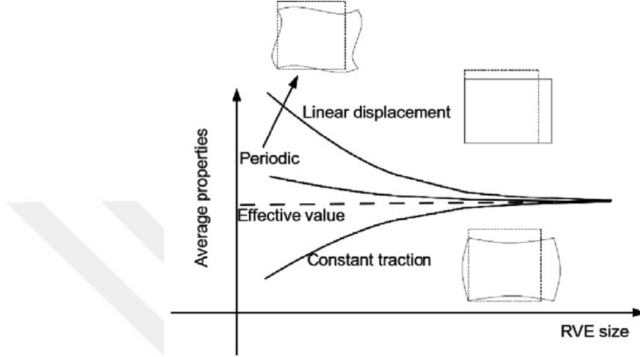
Figure 4.5: Convergence comparison of the boundary conditions in a RVE [88]
