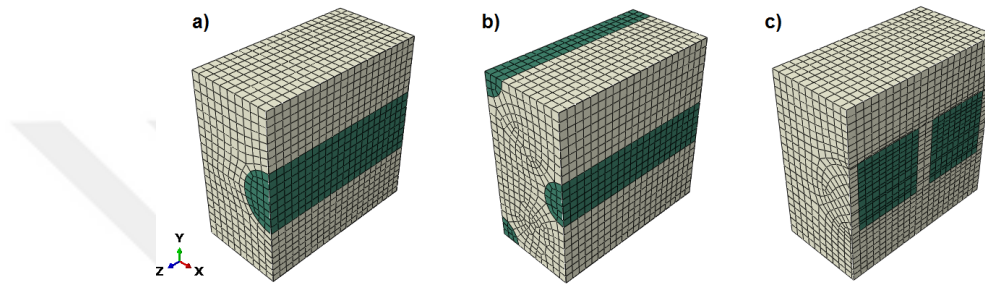
Figure 6.15: Cut-views of the RVEs that contain 10 % pore in the shape of a) a single cylinder, b) two cylinders, one at the center and the other divided into 1/4 located at the edges, and c) two cylinders aligned in the axis of isotropy
