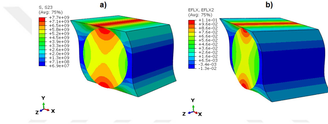
Figure 5.8: Under shear loading in Y - Z , a) stress distribution in Y - Z and b) electric displacement distribution in Y in the deformed shapes
