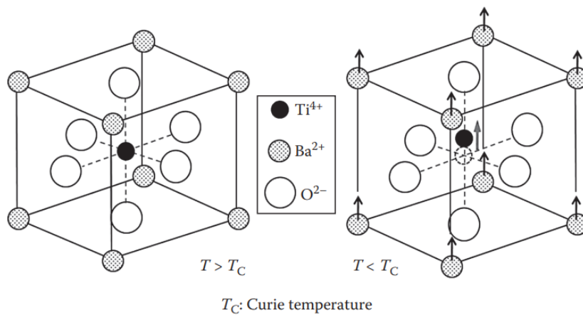
Figure 3.1: Crystal structure of Barium Titanate [37]
