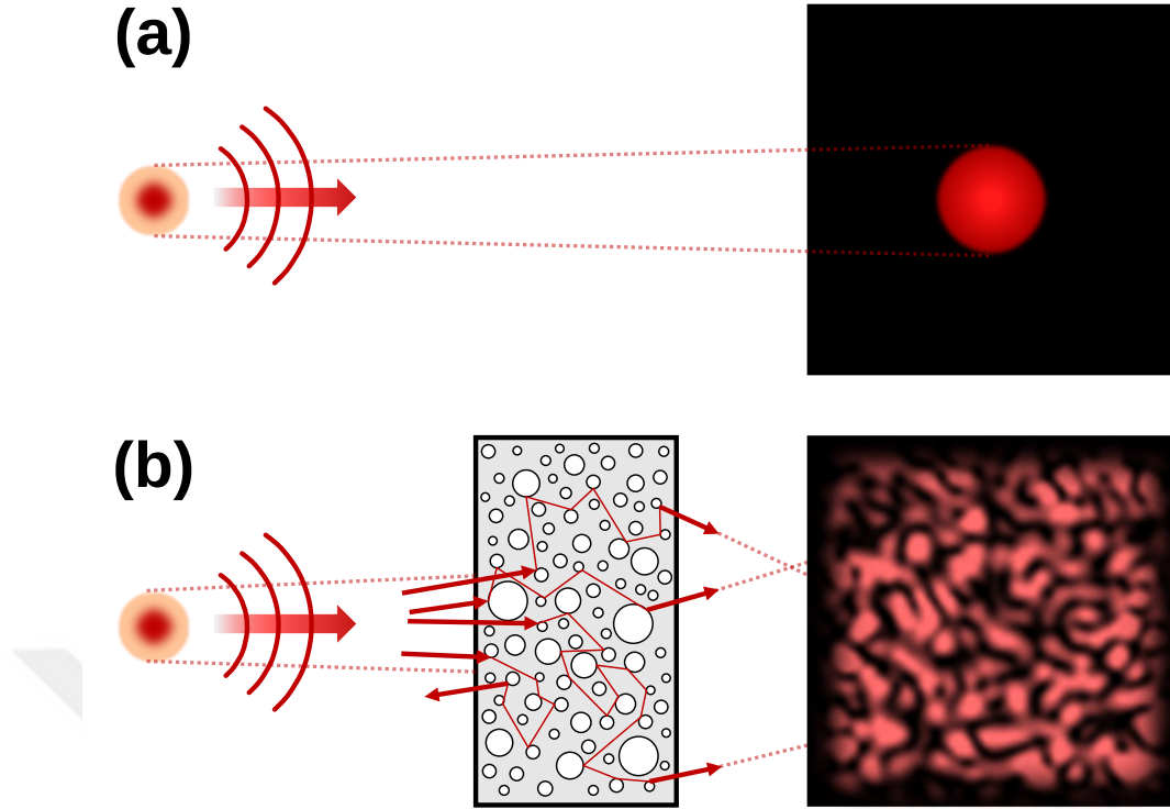
Figure 1.2: Interaction of light with matter. (a) A light source in free space travels undistorted and follows an almost straight line to form a sharp image of the light source. (b) The same light source creates a speckle pattern when it encounters a complex, disordered material due to the multiple scattering inside the medium.
