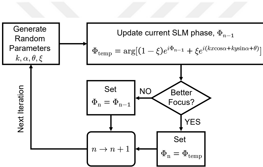
Figure 3.9: Flowchart of non-sequential algorithm. The SLM phase is updated in each iteration with random parameters. The SLM phase mask giving better focus on the desired target point is kept on the SLM after each iteration.
