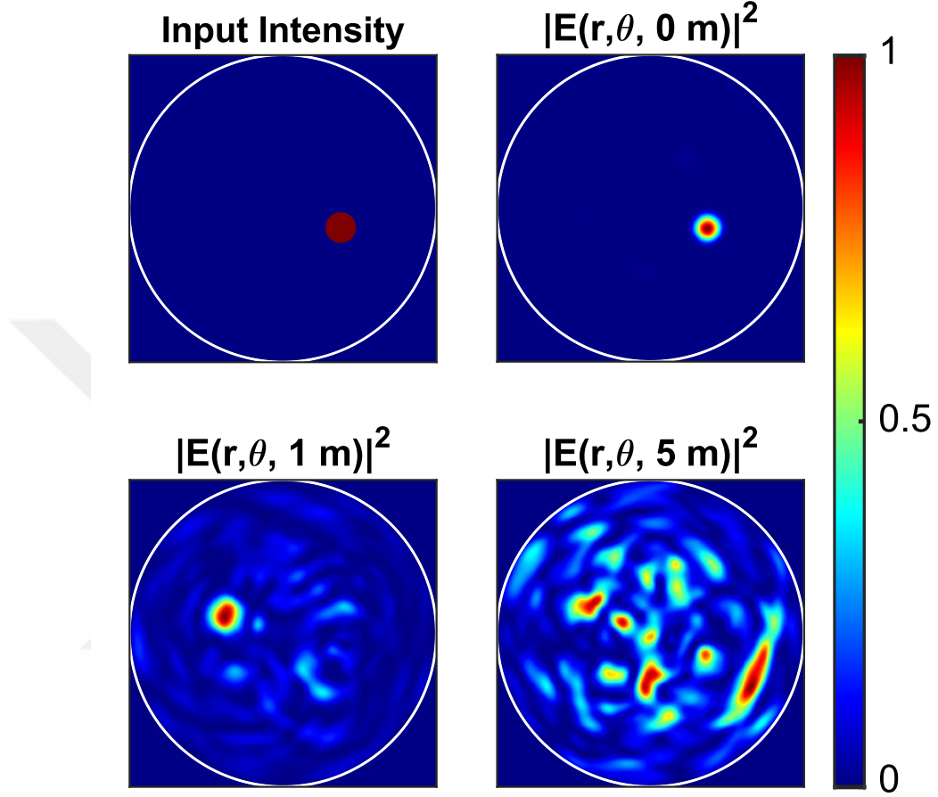
Figure 2.6: Propagation of a focused beam inside the fiber at various distances. The input field is first decomposed into the fiber modes by calculating the overlap integral between the two, and then it is propagated through the fiber by using the propagation constants of the decomposed modes. Thus, the input light is carried along the fiber with the propagation of its constituent modes. The wavelength of the incident light and the fiber parameters used in this simulation are the same as in the previous examples.
