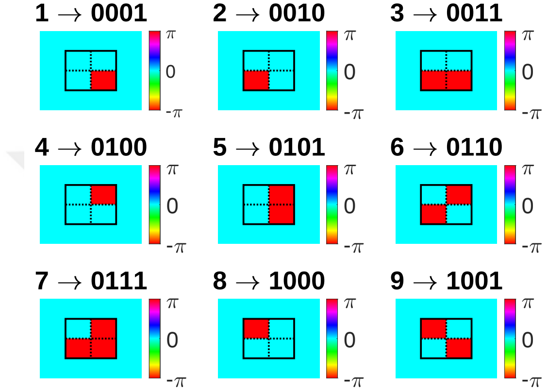
Figure 4.2: Phase distribution written on the SLM screen for encoding bit strings of length four corresponding to the numbers from 1 to 9. The binary number 0 (1) is encoded as 0 ( \pi ) phase shift. Encoding is applied to the most responsive regions of the SLM, which are determined by scanning varying-sized rectangles of phase 0 and \pi over the whole SLM screen. Four regions used to encode the digits in the bit string are separated by dashed lines.
