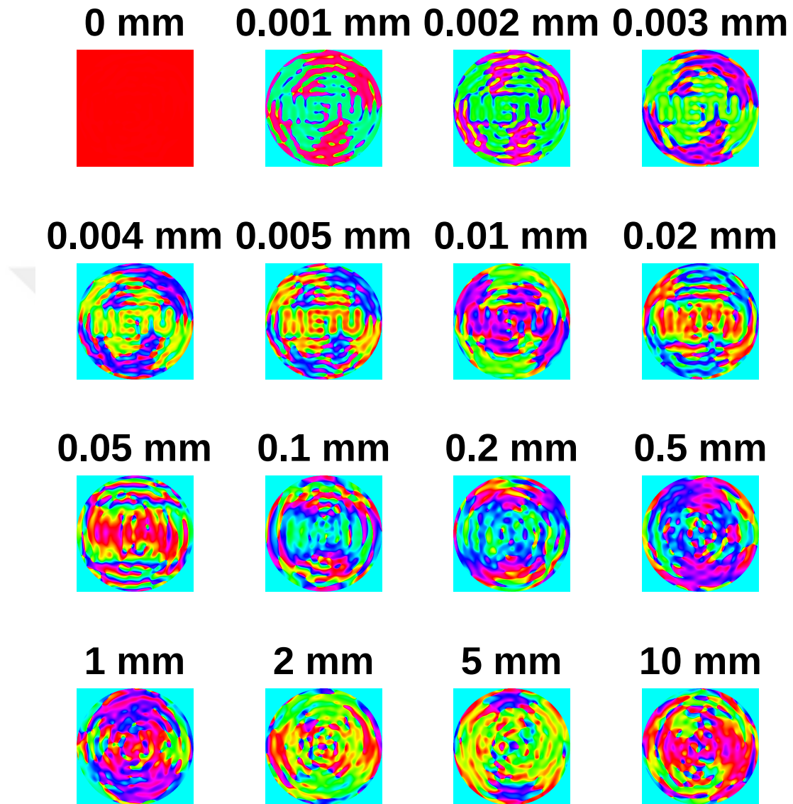
Figure 2.8: Phase variation of the text "METU" at different propagation distances along a multimode fiber.
