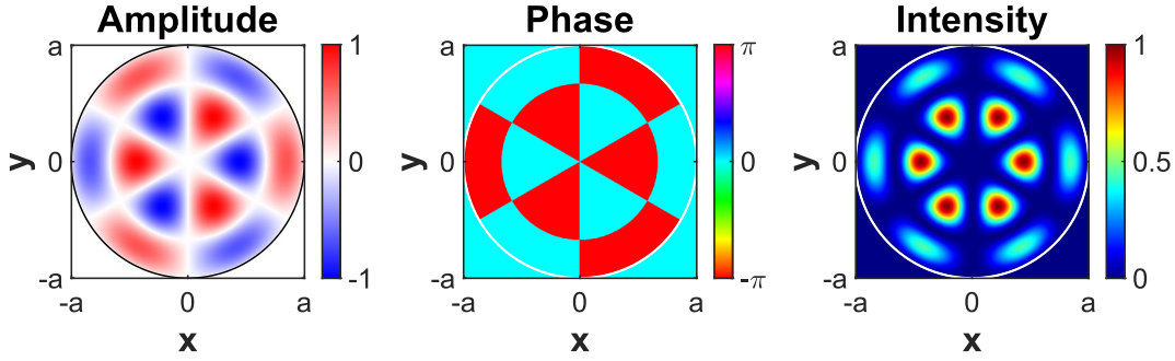
Figure 2.4: Normalized amplitude (real part), phase, and intensity profiles of LP_{32} ( m = 3 , p = 2 ) mode. The amplitude, E_{32} , is, in general, a complex number with both positive and negative values. Once the amplitude E_{32} and phase \phi_{32} of the mode is known, the intensity can be calculated as I = |E_{32}e^{i\phi_{32}}|^2 . The number of azimuthal and radial solutions represented in a mode can be verified from the intensity profile as there are 2m = 6 maxima along the azimuthal direction and p = 2 maxima along the radial direction.
