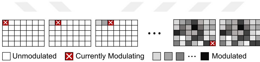
Figure 3.7: Principle of continuous sequential algorithm. Individual pixels (or groups of pixels) on the SLM are programmed sequentially to increase the focusing quality of the beam on the desired target region of the camera. The optimal phase value of each pixel is determined by calculating the PBR of the output image.
