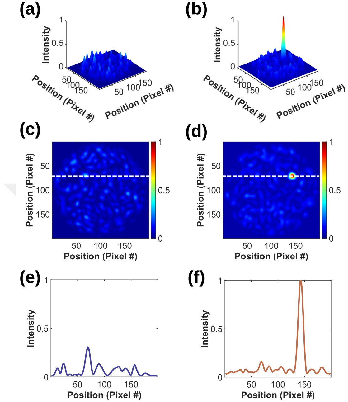
Figure 3.6: Comparison of speckle image before and after wavefront shaping. (a)-(b) 3D visualization of the speckles before and after optimization. (c)-(d) 2D visualization of the speckles before and after optimization. (e)-(f) Intensity variation along the white dashed line on the 2D speckles before and after optimization.
