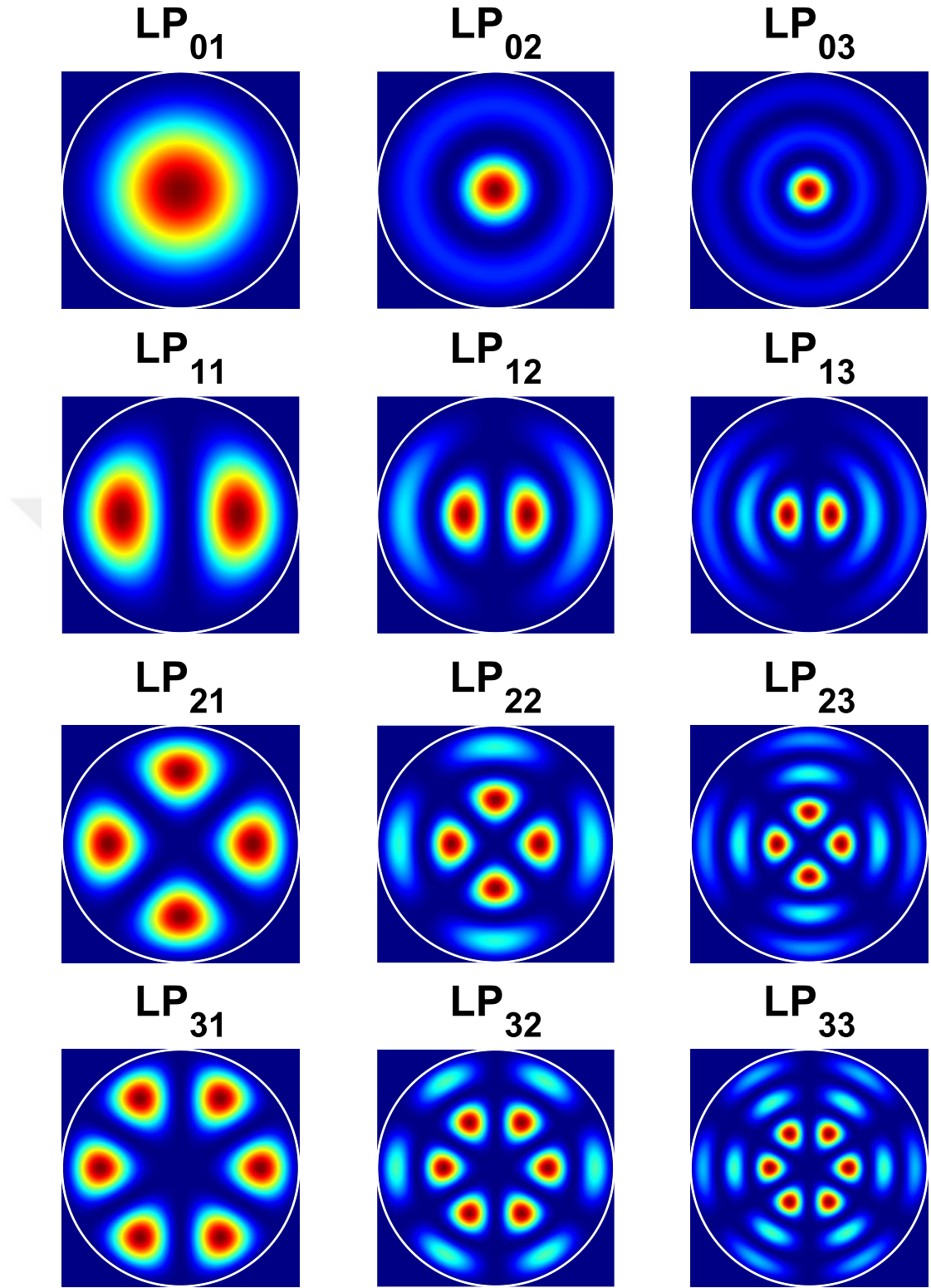
Figure 2.5: Examples of LP mode intensity profiles for a step-index multimode fiber with core diameter 105\ \mu\text{m} , \text{NA} = 0.22 ( n_{\text{core}} = 1.463 , n_{\text{cladding}} = 1.446 ) with an incident light of 1550\ \text{nm} wavelength.
