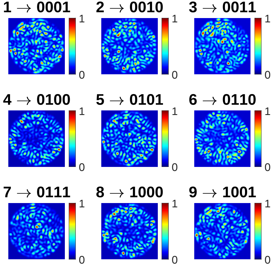
Figure 4.4: Speckle patterns obtained at the exit facet of the multimode fiber for bit strings of length four corresponding to numbers from 1 to 9. Most responsive regions of the SLM are modulated to guarantee distinct speckles. The similarity of the speckles is measured by calculating the correlation coefficients of speckles with each other.
