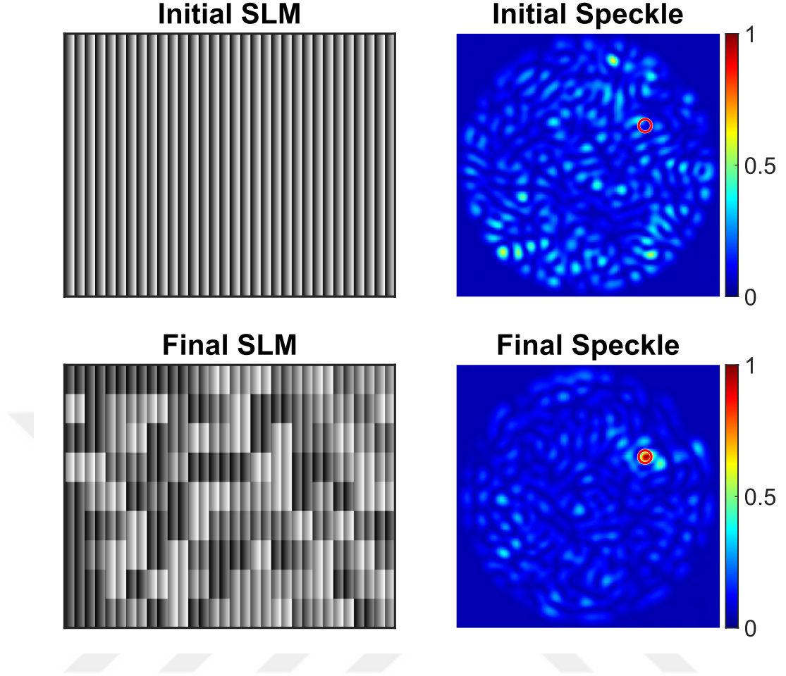
Figure 3.8: Initial and final SLM patterns (left) and corresponding speckles (right) obtained with the implementation of continuous sequential algorithm. All modulation is done on the blazed grating kept on the SLM. 144 macropixels are optimized in three iterations using four phase values between 0 - 3\pi/2 . A focus is obtained on the target location (shown with the red circle) after \sim 30 minutes. The PBR of the system is increased 6.6 times, from 78.3 to 517.3.
