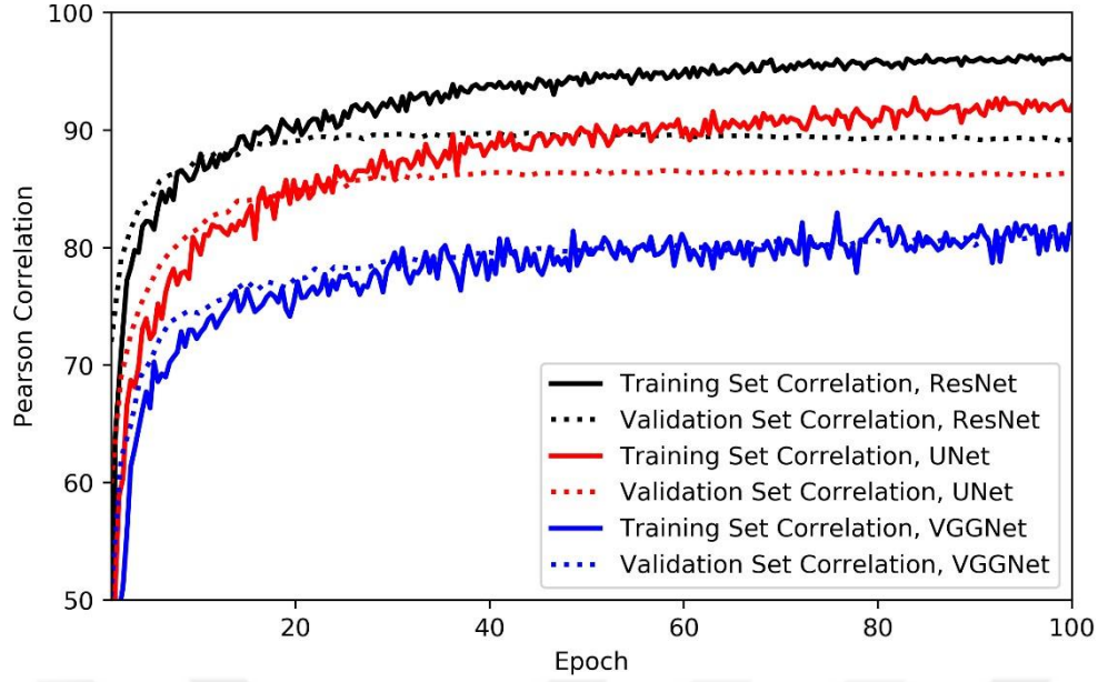
Figure 5.4: Average Pearson correlation coefficient (multiplied by 100) between pairs of predicted and ground truth images for the ResNet, UNet, and VGGNet-based networks after each epoch.
