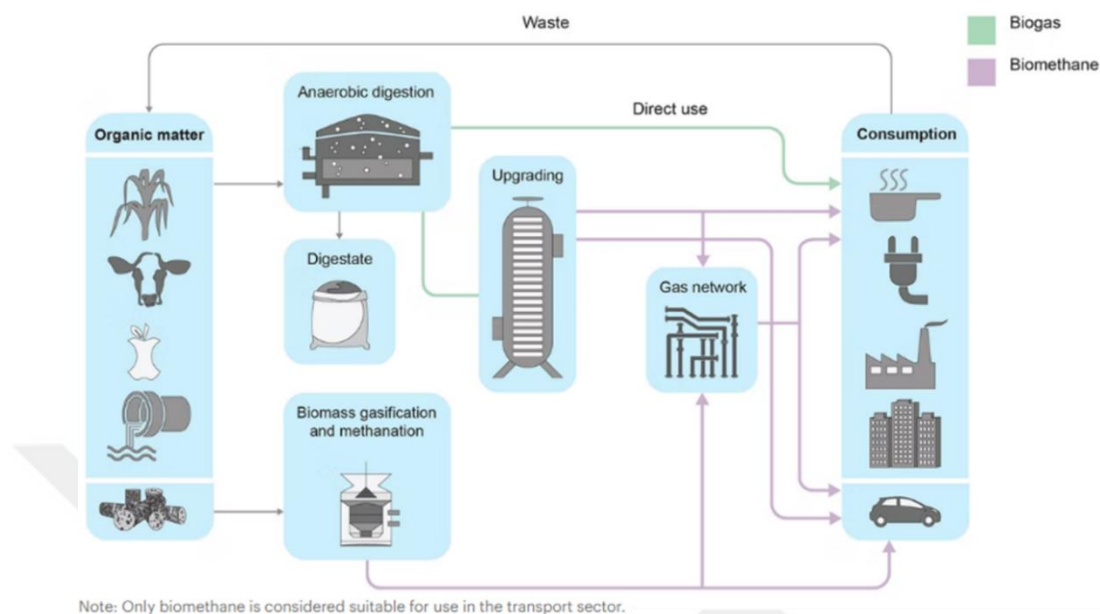
Figure 4.10: Biogas and Biomethane Chain
