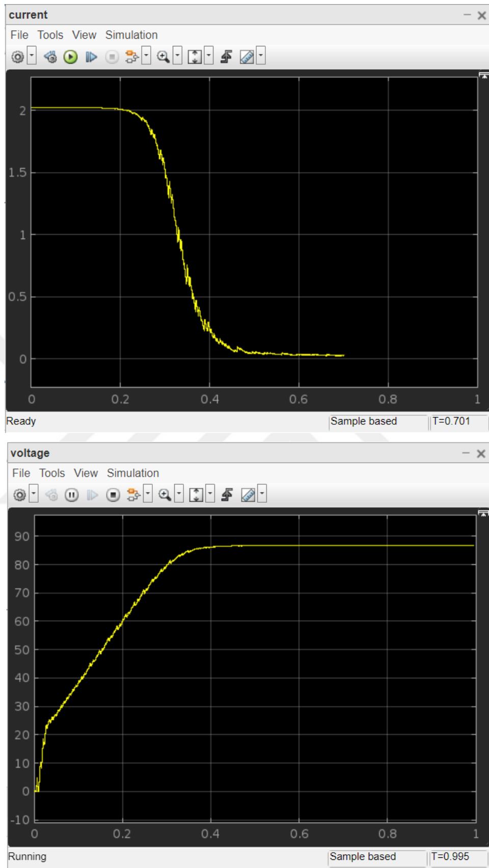
Figure 4.4. DC current and voltage of pv solar cell.
