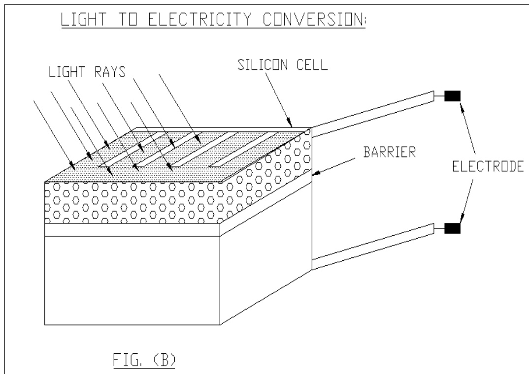
Figure 2.4. Converting the light to electricity [17].
