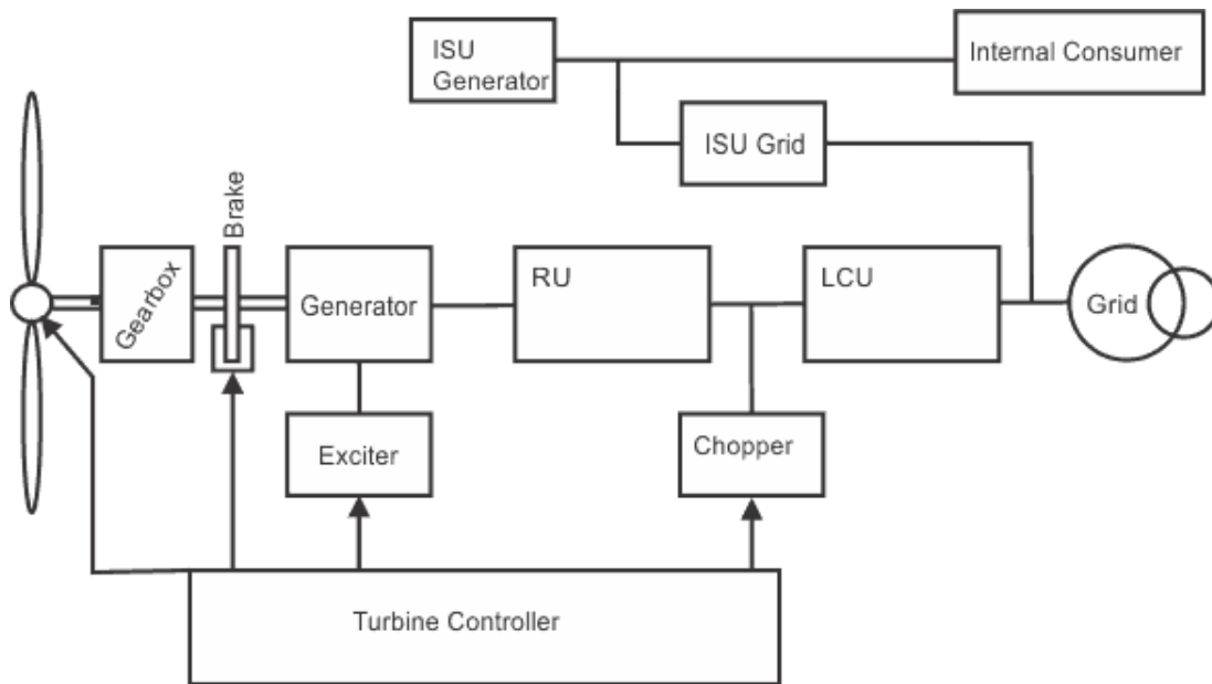
Figure 2.14. A Block plan of a wind turbine.
