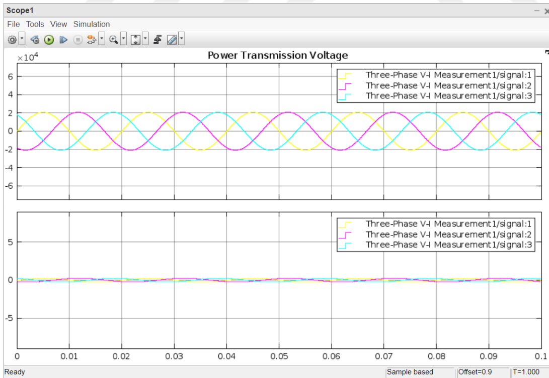
Figure 4.14. Power transmission voltage for scope 1.
