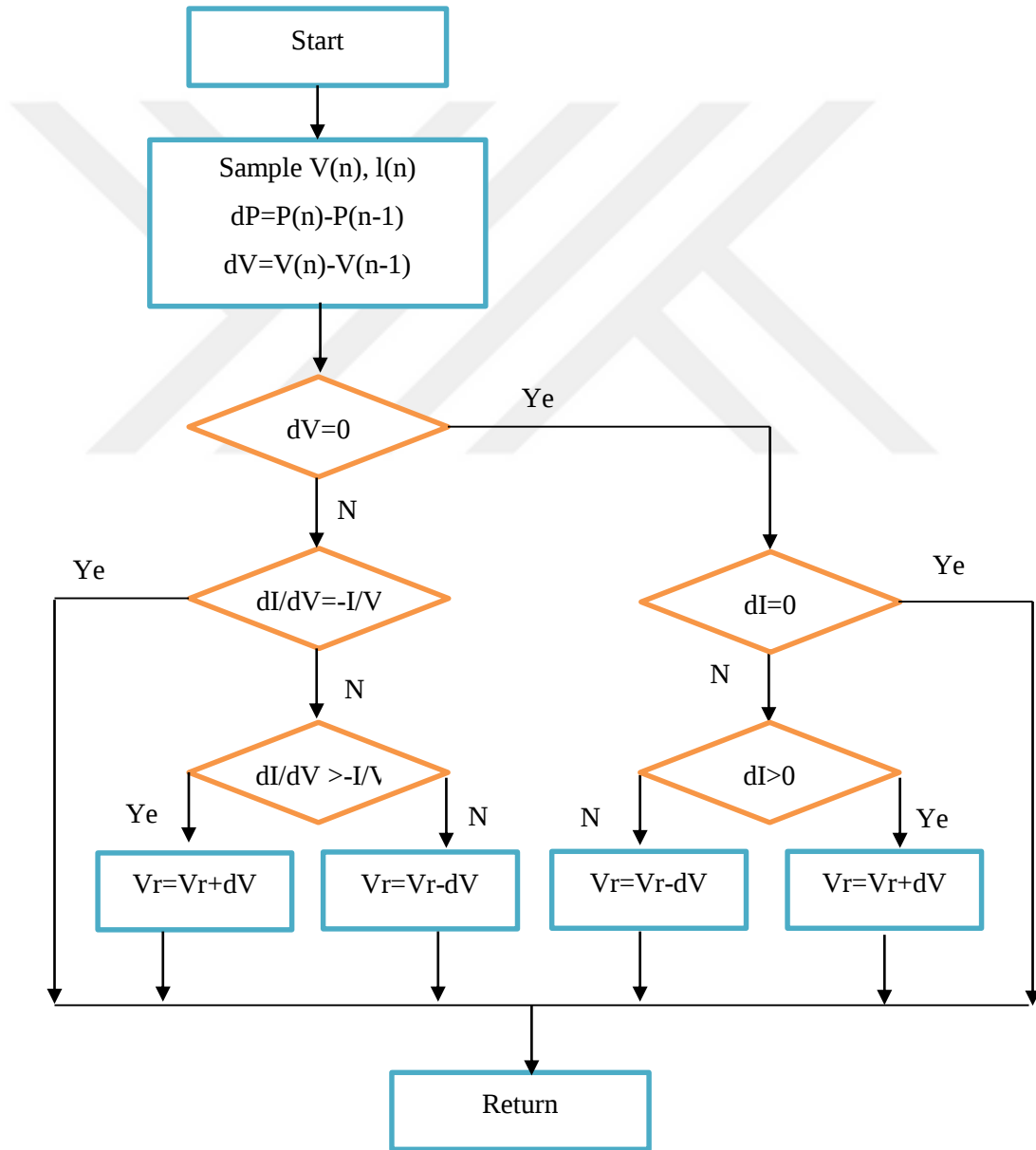
Figure 3.8. Flowchart for conductance technique [52].
