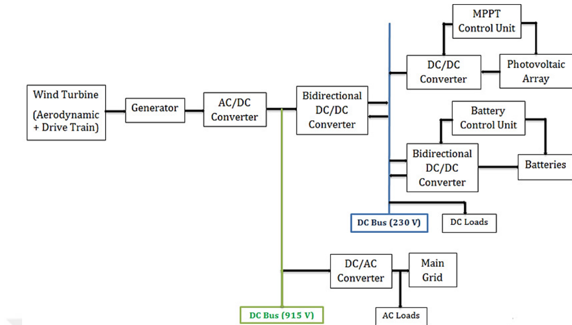
Figure 3.17. Hybrid power generator of wind solar system architecture.
