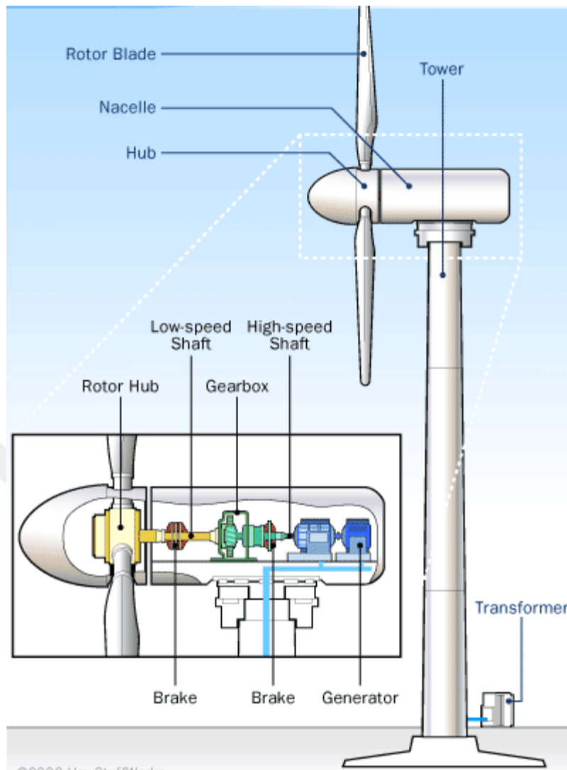
Figure 2.13. wind turbine.
