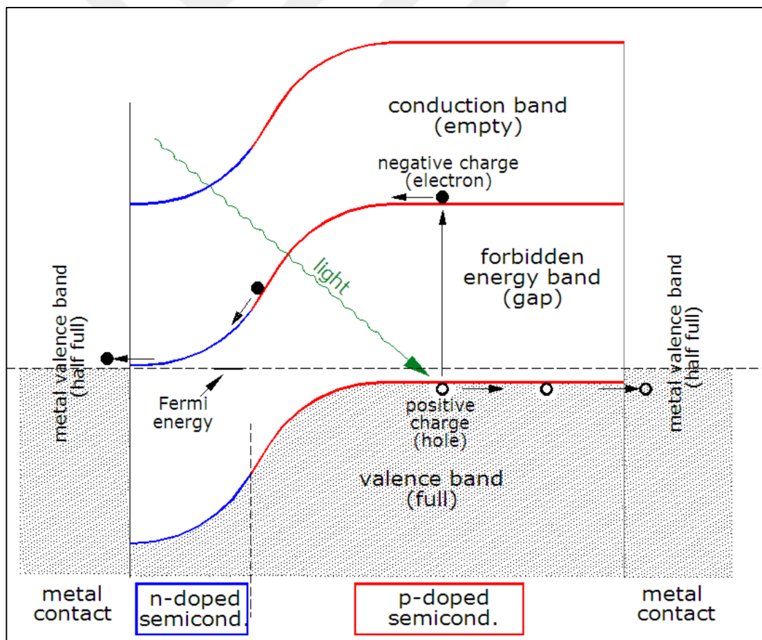
Figure 2.6. Graph of a Si solar cells, under illumination [20].
