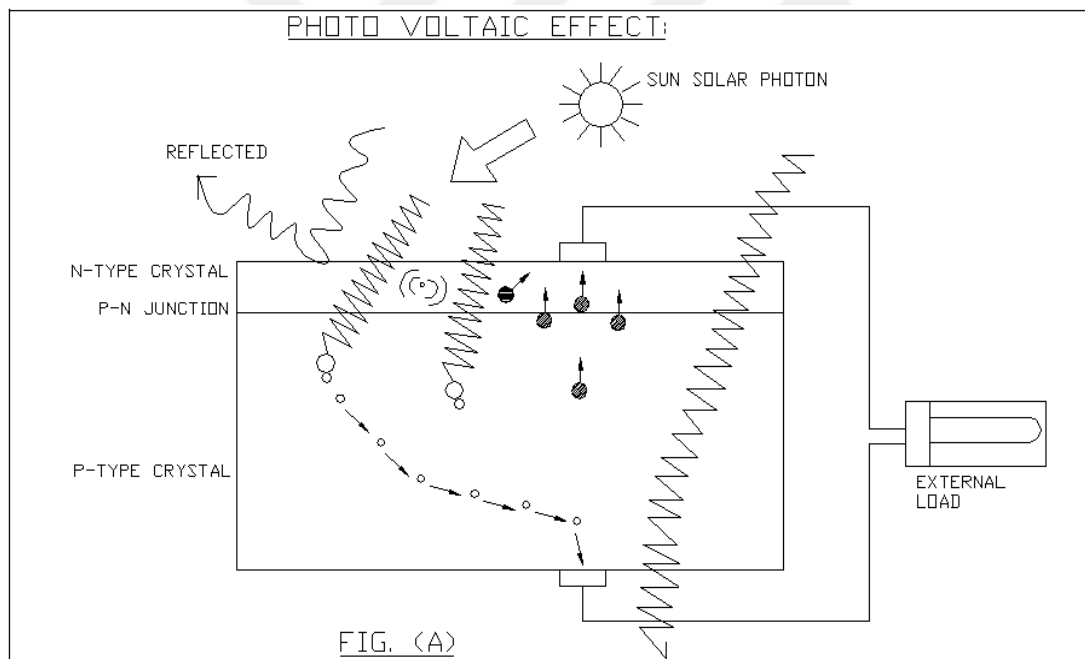
Figure 2.3. Voltaic effect process [16].
