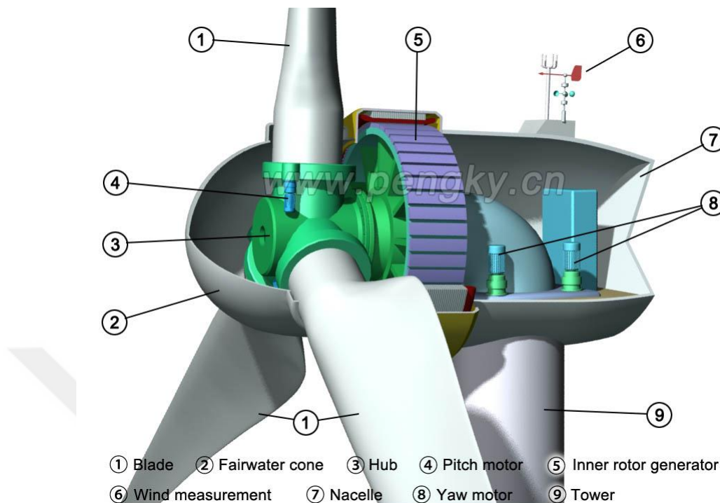
Figure 2.12. wind turbine parts.
