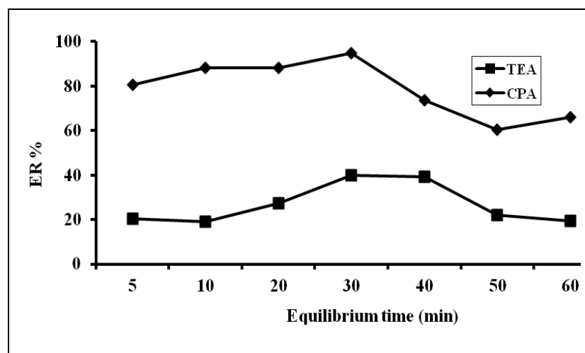
Figure 3.18 Effect of equilibration time on CPA and TEA extraction. Extraction conditions: synthetic sample solution, 2 mL; pH 2; volume of 4%w/v Triton X-114, 2 mL; volume of 1%w/v KNO 3 , 2 mL; T eq 50 °C
