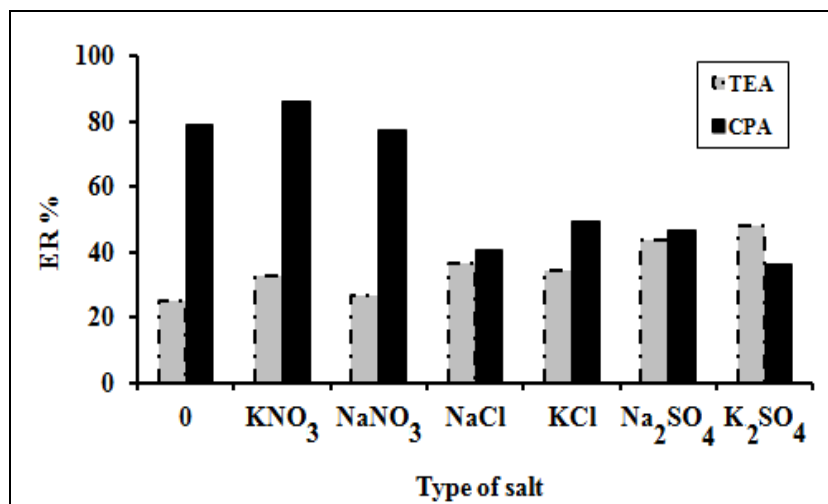
Figure 3.15 Effect of nature of salts on CPE and TEA extraction. Extraction conditions: synthetic sample solution, 2 mL; pH 2; volume of 4%w/v Triton X-114, 2 mL; volume of salt solution (1%,w/v, 2 mL; T_{eq} 60 °C
