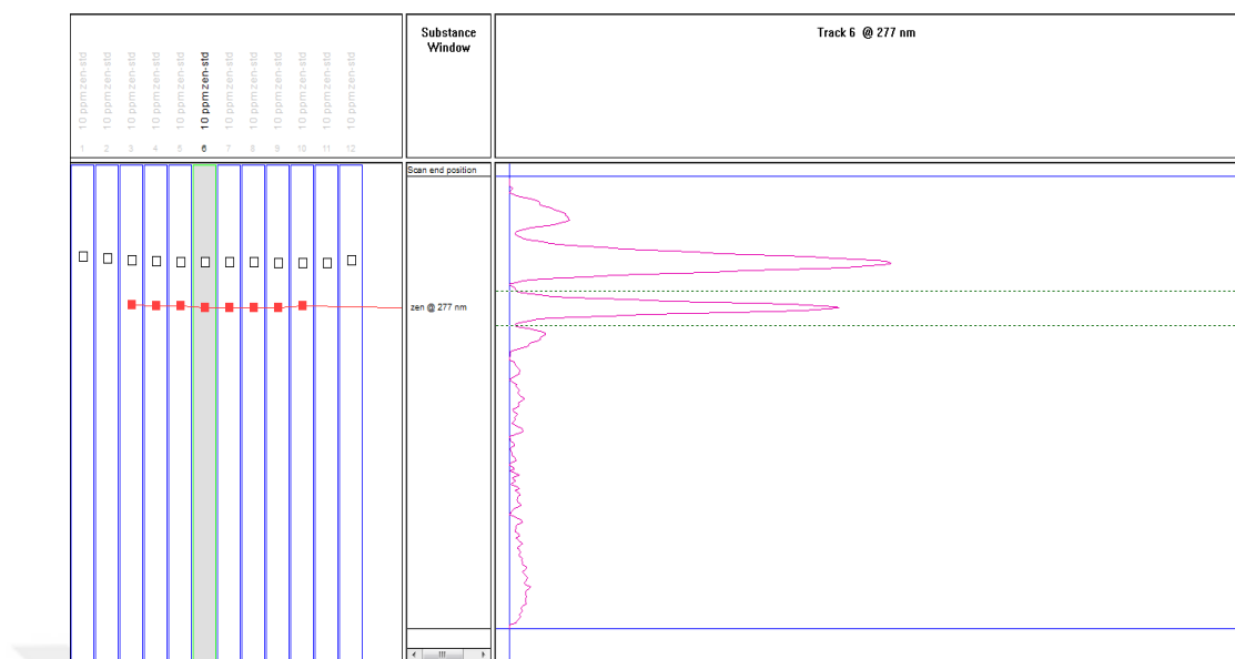
Figure 2.5 The HPTLC densitogram of standard ZEN
