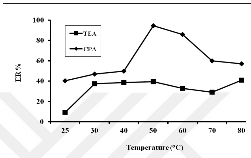
Figure 3.17 Effect of equilibrium temperature on CPA and TEA extraction. Extraction conditions: synthetic sample solution, 2 mL; pH 2; volume of 4%w/v Triton X-114, 2 mL; volume of 1%w/v KNO 3 , 2 mL
