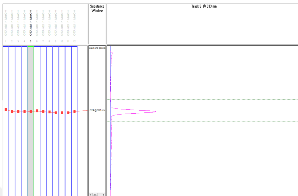
Figure 2.3 The HPTLC chromatogram of standard OTA
