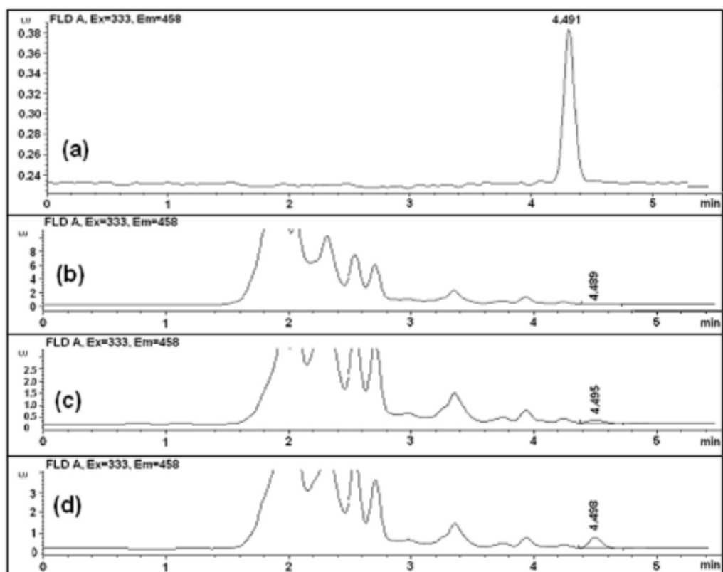
Figure 3.12 HPLC chromatogram of a) a standard OTA at 2.5 \text{ pg } \mu\text{L}^{-1} , b) unspiked wine sample containing app. 0.03 \text{ pg } \mu\text{L}^{-1} after DLLME method, c) same wine sample spiked at a conc. 0.1 \text{ pg } \mu\text{L}^{-1} after DLLME method and d) 0.5 \text{ pg } \mu\text{L}^{-1} .
