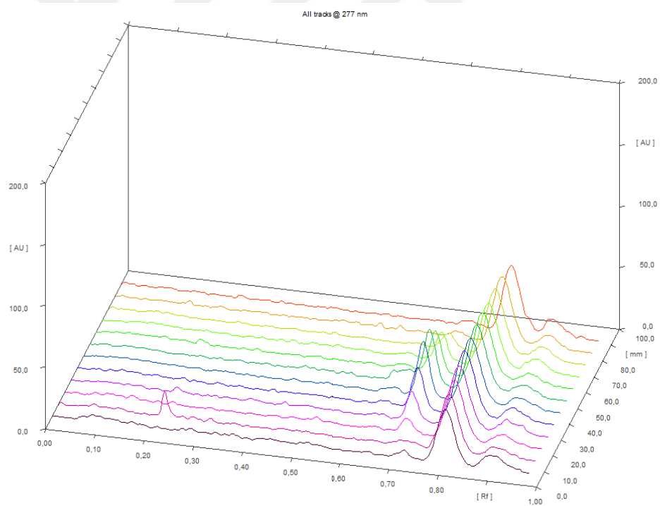
Figure 2.6 The HPTLC densitogram of standard ZEN
