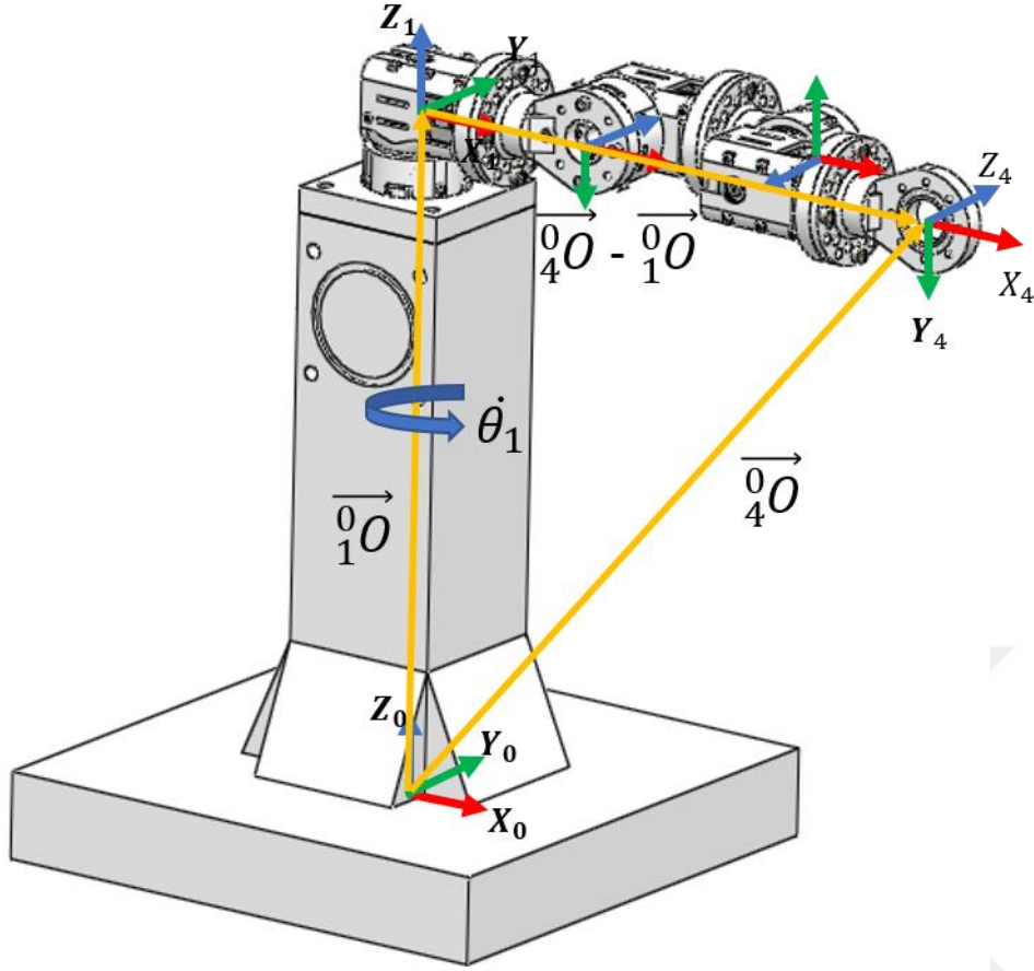
Figure 3.2 : Geometric Jacobian.
