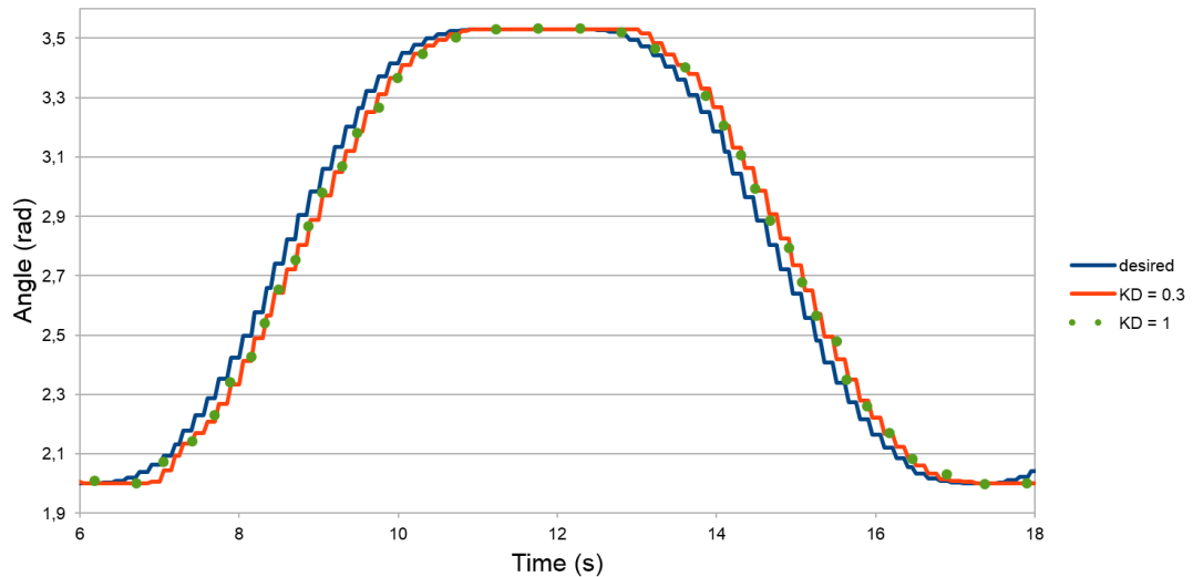
Figure 7.14 : Position tracking results of K_d coefficient determination of outer loop controller.
