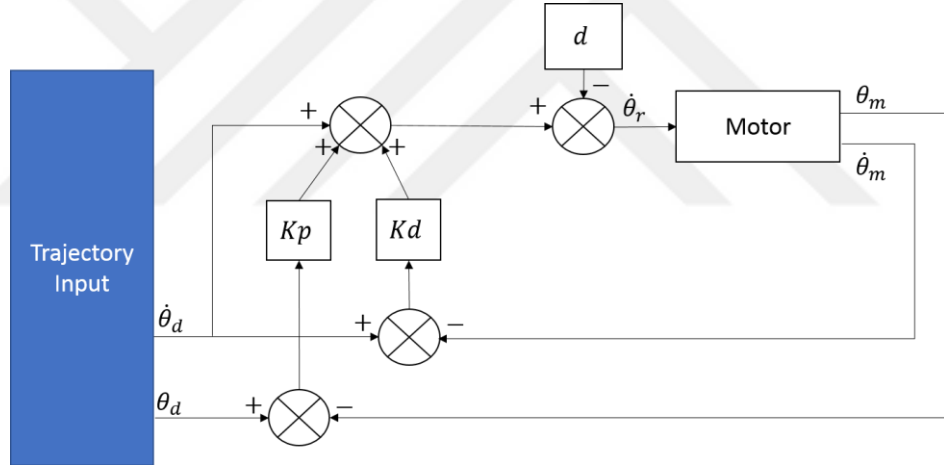
Figure 5.6 : Independent joint trajectory controller block diagram.
