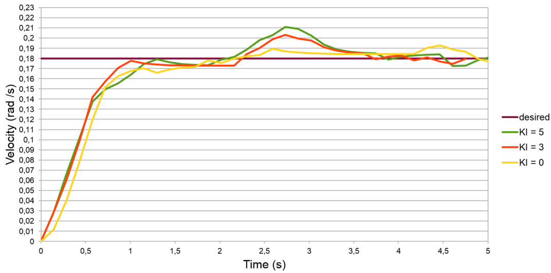
Figure 7.11 : K_i coefficient determination of inner loop controller.
