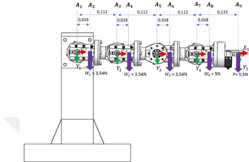
Figure 3.23 : 4 DOF modular robot manipulator payload analysis.
