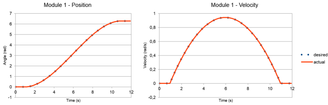
Figure 7.7 : Module 1 trajectory tracking results.
