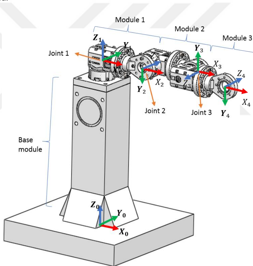
Figure 3.1 : 3 DOF modular robot configuration.
