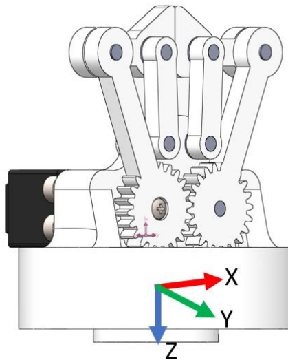
Figure 3.5 : Gripper module output coordinate frame.
