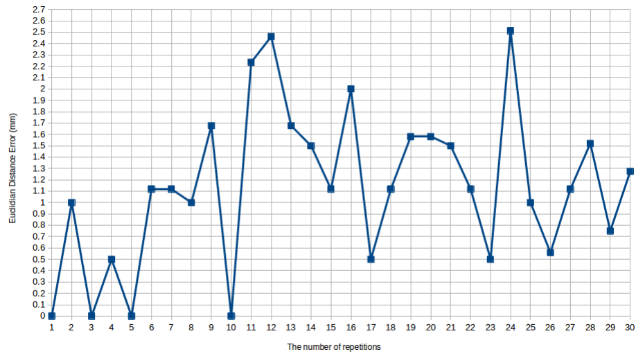
Figure 7.22 : Pick and Place task repeatability result.
