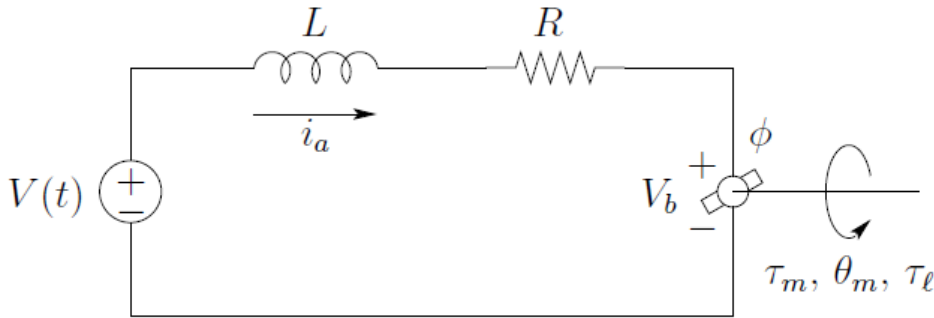
Figure 5.2 : DC motor model.
