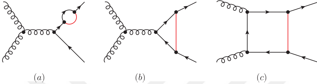
Figure 3.5: Generic self-energy, vertex-correction, and box diagrams for the process gg \rightarrow t\bar{c} .
