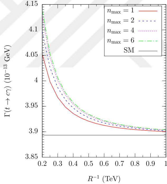
Figure 3.7: MUED contributions to the process t \rightarrow c\gamma as a function of the maximum KK number, n_{\max} , and the inverse radius of the extra dimension, R .
