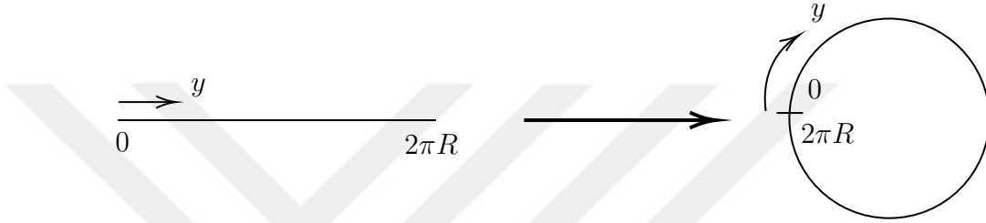
Figure 2.1: Compactification of the extra dimension on a circle of radius R .
