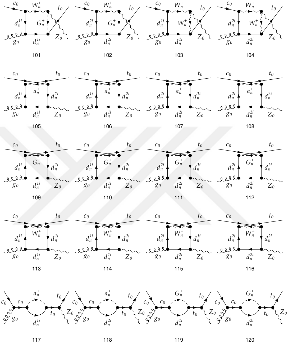
Figure A.66: MUED diagrams contributing to the process cg \rightarrow tZ .
