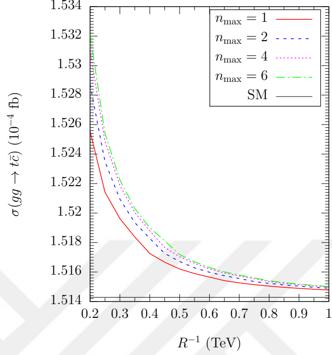
Figure 3.12: MUED contributions to the process gg \rightarrow t\bar{c} as a function of the maximum KK number, n_{\max} , and the inverse radius of the extra dimension, R .
