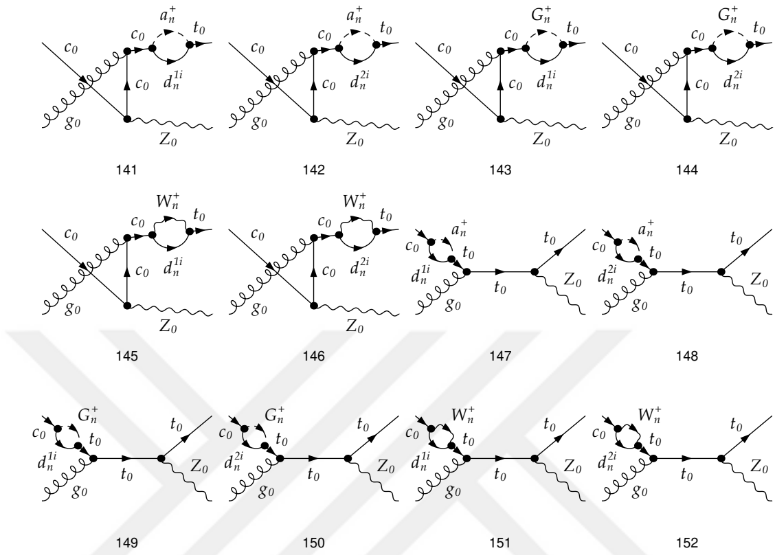
Figure A.68: MUED diagrams contributing to the process cg \rightarrow tZ .
