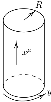
Figure 2.2: The 5D cylindrical universe.
