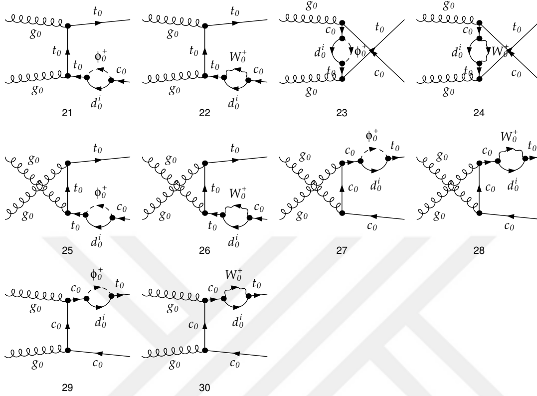
Figure A.9: SM diagrams contributing to the process gg \rightarrow t\bar{c} .
