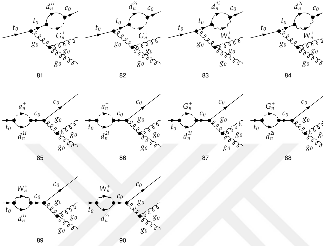
Figure A.33: MUED diagrams contributing to the process t \rightarrow cgg .
