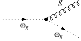
Figure 3.2: Gluon ghosts replaced with two gluons in the triple gluon vertex.
