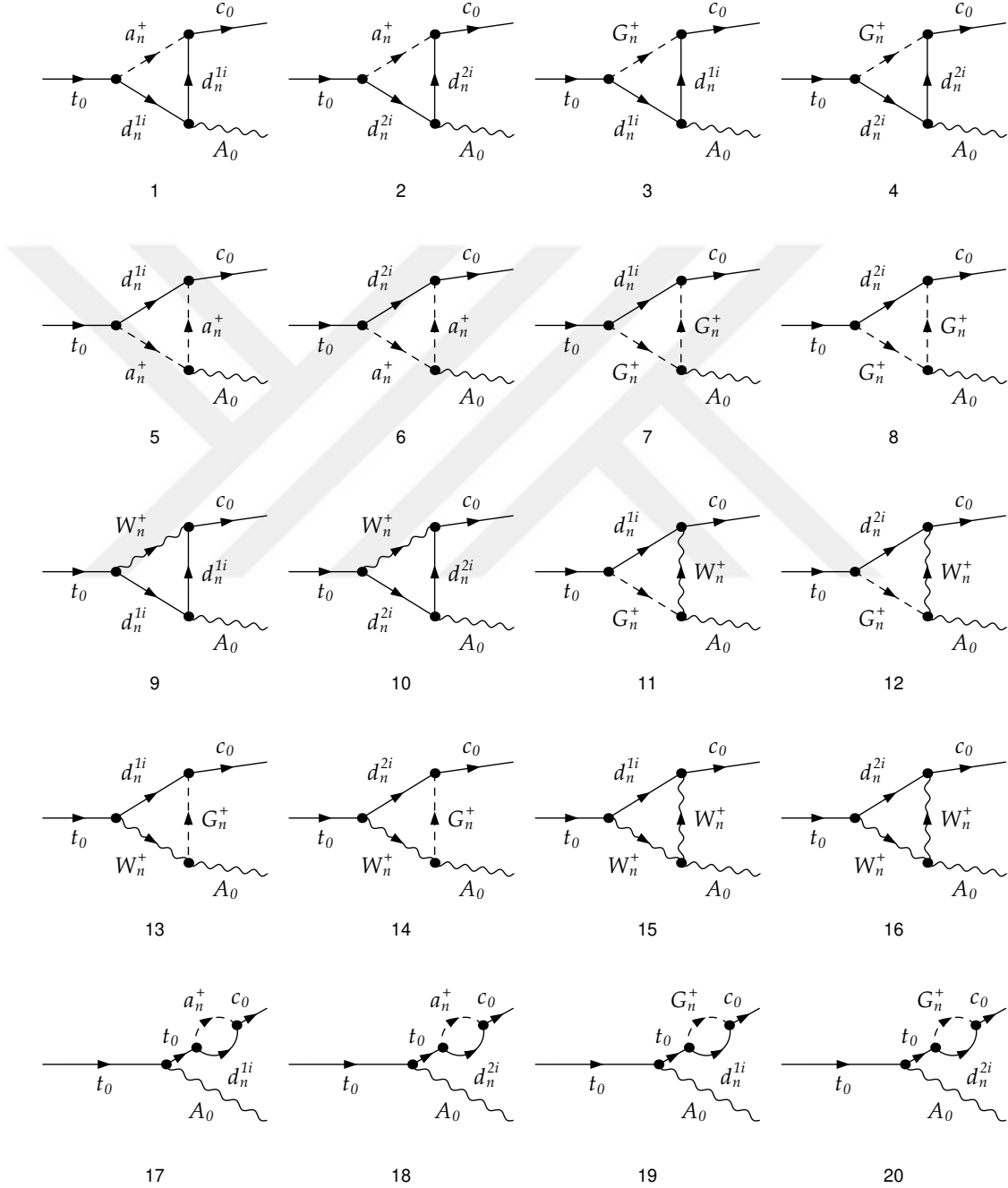
Figure A.20: MUED diagrams contributing to the process t \rightarrow c\gamma .
