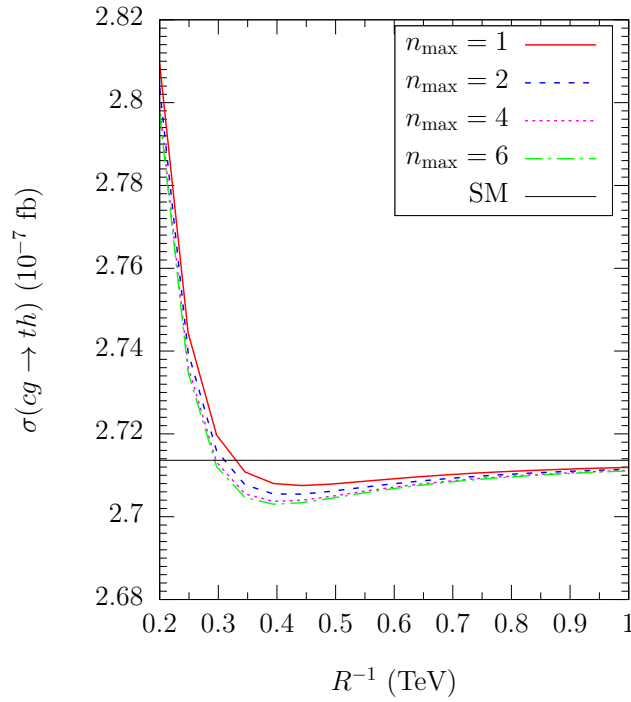
Figure 3.15: MUED contributions to the process cg \rightarrow th as a function of the maximum KK number, n_{\max} , and the inverse radius of the extra dimension, R .
