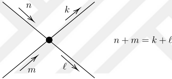
Figure 2.6: The sum of KK numbers incoming to a 4-point interaction is equal to the sum of KK numbers outgoing from the vertex.
