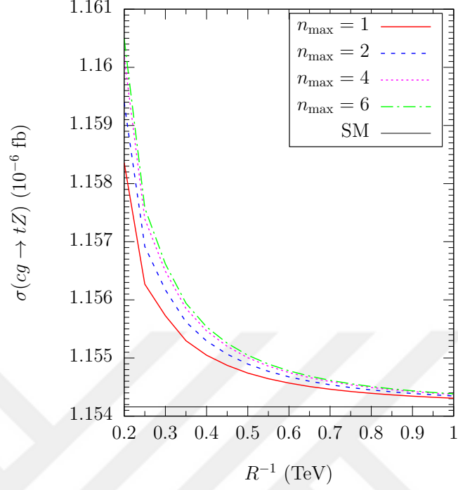
Figure 3.16: MUED contributions to the process cg \rightarrow tZ as a function of the maximum KK number, n_{\max} , and the inverse radius of the extra dimension, R .
