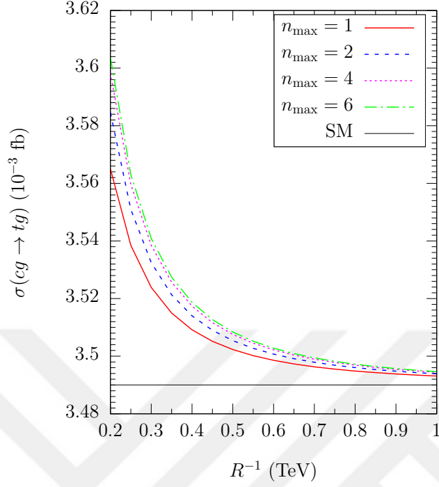
Figure 3.14: MUED contributions to the process cg \rightarrow tg as a function of the maximum KK number, n_{\max} , and the inverse radius of the extra dimension, R .
