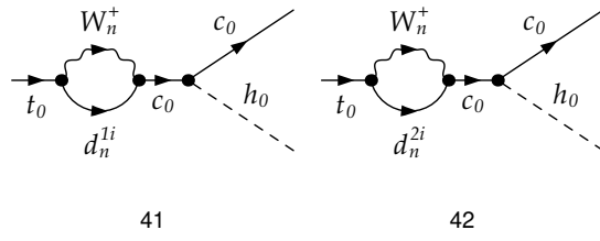
Figure A.25: MUED diagrams contributing to the process t \rightarrow ch .
