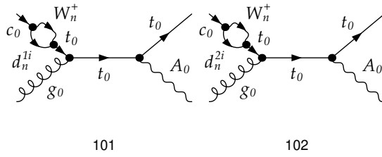
Figure A.46: MUED diagrams contributing to the process cg \rightarrow t\gamma .
