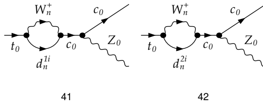
Figure A.28: MUED diagrams contributing to the process t \rightarrow cZ .
