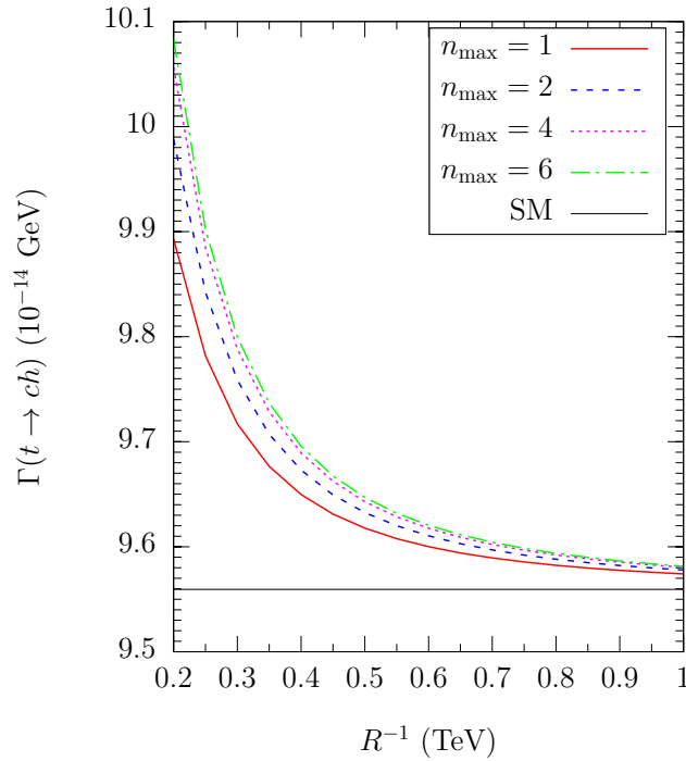
Figure 3.9: MUED contributions to the process t \rightarrow ch as a function of the maximum KK number, n_{\max} , and the inverse radius of the extra dimension, R .
