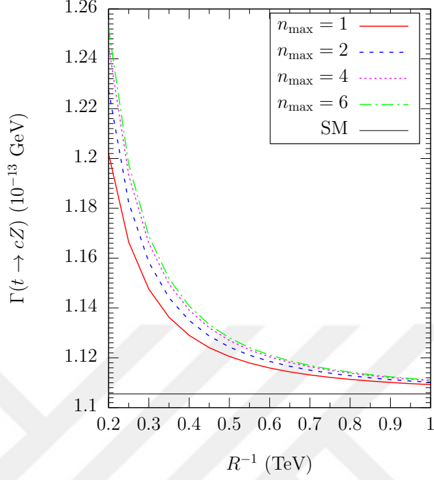
Figure 3.10: MUED contributions to the process t \rightarrow cZ as a function of the maximum KK number, n_{\max} , and the inverse radius of the extra dimension, R .
