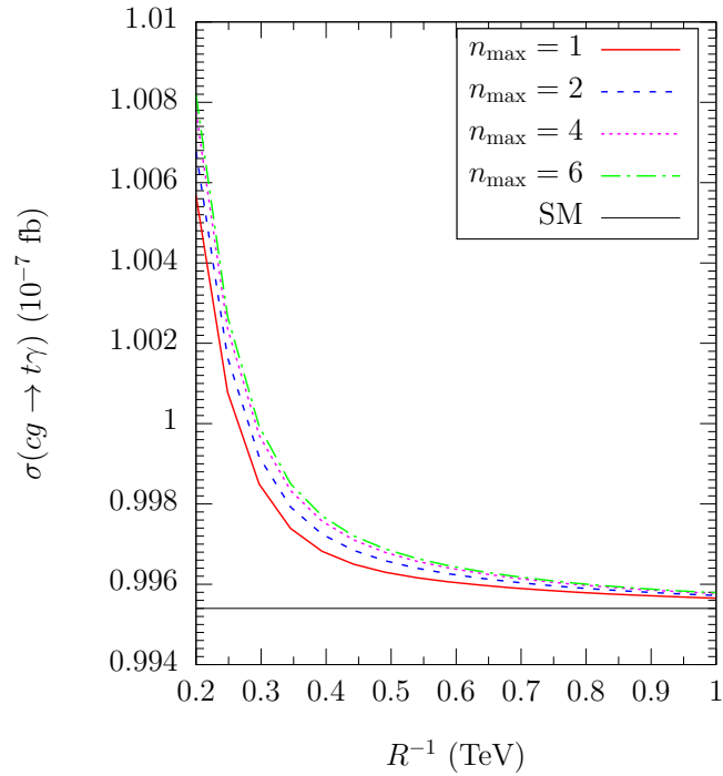
Figure 3.13: MUED contributions to the process cg \rightarrow t\gamma as a function of the maximum KK number n_{\max} , and the inverse radius of the extra dimension, R .
