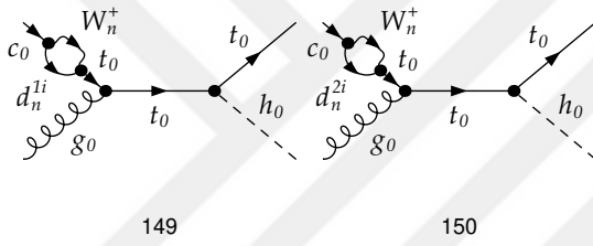
Figure A.60: MUED diagrams contributing to the process cg \rightarrow th .
