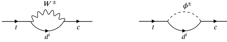
Figure 1.1: The loop that appears in the rare top quark processes occurring by FCNCs in the Feynman gauge.
