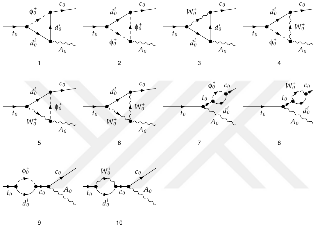
Figure A.1: SM diagrams contributing to the process t \rightarrow c\gamma .
