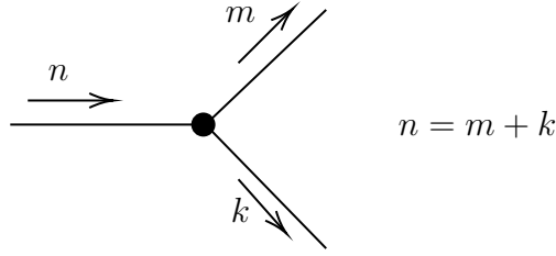
Figure 2.5: The sum of KK numbers incoming to a 3-point interaction is equal to the sum of KK numbers outgoing from the vertex.
