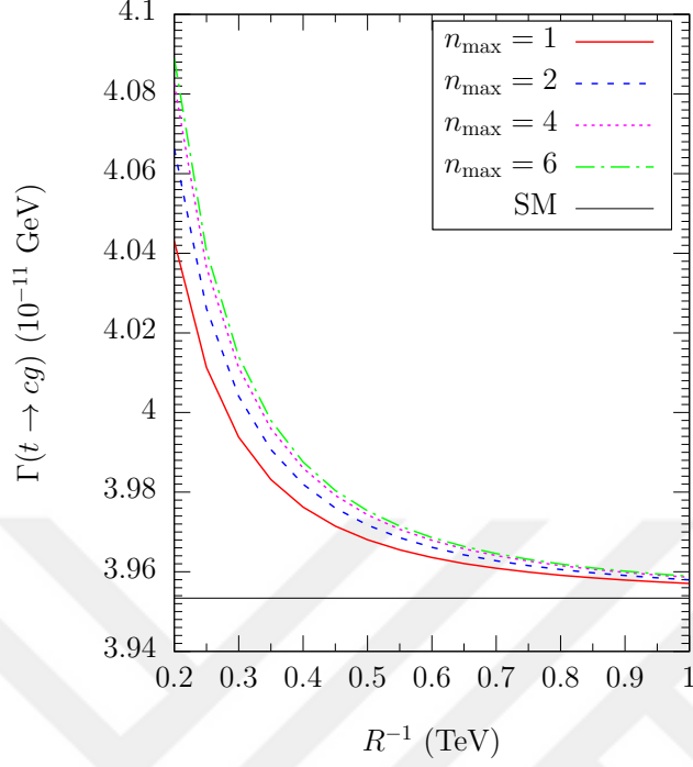
Figure 3.8: MUED contributions to the process t \rightarrow cg as a function of the maximum KK number, n_{\max} , and the inverse radius of the extra dimension, R .
