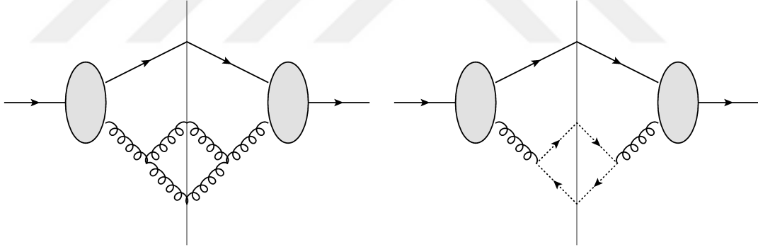
Figure 3.1: Gluon loops in the matrix element squared for the process t \rightarrow cgg .
