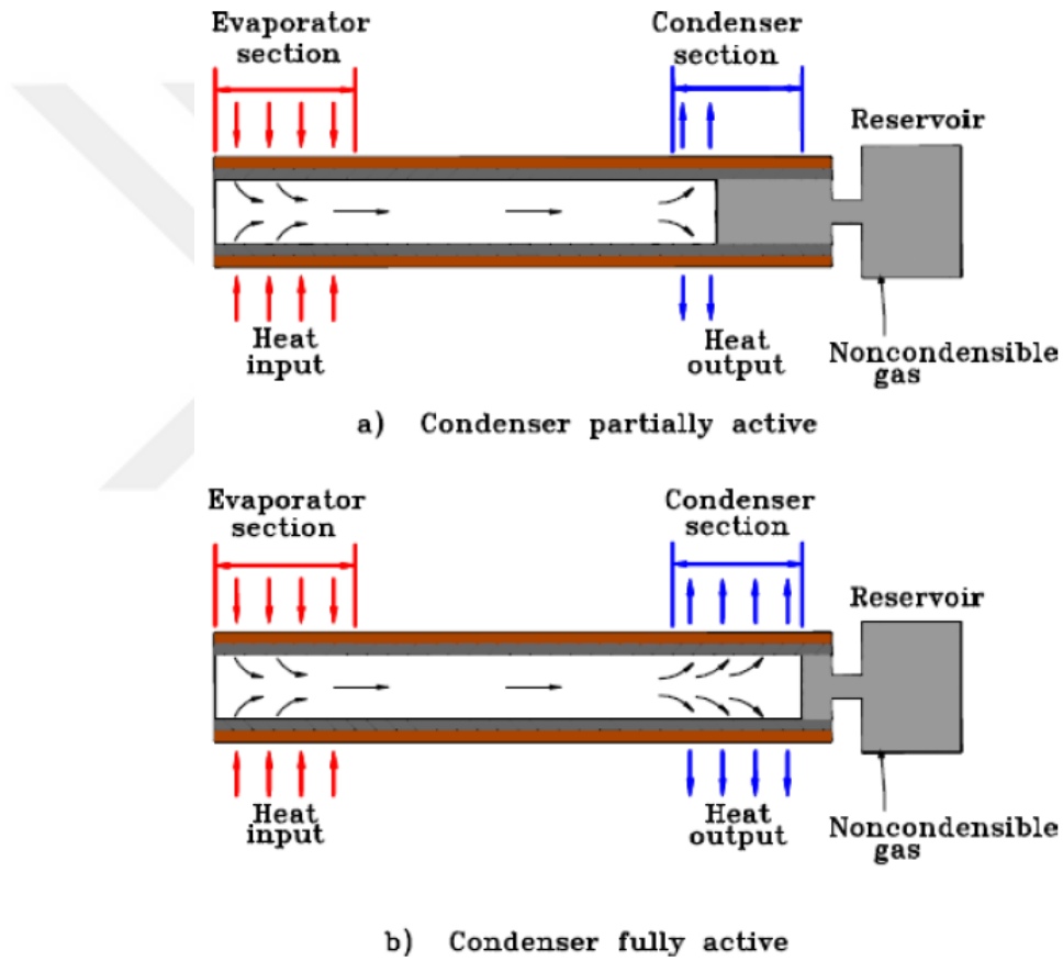
Figure 1.5: Variable conductive heat pipe [3]
