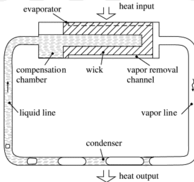
Figure 1.4: Loop heat pipe [6]
