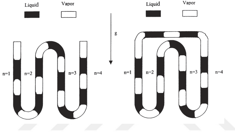
Figure 1.6: Open loop and closed loop pulsating heat pipes [7]
