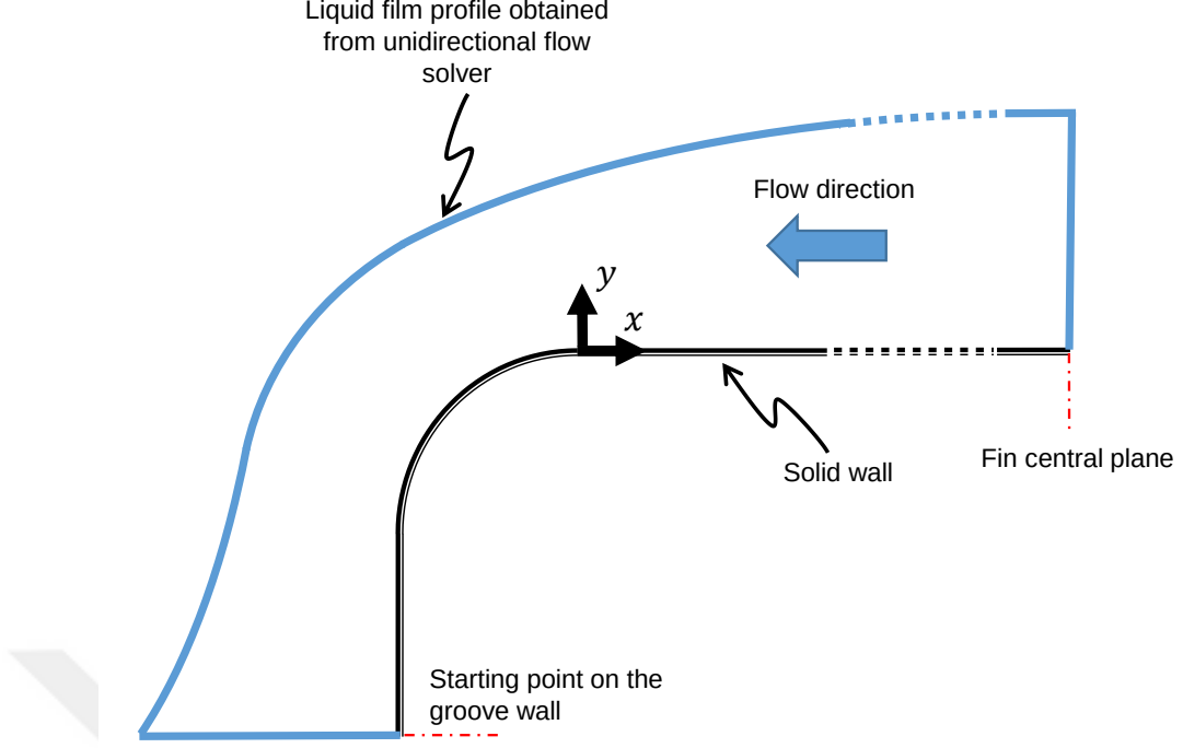
Figure 4.1: The problem domain used in the COMSOL simulations
