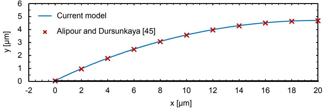
Figure 3.8: Comparison of the film profile obtained by the current model with the one presented by Alipour and Dursunkaya [45]
