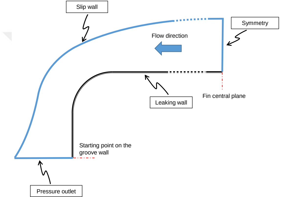
Figure 4.2: Boundary conditions specified in the COMSOL simulations
