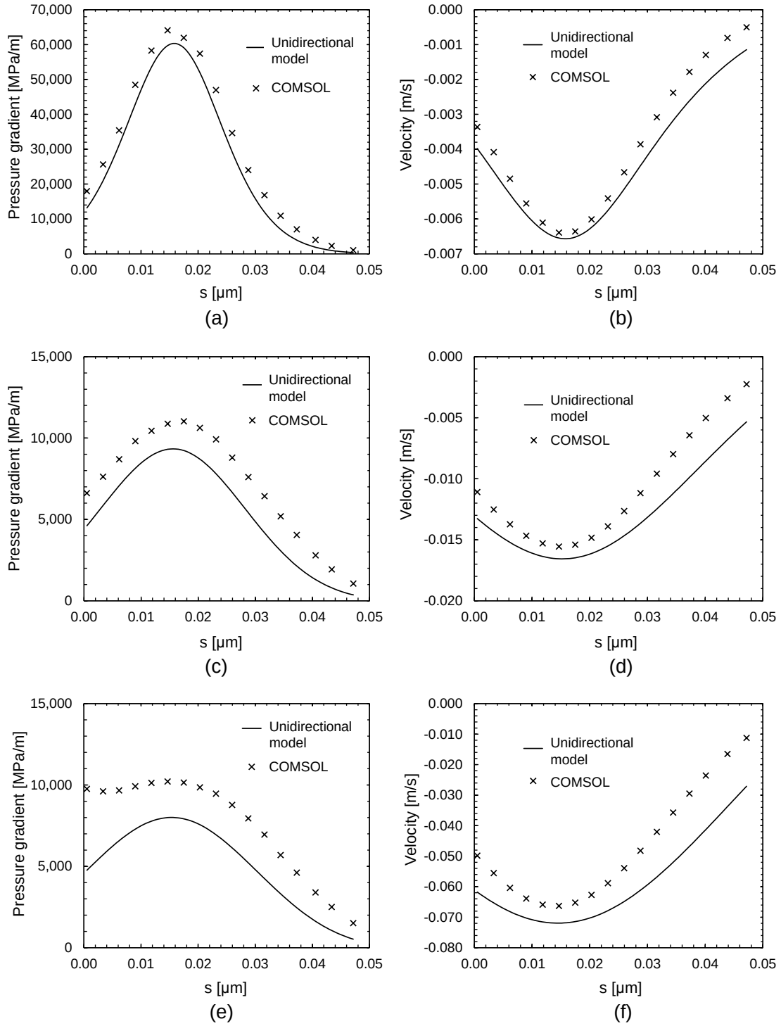
Figure 4.8: Comparison of the results of uni-directional model and COMSOL simulations: pressure gradient, dp_l/ds , at the corner region at the middle height ( \delta/2 ) for (a) 10^{-2} , (c) 10^{-1} , (e)1.0 K subcoolings; s - component of the free surface velocity at the corner region for (b) 10^{-2} , (d) 10^{-1} , (f)1.0 K subcoolings
