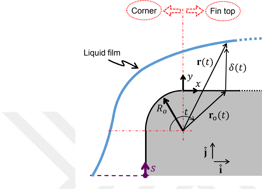
Figure 3.6: Parametric representation for the transition from corner to fin top
