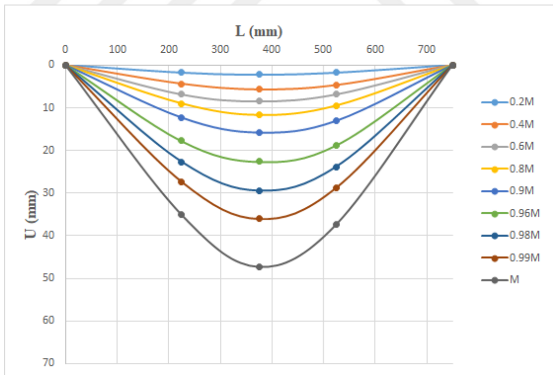
Figure 4.11 Deflection shape of the specimen 3-S-30×30-C.
