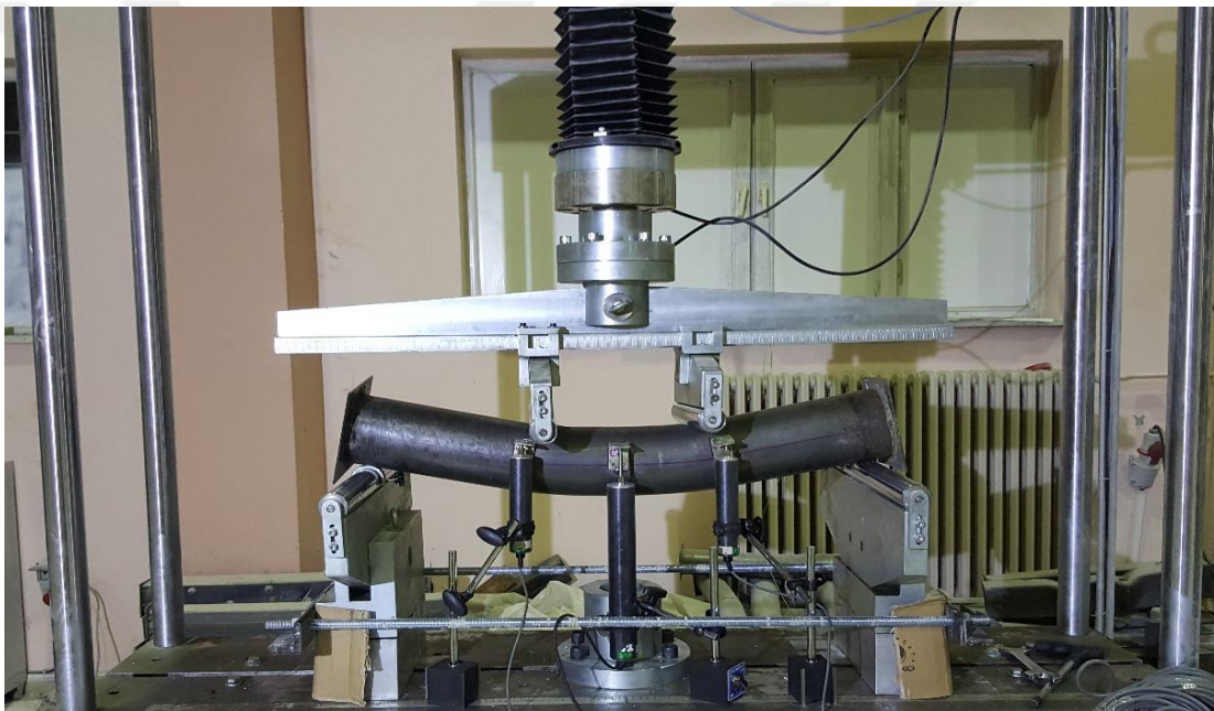
Figure 4.5 Deflected specimen.
