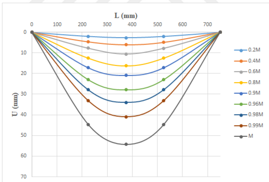
Figure 4.13 Deflection shape of the specimen 3-S-30×30-B.
