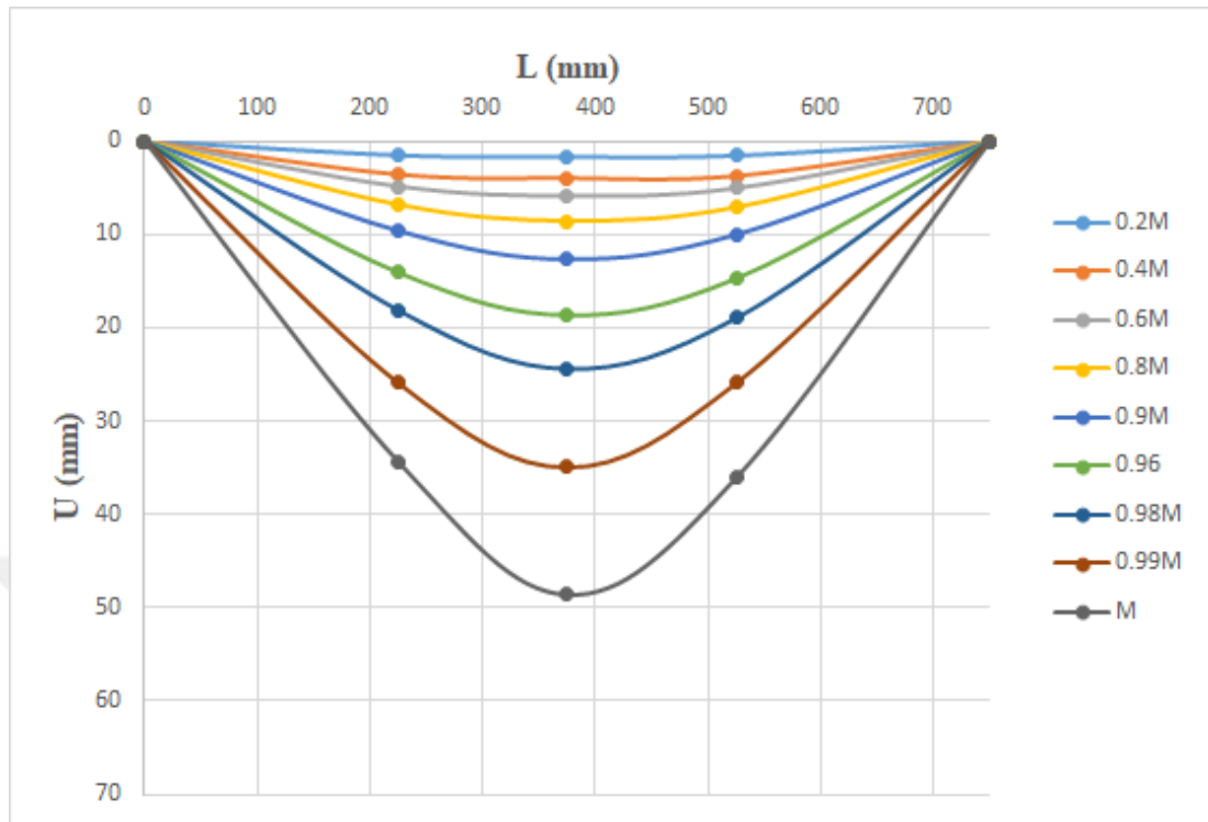
Figure 4.10 Deflection shape of the specimen 3-R-40×20-C.
