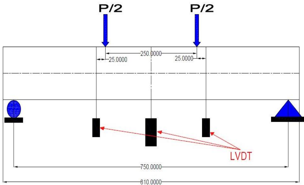
Figure 3.9 Sketch of test details.
