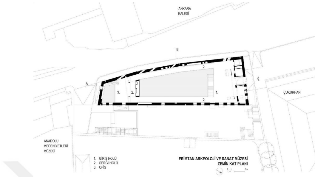
Figure 62. Ground plan drawing of Erimtan Museum.
