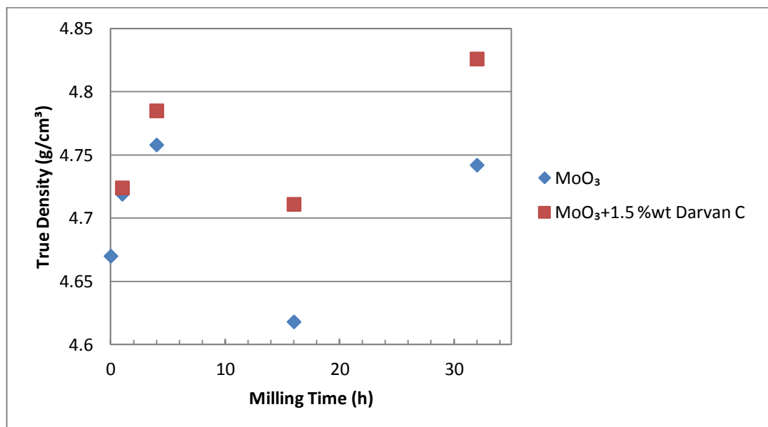
Figure 6.18: True density values of \text{MoO}_3 samples at different milling times.
