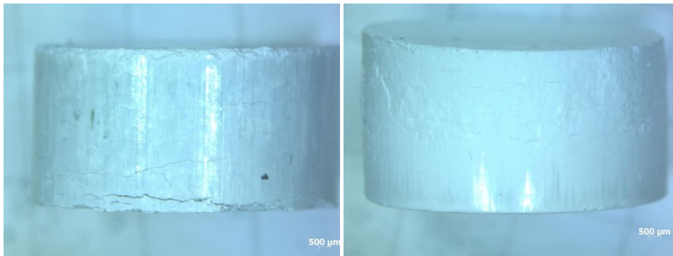
Figure 6.42: Sintered pellets of: a) M1 and b) M6 samples.
