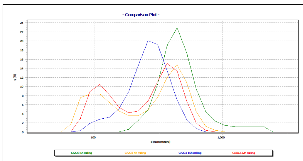
Figure 6.9: Comparative plots of particle size distributions of the HEM'd Cr 2 O 3 samples milled for 1, 4, 16, and 32 hours.
