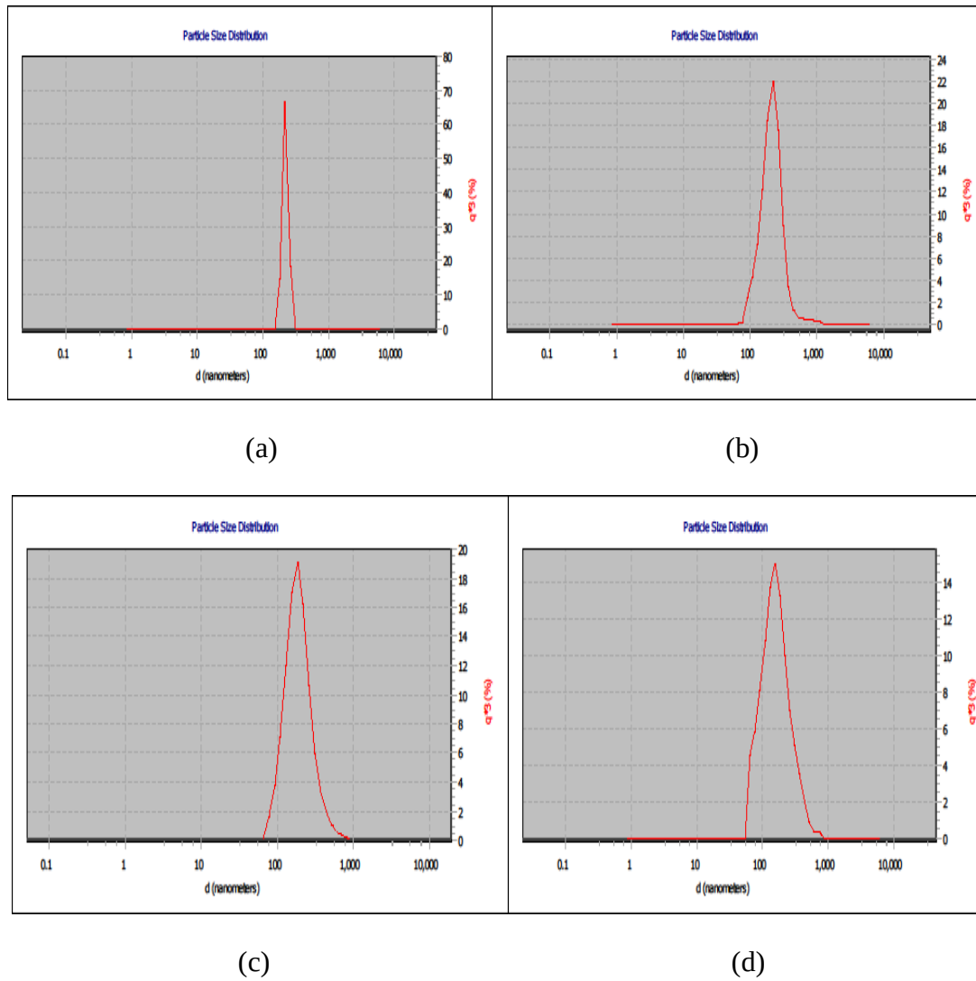
Figure 6.3: Particle size distributions of HEM'd \text{MoO}_3 +Darvan C samples with different milling times of: a) 1 hour, b) 4 hours, c) 16 hours and, d) 32 hours.
