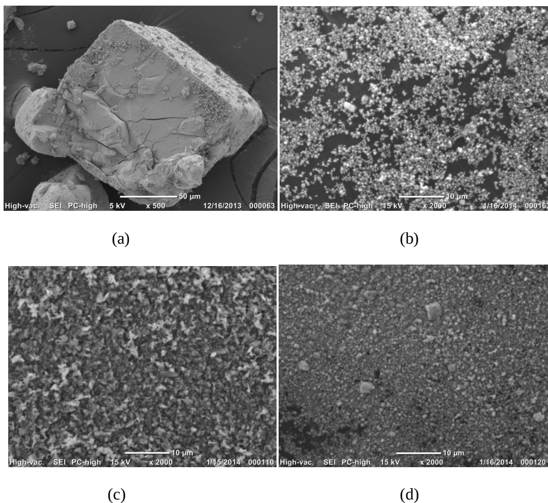
Figure 6.27: SEM images of: a) initial, b) 4h HEM'd, c) 16h HEM'd, and d) 32h HEM'd MoO 3 samples.
