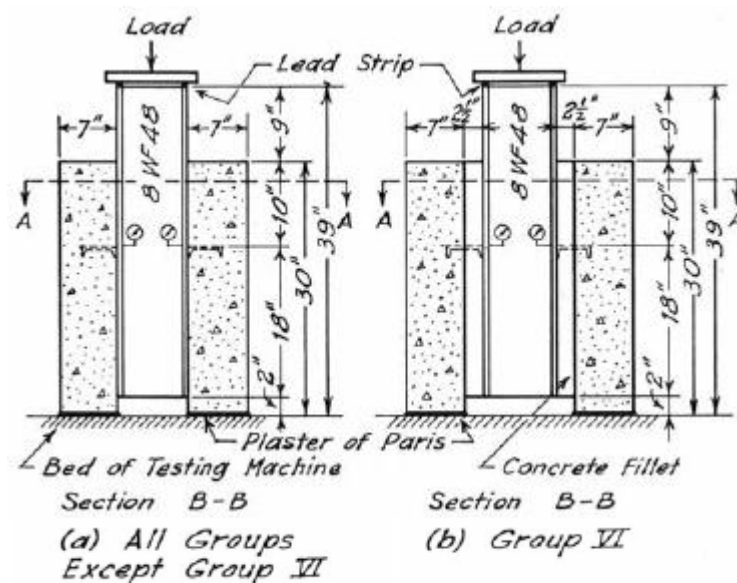
Figure 1.9 Push-Out Specimens (Ref: Viest et al., 1952)
