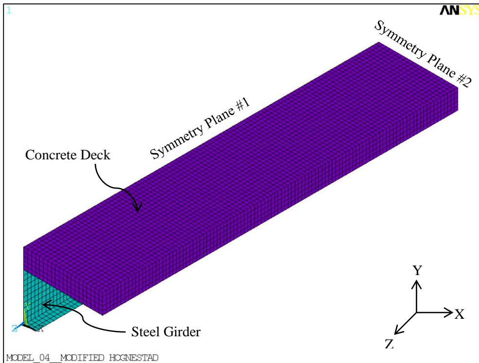
Figure 3.11 ANSYS Model
