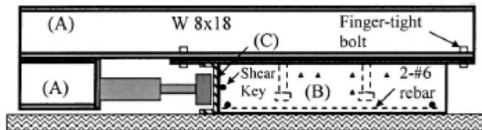
Figure 1.10 Push-Out Test Setup (Ref: Topkaya, 2004)
