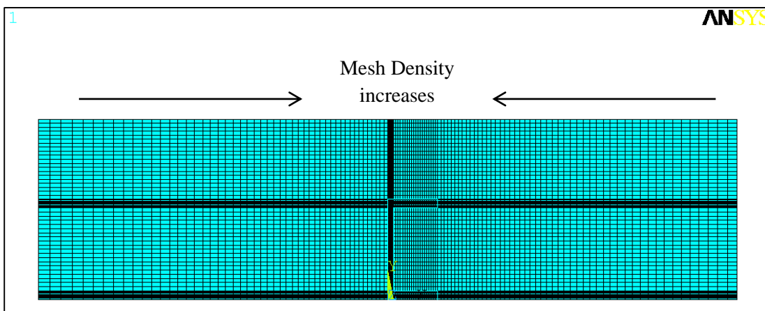
Figure 2.5 Meshed Geometry in ANSYS (*UM)
