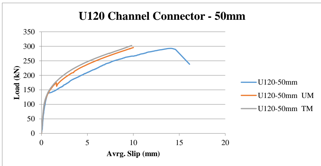
Figure 2.12.a U120 Channel Connector Results for 50mm Length
