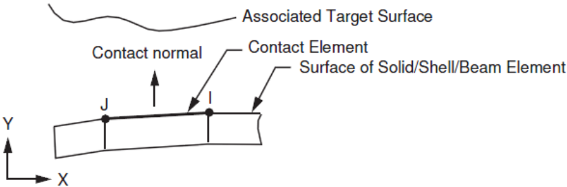
Figure 2.2.b CONTA171 Geometry (Ref: ANSYS, 2010)
