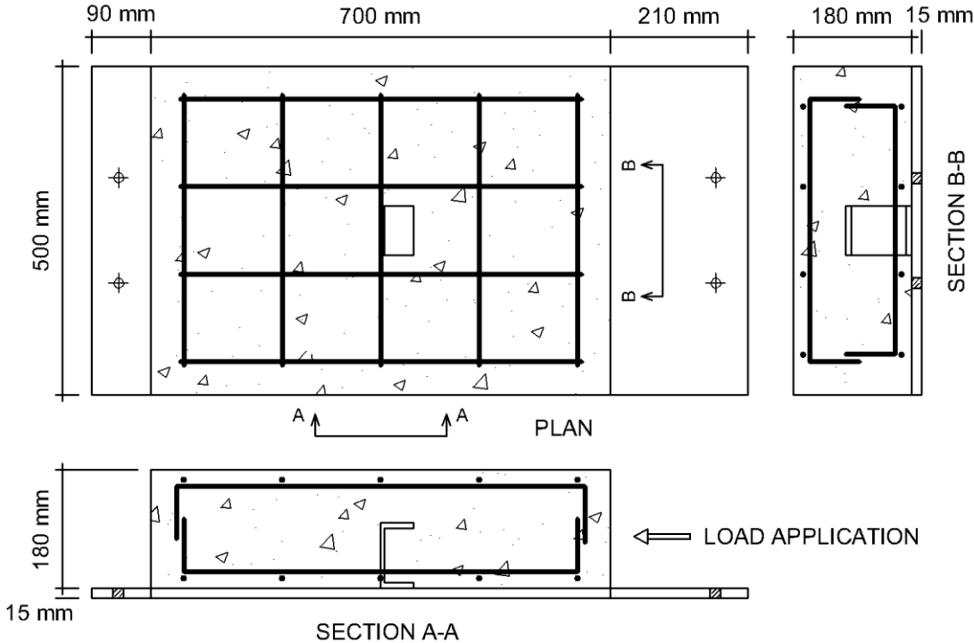
Figure 1.12 Push-Out Specimen Reinforcement Drawing
