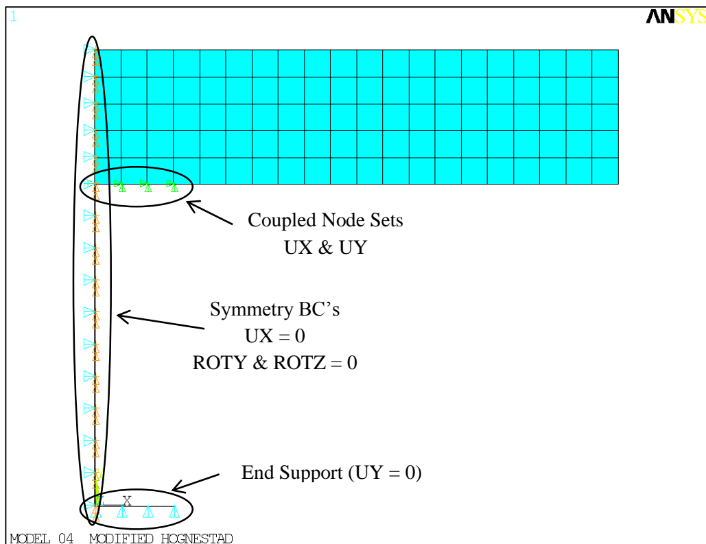
Figure 3.13 Boundary Conditions for the Model
