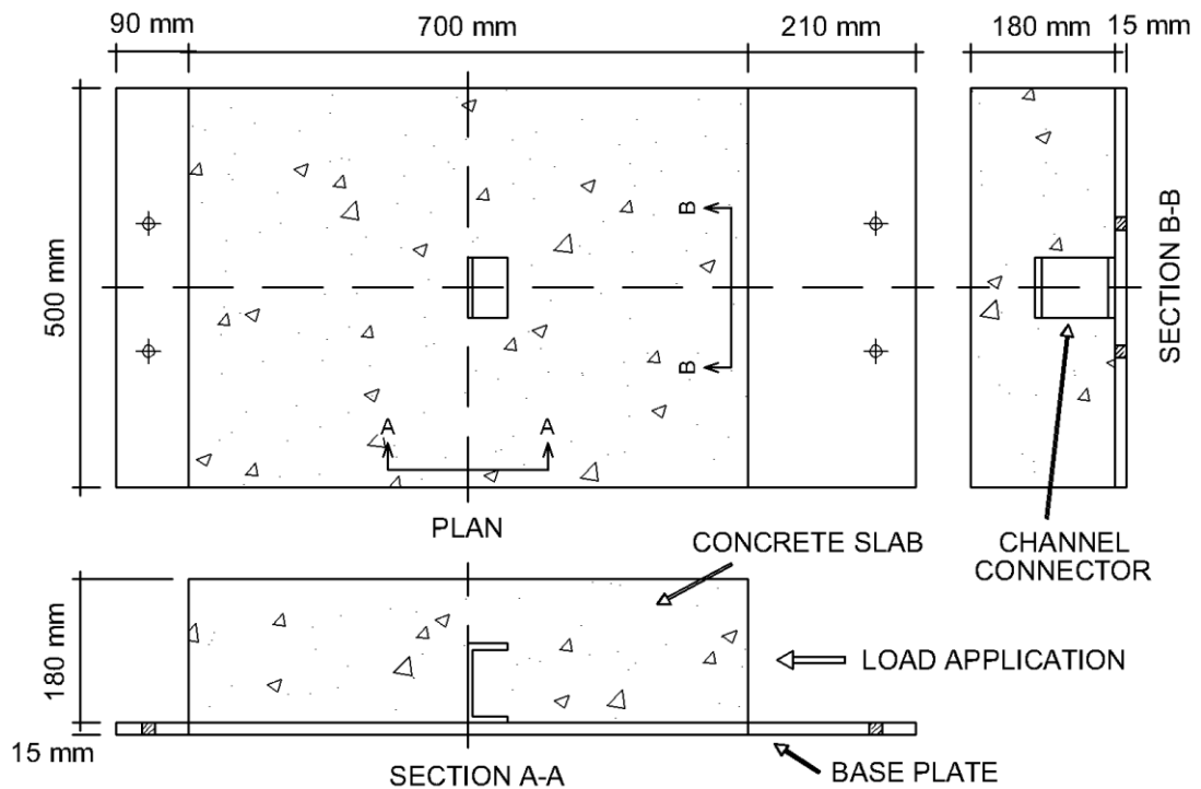
Figure 1.11 Push-Out Specimen
