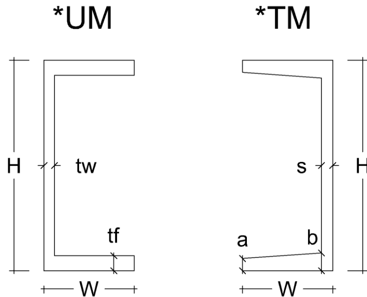
Figure 2.3 Two Different Channel Models Untapered Model, UM (left hand side) Tapered Model, TM (right hand side)
