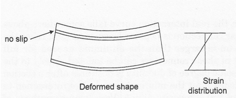
Figure 1.3 Complete Interaction (Ref: Viest et al., 1997)
