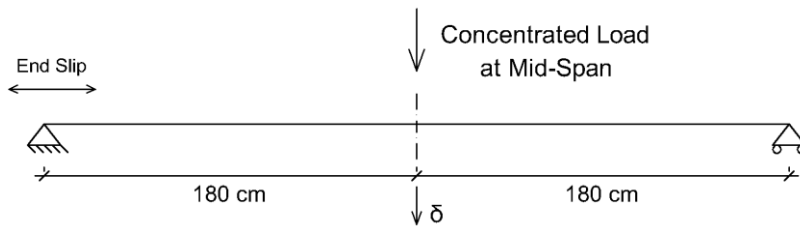
Figure 3.1.b Beam Dimensions
