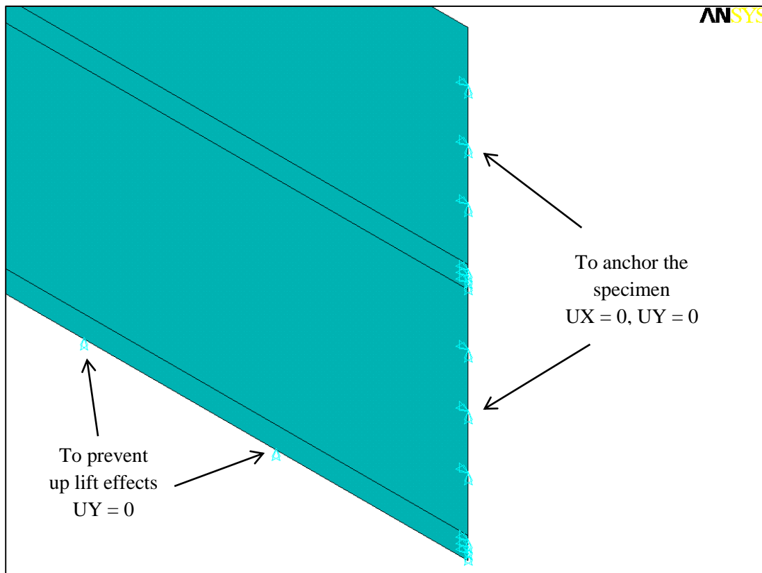
Figure 2.7 Boundary Conditions
