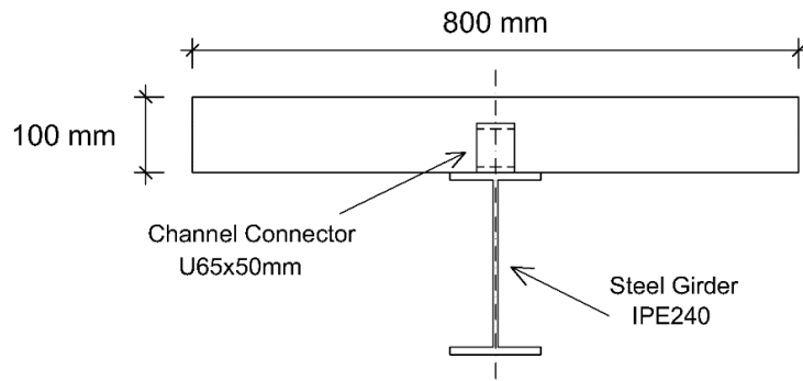
Figure 3.1.a Cross-Section of the Beam Specimen
