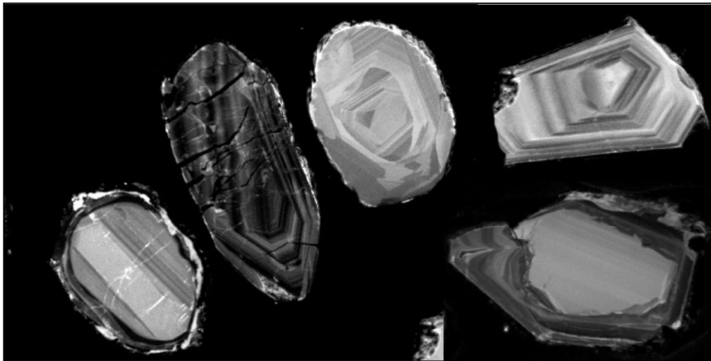
Figure A.6 Cathodoluminescence images of detrital zircons from Kurudere metaconglomerates (sample 331).
