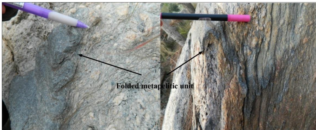
Figure 4.10 Folded thin, fine-grained dark metapelitic unit within the metaconglomerates, Karaburun Ridge.
