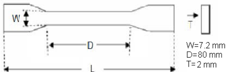
Figure 3.6 – Dimensions for dog-bone mold
