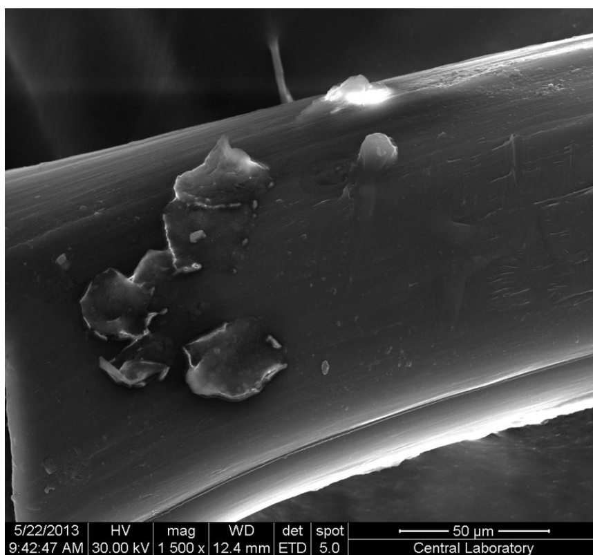
Figure 4.6b – SEM micrograph of PET showing the deformations on the surface
