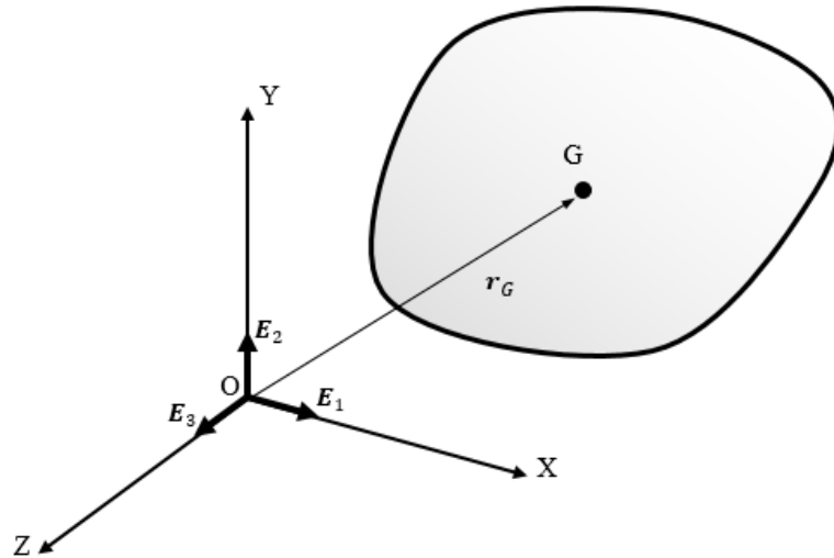
Figure 1. Center of gravity position of the given solid body is defined as \mathbf{r}_G = x_G \mathbf{E}_1 + y_G \mathbf{E}_2 + z_G \mathbf{E}_3.
