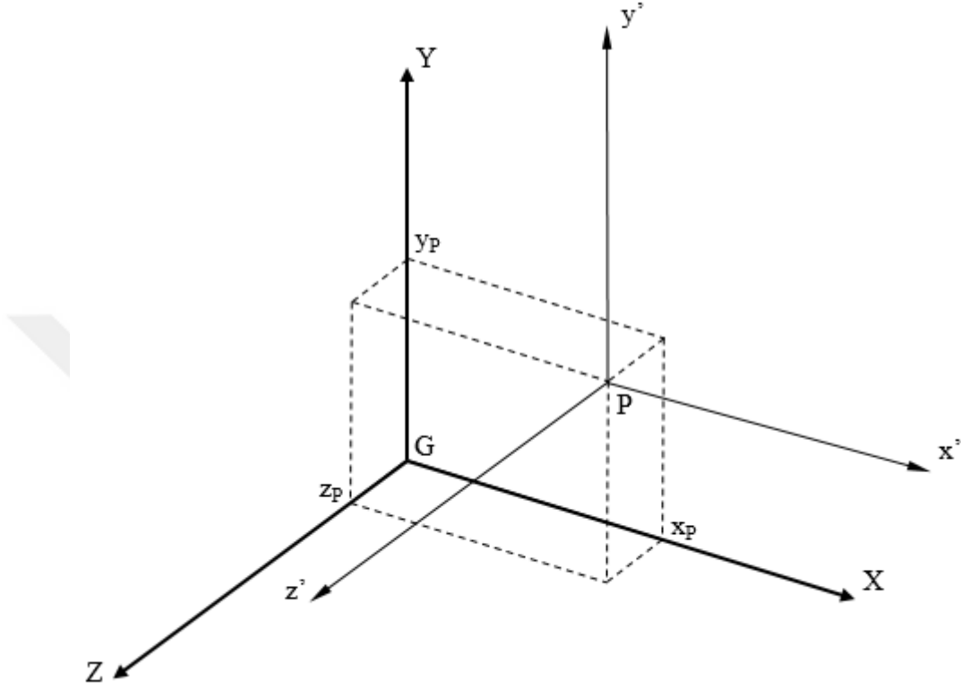
Figure 12. Inertia parameters with respect to center of gravity G and arbitrary point P can be correlated by using parallel distances between their axes.
