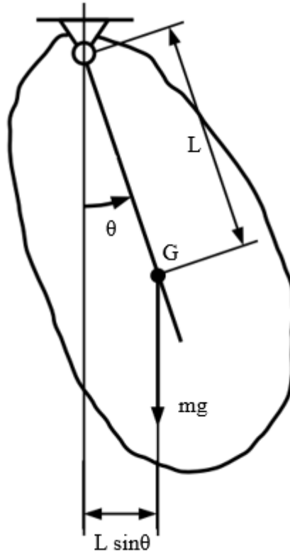
Figure 18. Initial displacement, \theta , is given to the specimen and gravitational force tries to bring the specimen to the equilibrium.
