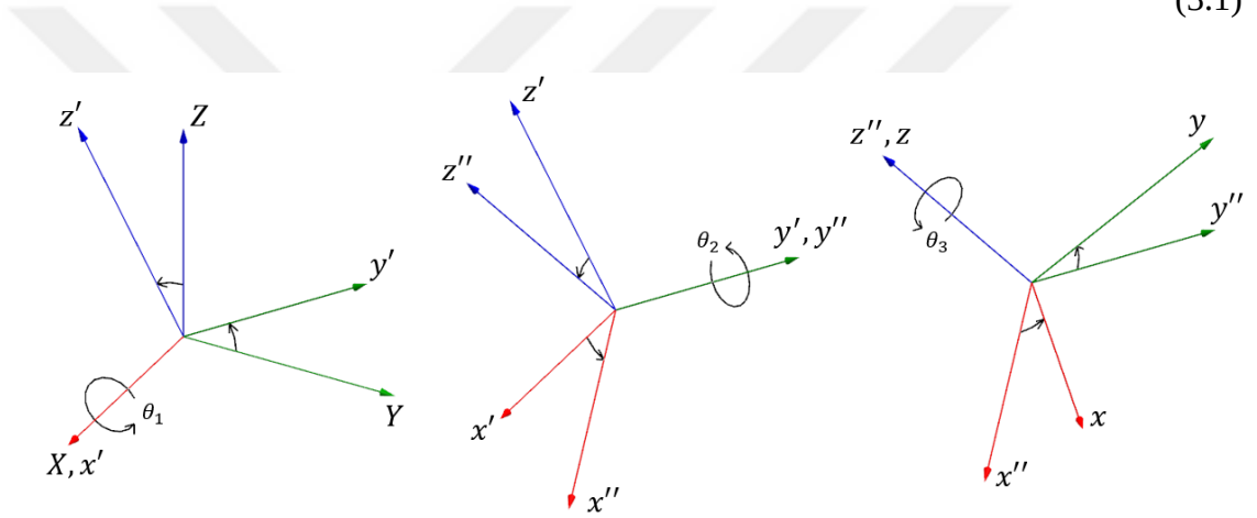
Figure 35. Sequential rotation and intermediate coordinate systems are demonstrated. Rotational velocity and acceleration values seen in equations (3.1) are derived using the outputs of the encoders. Taking derivatives of these angular displacements does not give the rotational velocity of the body directly. Because the measured angular displacements are the rotations of the intermediate coordinate systems between the fixed and body coordinate systems. Using Figure 35, that statement can be explained more precisely as
