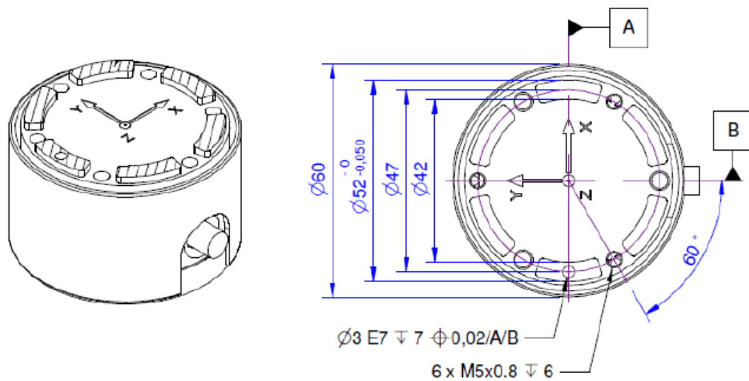
Figure B-2. Dimensions of the load sensor
