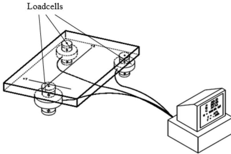
Figure 17. Test specimen is placed on the plate shown and arising forces are measured. [12]
