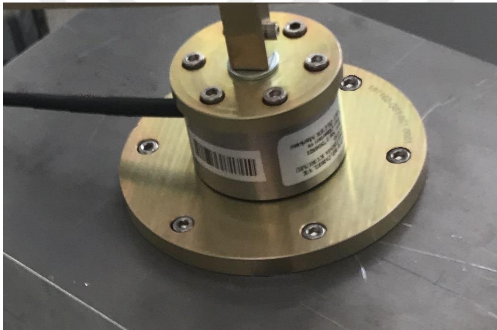
Figure 33. 6-axis load sensor and its connection interfaces
