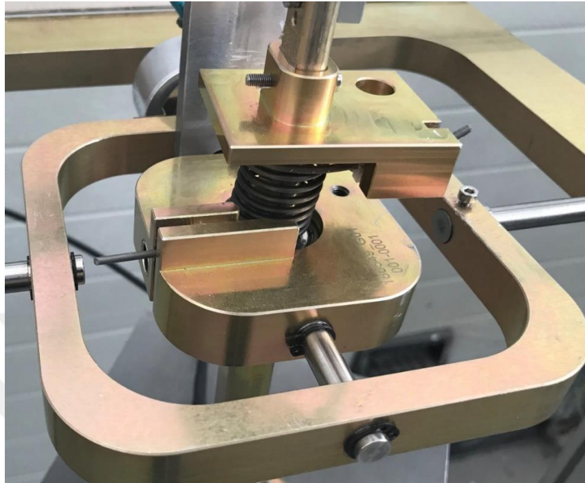
Figure 31. Torsional spring between frame 1 and extension link
