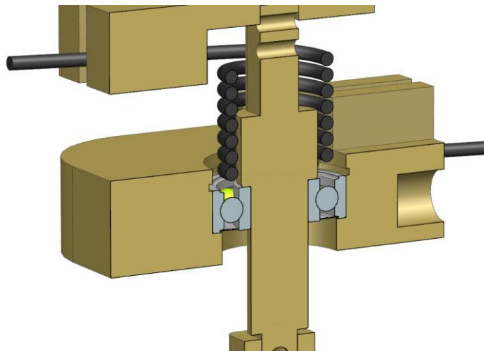
Figure 29. Bearing and rotational spring between the frame 1 and the extension link is shown.
