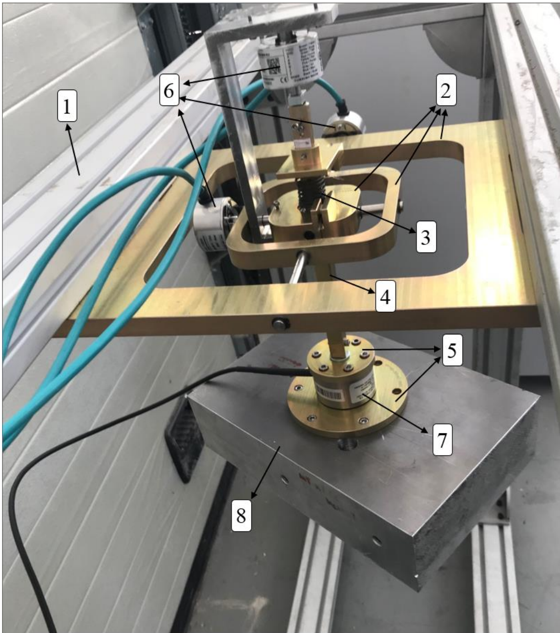
Figure 25. The configuration of test device is given. Main parts of the system are numbered.
