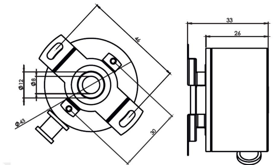
Figure A-2. Dimensions of the rotary encoder
