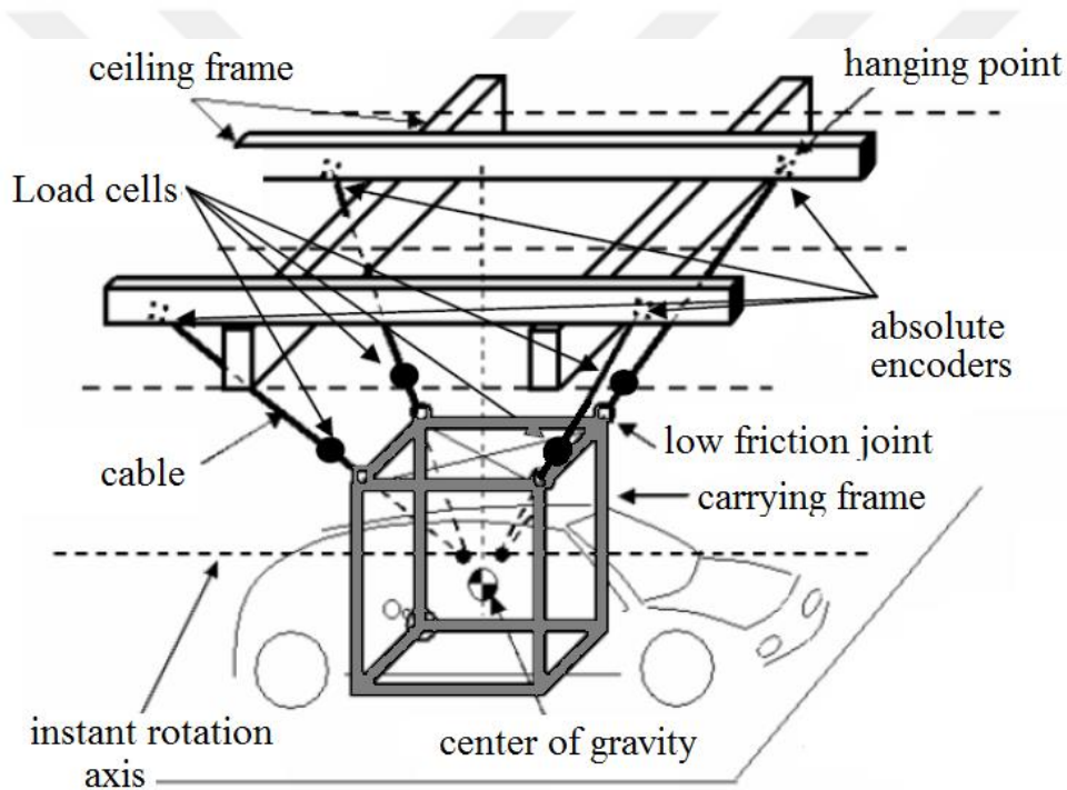
Figure 22. The test specimen is hanged with four non-parallel cables. [33]
