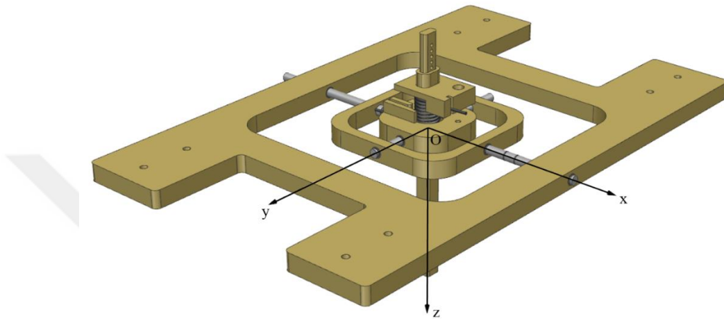
Figure 28. Nested frames and the reference coordinate axes are shown.
