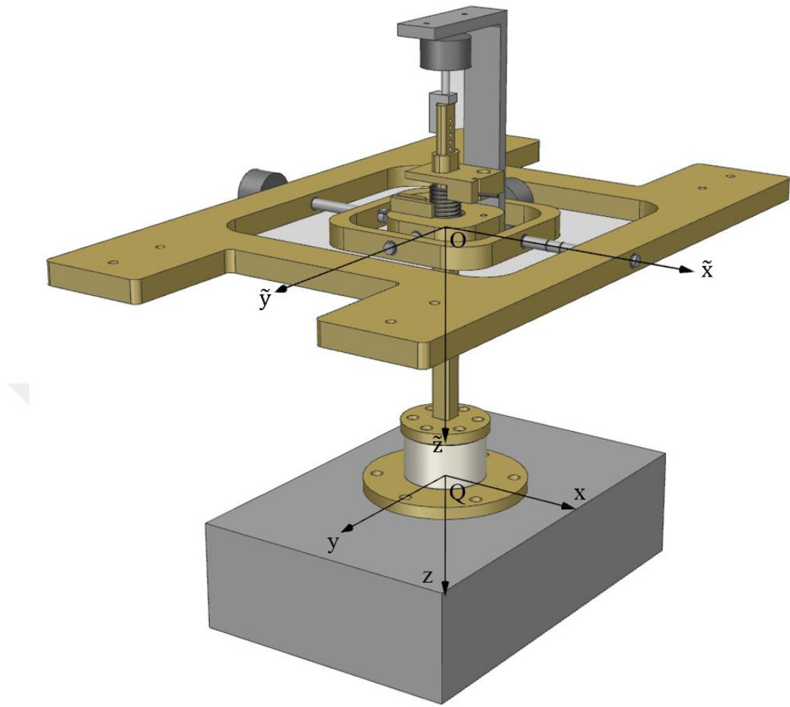
Figure 26. Computer model of configuration of the developed design is shown.
