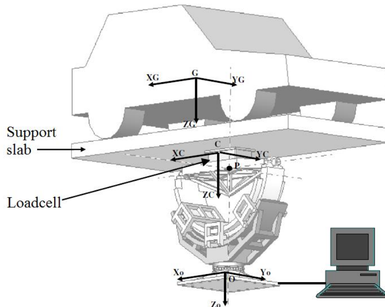
Figure 23. The actuator configuration rotates the specimen about point P , and forces and accelerations are measured. [35]
