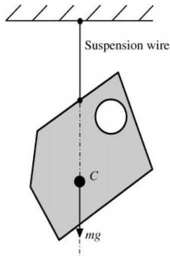
Figure 14. Configuration for hanging method. Wire direction points out the center of gravity location. [66]
