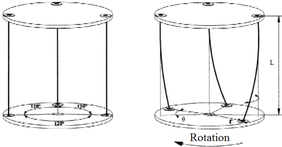
Figure 19. Test specimen is placed on the plate shown and initial angular displacement is given. [31]
