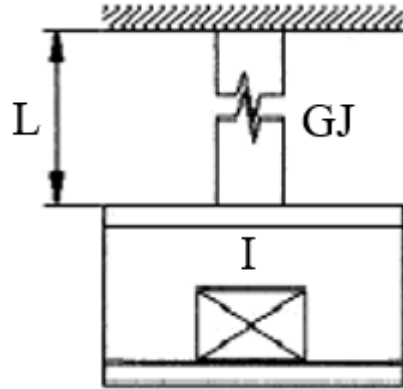
Figure 21. The test specimen is attached to the ceiling with a rod. Torsional stiffness of the rod is found by the formula k = GJ/L . [31]
