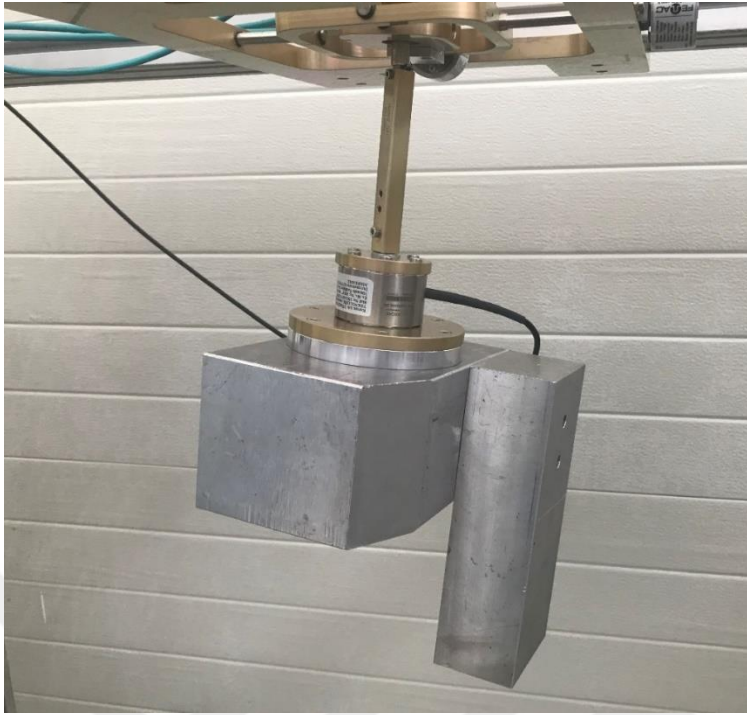
Figure 39. Mass properties of the shown dummy mass consists of two aluminum block are measured.
