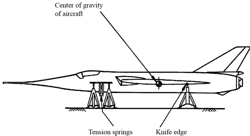
Figure 20. Tension springs acts as a restoring force and creates an oscillatory rotational motion about knife edge. [26]
