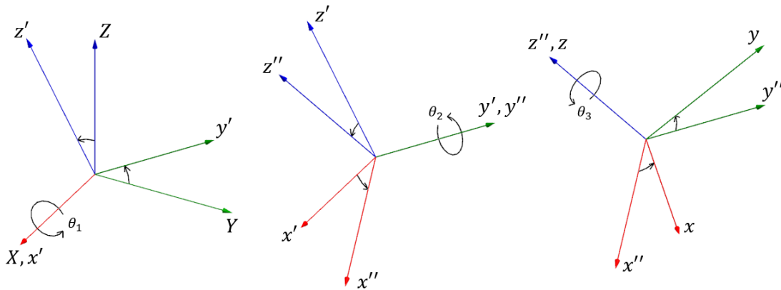
Figure C-1. Euler angles in 123 rotation sequence
