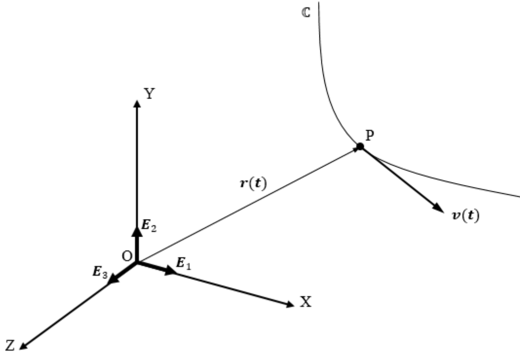
Figure 3. Particle P is moving along the shown path \mathbb{C} with velocity \mathbf{v}(t) . Its position is described by the position vector \mathbf{r}(t) at time t .
