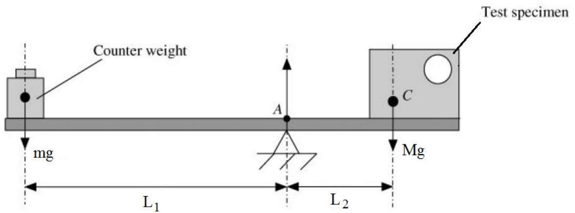
Figure 16. Moment balance about point A is used to find the distance between center of gravity position along vertical axis and point A, L_2 . [66]
