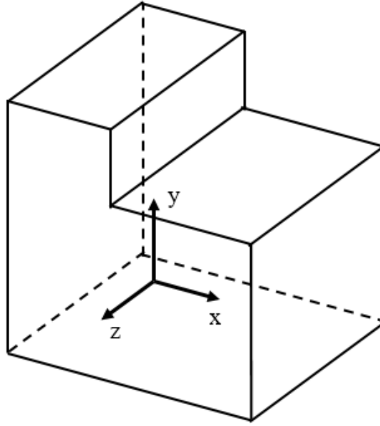
Figure 2. Solid body, whose symmetry plane is xy plane, is demonstrated.
