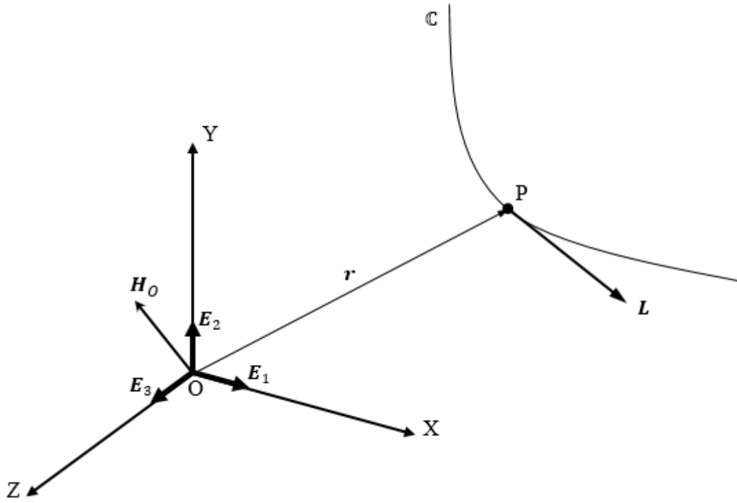
Figure 4. Representation of linear momentum L of particle P and resulted angular momentum H_o at point O.
