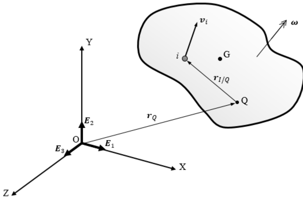
Figure 9. Kinetics of a rigid body is examined by using its particles' linear and angular momentums.
