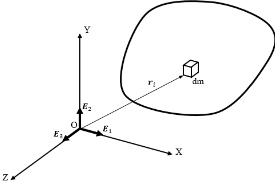
Figure 10. Differential element of mass dm relative to reference coordinate frame is shown.
