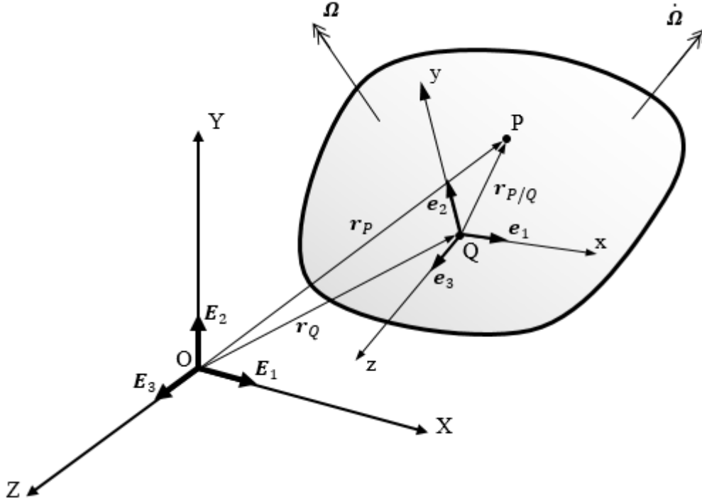
Figure 8. Local frame is located on a body which is in general motion. Kinematic of point P on the body is going to be analyzed.
