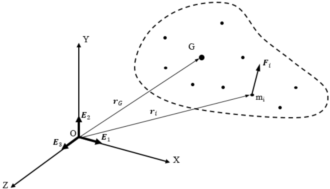
Figure 5. System of particles whose center of mass is located at G and force acting on one particle are demonstrated.
