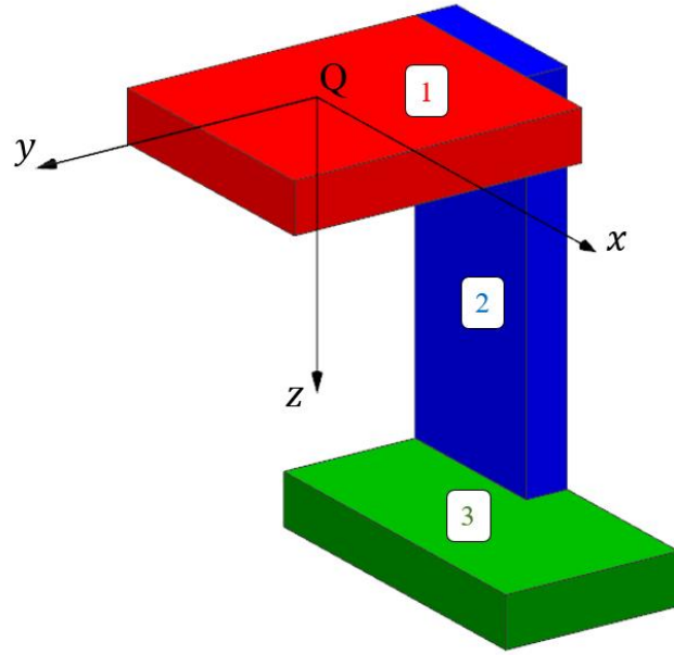
Figure 37. Arbitrary shape simulation model is divided into three segments for calculation of inertia values.
