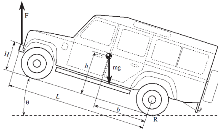
Figure 15. The specimen can rotate about point R. The distance, b , is calculated using moment balance about point R. [10]
