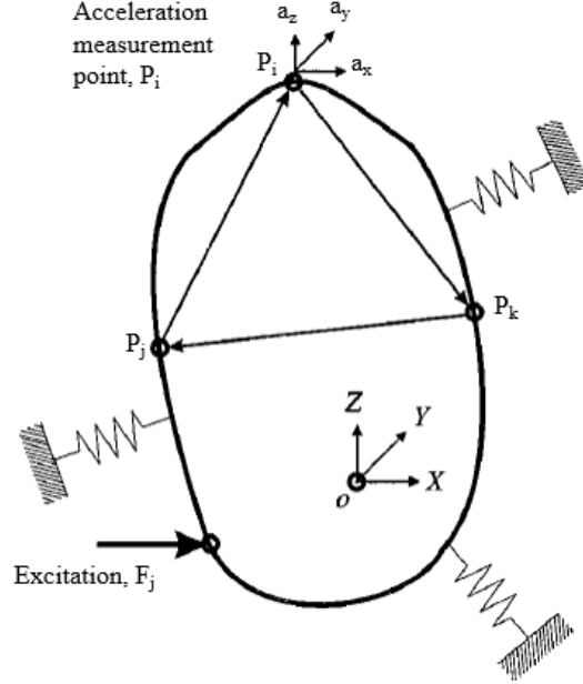
Figure 24. The specimen is placed on springs and makes a general motion with the excited force. [52]
