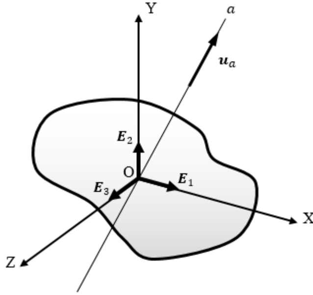
Figure 13. Representation of an arbitrary axis passing through origin of the reference frame.
