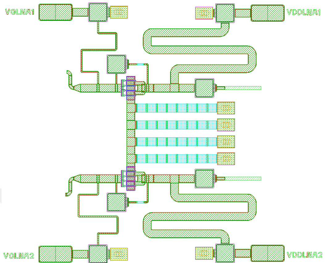
Figure 3.14: Differential LNA layout
