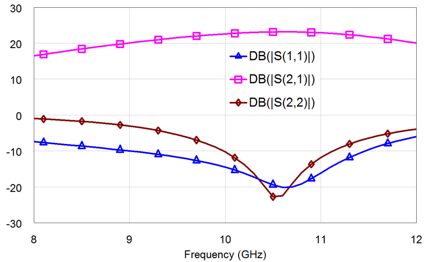
Figure 3.9: Small signal parameters of PA
