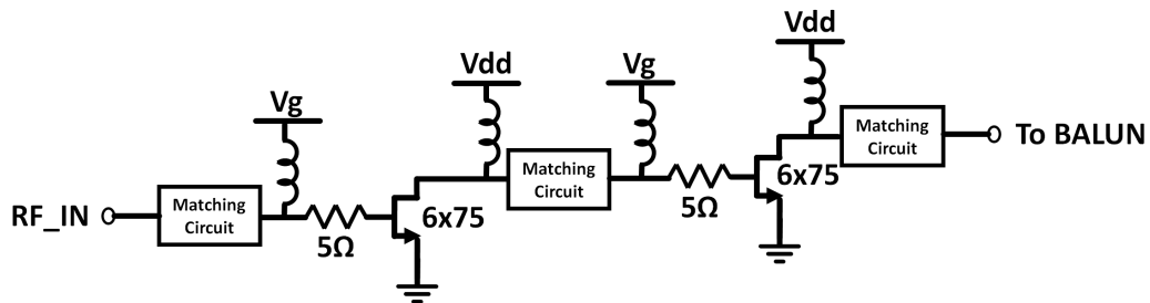
Figure 3.6: PA schematic view
