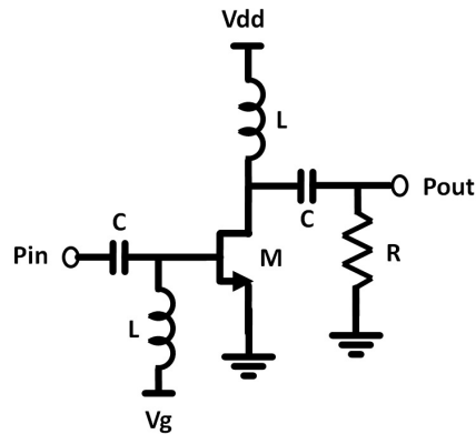
Figure 3.2: Class A PA schematic
