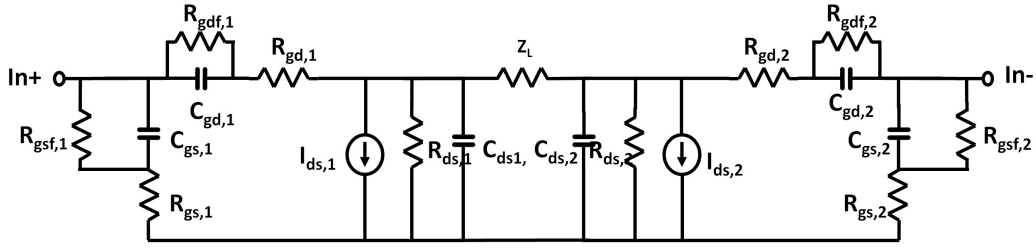
Figure 3.12: Small signal model for common mode analysis of differential LNA
