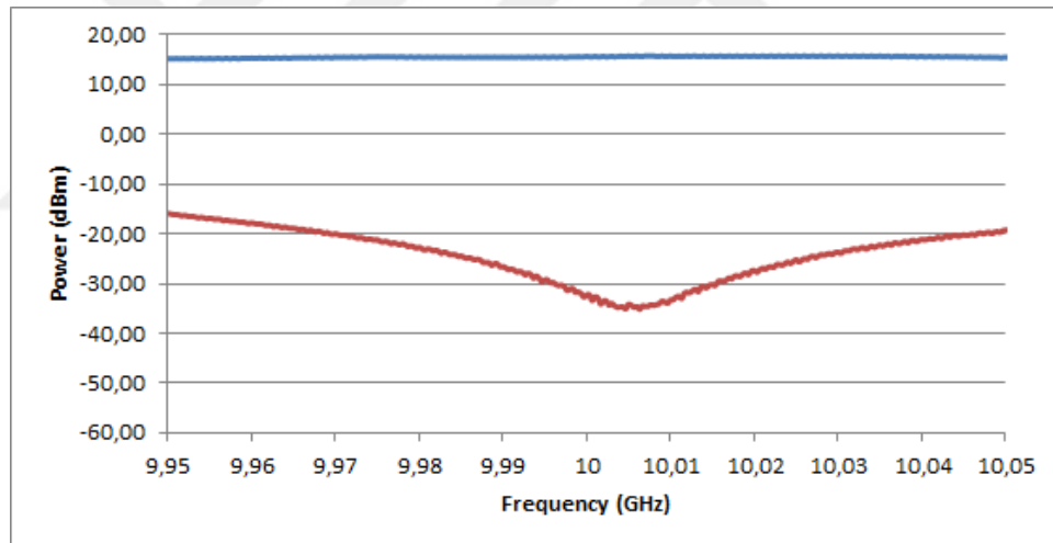
Figure 4.9: Transmitted (blue) and self-interference (red) power at 46-j29 \Omega load
