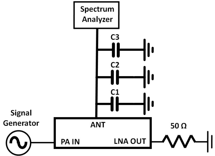
Figure 4.5: Test setup for measuring power output at antenna
