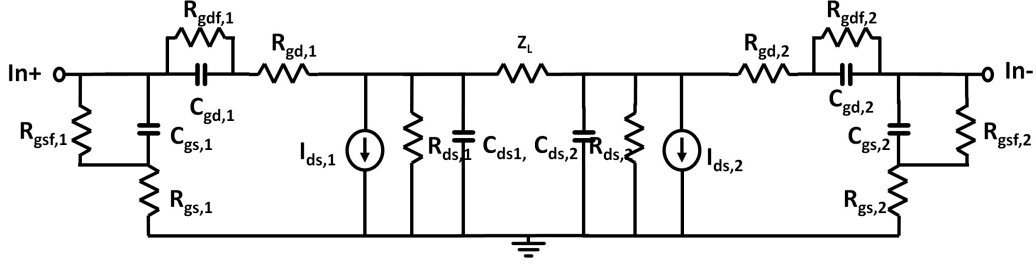
Figure 3.11: Small signal model for differential analysis of differential LNA
