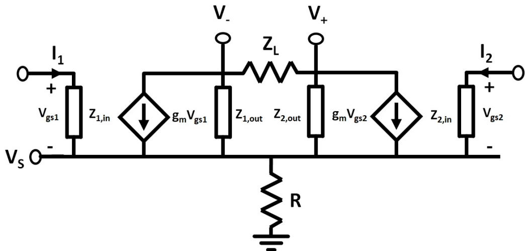
Figure 2.9: Small signal model for a differential amplifier
