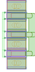
(a) ISV transistor layout
