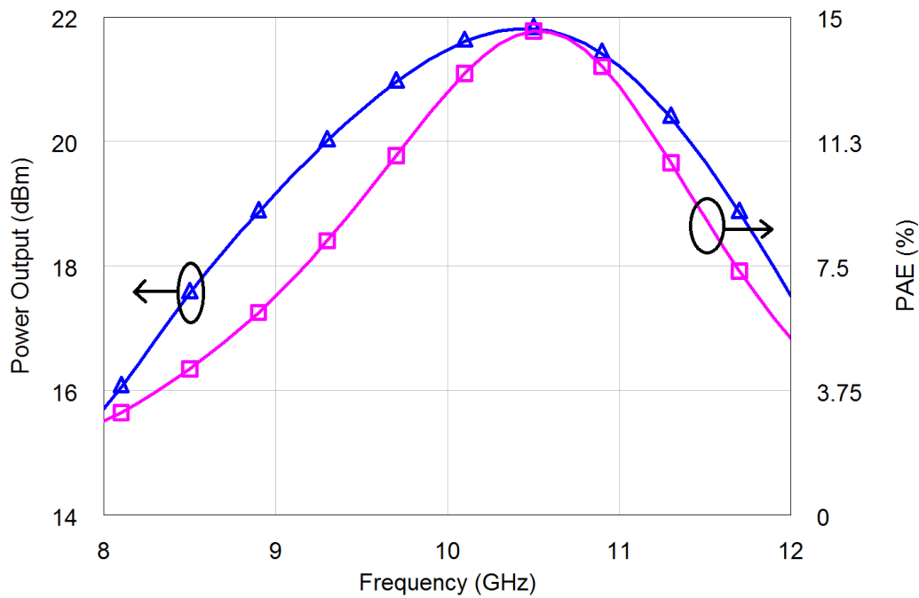
Figure 4.7: Power output and PAE of PA under 10V drain bias
