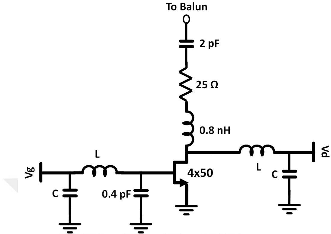
Figure 3.22: Balancing load schematic
