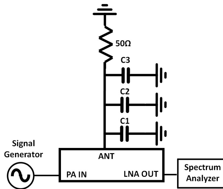
Figure 4.4: Test setup for measuring SIC
