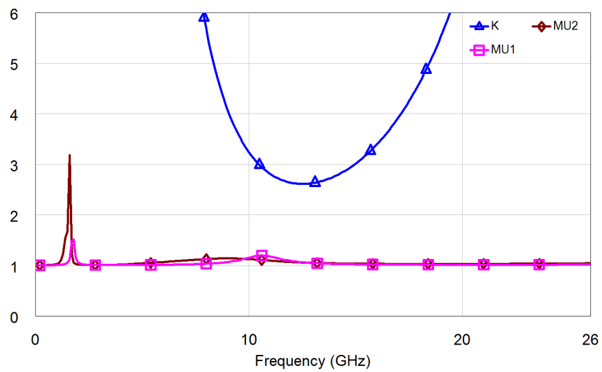
(b) Second stage stability results
