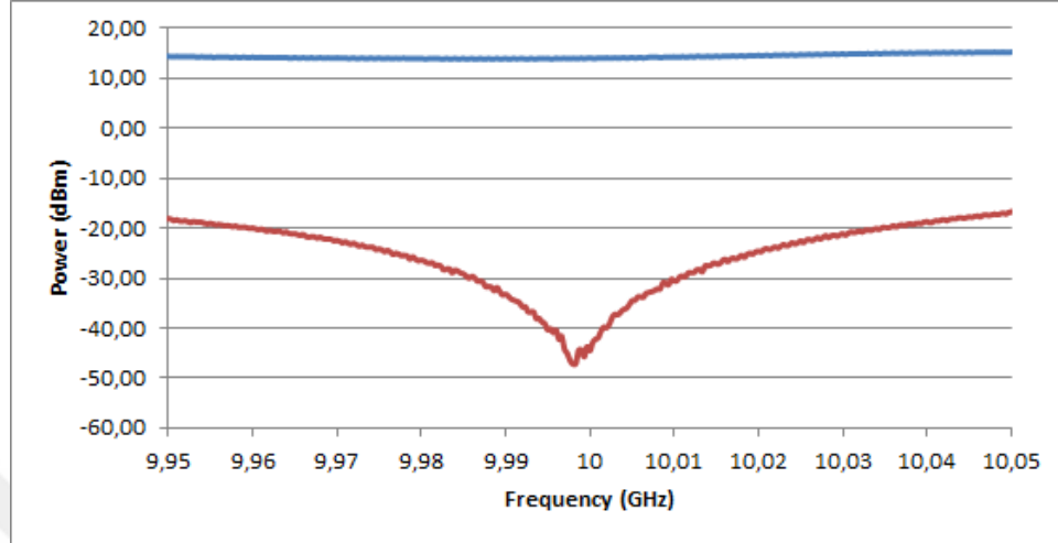
Figure 4.8: Transmitted (blue) and self-interference (red) power at 50 \Omega load
