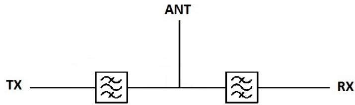
Figure 1.6: Diplexer connection in an FDD system
