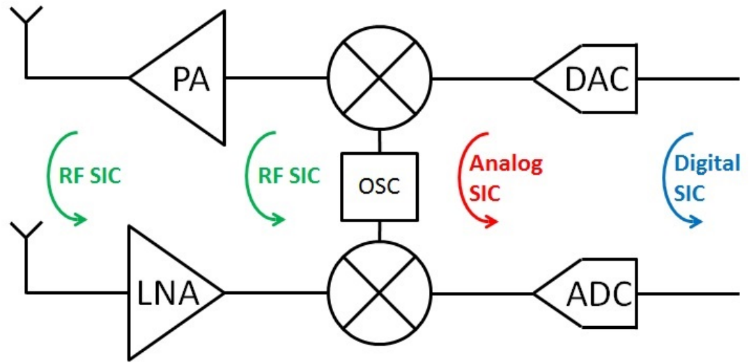
Figure 1.8: Self Interference Cancellation Paths
