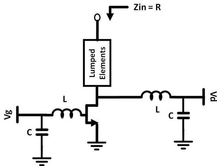
Figure 2.10: Simplified schematic of balancing load
