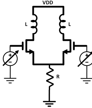
Figure 2.8: A simple differential amplifier
