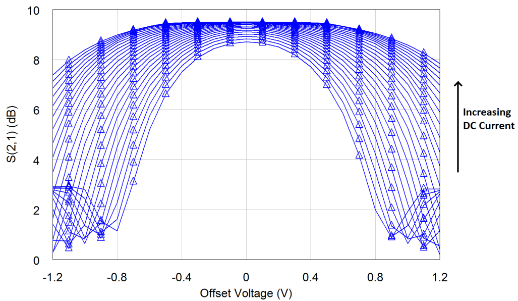
Figure 3.15: Differential amplifier gain with respect to offset voltage
