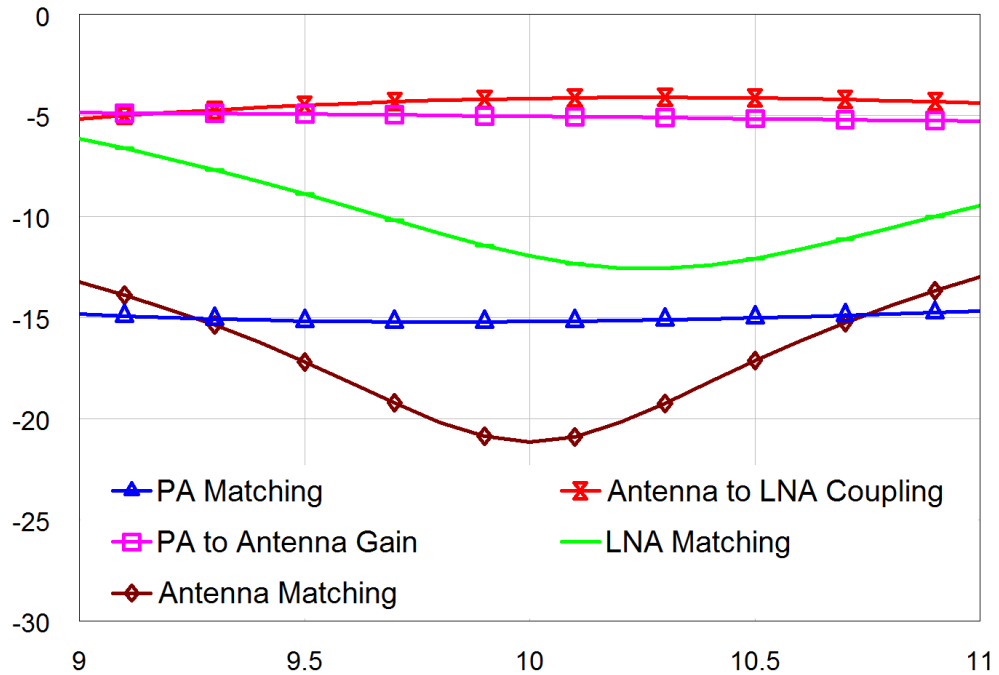
Figure 3.21: Balun S parameter results
