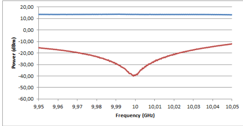
Figure 4.12: Transmitted (blue) and self-interference (red) power at 54.5+j20.8 \Omega load
