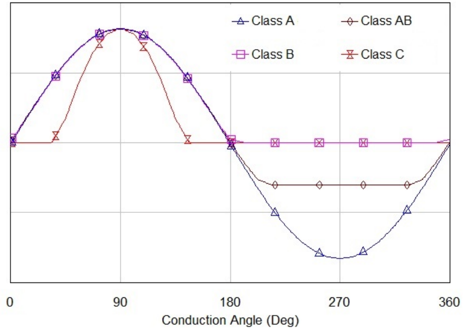
Figure 3.1: PA Classes at different conduction angles
