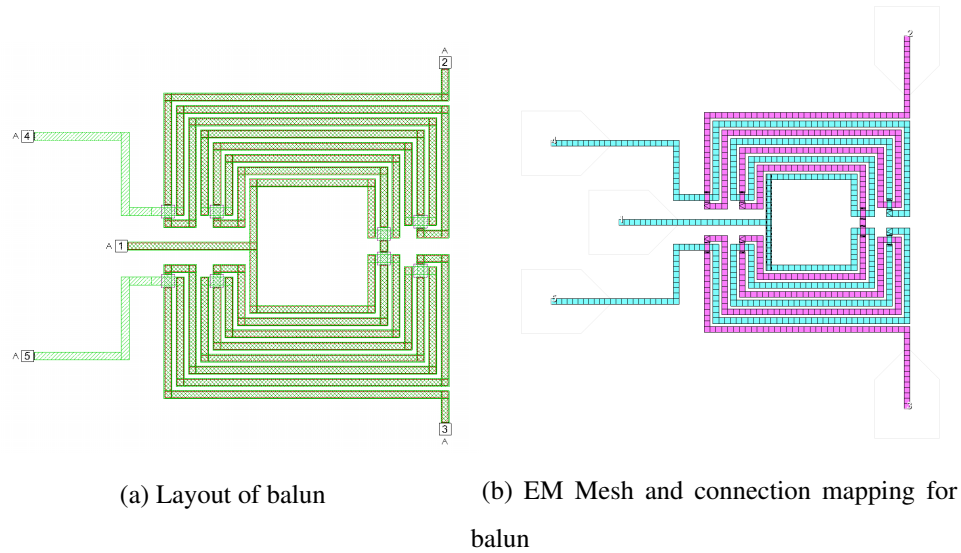
Figure 3.20: Balun layout and connection
