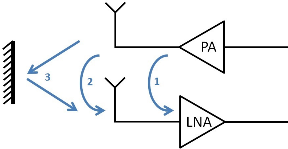
Figure 1.7: RF Self Interference paths
