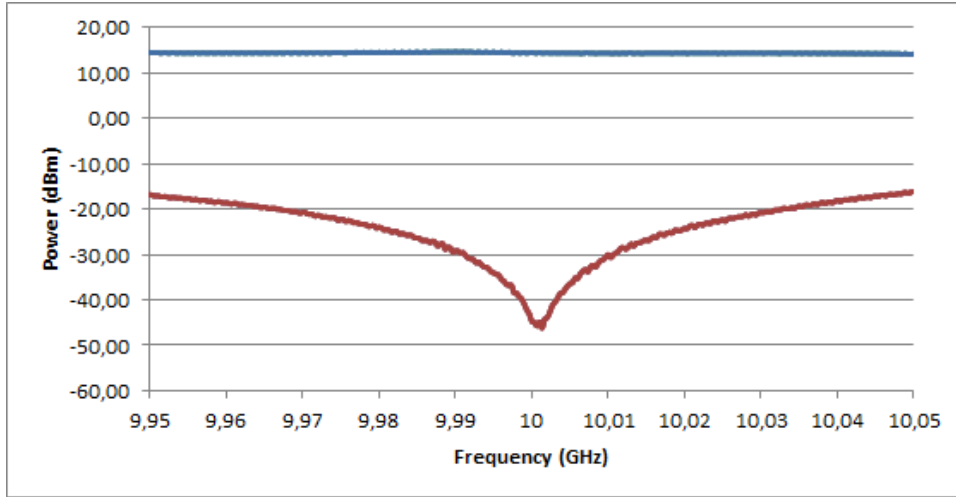
Figure 4.10: Transmitted (blue) and self-interference (red) power at 30.6-j10.5 \Omega load
