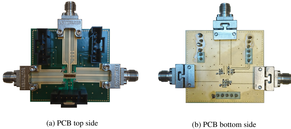
Figure 4.3: Photo of assembled pcb
