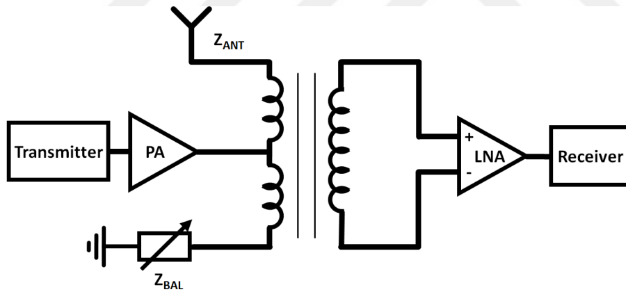
Figure 1.13: A simplified EBD system
