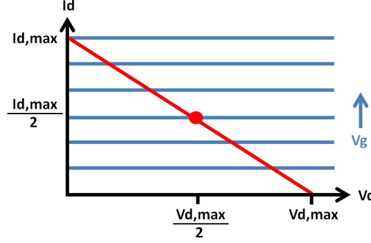
Figure 3.3: Linearized I-V characteristics
