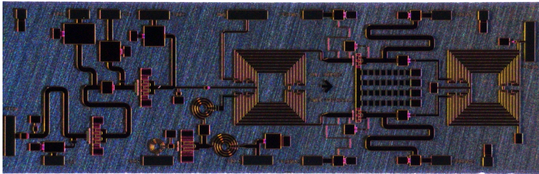
Figure 4.1: Die photo of the manufactured IC. Left side transmitter input, right side LNA output, middle side antenna output
