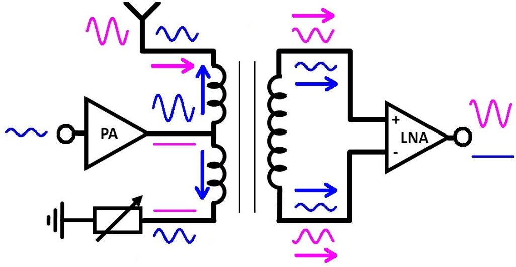
Figure 1.14: Transmitter and receiver signal flow in an EBD system. Blue lines show the transmitted signal, purple line shows received signal
