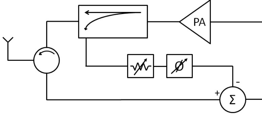
Figure 1.11: RF Feedforward cancellation schematic
