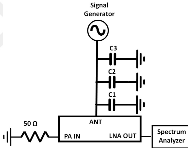
Figure 4.6: Test setup for measuring LNA gain
