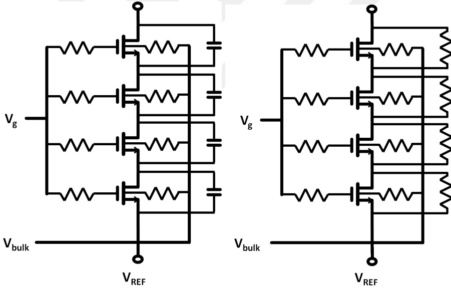
Figure 1.17: Tunable capacitor (left) and resistor (right) structures
