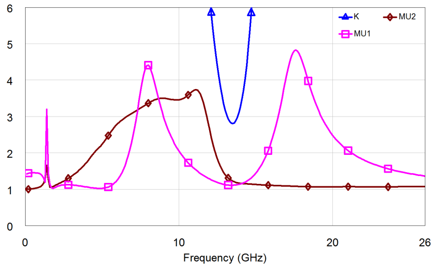
(a) First stage stability results
