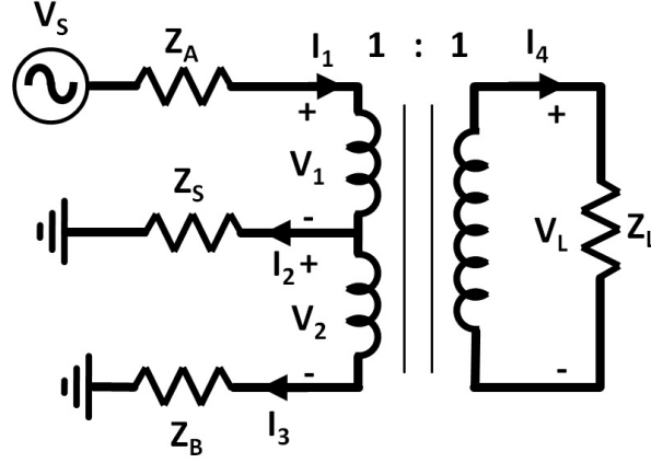
Figure 2.5: EBD analysis from antenna side
