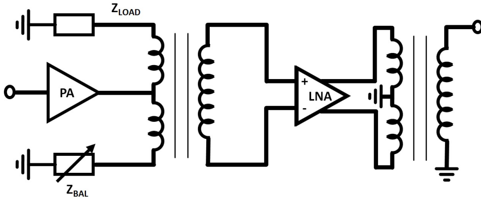
Figure 2.1: EBD system design
