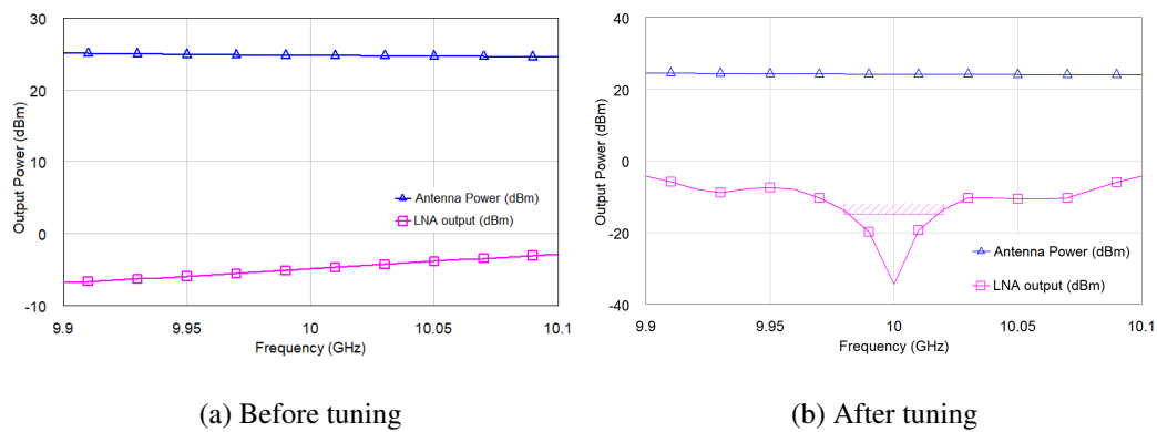
Figure 3.28: Antenna (blue) power and LNA output (purple) before and after tuning for \Gamma=(0.3, 45^\circ) load impedance
