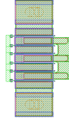
(b) OSV transistor layout
