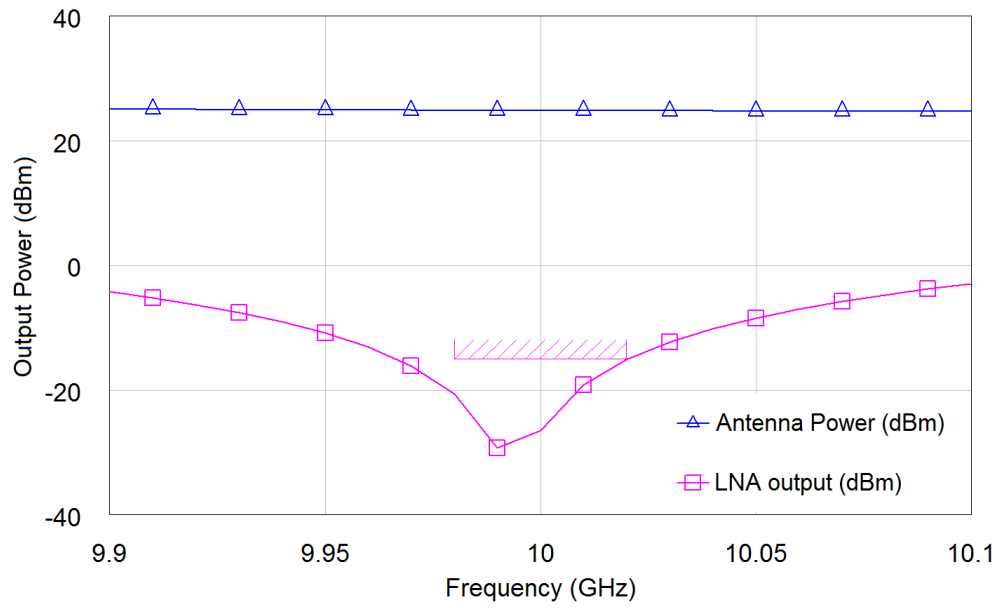
Figure 3.27: Antenna (blue) power and LNA output (purple) before and after tuning for 50\ \Omega load
