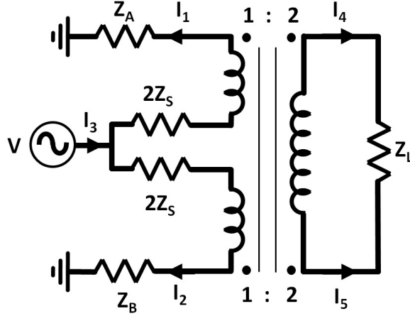
Figure 2.4: Analysis circuit for unbalanced case
