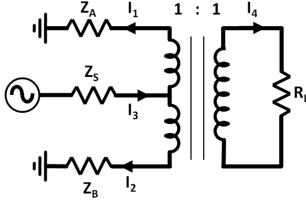
Figure 2.3: Port impedances in an ideal balun
