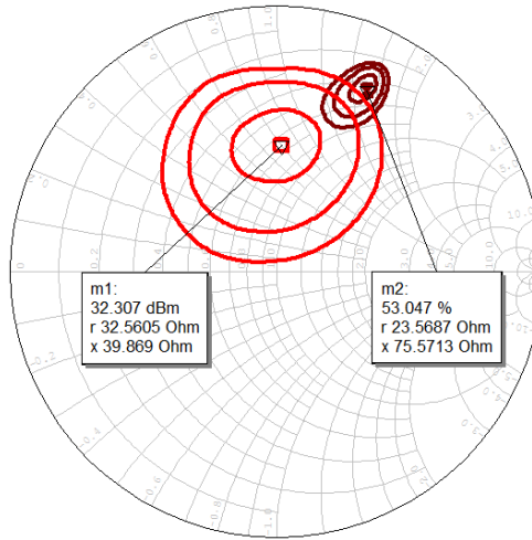
Figure 3.5: Load pull results for a 6 \times 75 \mu\text{m} transistor
