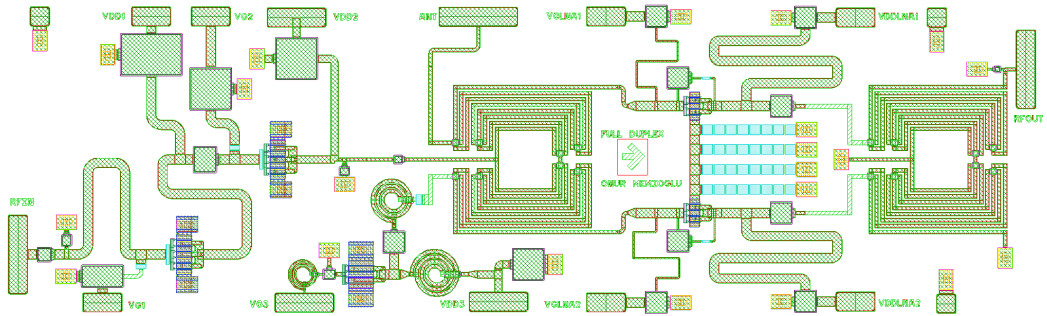
Figure 3.26: Fully integrated MMIC layout
