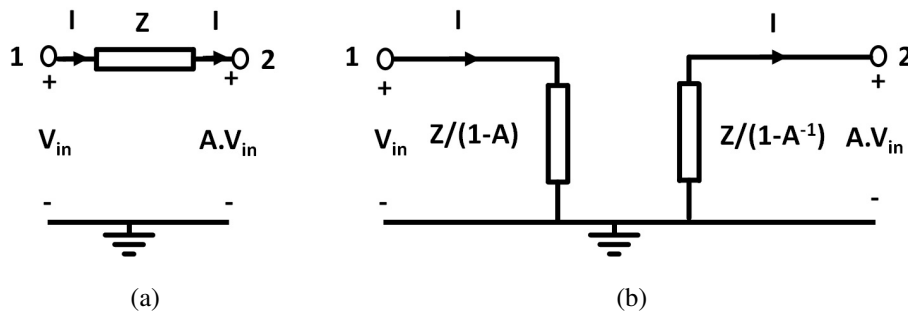
Figure 2.7: Miller theorem equivalent circuit[37]
