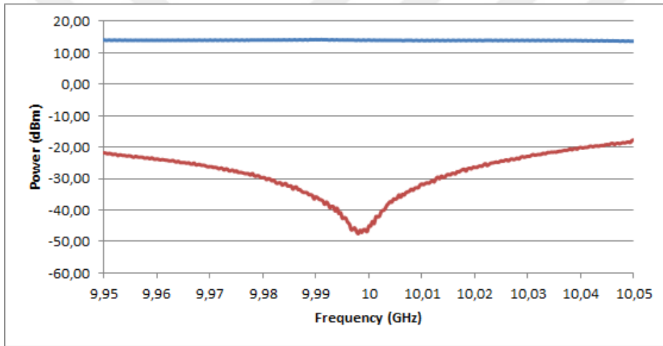
Figure 4.11: Transmitted (blue) and self-interference (red) power at 34.1+j9.4 \Omega load
