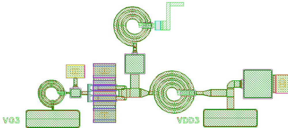
Figure 3.23: Balancing load layout
