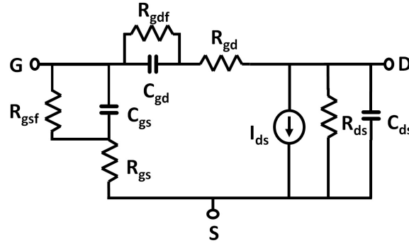
Figure 2.6: A small signal linearized model for HEMT devices [36]
