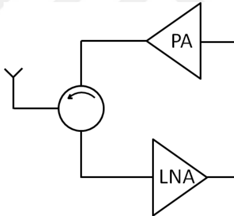
Figure 1.10: RF Circulator usage in IBFD system
