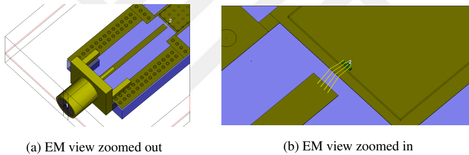
Figure 4.2: 3D EM setup for the PCB and MMIC interface
