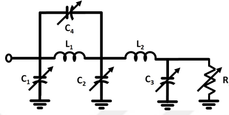
Figure 1.16: Modified \pi matching section
