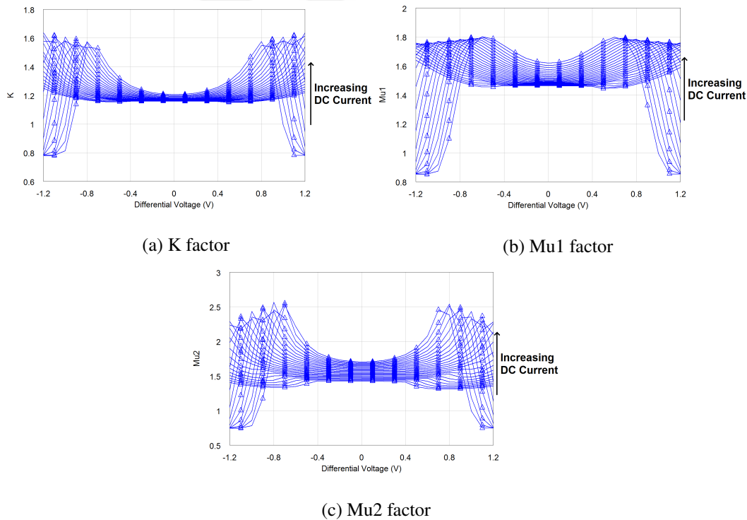
Figure 3.16: Differential mode LNA stability at single frequency
