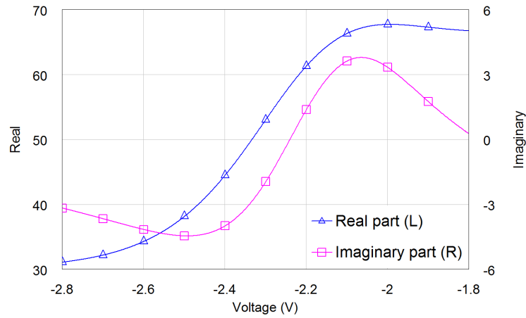
Figure 3.24: Balancing load impedance with respect to gate voltage
