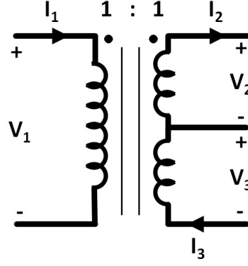
Figure 2.2: A hybrid transformer with a center tap which is a balun
