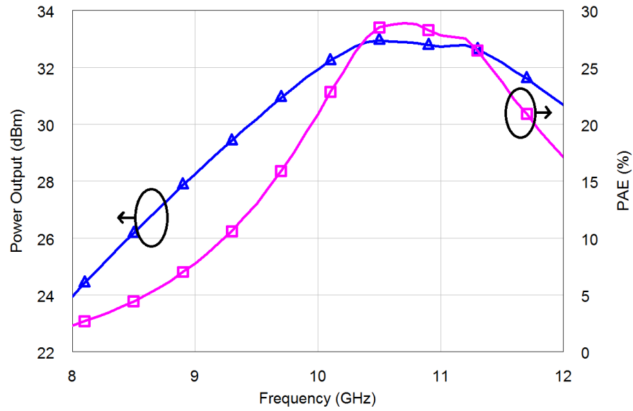
Figure 3.8: Saturated power output and PAE of PA
