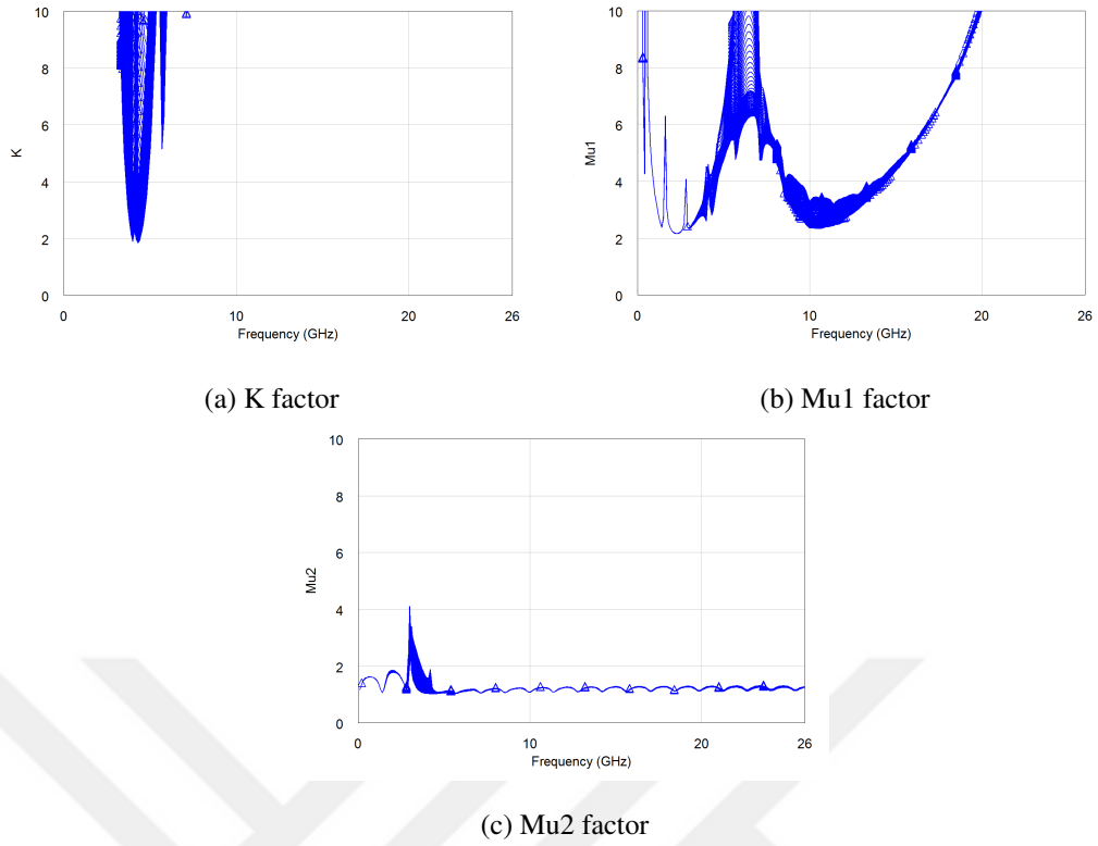
Figure 3.25: Balancing load stability with respect frequency at different bias voltages
