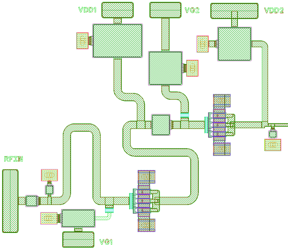
Figure 3.7: Layout of PA
