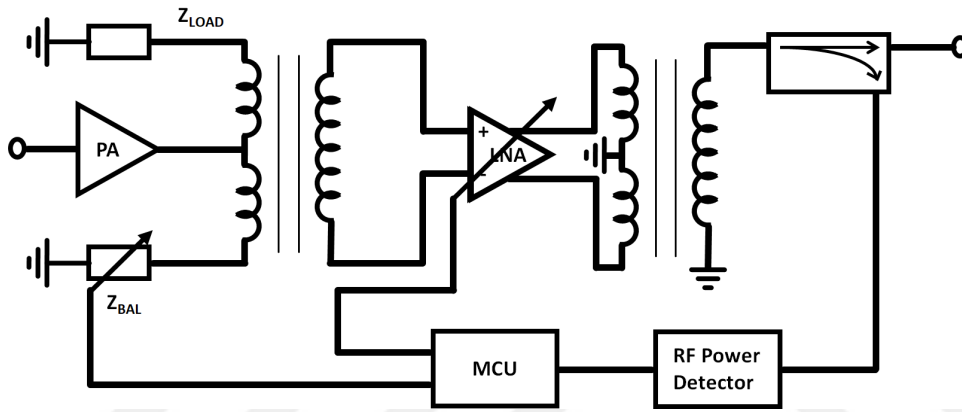
Figure 5.1: Proposed system diagram for self adapting loop
