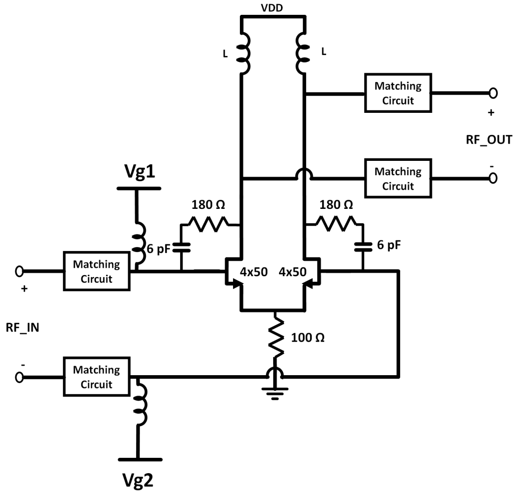
Figure 3.13: LNA schematic view
