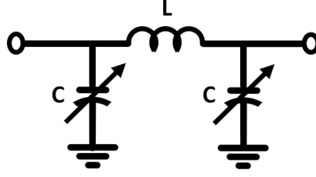
Figure 1.15: Low pass \pi matching section
