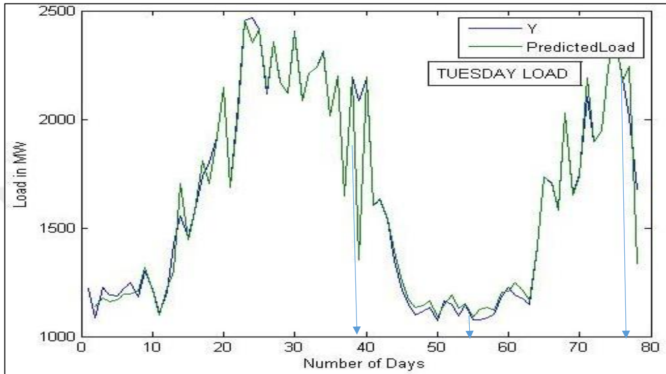
Figure 4.12: Comparison between actual and forecasted load for Tuesday
