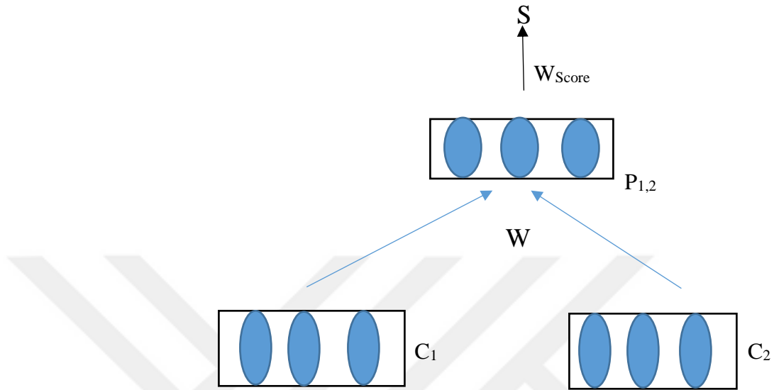
Figure 2.6: Simple recursive neural network architecture [17]
