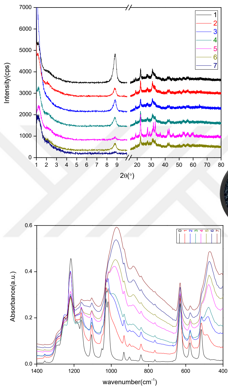
Figure 3.3.4. (Top) XRD patterns of different phosphoric acid mole ratios at 12 mole ratios of AgOTf in \text{C}_{12}\text{E}_{10} and 5 ml water with various \text{H}_3\text{PO}_4 amount. (Bottom) ATR-IR spectra of the same samples and POM image of 12:36 \text{Ag}^+:\text{H}_3\text{PO}_4 mole ratios. The mole ratios of \text{C}_{12}\text{EO}_{10}:\text{AgOTf}:\text{H}_3\text{PO}_4 are 1:12:0 (0), 1:12:4 (1), 1:12:8 (2), 1:12:12 (3), 1:12:16 (4), 1:12:20 (5), 1:12:24 (6), 1:12:36 (7).
