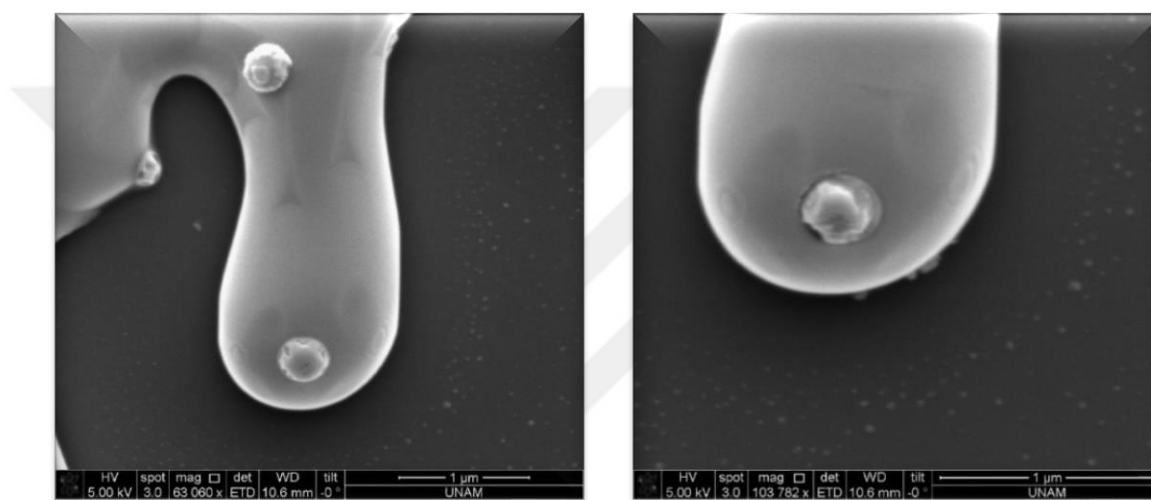
Figure 3.1.2.8. The SEM images of 1:16:5.33 C_{12}E_{10} :Ag:PO 4 mole ratio of thin film on silicon by focusing sample.
