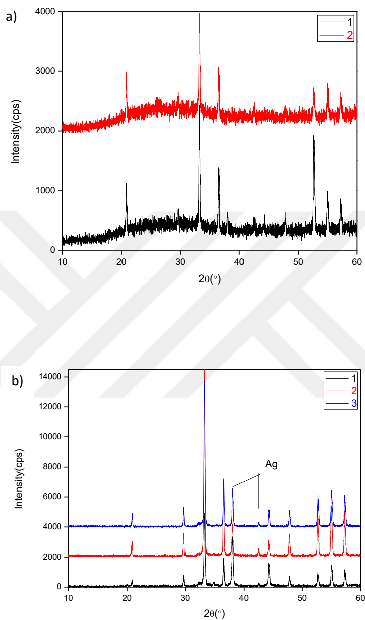
Figure 3.1.2.6. The XRD patterns of C_{12}E_{10}:Ag:PO_4 mole ratios (a) 1:12:4 (1) and 1:9:3 (2) thin films on glass slides, calcined at 300^\circ C and (b) 1:12:4 powder sample with different calcination steps, spin coating films (1), aged film with drop cast (2) and preheated oven before calcination process (3).
