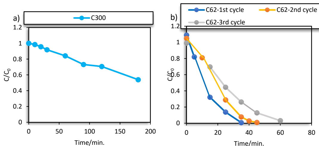
Figure 3.5.2. The graph of C/C_0 vs time for ppt in ethanol, the sample is calcined under vacuum without washing at a) 300°C and b) 150°C.
