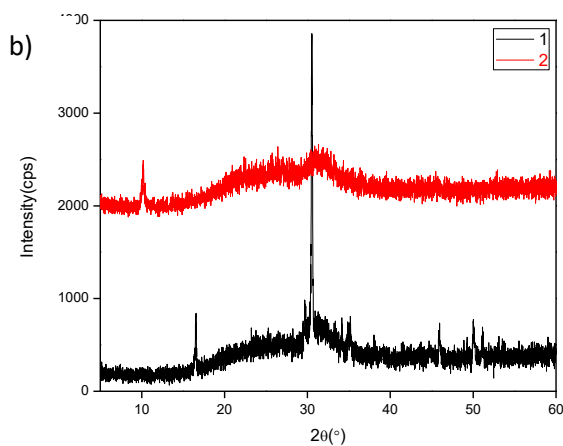
Figure 3.2.1. The XRD Patterns of 12:4 mole ratio of SNPA fresh films a) small angle and b) high angle with (1) and without (2) \text{HNO}_3 in water.
