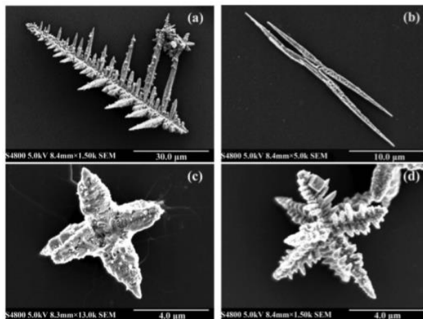
Figure 1.2.2.1. SEM images of Jin-Ku synthesis silver phosphate crystals. [23] 5
