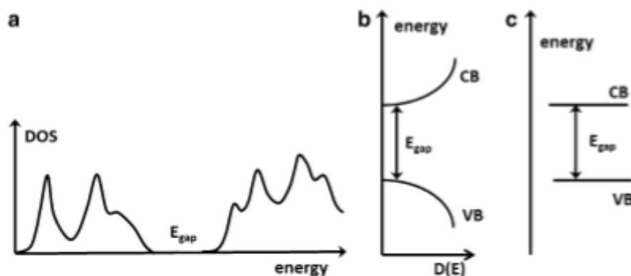
Figure 1.1.2. (a) Density of state (DOS) curve for a typical semiconductor; (b) parabolic approximation near band edges; (c) simplified band gap. [3] 2
