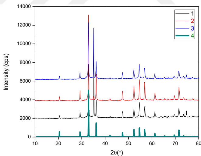
Figure 3.4.5. XRD patterns of Co (1), Mn (2), Ni (3) 90 mole ratios after cation exchange and with \text{Ag}_3\text{PO}_4 PDF card (4).
