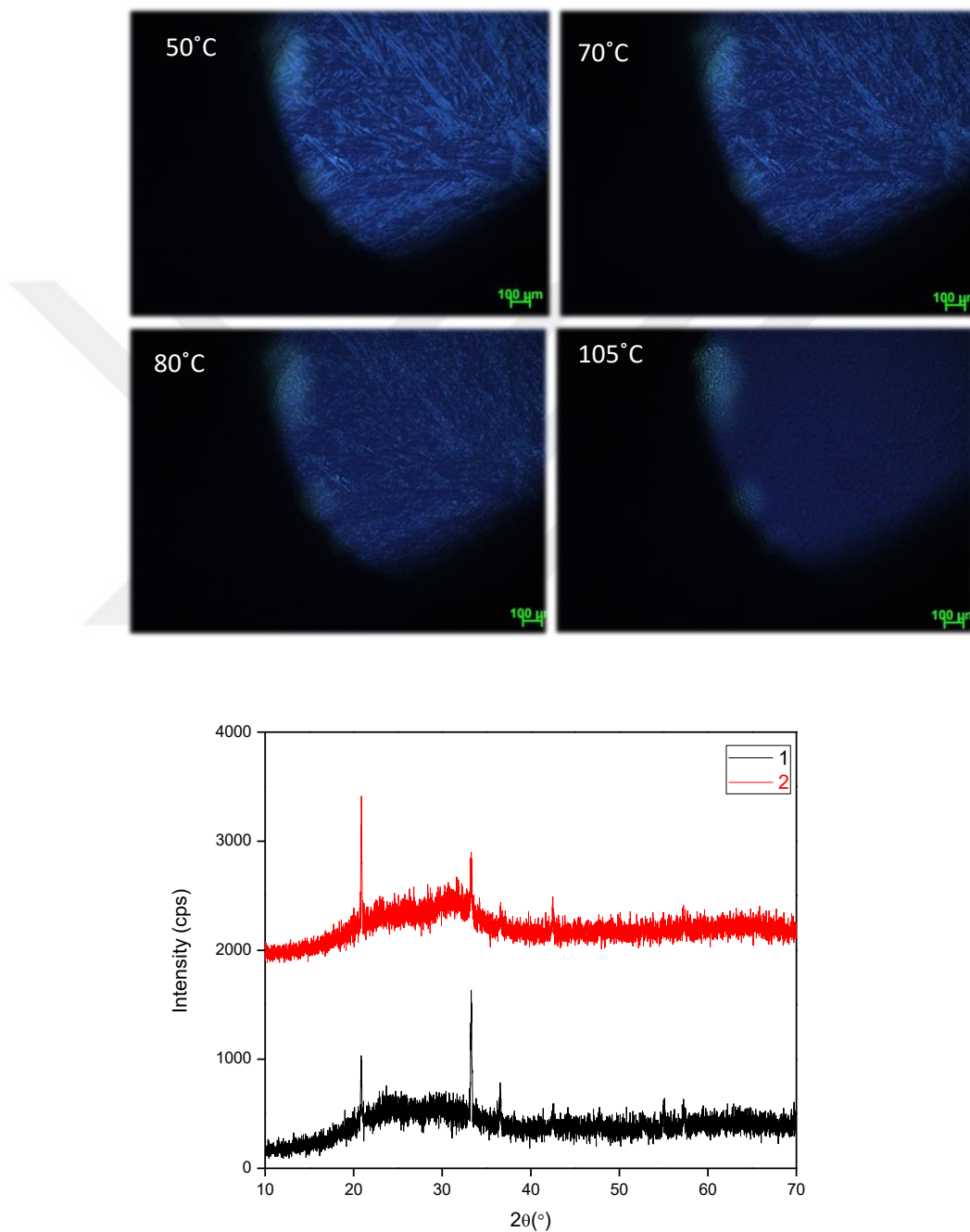
Figure 3.1.3.8. The POM images of 6:2 film at indicated temperatures and XRD patterns at 50(2) and 80°C (1).
