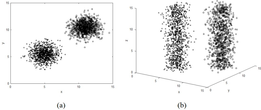
Figure 7.1: An example for a redundant feature
