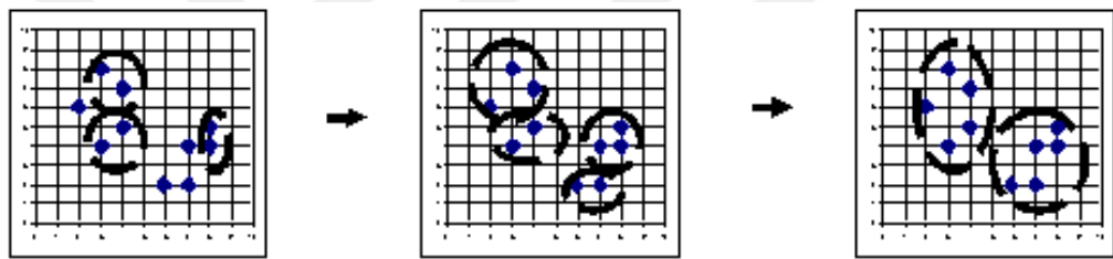
Figure 6-4. Agglomerative clustering example
