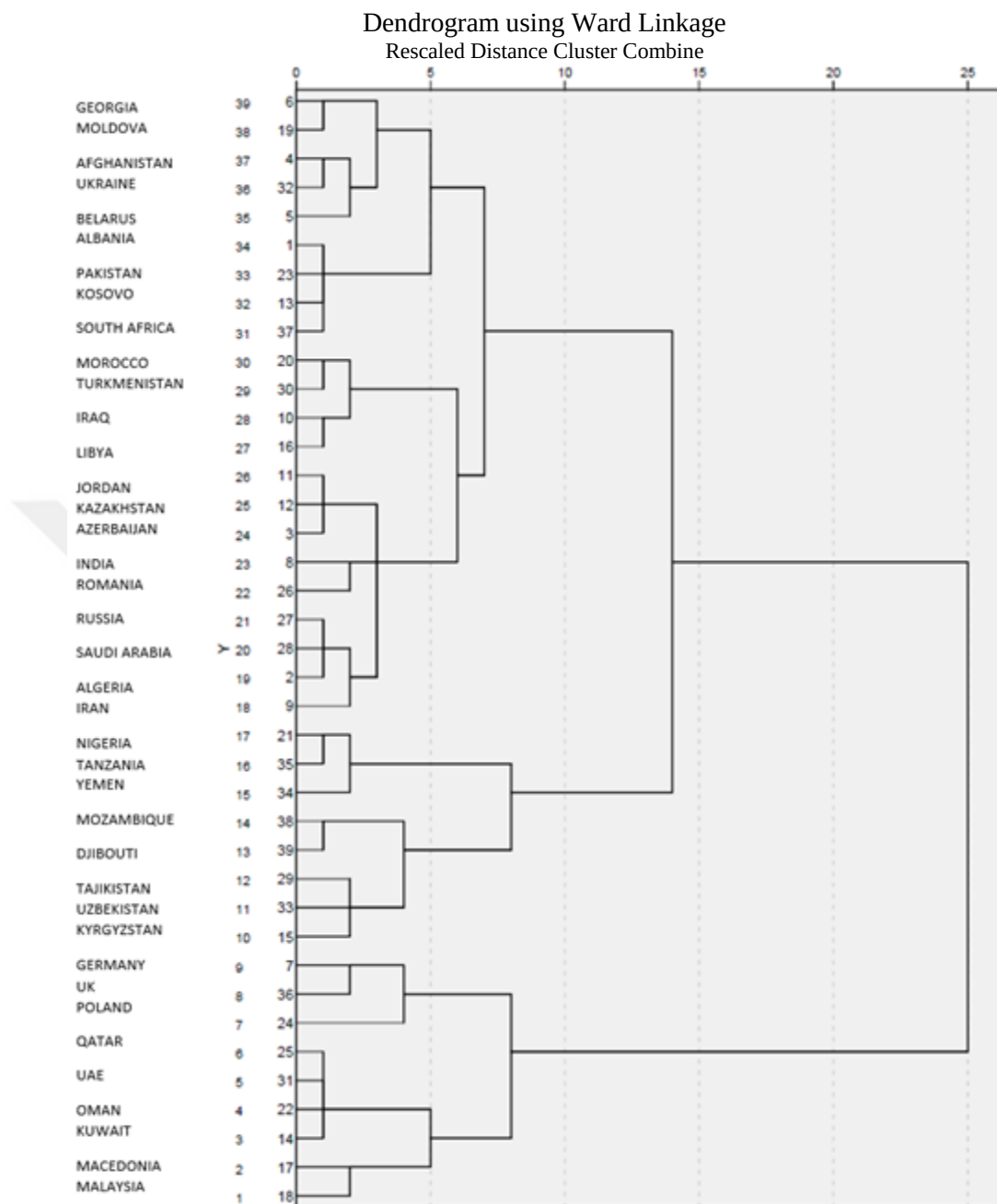
Figure 7-1. Dendrogram (taken from SPSS)
