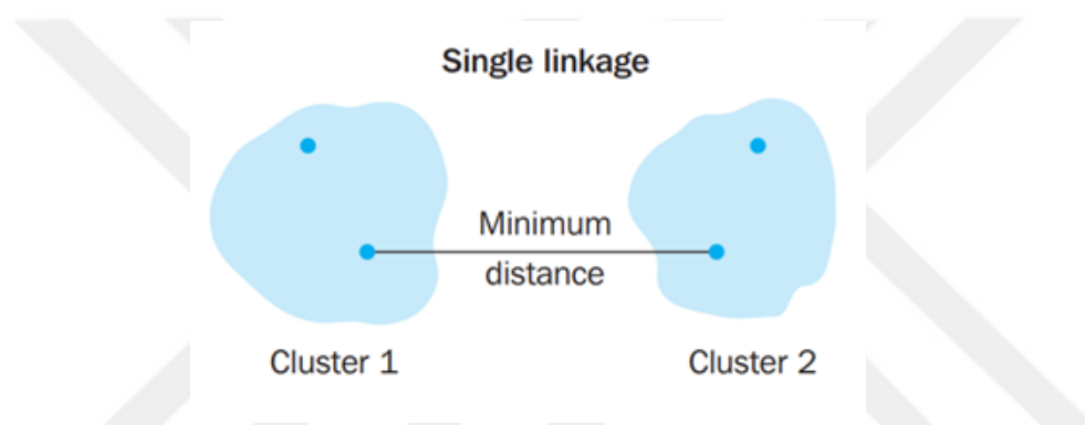
Figure 6-5. Single linkage method (Malhotra and Birks, 2006)
