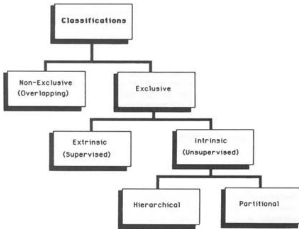
Figure 6-1. Tree of grouping types (Jain and Dubes, 1988)
