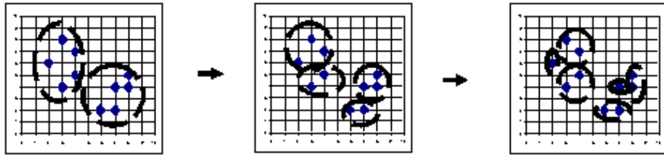
Figure 6-8. Divisive clustering example
