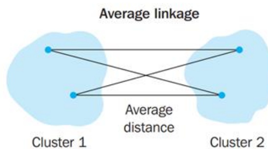
Figure 6-7. Average linkage method (Malhotra and Birks, 2006)
