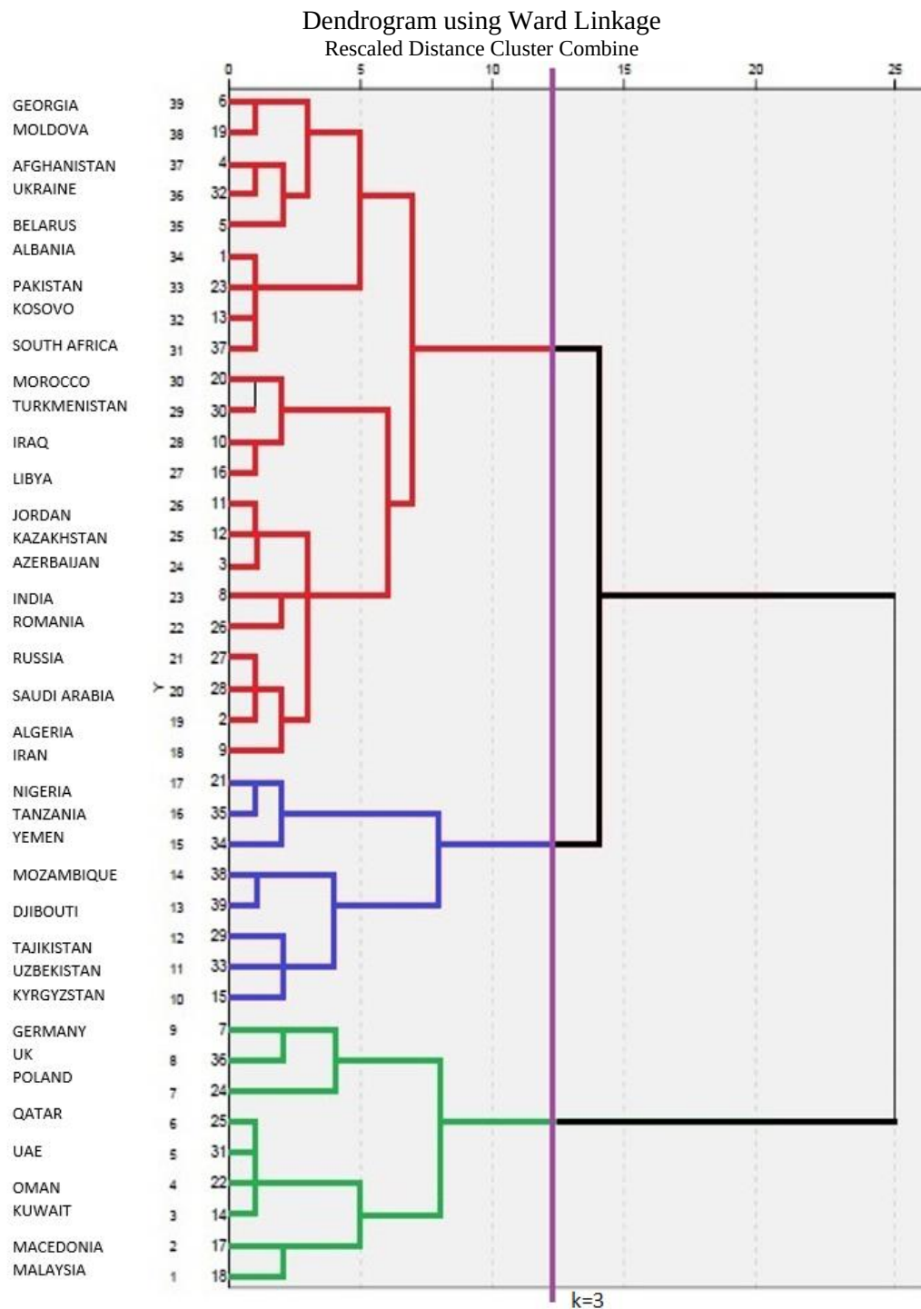
Figure 8-1. Dendrogram (with coloured representations of clusters)
