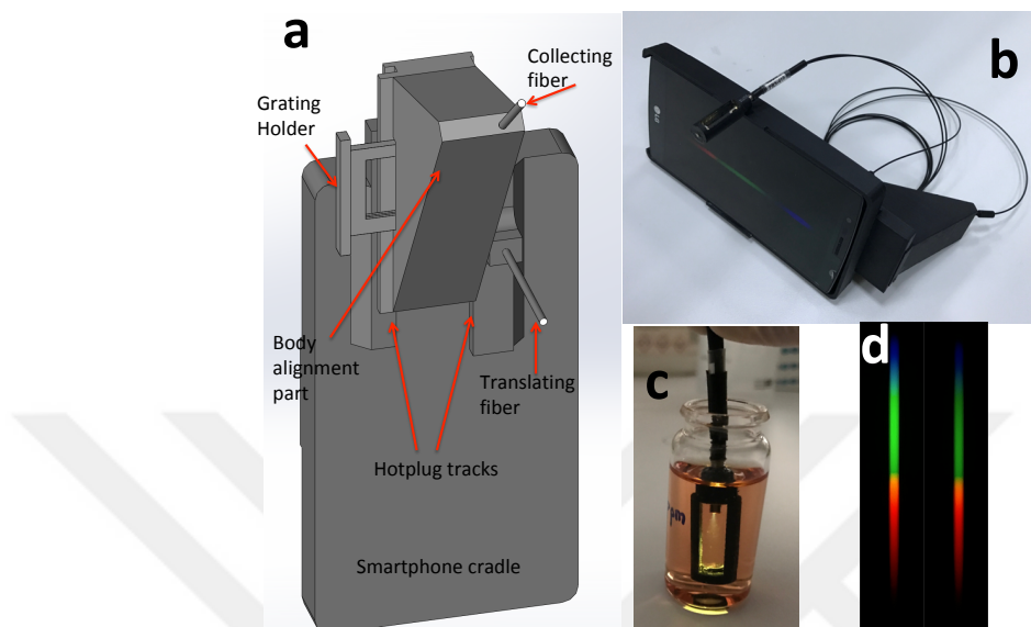
Figure 4.1 : (a) 3D printed components of smartphone based spectrometer, (b) completed form of the smartphone spectrometer with a plastic immersion probe, (c) the probe immersed into an analyte solution, (d) Representative spectral images from smartphone spectrometer.
