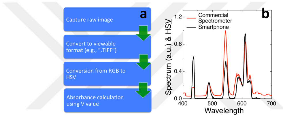
Figure 4.2 : (a) Image processing steps for the conversion of raw image into absorbance data, (b) The output spectra from commercial and smartphone spectrometers for calibration process.
