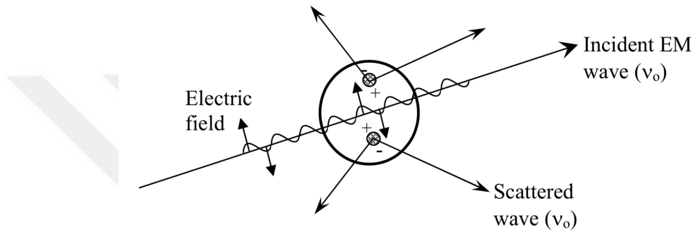
Figure 2.6 : Induced dipole moment and light scattering by an EM wave [83].
