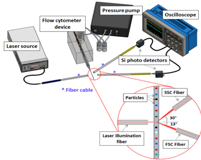
Figure 3.4 : Schematic illustration of the setup used to test the glass micropipette based flow cytometry device
