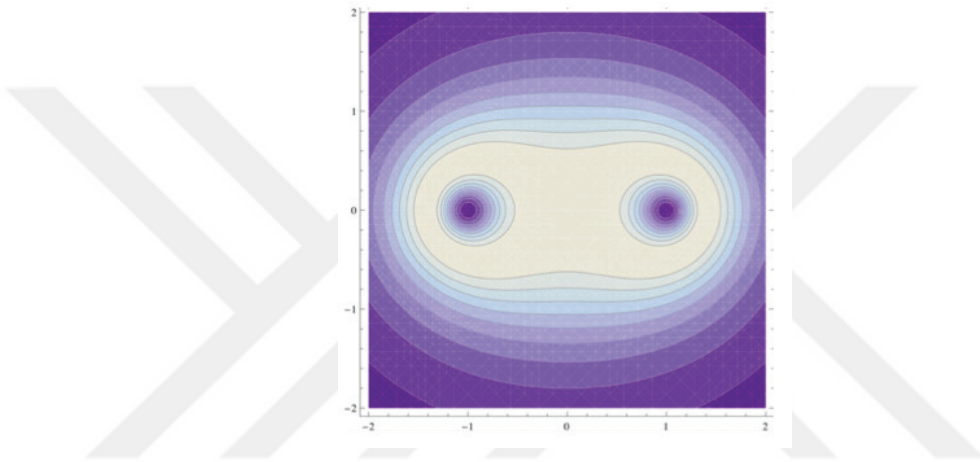
Figure 7.10. n - tangle for Cassini Qubit Contour Plot
