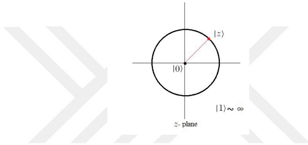
Figure 5.2. Coherent states plane
