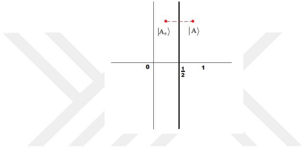
Figure 5.13. Symmetric qubit states
