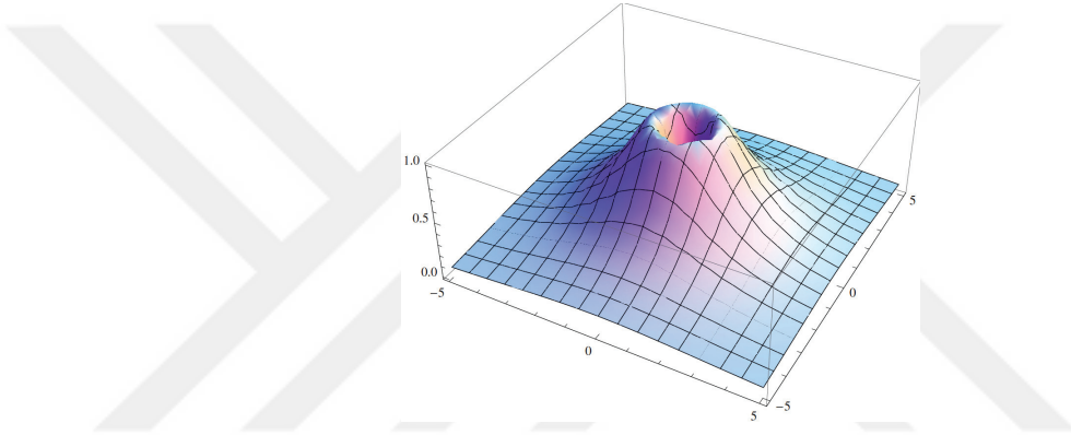
Figure 6.2. 3-tangle Coherent State 3D
