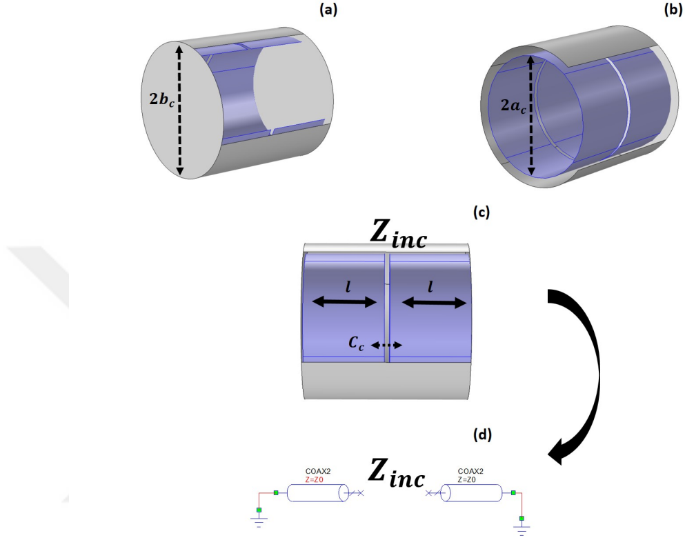
Figure 2.2: The re-entrant cavity resonator shown in three perspective angles for better visualization. All of the walls of the cavity resonator are supposed to be perfect conductors and the inner conductor is bisected in the middle. It should be noticed that Z_{inc} corresponds to the resultant input impedance due to the both ends of bisection.
