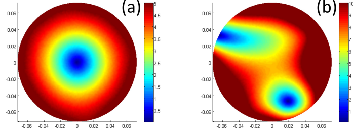
Figure 5.7: (a): E_z magnitude for normal drive, (b) E_z magnitude for modified drive. Both of the images belong to the homogeneous phantom.
