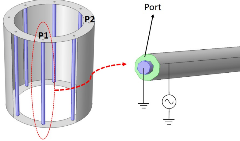
Figure 2.8: The coil for 3T and the driving port of the coil. The lumped port corresponds to the dielectric region between the inner and outer conductors of the line element.
