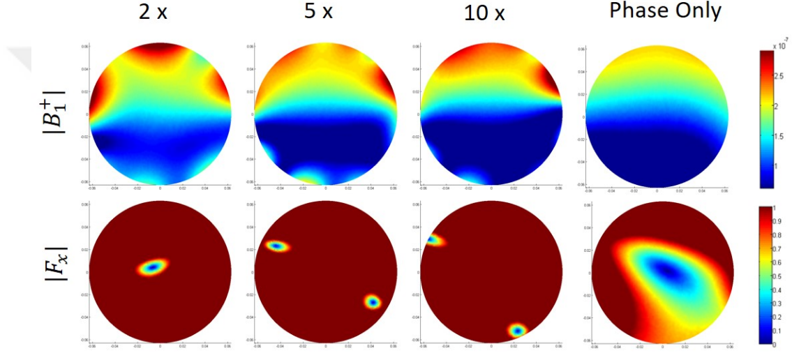
Figure 5.5: The B_1^+ magnitude (Tesla) and F_x magnitude distributions for the 2x, 5x, 10x cases as well as for the phase-only optimization methods.
