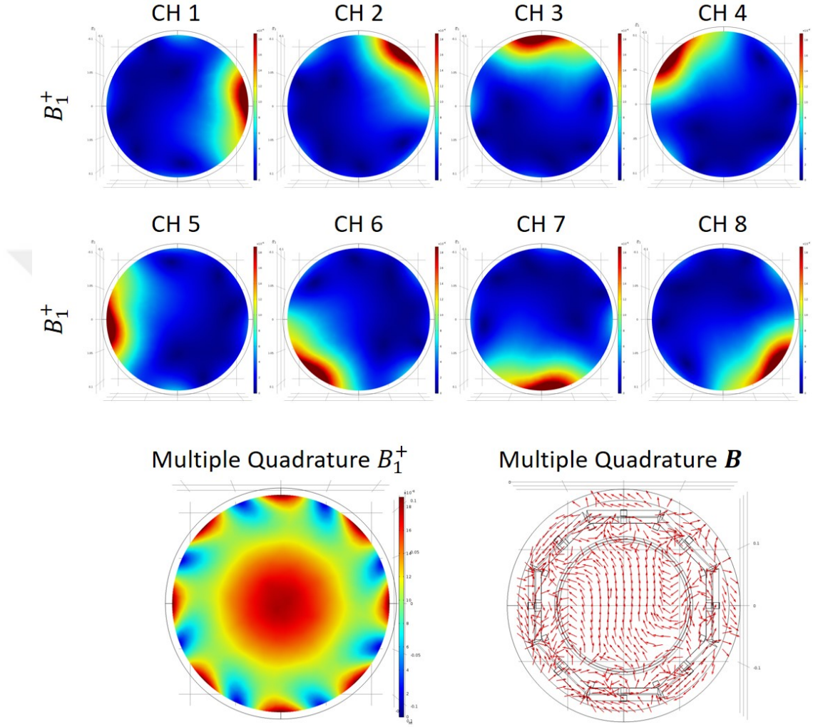
Figure 3.9: B_1^+ distributions for the one-channel only drive cases are given on the top, when each of channel is individually driven. Bottom two figures demonstrate the B_1^+ and \mathbf{B} field distributions for the multiple quadrature excitation.
