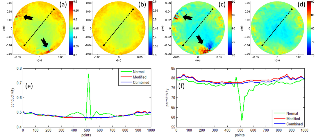
Figure 5.6: (a), (b): Modified and Combined conductivity reconstructions (in S/m), (c), (d): Modified and combined relative permittivity reconstructions. (e), (f): Profile plot of conductivity and relative permittivity reconstructions along the dashed lines on (a),(b),(c),(d) for normal drive, modified drive and combined cases.
