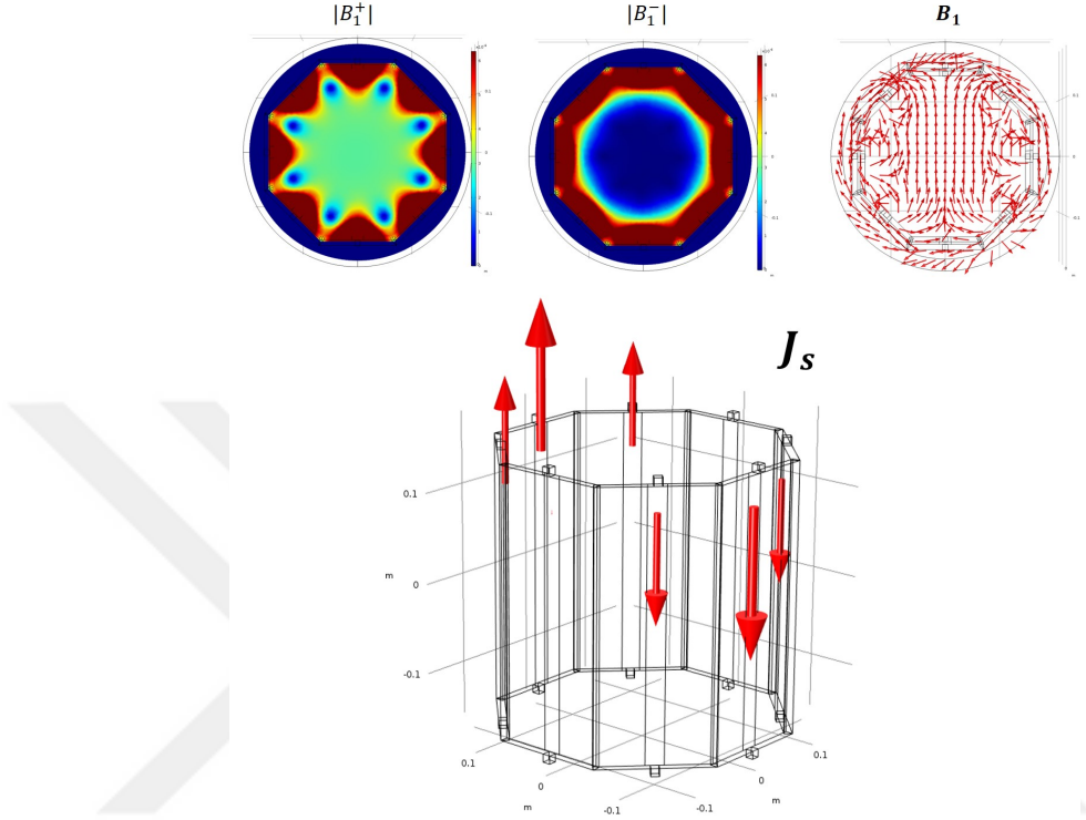
Figure 3.5: (a): The \mathbf{B}_1 fields of the MTL TEM coil and the surface current densities on the microstrips in quadrature excitation.
