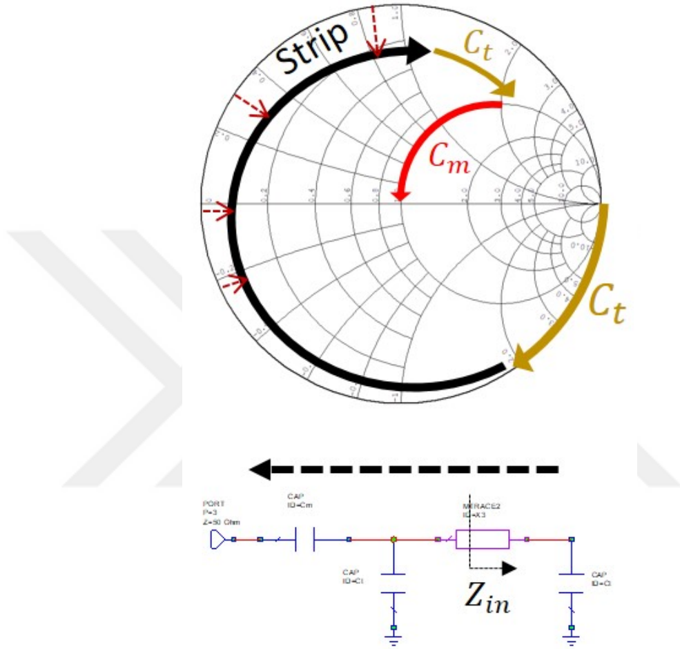
Figure 3.6: Input matching process of a single line element of the coil, explained on the Smith Chart. C_t represents the tuning and C_m denotes the matching capacitor. “Strip” refers to the transmission line. The direction of the arrows shows the movement of the input impedance from “open” to 50\ \Omega .
