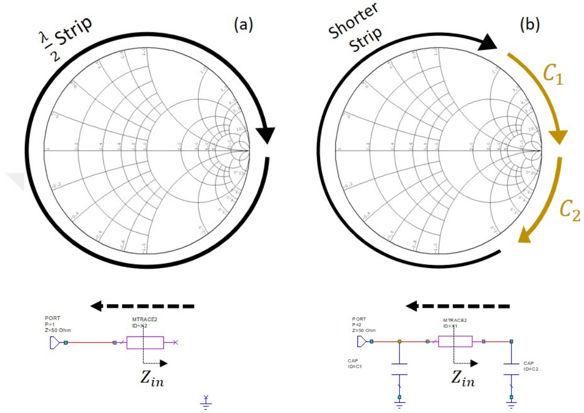
Figure 3.2: (a): Smith chart representation of the input impedance of a \lambda/2 open ended resonator and its schematic. (b): Smith chart representation of the input impedance of an MTL resonator shunted at both ends with capacitors C_1 and C_2 and its schematic.
