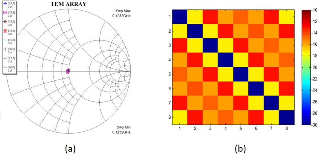
Figure 3.8: (a): The input impedances of the eight ports shown on smith chart. (b): The complete S-matrix (in dB units) of the TEM array at 123.2\text{ MHz} with a reference impedance of 50\ \Omega . Color scale is saturated at -30\text{ dB} in order for better visualization of the non-diagonal elements..
