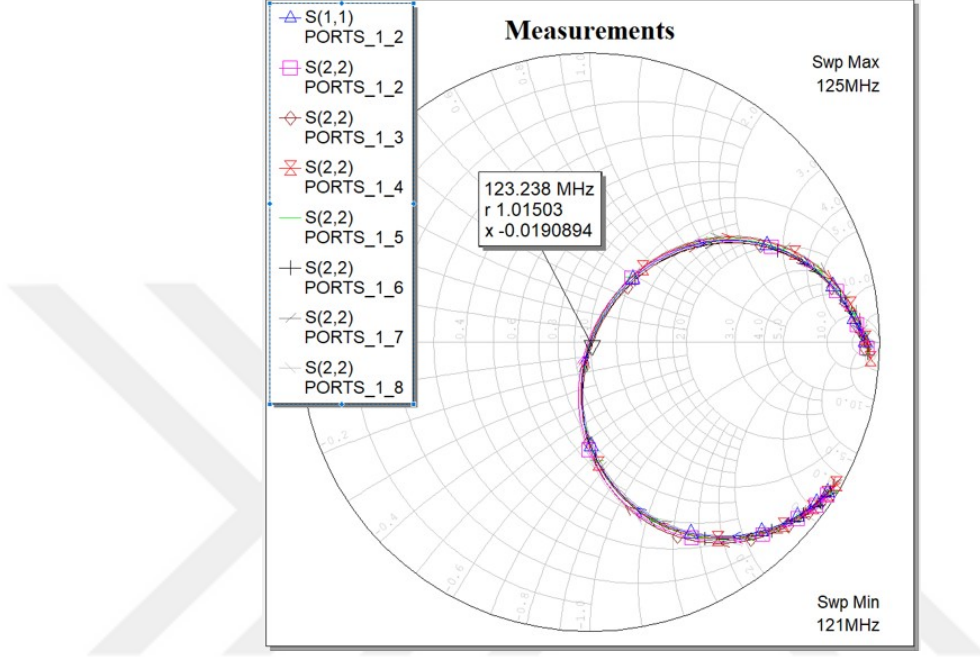
Figure 4.3: Reflection coefficients ( S_{11}, S_{22} \dots S_{88} ) on the Smith Chart.
