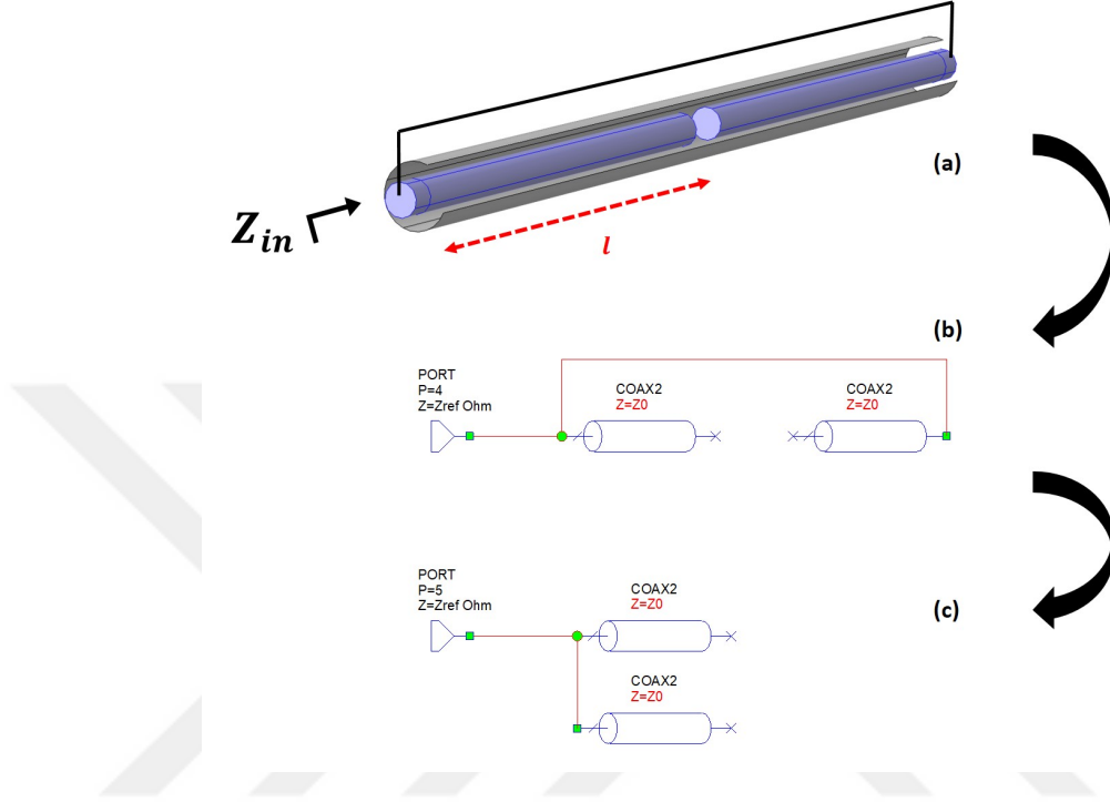
Figure 2.5: A single line element of the coil. (a): The coaxial line element, (b,c): approximation models of the line element.
