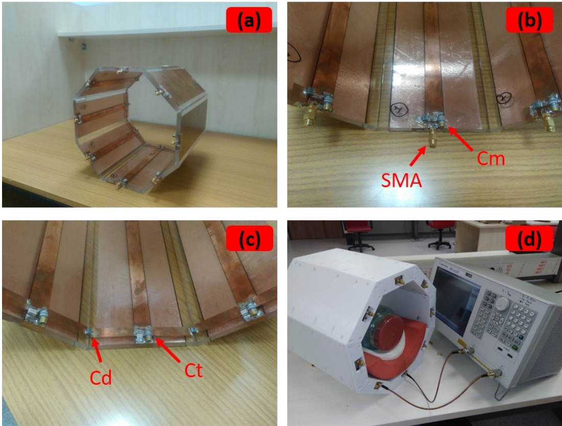
Figure 4.1: The TEM array with and without casing: (a): Constructed 8 channel TEM array. (b),(c): The bare structure viewed from front and back end respectively. C_t and C_d are the tuning and decoupling capacitors, C_m is the matching capacitor. (d): The coated coil being shown in measurements.
