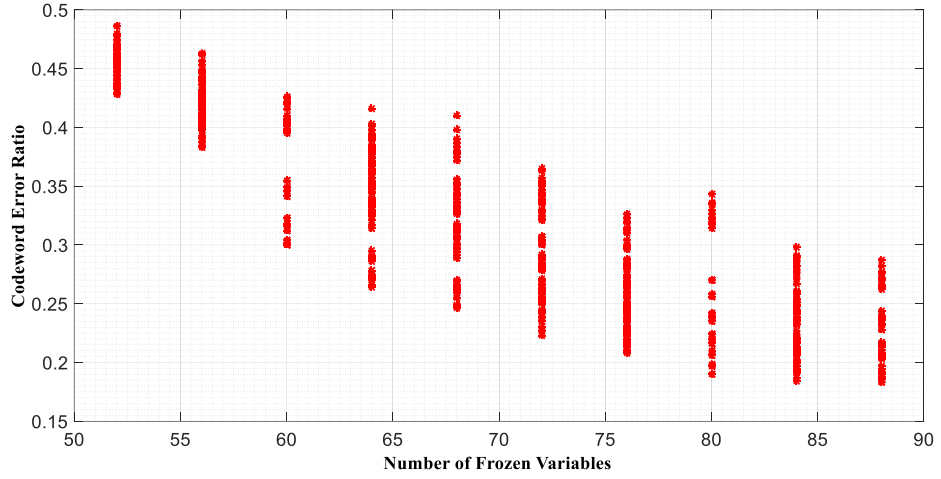
Figure 3.9 Codeword Error Ratio (CER) performance versus the Number of Frozen Variables for Single-FG BP decoder of the (64, 32) adaptive polar code over BEC(0.35).
