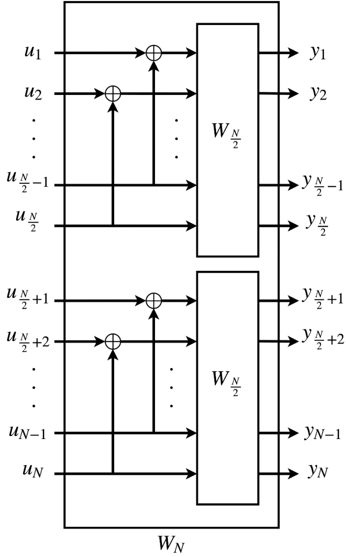
Figure 2.6 W_N channel by combining two independent copies of W_{\frac{N}{2}} .
