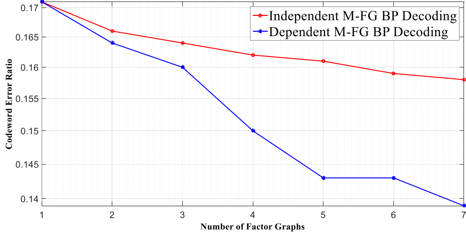
Figure 3.12 Codeword error ratio (CER) comparison of the independent and dependent 7-FG belief propagation decoders for the (128, 64) adaptive polar code over BEC(0.35).
