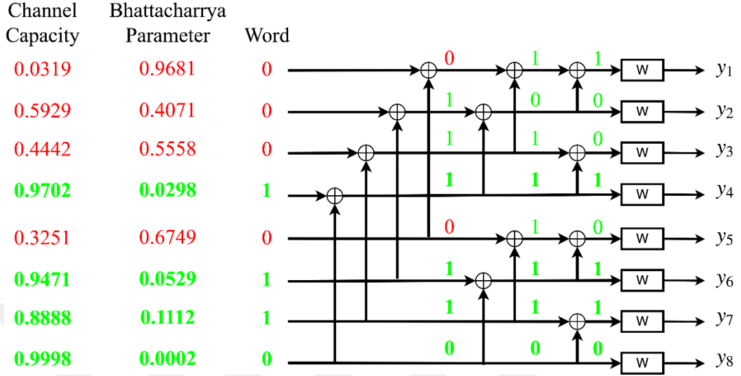
Figure 2.10 Choosing the information bits for an (8, 4) polar code over BEC(0.35), and encoding of the word [1,1,1,0].
