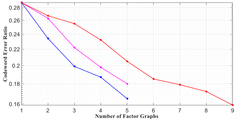
Figure 3.28 Codeword error ratio performance for the (512, 256) adaptive polar code over BEC(0.4) of three M -FG decoder sets, i ) red curve: 9 FG's by cyclically left-shifting stages of the RFG, ii ) pink curve: 5 FG's sampled from the first set, iii ) blue curve: 5 FG's by the Set Choice algorithm.
