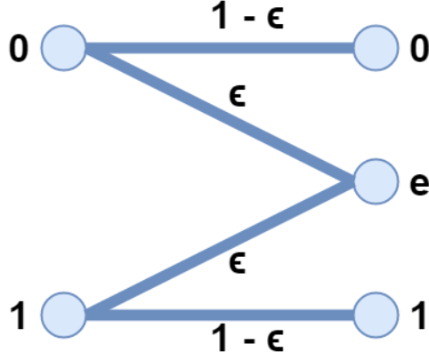
Figure 2.1 Binary erasure channel BEC( \epsilon ).
