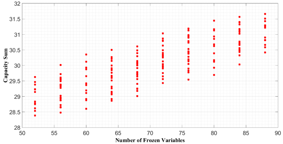
Figure 3.6 Relation between FV and CS values of factor graphs for the (64, 32) adaptive polar code over BEC (0.35).
