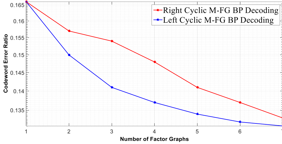
Figure 3.14 Codeword error ratio (CER) comparison of the dependent 7-FG BP decoders with cyclically right and left-shifted RFG sets for the (128, 64) adaptive polar code over BEC(0.35).
