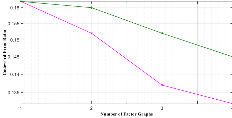
Figure 3.22 Codeword error ratio (CER) performance for the (128, 64) adaptive polar code over BEC(0.35) of two decoder sets, i) green curve: trial set with 4 FG's “7654321-5764321-3765421-1765432”, ii) purple curve: 4-FG cyclic subset starting with odd-numbered stages, chosen from the cyclic set
