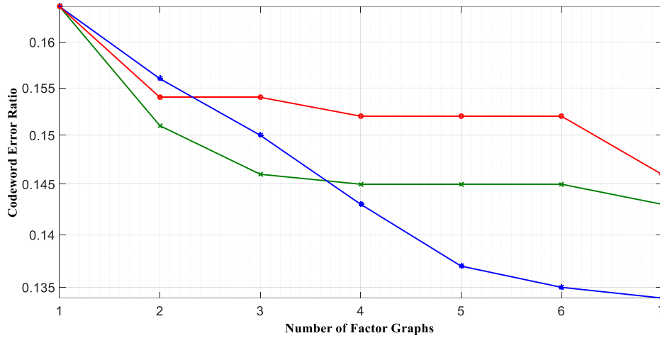
Figure 3.19 Codeword error ratio (CER) performance for the (128, 64) adaptive polar code over BEC(0.35) of three 7-FG decoder sets, i) green curve: 7 top FG's of the SON-sorted list, ii) red curve: the highest CS-valued FG of 7 highest equi-FV groups, and iii) blue curve: 7 FG's generated by cyclic shifts; i.e., the cyclic set.
