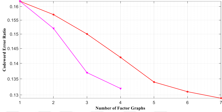
Figure 3.21 Codeword error ratio (CER) performance for the (128, 64) adaptive polar code over BEC(0.35) of two decoder sets, i) red curve: cyclic set with 7 FG's, ii) purple curve: 4 FG's starting with odd-numbered stages, chosen from the cyclic set.
