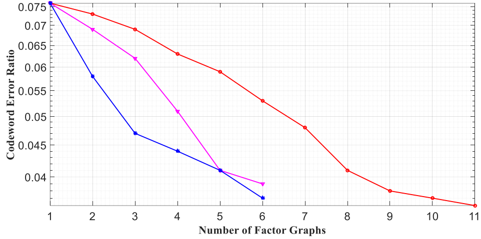
Figure 3.30 Codeword error ratio performance for the (2048, 1024) adaptive polar code over BEC(0.4) of three M -FG decoder sets, i) red curve: 11 FG's by cyclically left-shifting stages of the RFG, ii) pink curve: 6 FG's sampled from the first set, iii) blue curve: 6 FG's by the Set Choice algorithm.
