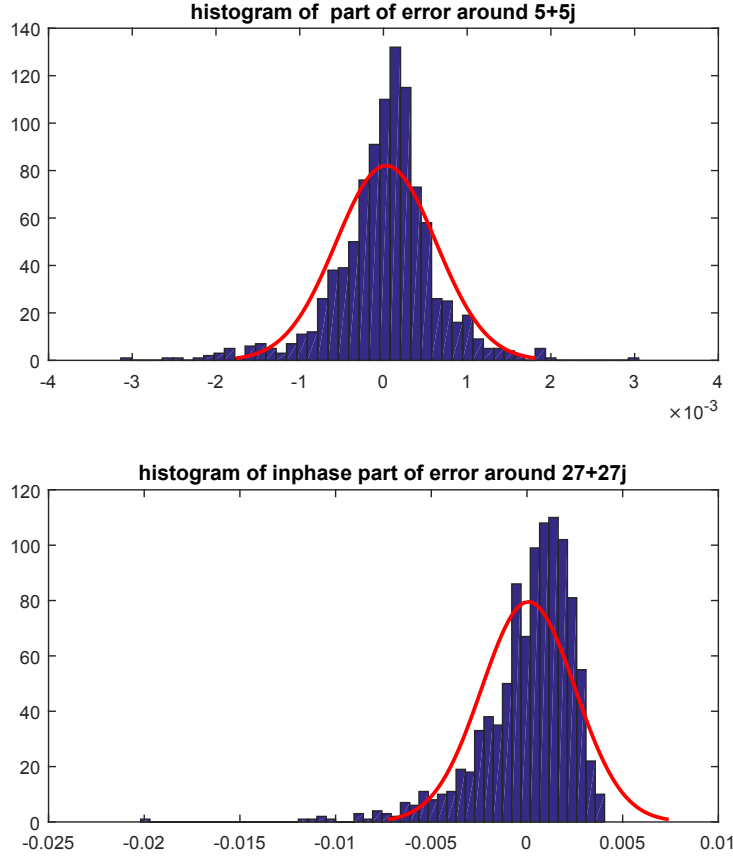
Figure 4.3: Histograms of in-phase part of error distributions around 5+5j and 27+27j for the Saleh model
