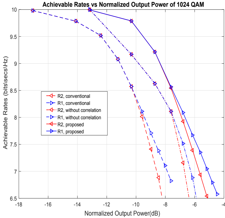
Figure 5.4: Achievable Rates of the channel for the Saleh model
