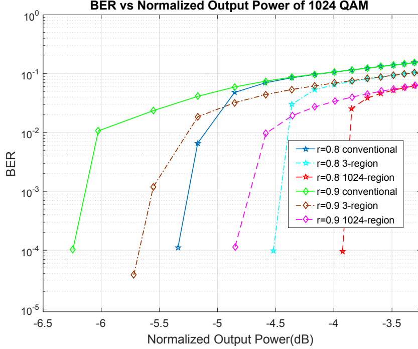
Figure 5.3: BER curves of the receivers with rate 0.8 and 0.9
