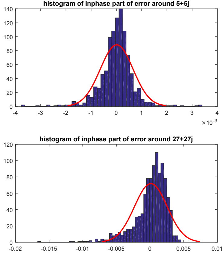
Figure 4.2: Histograms of in-phase part of error distributions around 5+5j and 27+27j for the Rapp model
