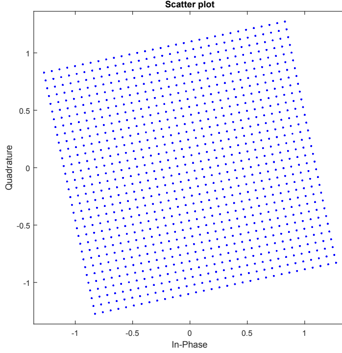
Figure 3.2: Rotation of the 1024QAM constellation with the complex \alpha or the rotation matrix
