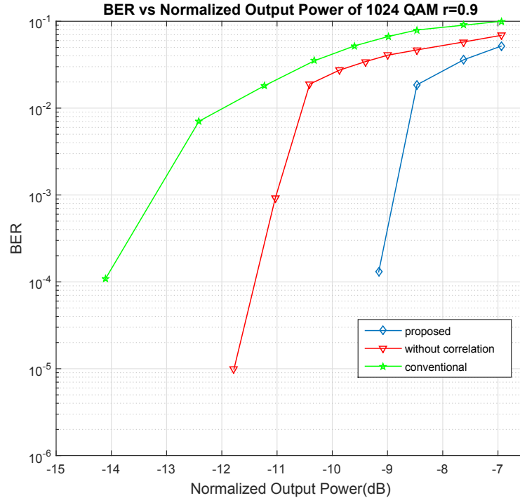
Figure 5.5: BER curves of the receivers with rate 0.9
