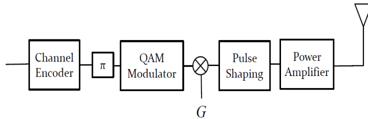
Figure 2.1: Transmitter Side
