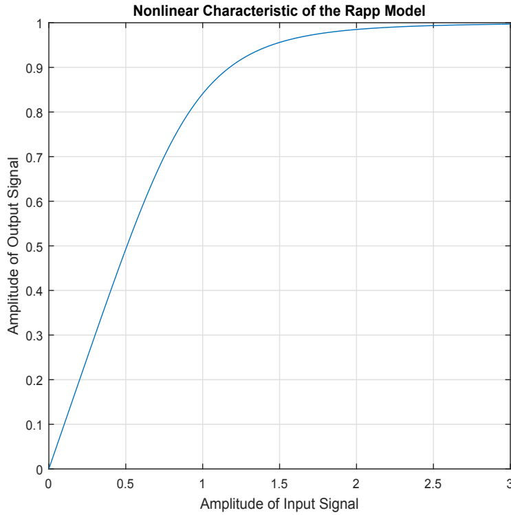
Figure 2.3: Nonlinear Characteristic of the Rapp model with parameters p = 2 , A_0 = 1 , v = 1
