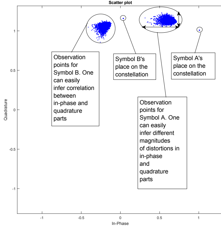
Figure 3.1: Two specific outermost constellation points' observation symbols in the receiver side
