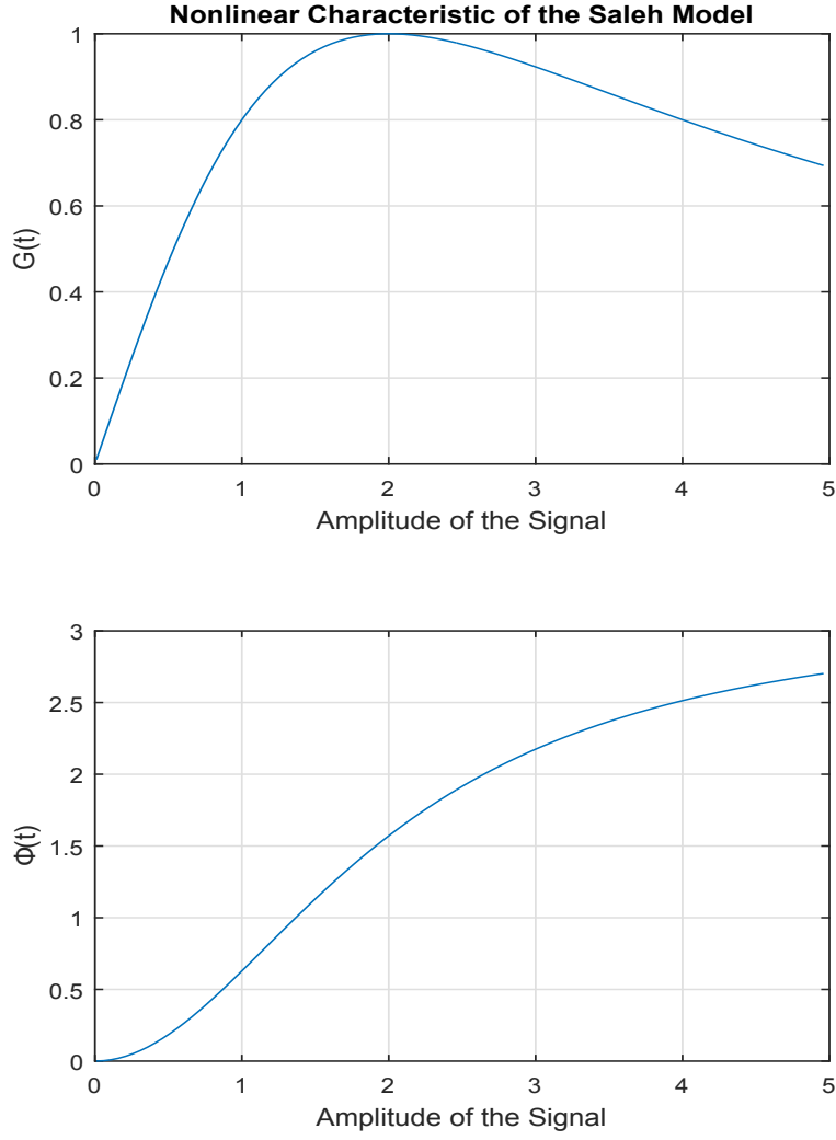
Figure 2.4: Nonlinear Characteristic of the Saleh model with parameters g_0 = 1 , A_0 = 2 , \alpha = \pi/4 , \beta = 0.25
