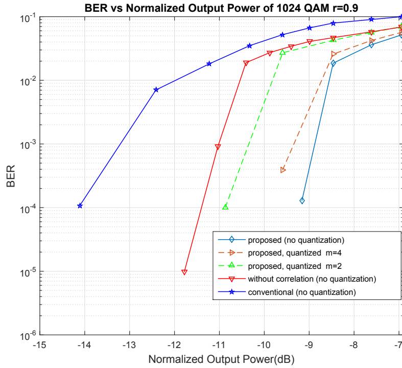
Figure 5.7: BER curves of the receivers for the Saleh model
