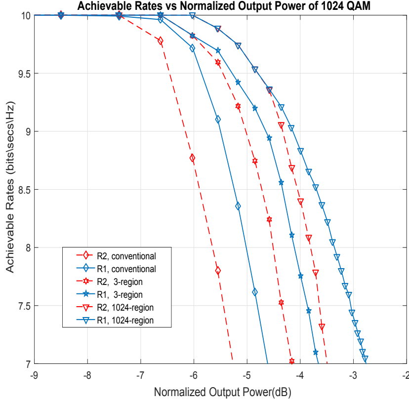
Figure 5.2: Achievable Rates of the channel for the Rapp model
