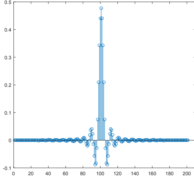
Figure 2.2: Root Raised Cosine Filter with 0.25 roll of factor, 5 samples per symbol and 201 taps
