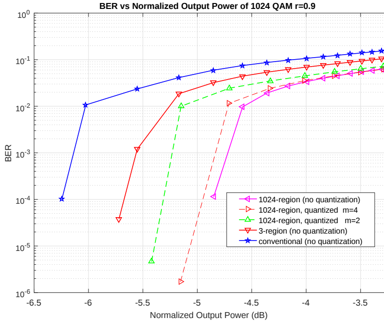
Figure 5.6: BER curves of the receivers for the Rapp model
