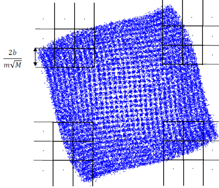
Figure 5.1: Quantization Regions
