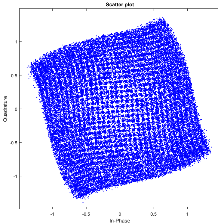
Figure 1.2: 1024 QAM constellation points passed through a power amplifier with the Saleh model
