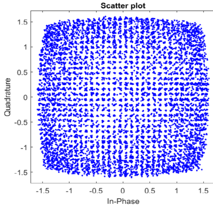
Figure 1.1: 1024 QAM constellation points passed through a power amplifier with the Rapp model
