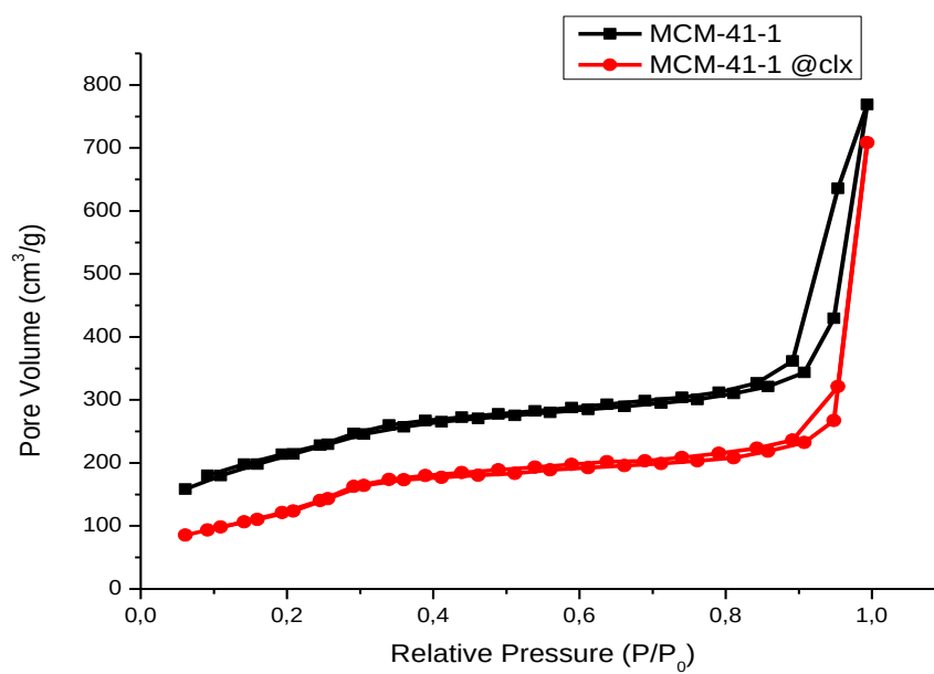
Figure A.2: BET isotherms of isotherms of MCM-41-1 and MCM-41-1@clx in ethanol
