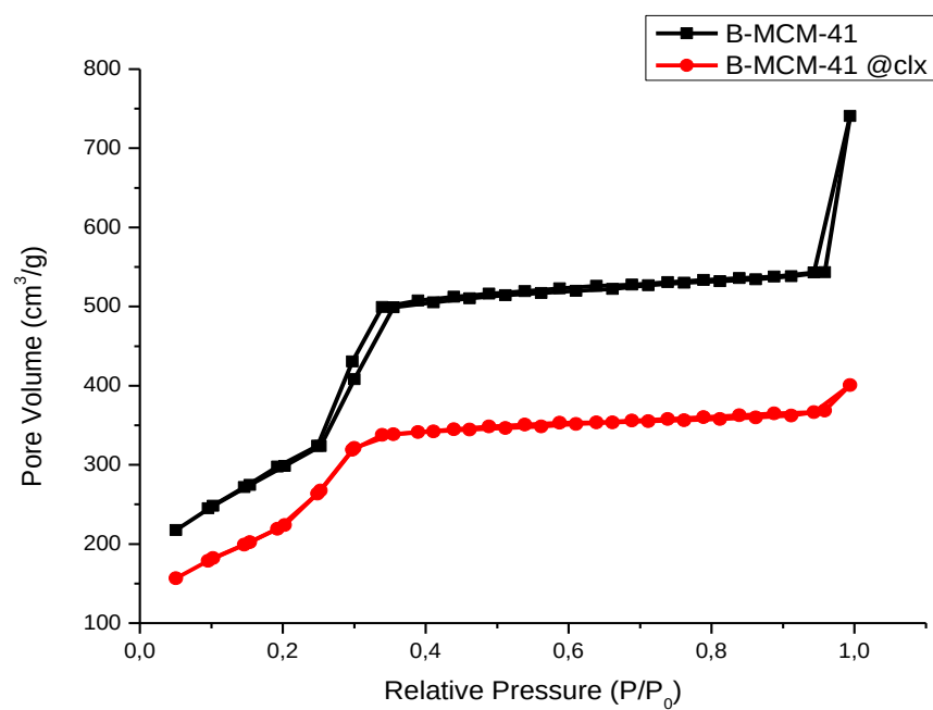
Figure A.5: BET isotherms of isotherms of B-MCM-41 and B-MCM-41@clx in ethanol
