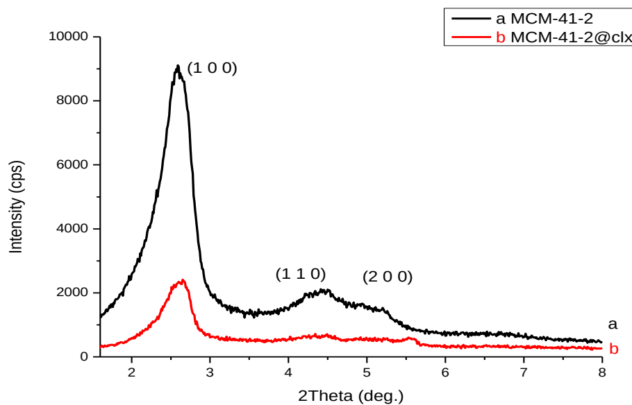
Figure 23: Small angle powder XRD patterns of a) MCM-41-2 b) MCM-41-2@clx in hexane
