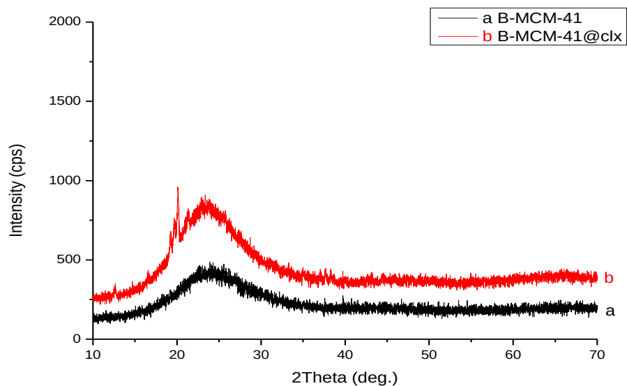
Figure 20: Wide angle powder XRD patterns of a) B-MCM-41 b) B-MCM-41@clx in ethanol
