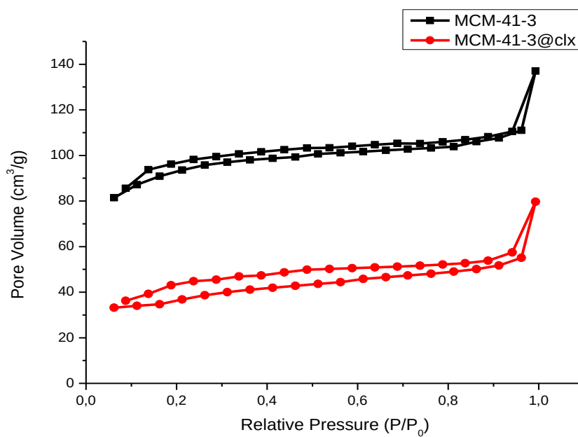
Figure A.4: BET isotherms of isotherms of MCM-41-3 and MCM-41-3@clx in ethanol
