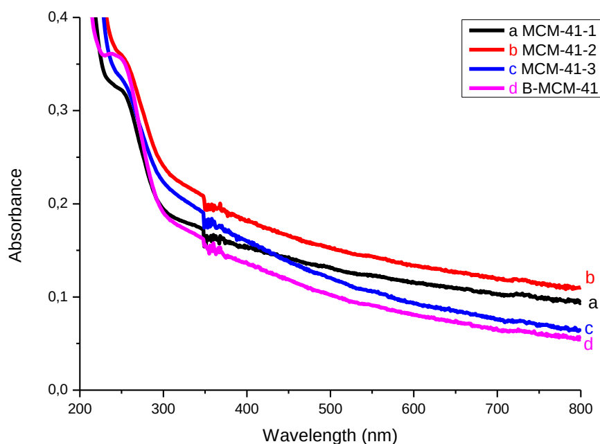
Figure 59: UV graph of a) MCM-41-1 b) MCM-41-2 c) MCM-41-3 d) B-MCM-41 in hexane filtrate in the loading process
