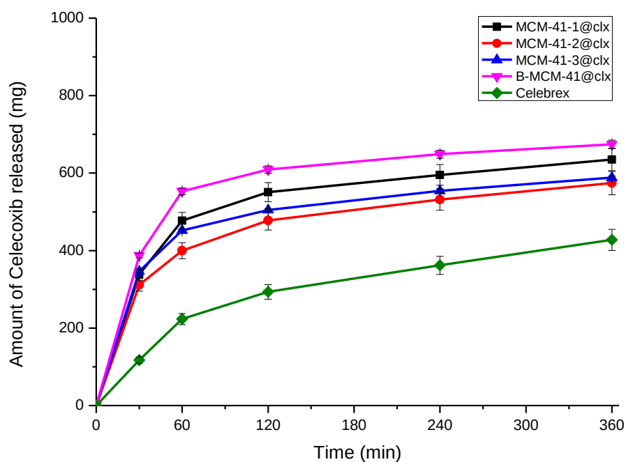
Figure 66: Amount of Celecoxib released from 1.0 g of Celecoxib loaded to MCM-41 in hexane within 6 hours
