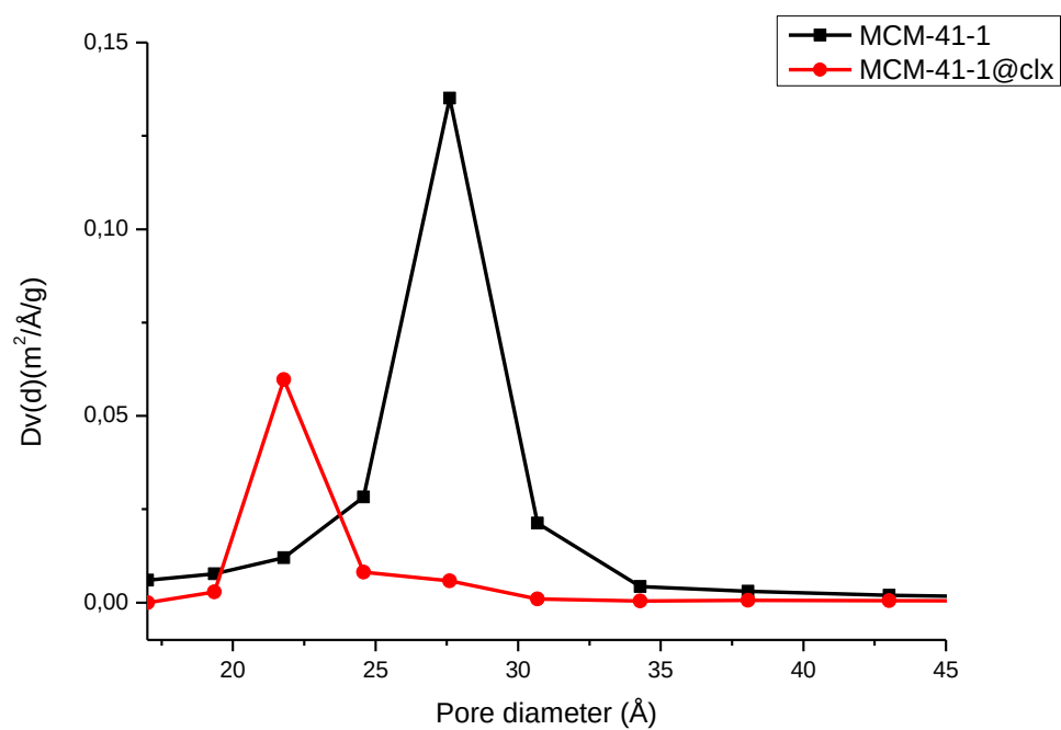
Figure 44: Pore size distribution of MCM-41-1 and MCM-41-1@clx in hexane
