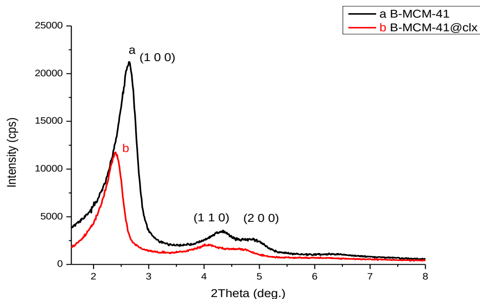
Figure 16: Small angle powder XRD patterns of a) B-MCM-41 b) B-MCM-41@clx in ethanol
