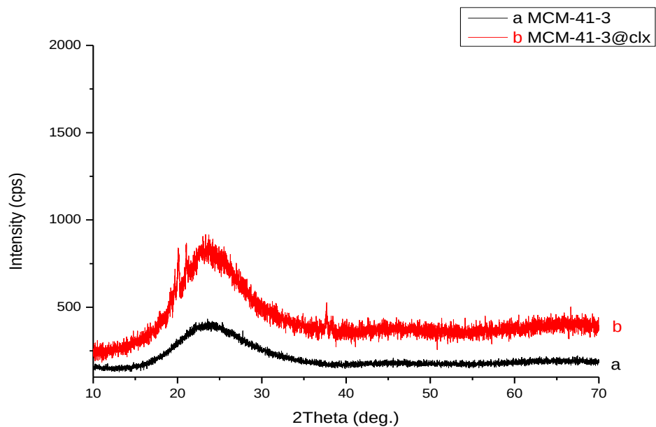
Figure 19: Wide angle powder XRD patterns of a) MCM-41-3 b) MCM-41-3@clx in ethanol
