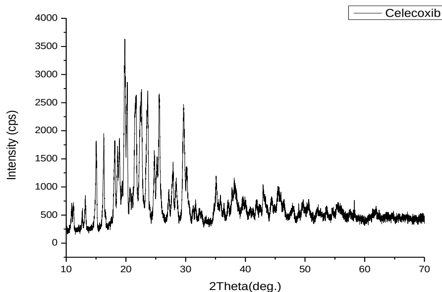
Figure 21: Wide angle powder XRD of Celecoxib
