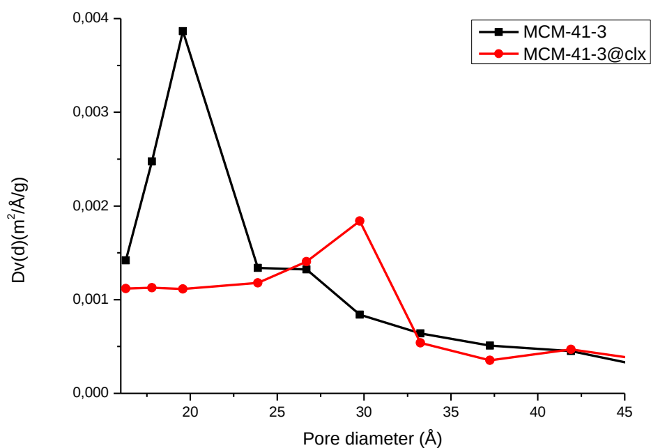
Figure 46: Pore size distribution of MCM-41-3 and MCM-41-3@clx in hexane
