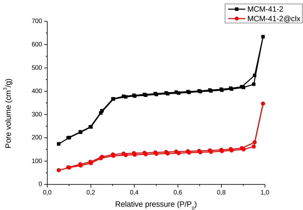
Figure 41: BET isotherms of MCM-41-2 and MCM-41-2@clx in hexane
