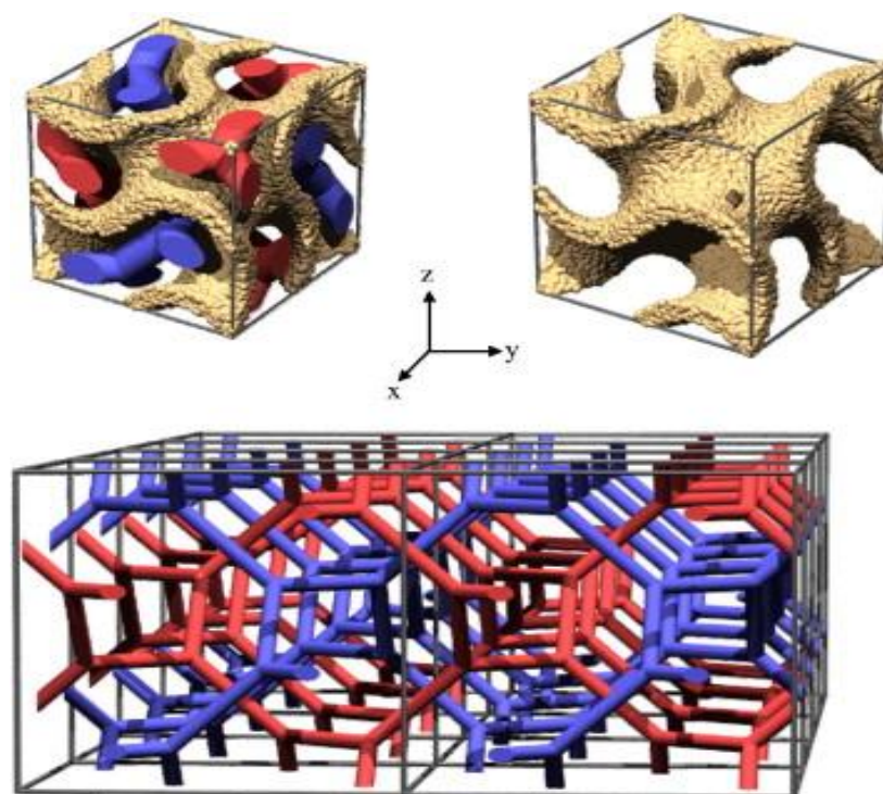
Figure 1: Cubic unit cell of MCM-48 [7]
