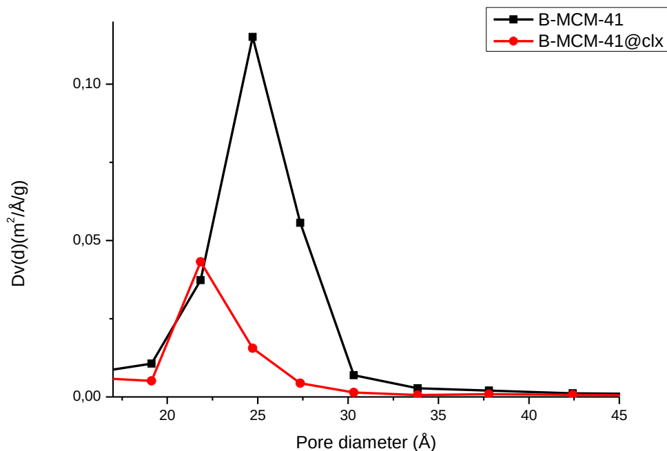
Figure 47: Pore size distribution of B-MCM-41 and B-MCM-41@clx in hexane
