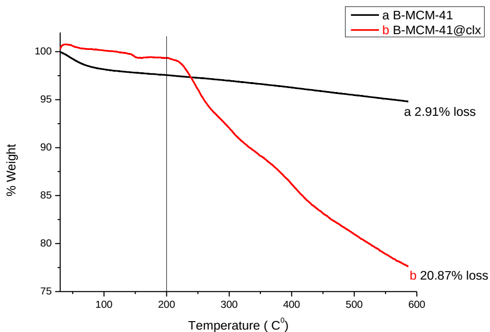
Figure 70: % Weight loss of a) B-MCM-41 b)B-MCM-41@clx samples
