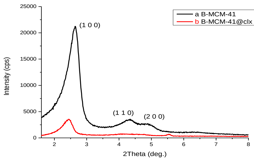
Figure 25: Small angle powder XRD patterns of a) B-MCM-41 b) B-MCM-41@clx in hexane
