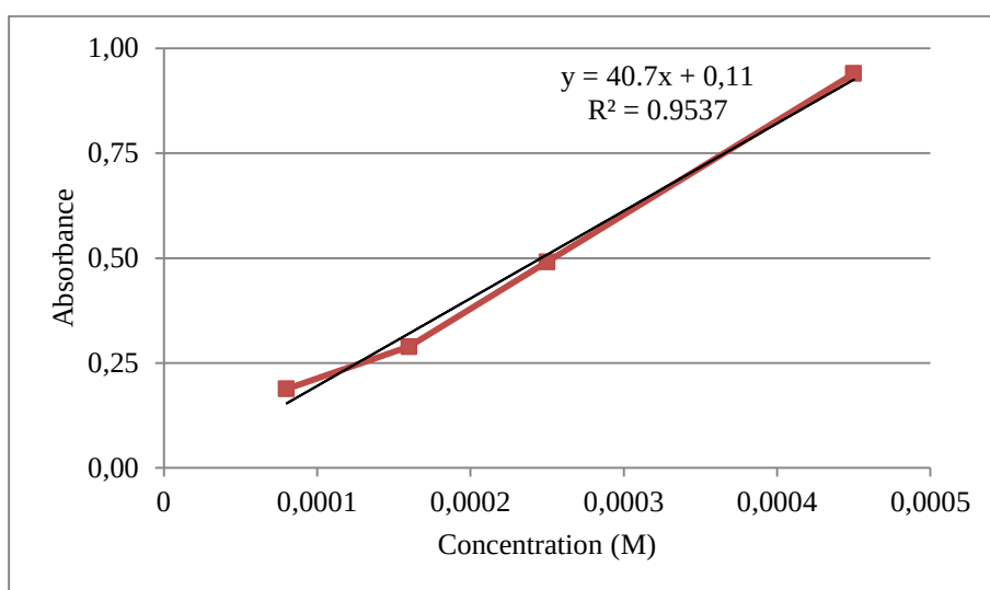
Figure 60: Calibration curve of release process of Celecoxib in PBS
