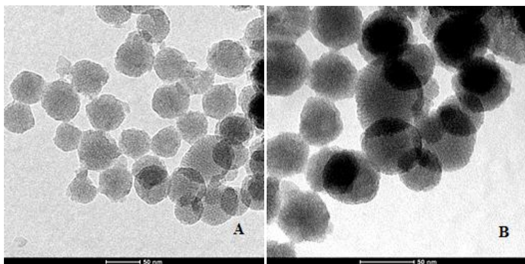
Figure 48: TEM images of A) MCM-41-1 and B) MCM-41-1@clx in ethanol
