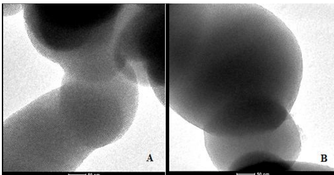
Figure 51: TEM images of A) B-MCM-41 and B) B-MCM-41@clx in ethanol
