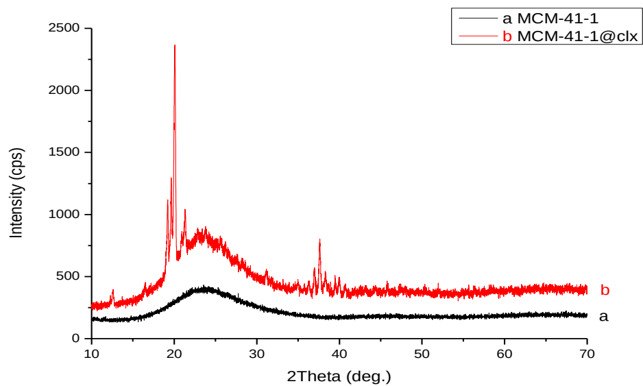
Figure 17: Wide angle powder XRD patterns of a) MCM-41-1 b) MCM-41-1@clx in ethanol
