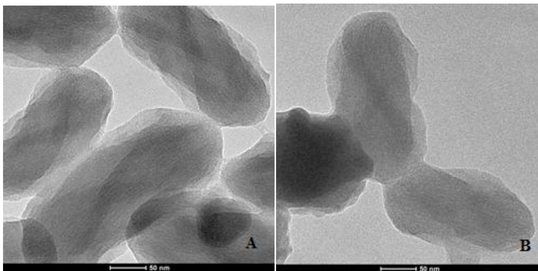
Figure 50: TEM images of A) MCM-41-3 and B) MCM-41-3@clx in ethanol
