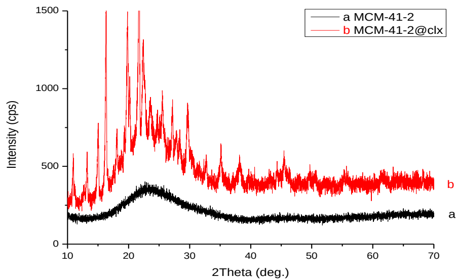
Figure 28: Wide angle powder XRD patterns of a) MCM-41-2 b) MCM-41-2@clx in hexane
