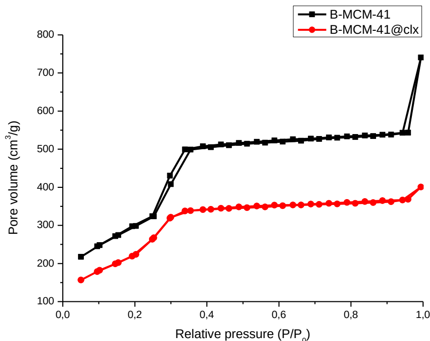
Figure 43: BET isotherms of B-MCM-41 and B-MCM-41@clx in hexane
