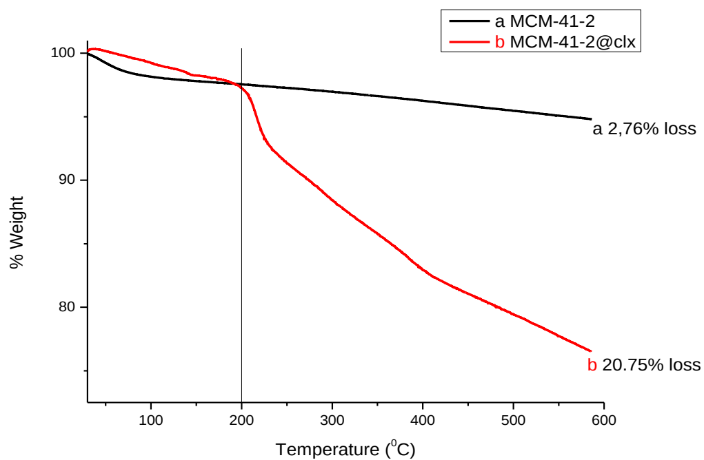
Figure 68: % Weight loss of a) MCM-41-2 b)MCM-41-2@clx samples
