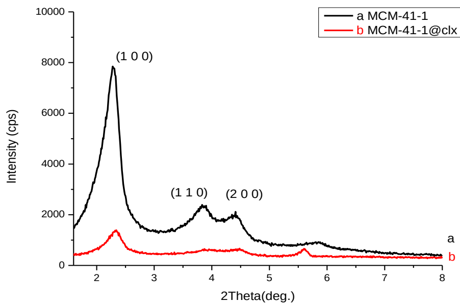
Figure 22: Small angle powder XRD patterns of a) MCM-41-1 b) MCM-41-1@clx in hexane
