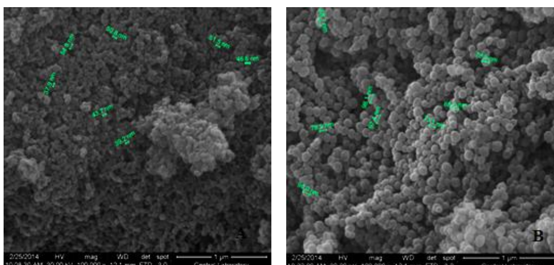
Figure 53: SEM images of A) MCM-41-2 and B) MCM-41-2@clx in ethanol
