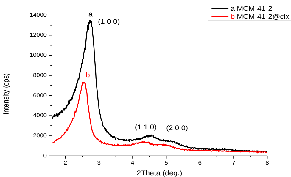
Figure 14: Small angle powder XRD patterns of a) MCM-41-2 b) MCM-41-2@clx in ethanol
