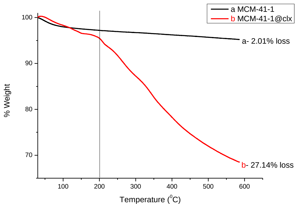
Figure 67: % Weight loss of a) MCM-41-1 b)MCM-41-1@clx samples
