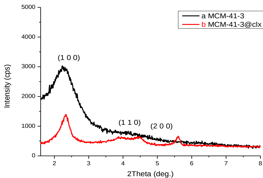
Figure 24: Small angle powder XRD patterns of a) MCM-41-3 b) MCM-41-3@clx in hexane
