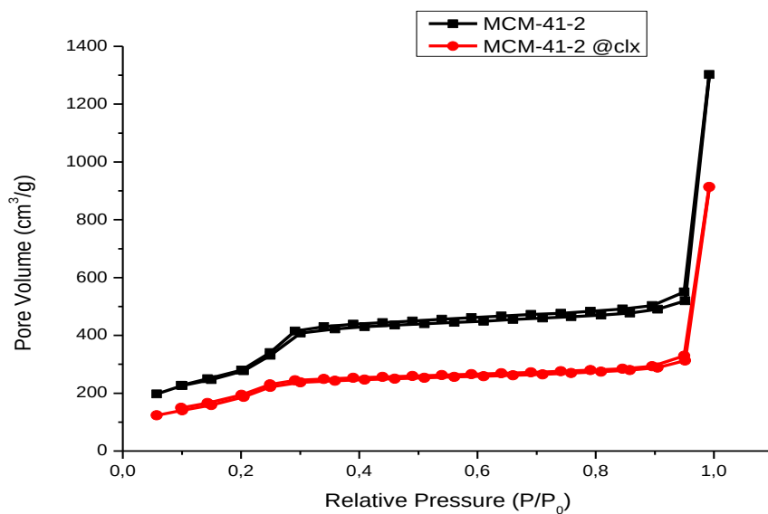
Figure A.3: BET isotherms of isotherms of MCM-41-2 and MCM-41-2@clx in ethanol
