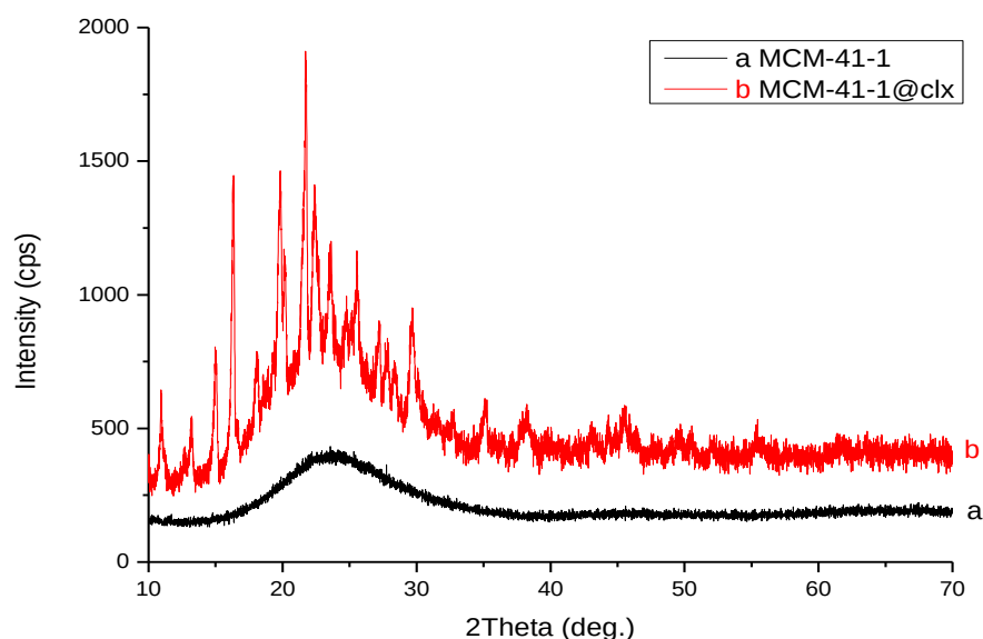
Figure 27: Wide angle powder XRD patterns of a) MCM-41-1 b) MCM-41-1@clx in hexane
