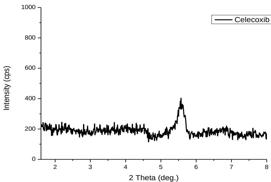
Figure 26: Small angle powder XRD pattern of Celecoxib
