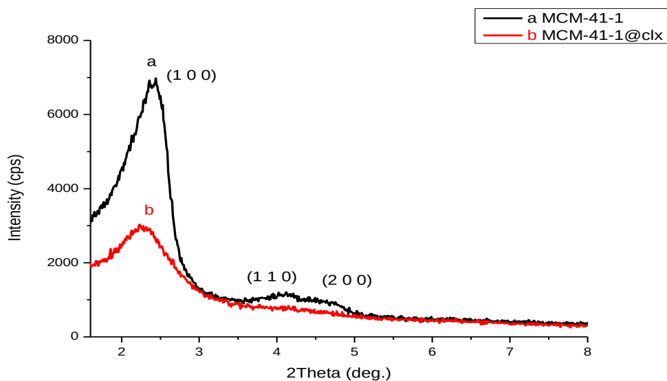
Figure 13: Small angle powder XRD patterns of a) MCM-41-1 b) MCM-41-1@clx in ethanol
