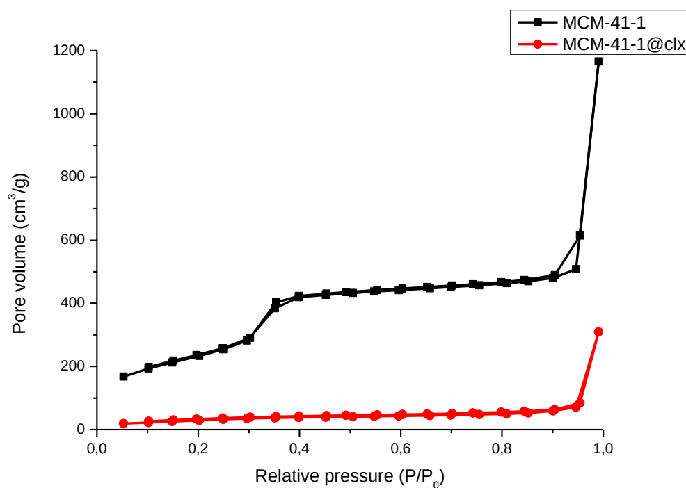
Figure 40: BET isotherms of MCM-41-1 and MCM-41-1@clx in hexane
