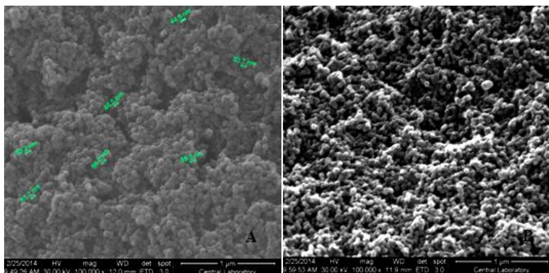
Figure 52: SEM images of A) MCM-41-1 and B) MCM-41-1@clx in ethanol
