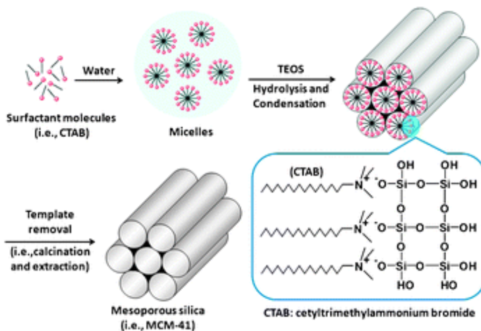
Figure 2: Scheme of the formation mechanism of MCM-41[10]
