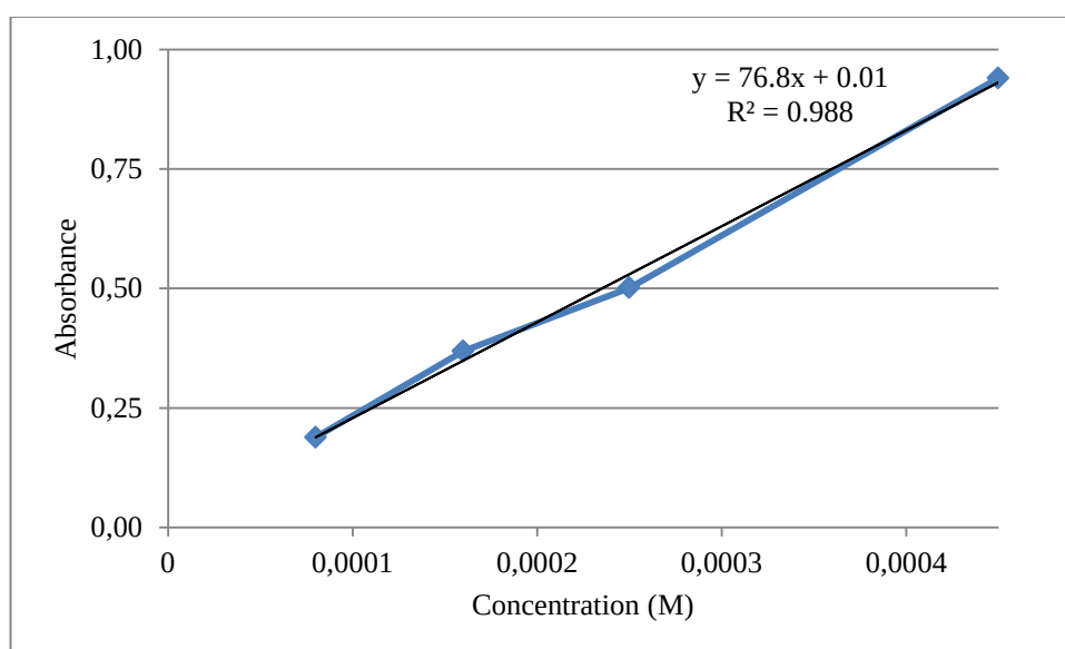
Figure 56: Calibration curve of loading process of Celecoxib in ethanol
