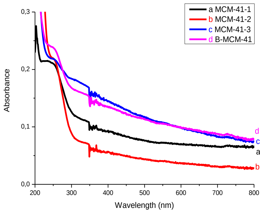
Figure 58: UV graph of a) MCM-41-1 b) MCM-41-2 c) MCM-41-3 d) B-MCM-41 in ethanol in the loading process
