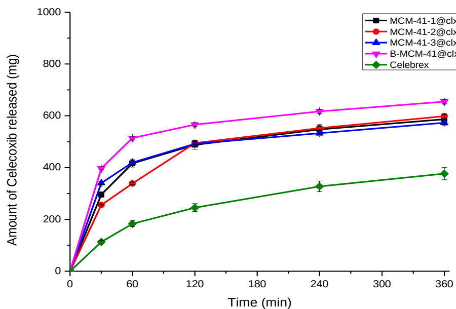
Figure 65: Amount of Celecoxib released from 1.0 g of Celecoxib loaded to MCM-41 in hexane within 6 hours
