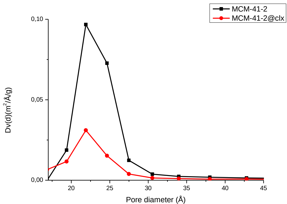
Figure 45: Pore size distribution of MCM-41-2 and MCM-41-2@clx in hexane
