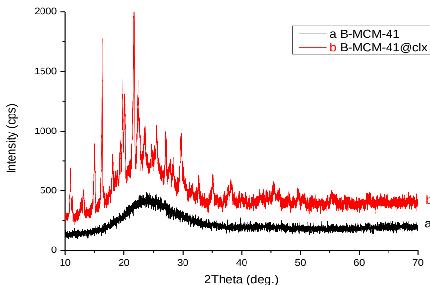
Figure 30: Wide angle powder XRD patterns of a) B-MCM-41 b) B-MCM-41@clx in hexane
