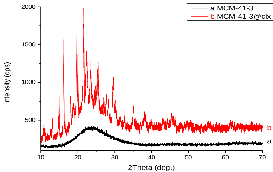
Figure 29: Wide angle powder XRD patterns of a) MCM-41-3 b) MCM-41-3@clx in hexane
