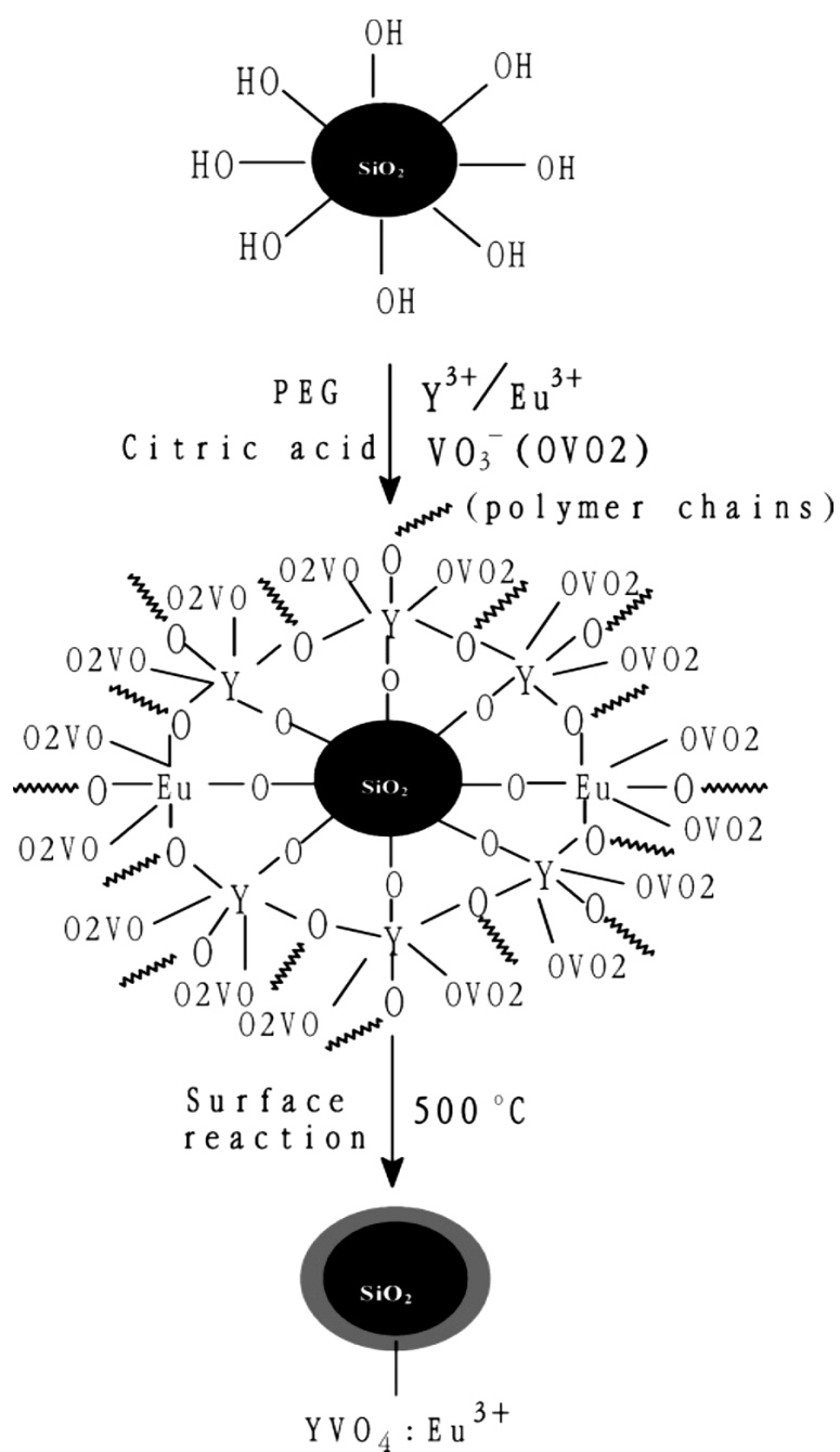
Figure 11: Schematic representation of formation Process of YVO 4 :Eu 3+ functionalized MCM-41 particles [50]
