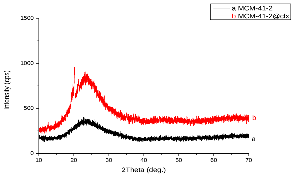
Figure 18: Wide angle powder XRD patterns of a) MCM-41-2 b) MCM-41-2@clx in ethanol
