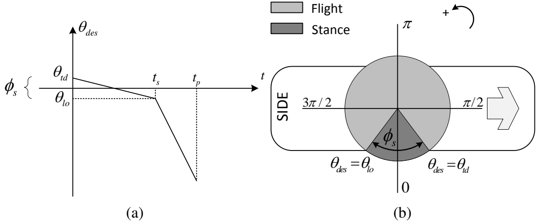
Figure 6.4: (a)The Buehler two speed profile is defined by 4 parameters (b) Side view of the robot with a desired leg angle of the flight and stance phase [\theta_{id}, \theta_{lo}, t_s, t_p] [4].
