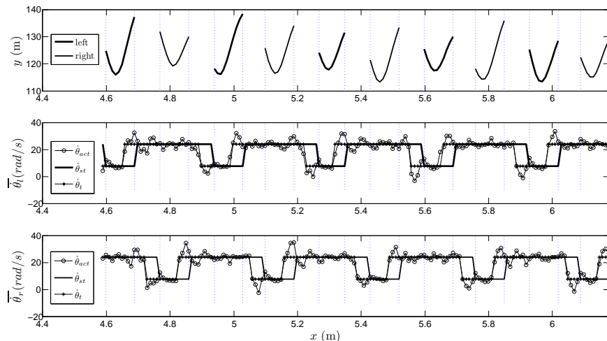
Figure 6.6: The stance phases of one run (top), mean of the actual \dot{\theta}_{act} , target angular velocity \dot{\theta}_t and shifted target angular velocity \dot{\theta}_{st} of the left (middle) and right tripod (bottom).
