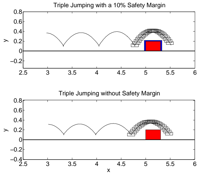
Figure 5.19: The COM trajectory of the robot that jumps over obstacle ( h_{obs} = 0.2 (m) and w_{obs} = 0.3 ) (top) with a 10% safety margin (bottom) without the safety margin.
