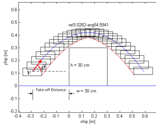
Figure 5.1: Jumping over obstacles whose height is 0.3 m and width is 0.3 m. The red line represents the clearance of the robot.
