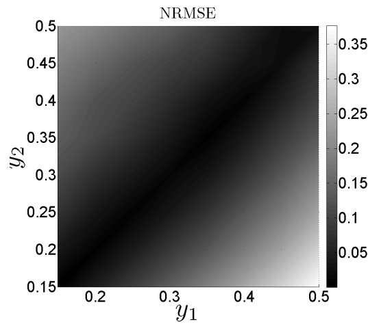
Figure 3.11: Accuracy of steady-state height control for different initial condition and desired height pairs. The color code corresponds to the values of the N-RMSE calculated by (3.9).
