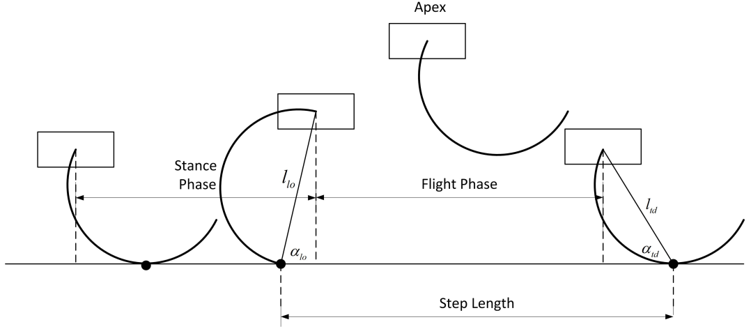
Figure 3.1: Stance, flight phase and step length of the robot
