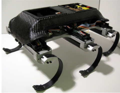
Figure 6.1: Edubot [3]
