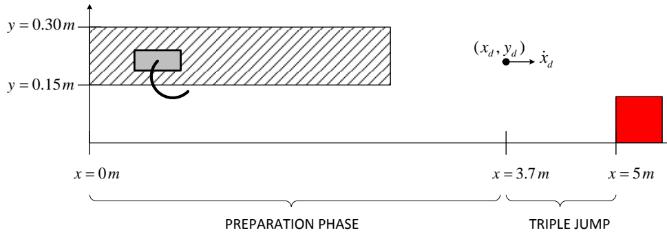
Figure 5.4: The preparation and triple jump phase of the second case. The obstacle is placed at x = 5 m . The shaded area represents the initial state space. The robot is left from any point in the shaded area with a zero velocity.
