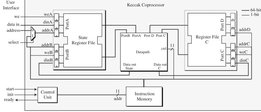
Figure 4.2: KECCAK coprocessor.
