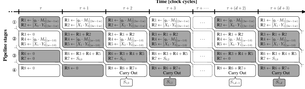
Figure 5.2: A view for pipelined computation of high-radix modular multiplication operation.
