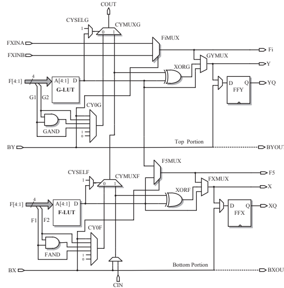
Figure 2.5: Simplified architecture of a Spartan-3 slice.
