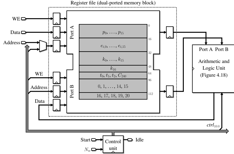
Figure 4.16: Architecture of the Threefish coprocessor.
