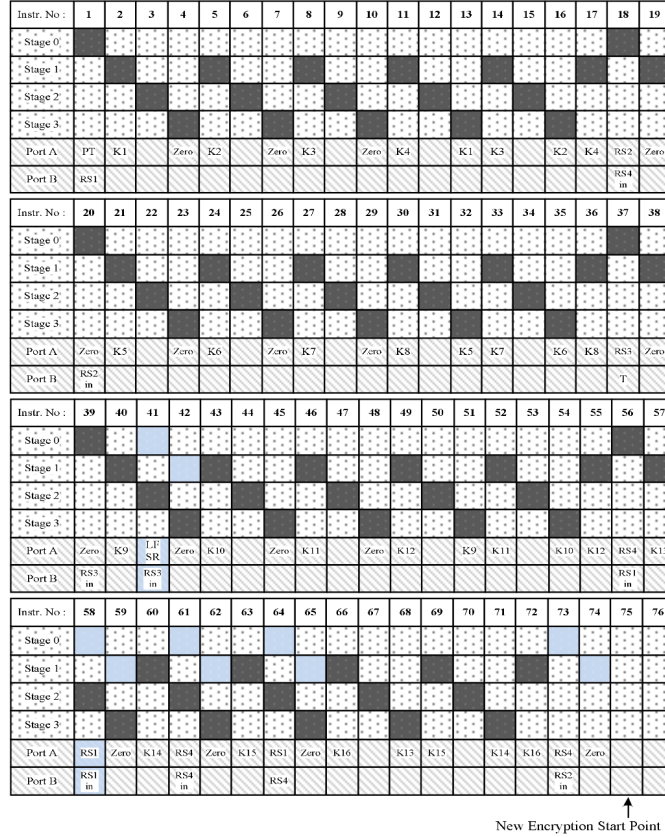
Figure 3.4: Instruction Scheduling.
