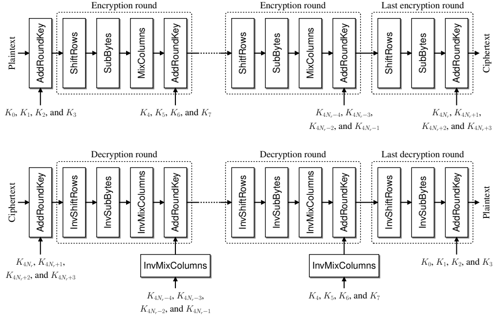
Figure 2.3: AES encryption and decryption flowcharts (reprinted from [33])
