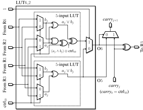
Figure 4.19: Computation of R3 \leftarrow R1 \oplus R2 or R3 \leftarrow R3 \oplus R6 on a Virtex-6 device.
