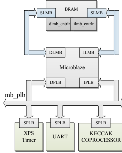
Figure 4.8: PLB connection for the KECCAK coprocessor in MicroBlaze based embedded system (KECCAK PLB SoC).
