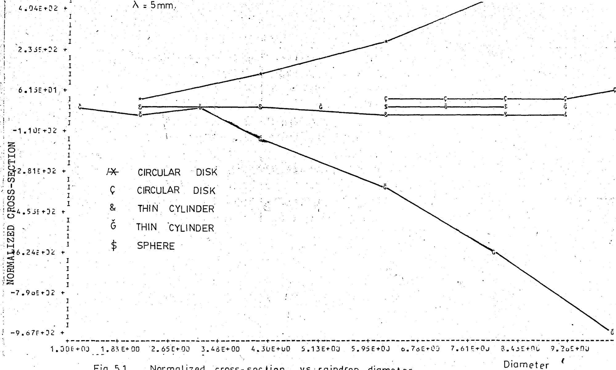
Fig 51 Normalized cross-section vs raindrop diameter.
