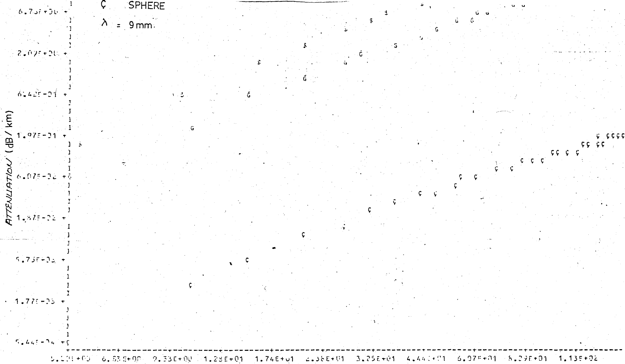
Fig 5 5 Attenuation VS Rainfall rate
