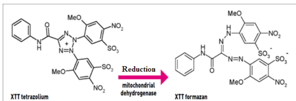
Figure 2.4: The reduction of XTT to form the colored formazan.
