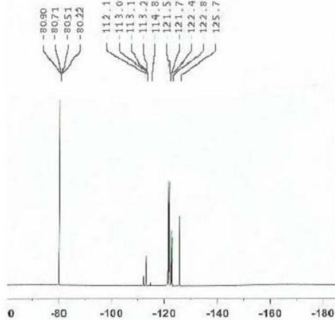
Şekil 3.2. 4-(3,3,4,4,5,5,6,6,7,7,8,8,9,9,10,10,10-heptadekafluorodesiltiyo)ftalonitril (6) maddesine ait ^{19}\text{F} NMR Spektrumu
