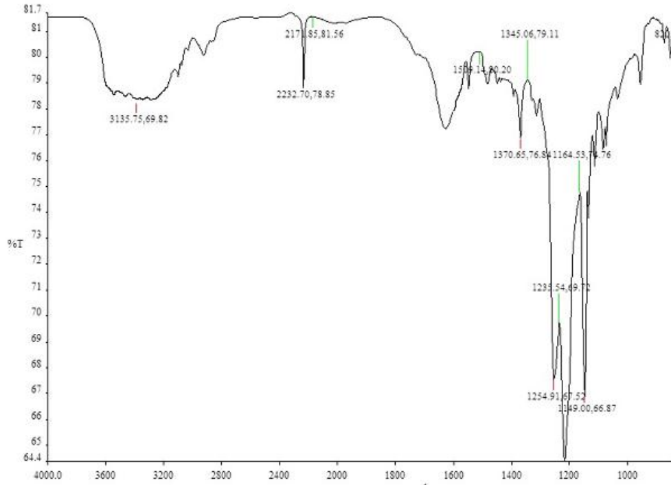
Şekil 3.1. 4-(3,3,4,4,5,5,6,6,7,7,8,8,9,9,10,10,10-heptadecafluorodesiltiyo)ftalonitril (6) maddesine ait IR Spektrumu
