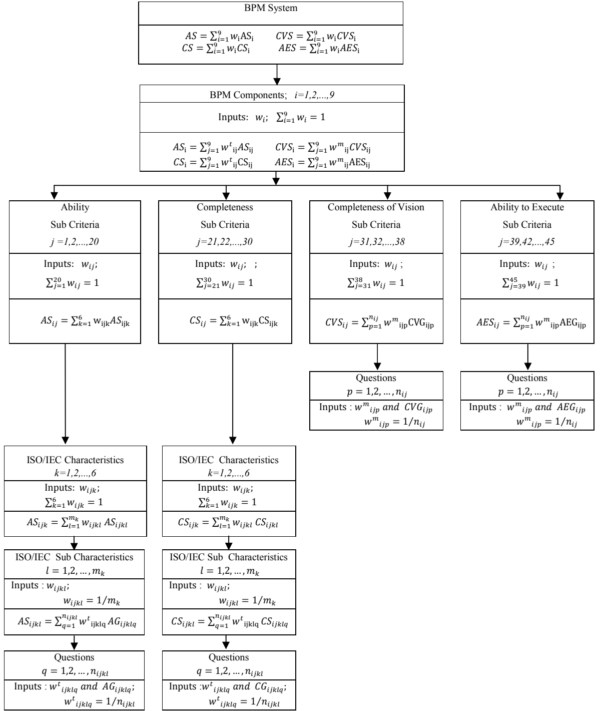
Fig 13 Quantification of the BPM System Evaluation Framework Model
