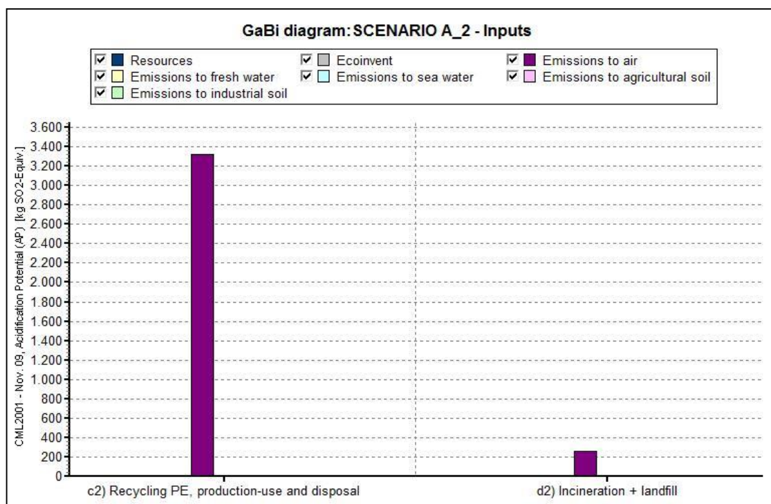
Figure C.15. CML 2001 Nov. '09 Method. Acidification Potential results for Scenario A.2.
