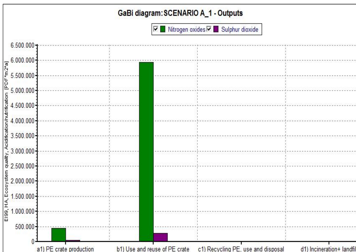
Figure C.17. EI 99 Method. Acidification / Nutritation results for Scenario A.1.
