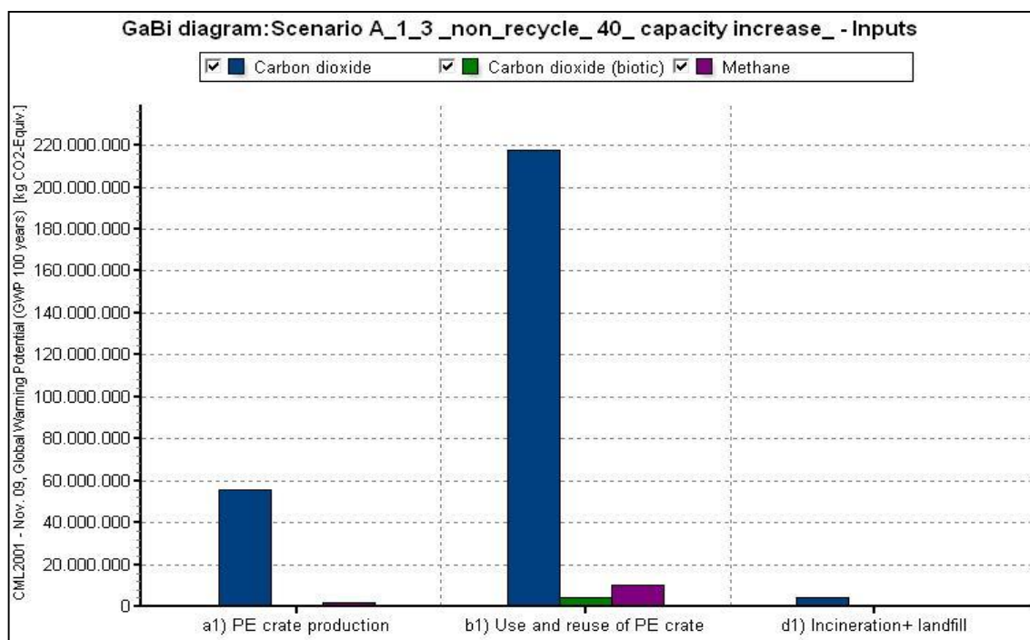
Figure C.91. CML 2001 Nov. '09 Method. Global Warming Potential results for Scenario A.1.3.
