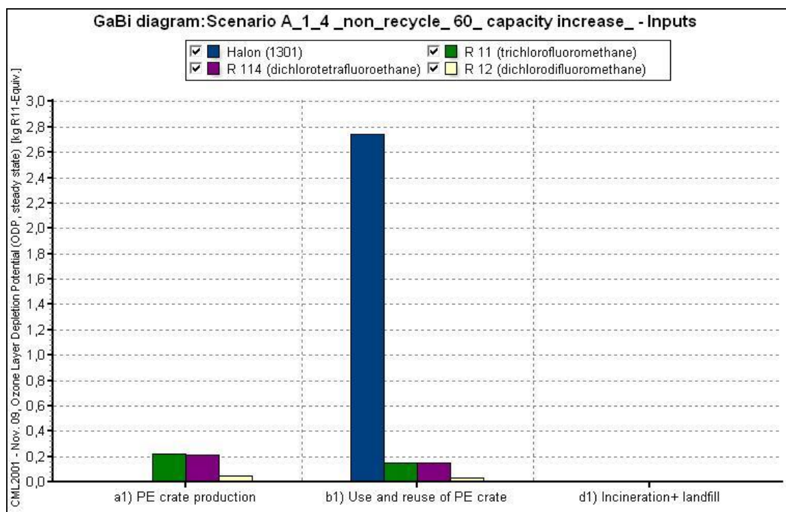
Figure C.95. CML 2001 Nov. '09 Method. Ozone Layer Depletion results for Scenario A.1.4.
