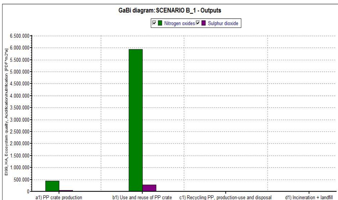
Figure C.18. EI 99 Method. Acidification / Nutritation results for Scenario B.1.
