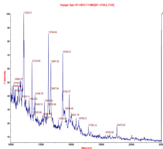
Figure 4.1. MALDI-TOF-MS spectra of control group.
