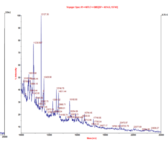
Figure 4.1. MALDI-TOF-MS spectra of control group.
