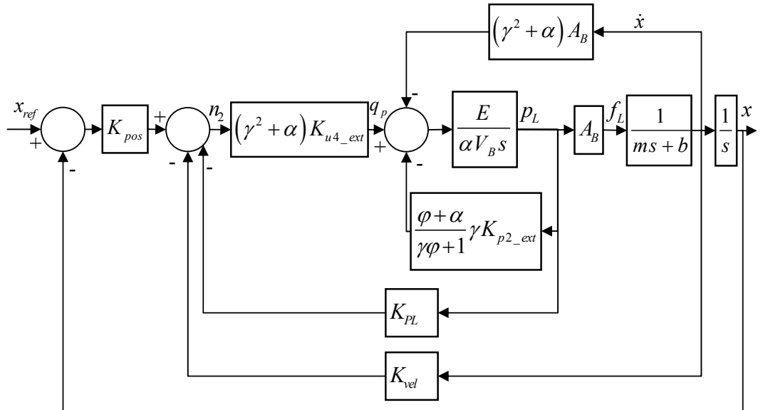
Figure 4-3 Block Diagram Representation of the Closed Loop Valve Controlled System
