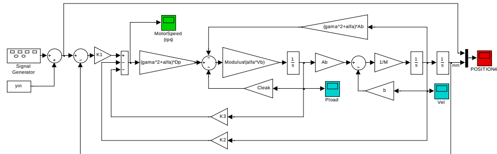
Figure 4-2 MATLAB Simulink Model of the Closed Loop Pump Controlled Position Control System
