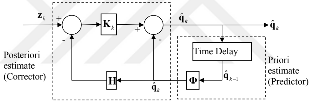
Figure 4-5 Kalman Filter Block Diagram
