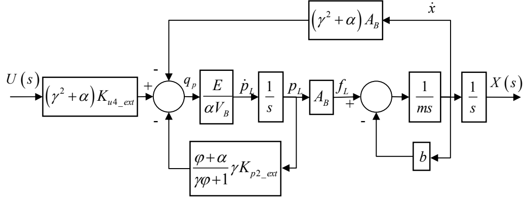
Figure 3-22 Block Diagram Representation of the Valve Controlled System for the Extension Case
