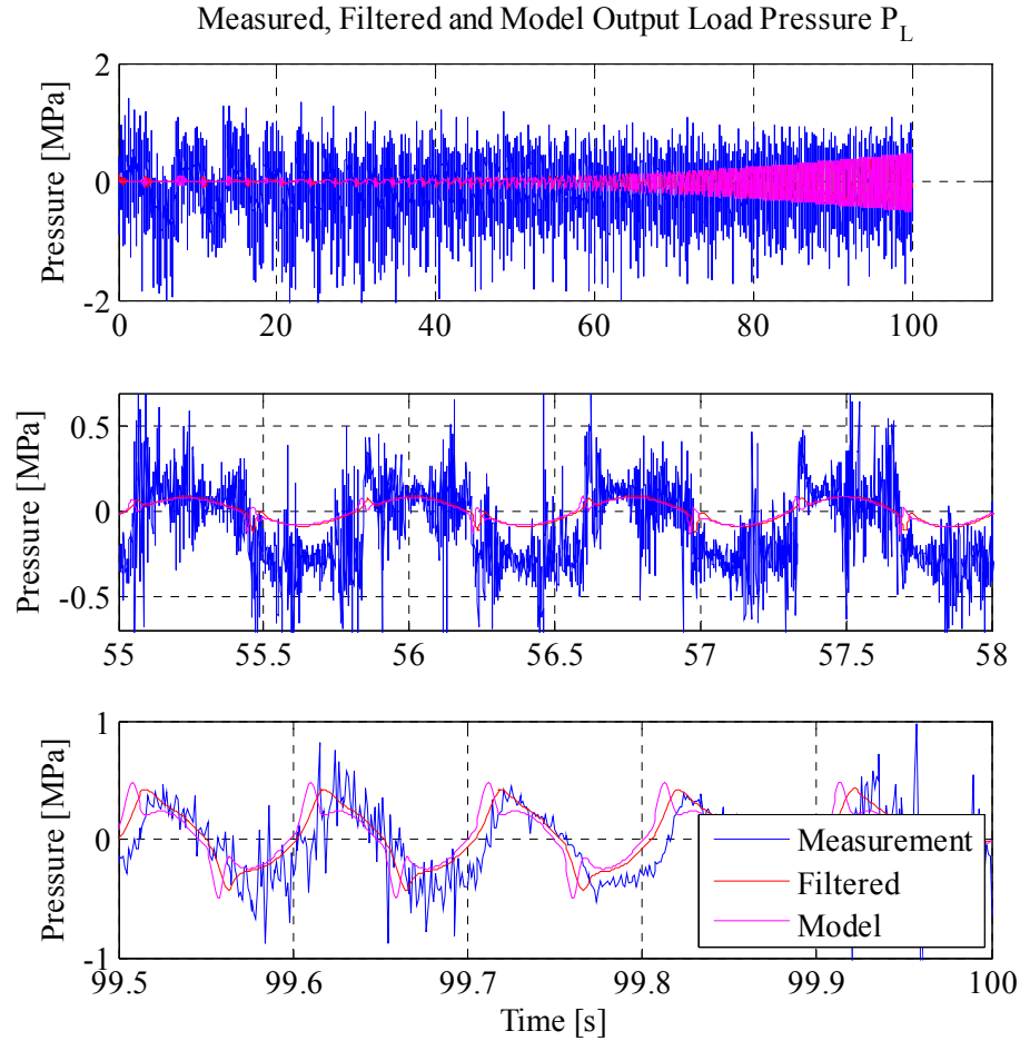
Figure 5-31 Valve Controlled System Load Pressure Response
