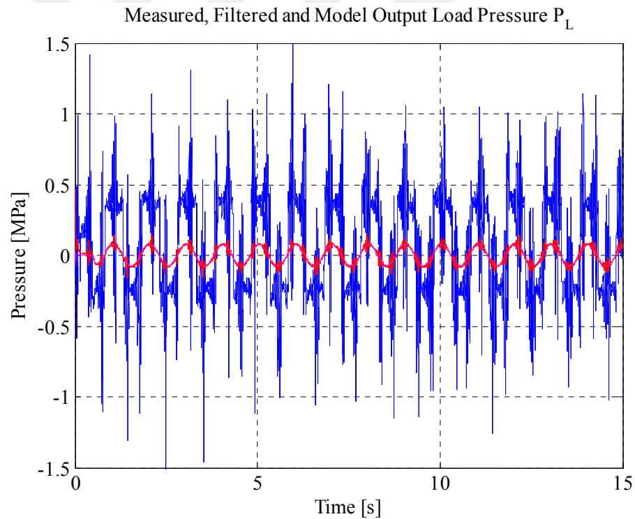
Figure 4-14 Kalman Filter Performance Load Pressure
