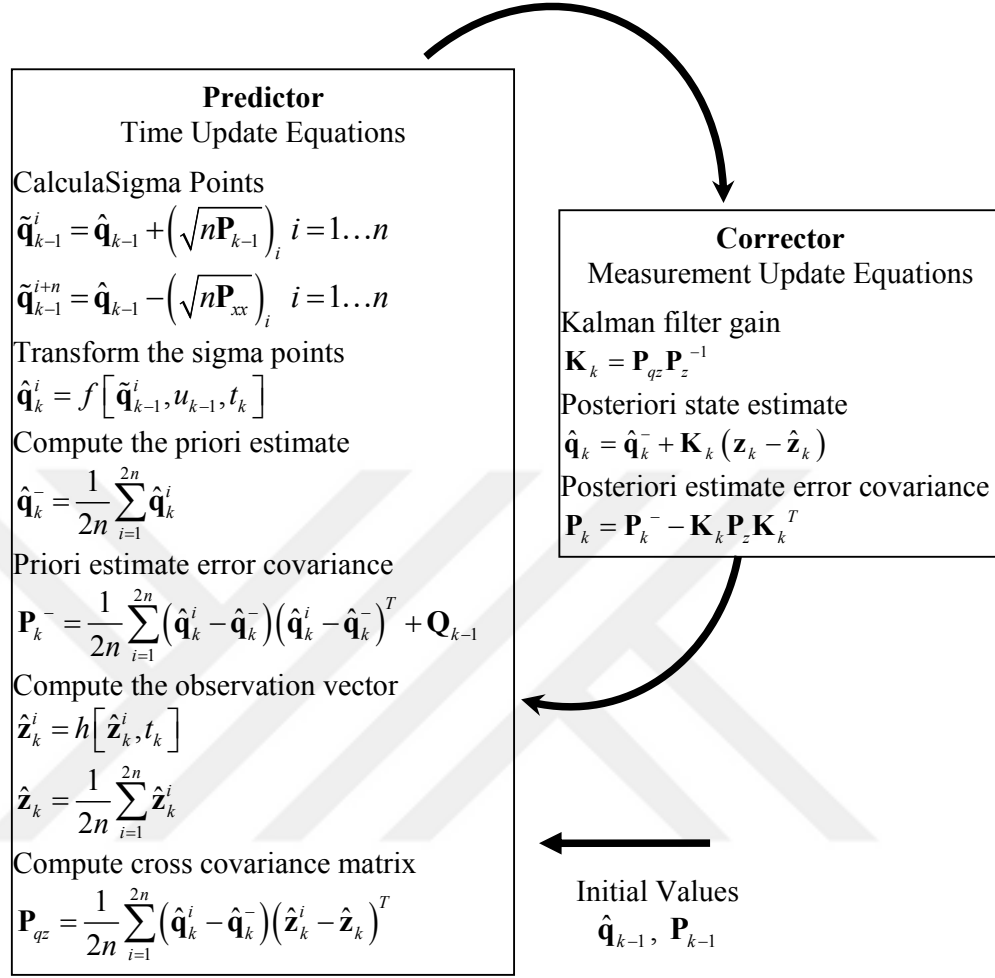
Figure 4-8 Unscented Kalman Filter Algorithm
