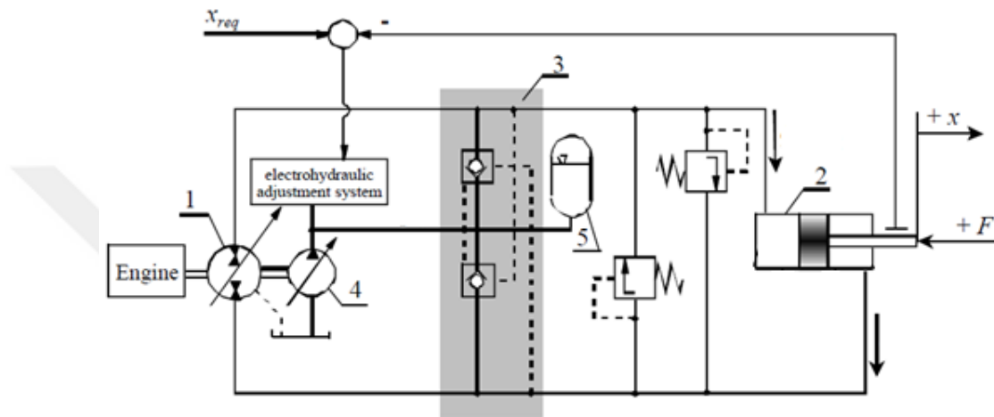
Figure 2-12 Displacement Controlled Drive with Single Rod Cylinder in Position Control [7]
