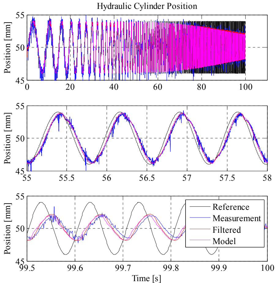
Figure 5-28 Valve Controlled System Position Response
