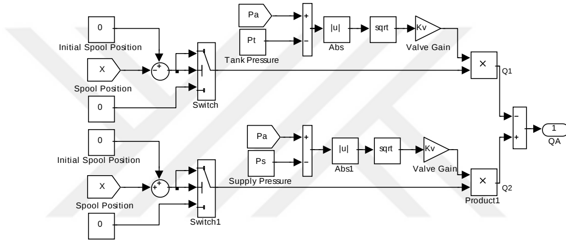
Figure 3-18 MATLAB Simulink Model of the Proportional Valve with Zero Lap
