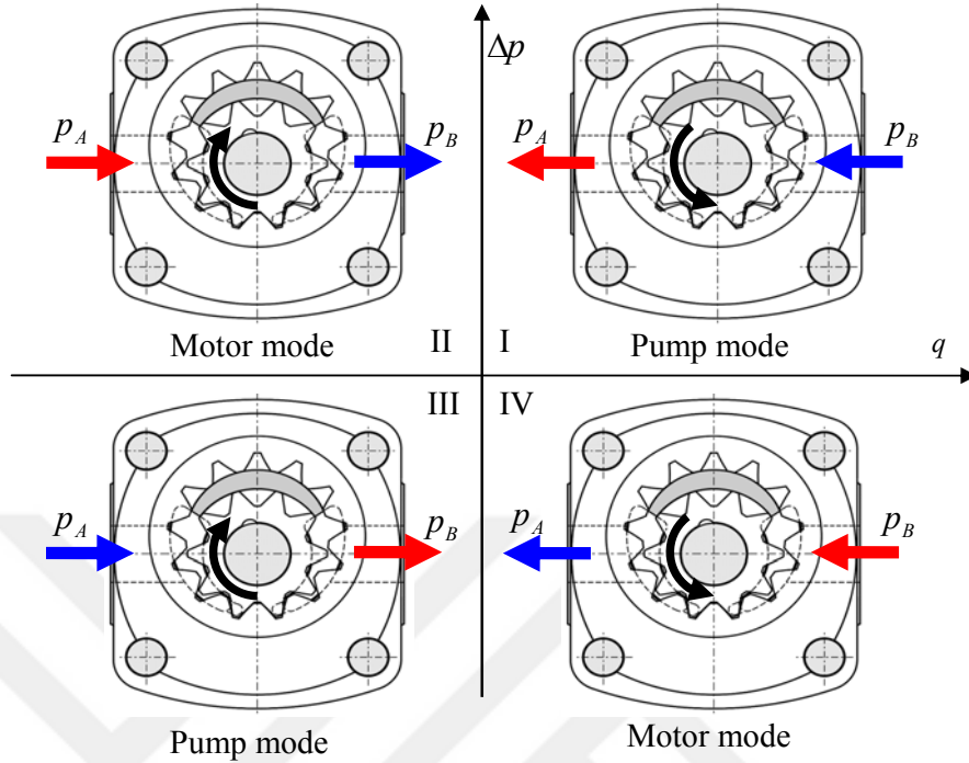
Figure 3-6 Hydraulic Pump Operation in 4 Quadrants
