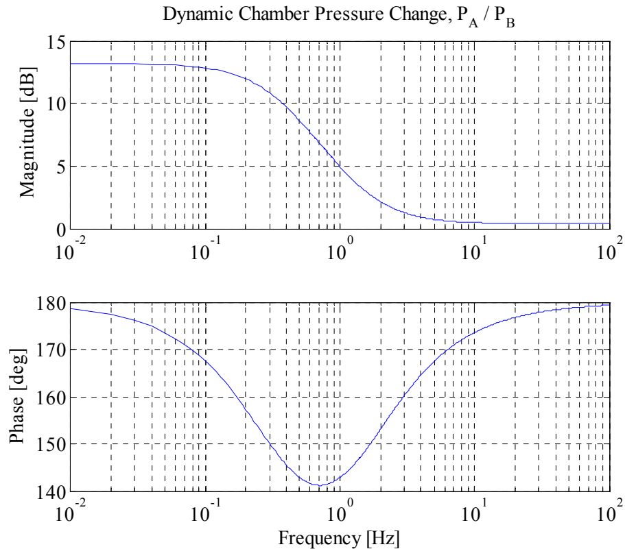
Figure 3-16 Pump Dynamic Chamber Pressure Change Relations
