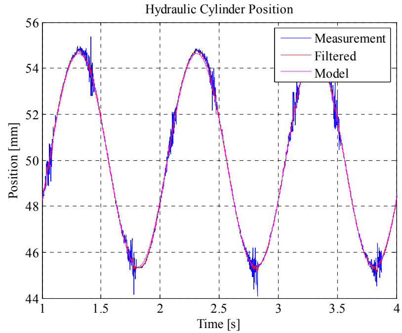
Figure 4-12 Kalman Filter Position Filtering Performance
