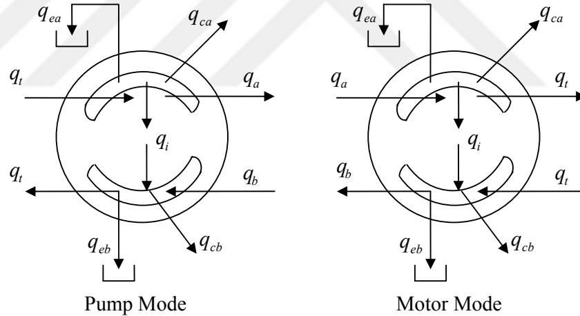
Figure 3-7 Representation of Flow Losses in Hydraulic Pumps and Motors [28]
