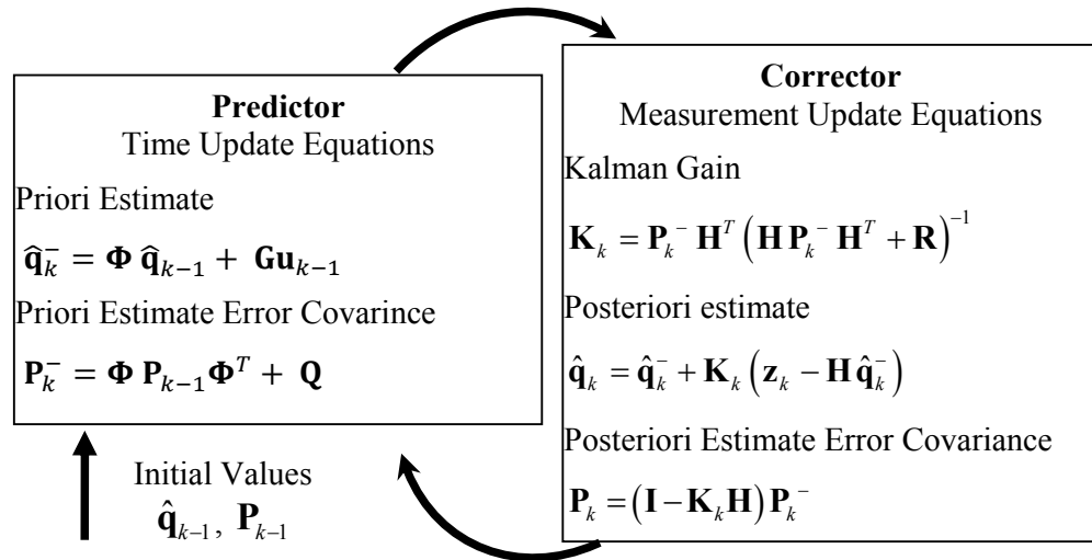
Figure 4-6 Kalman Filter Algorithm
