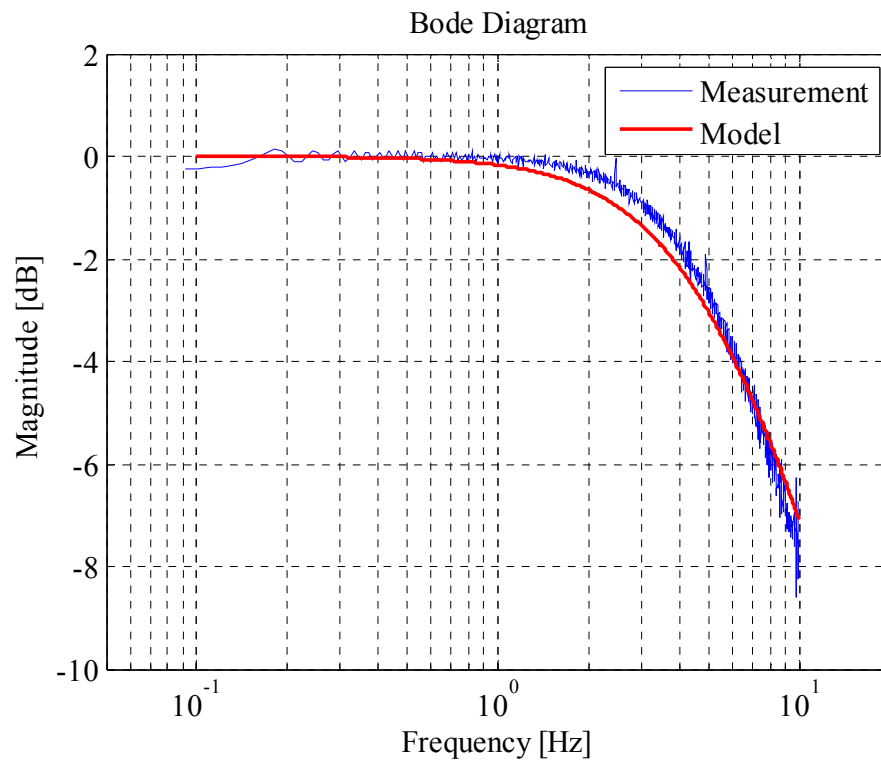
Figure 5-23 Magnitude Plot of the Experimental and Theoretical Frequency Response of Pump Controlled System with Desired Dominant Pole Located at -5.2\pi rad/s
