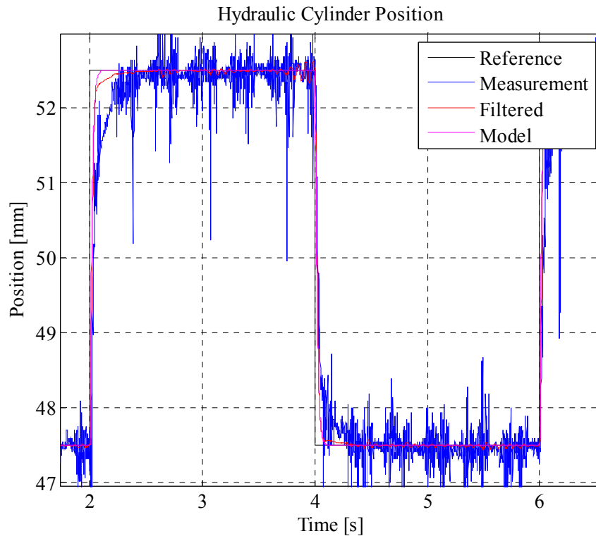
Figure 5-12 Step Response of the Valve Controlled System with Dominant Desired Closed Loop Pole Located at -10.2\pi rad/s
