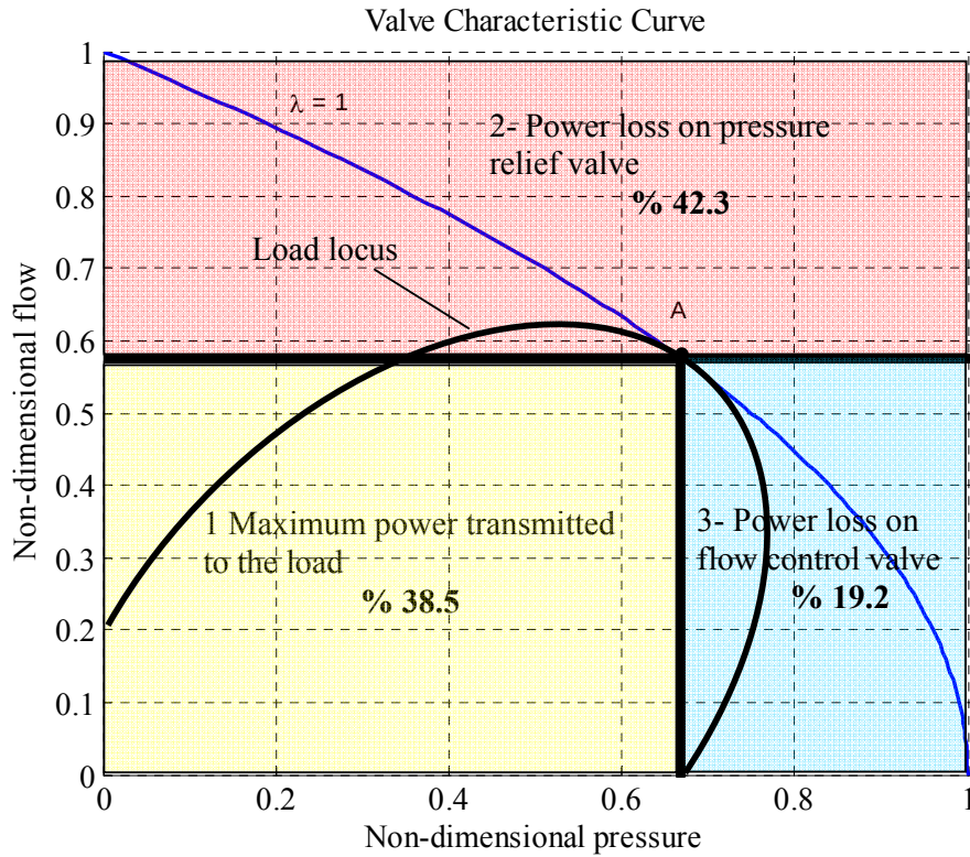
Figure 2-4 Valve Losses of a Constant Pressure Valve Controlled Circuit for Maximum Energy Efficiency
