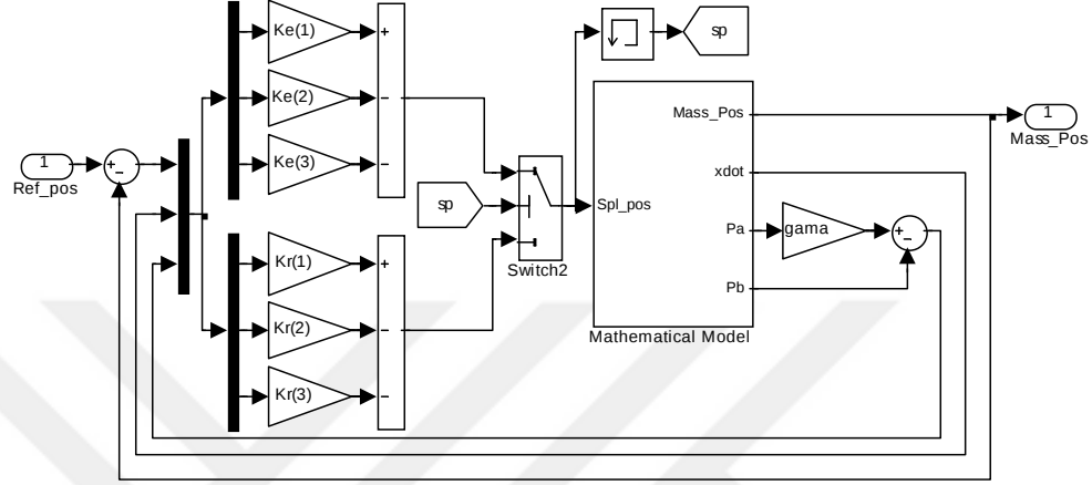
Figure 4-4 MATLAB Simulink Model of the Closed Loop Valve Controlled Position Control System
