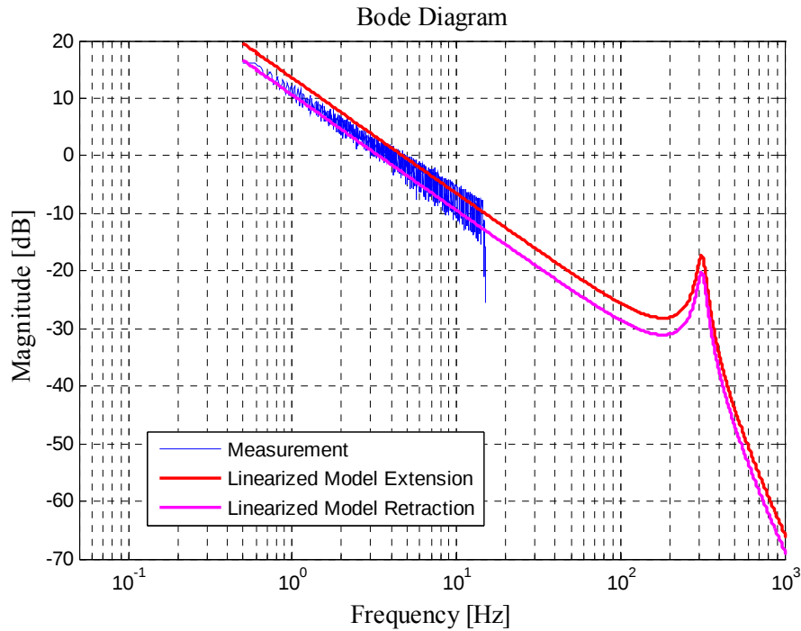
Figure 5-26 Magnitude Plot of the Experimental and Theoretical Open Loop Frequency Response of the Valve Controlled System
