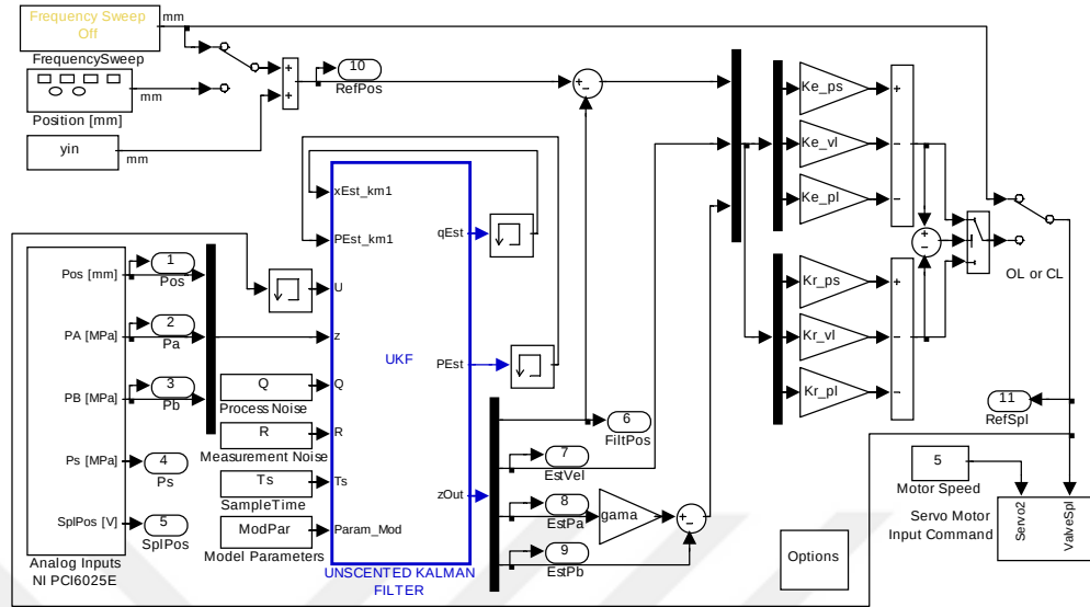
Figure 5-2 MATLAB Simulink RTWT Controller of the Valve Controlled System
