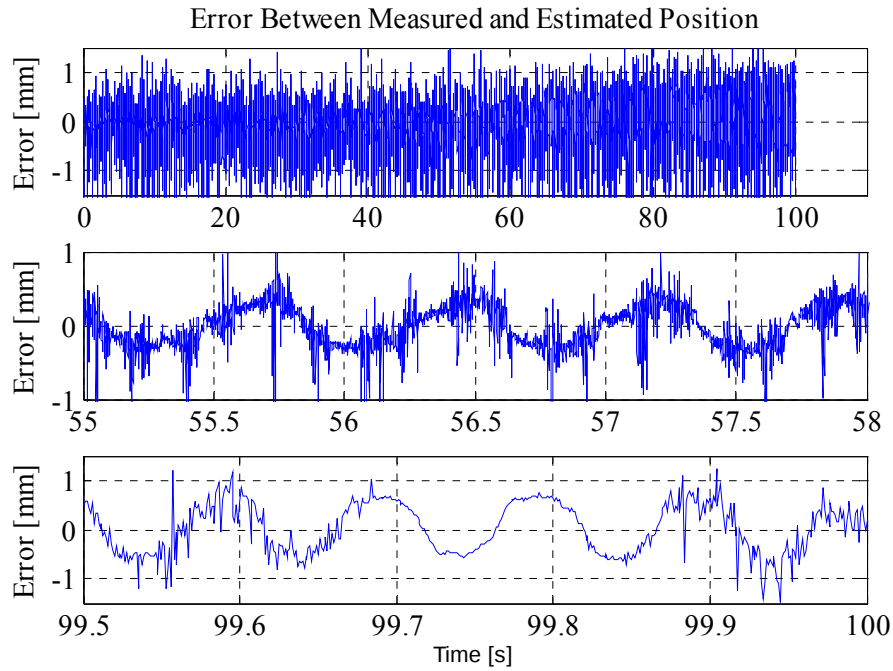
Figure 5-29 Valve Controlled System Error Between the Measured and Filtered Position Signal
