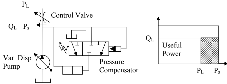
Figure 2-5 Pressure Compensated Pump [23]
