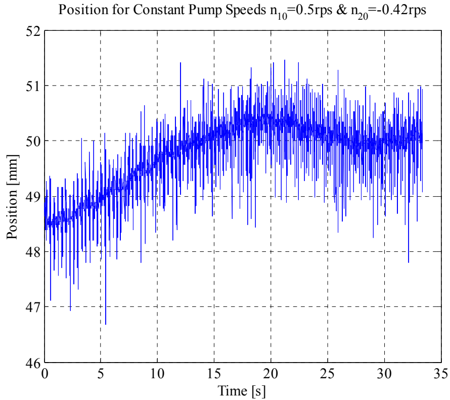
Figure 5-4 Steady State Cylinder Position for the Given Offset Pump Speeds
