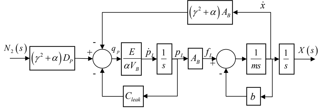
Figure 3-15 Block Diagram Representation of the Open Loop Position Response of the Variable Speed Pump Controlled System
