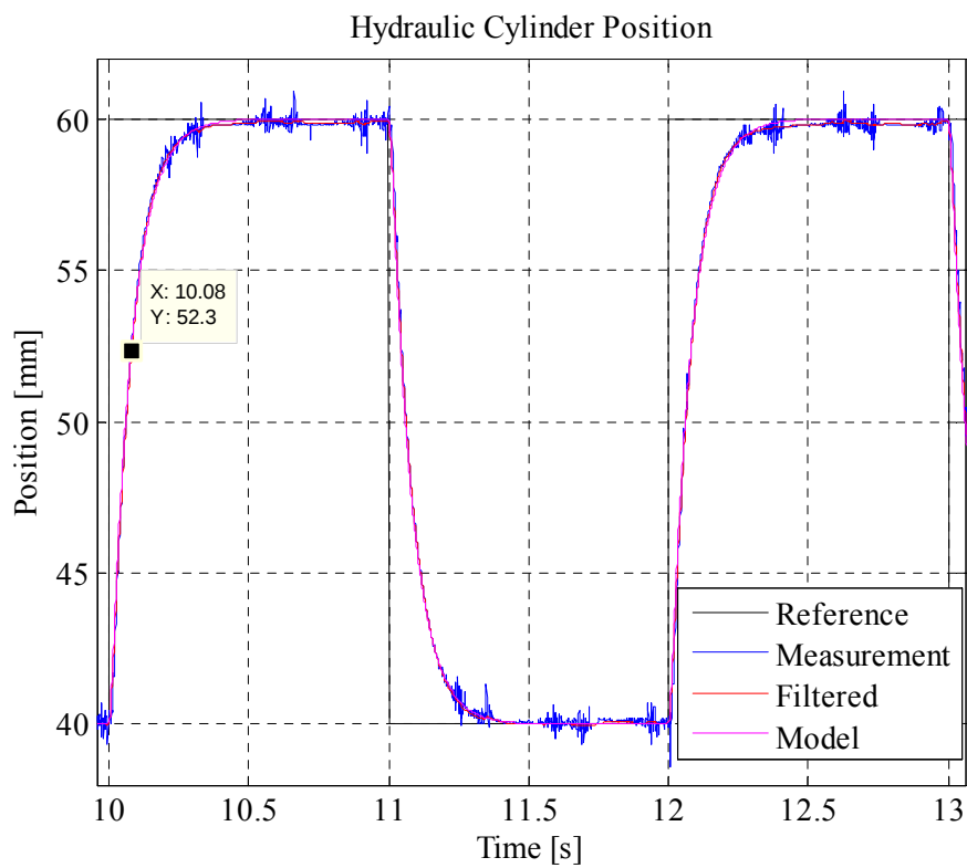
Figure 5-9 Step Response of the Pump Controlled System with Dominant Desired Closed Loop Pole Located at -2 \cdot 2\pi rad/s
