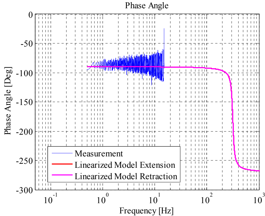
Figure 5-27 Phase Plot of the Experimental and Theoretical Open Loop Frequency Response of the Valve Controlled System
