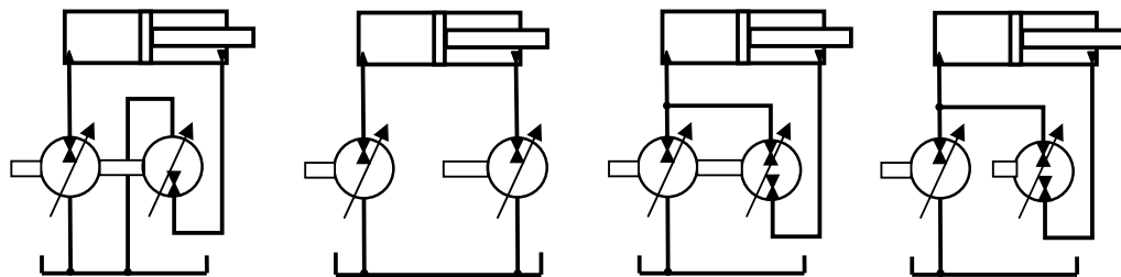
Figure 2-15 Two Pump Control Circuit Configurations
