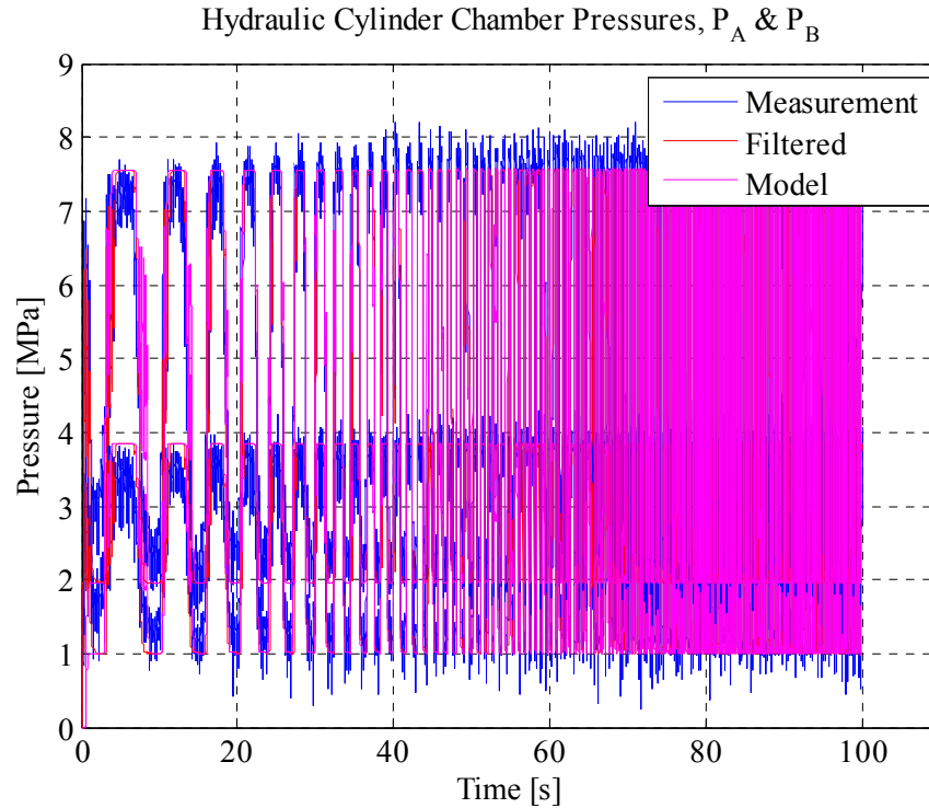
Figure 5-30 Valve Controlled System Hydraulic Cylinder Chamber Pressure Response
