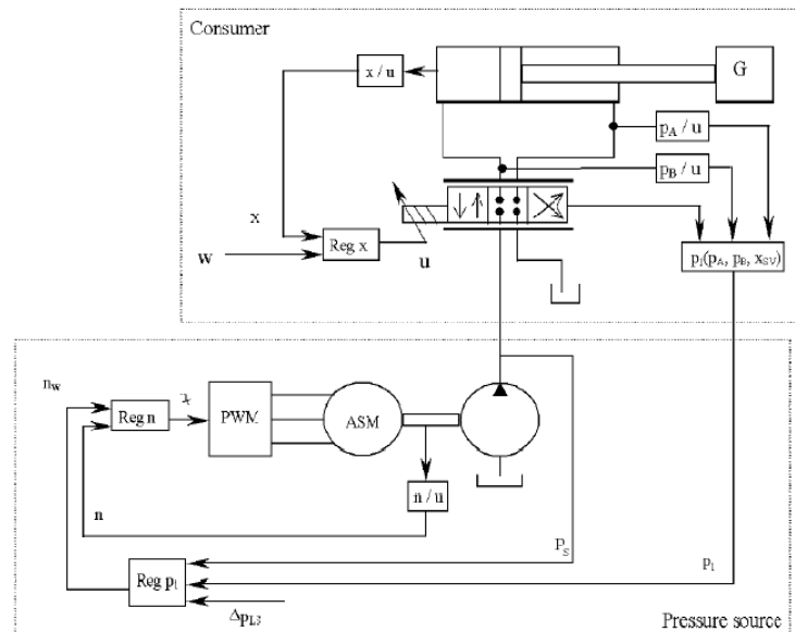
Figure 2-7 Electro-Hydraulic Load Sensing System with Constant Displacement Pump [8]
