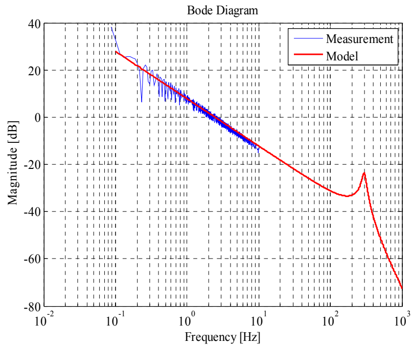
Figure 5-15 Experimental and Theoretical Open Loop Frequency Response of the Pump Controlled System
