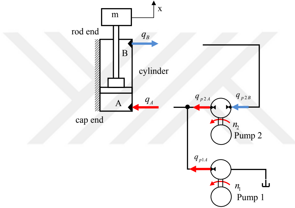
Figure 3-8 Flow Rates of the Hydraulic Cylinder and Pumps
