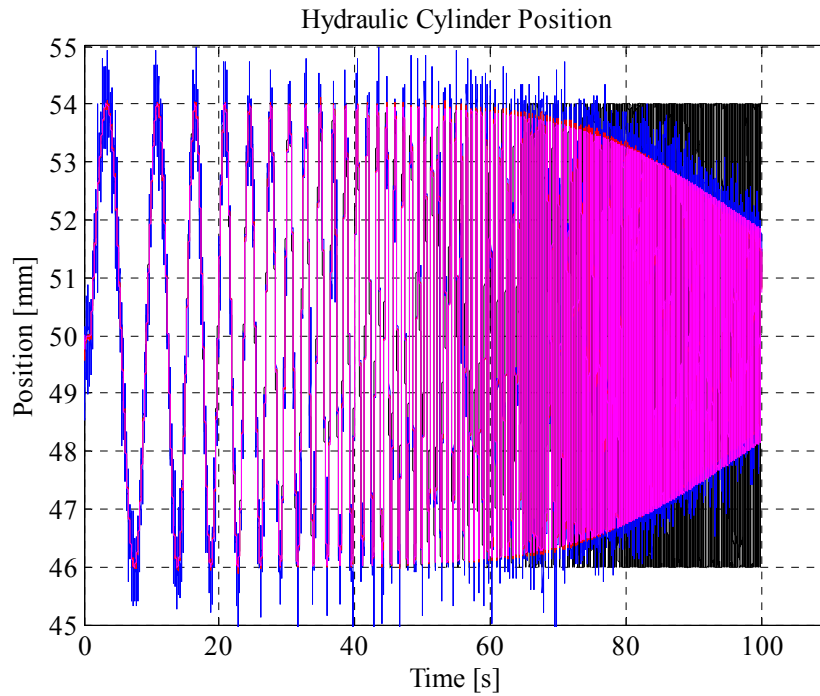
Figure 5-17 Position Response of Pump Controlled System
