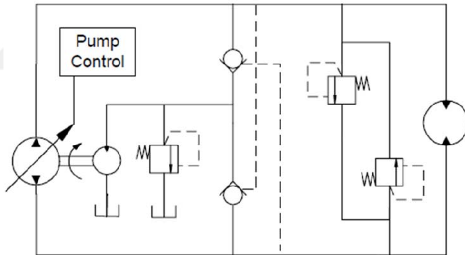
Figure 2-10 Hydrostatic Transmission System with Variable Displacement Pump Control Technique
