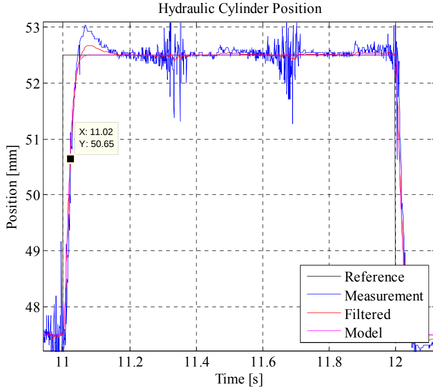
Figure 5-10 Step Response of the Pump Controlled System with Dominant Desired Closed Loop Pole Located at -10.2\pi rad/s
