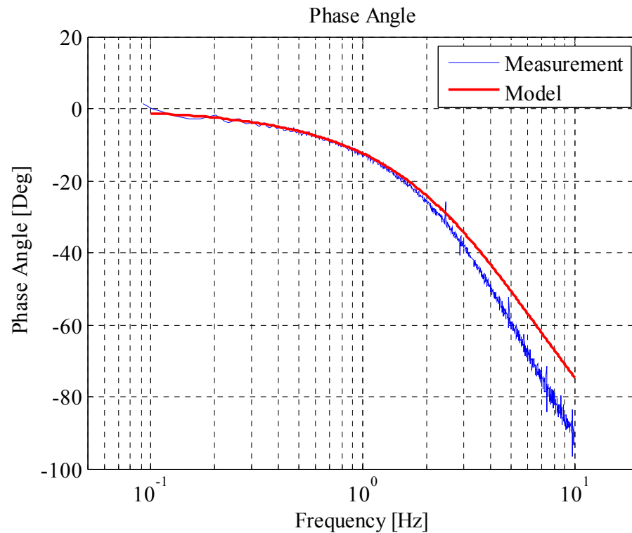
Figure 5-24 Phase Plot of the Experimental and Theoretical Frequency Response of Pump Controlled System with Desired Dominant Pole Located at -5.2\pi rad/s
