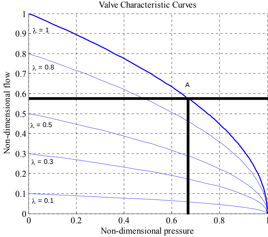
Figure 2-3 Valve Characteristic Curves for Different Valve Openings
