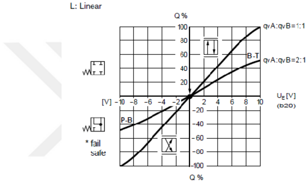
Figure 3-4 Flow Rate versus Valve Spool Position Signal of the Servo Solenoid Valve [27]
