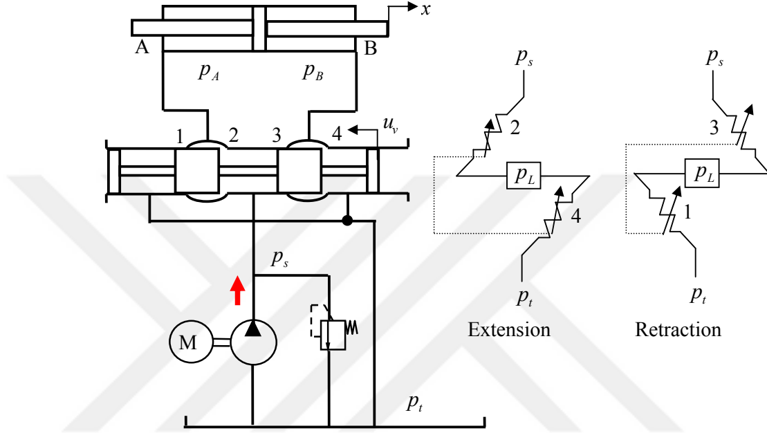
Figure 2-2 Constant Pressure Valve Controlled Hydraulic Circuit
