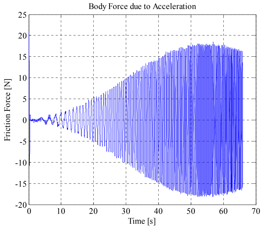
Figure 5-8 Body Force due to Acceleration
