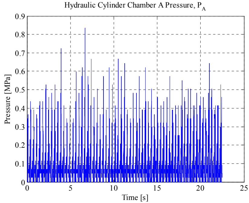
Figure 4-11 Hydraulic Cylinder Chamber A Pressure Transducer Measurement for Zero Reference Signal
