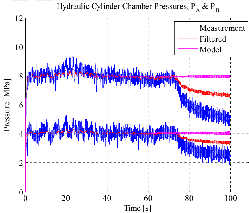
Figure 5-20 Pressure Response
