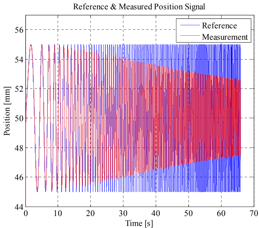
Figure 5-5 Friction Test Signal and System Response
