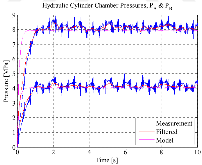
Figure 4-13 Kalman Filter Pressure Filtering Performance
