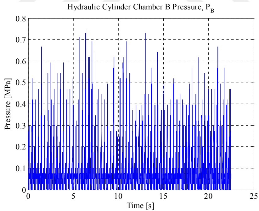
Figure 4-10 Hydraulic Cylinder Chamber B Pressure Transducer Measurement for Zero Speed
