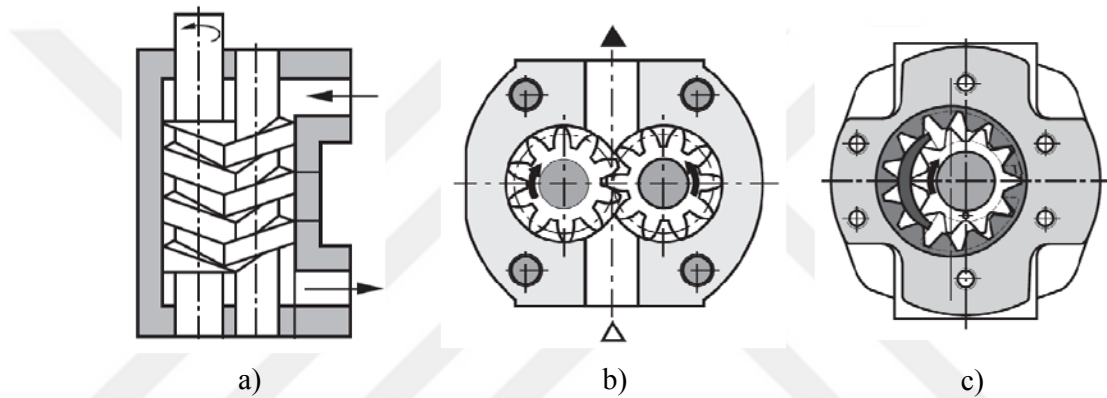
Figure 2-13 Constant Displacement Pump Types a) Screw Type, b) External Gear, c) Internal Gear
