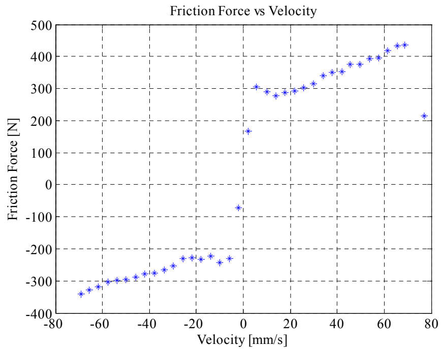
Figure 5-7 Mean Friction Force vs Cylinder Velocity
