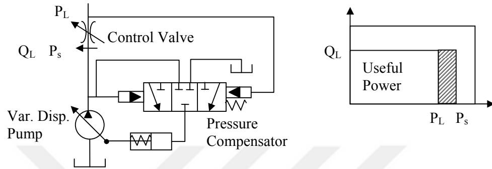
Figure 2-6 Load Sensing Pump Schematic [23]
