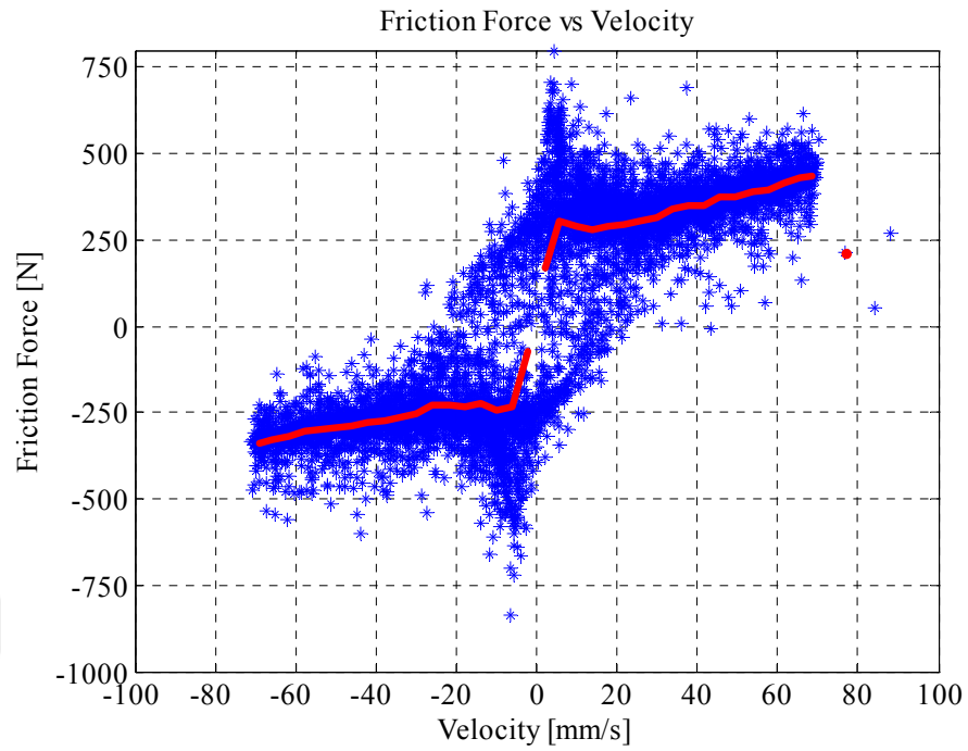
Figure 5-6 Friction Force vs Cylinder Velocity
