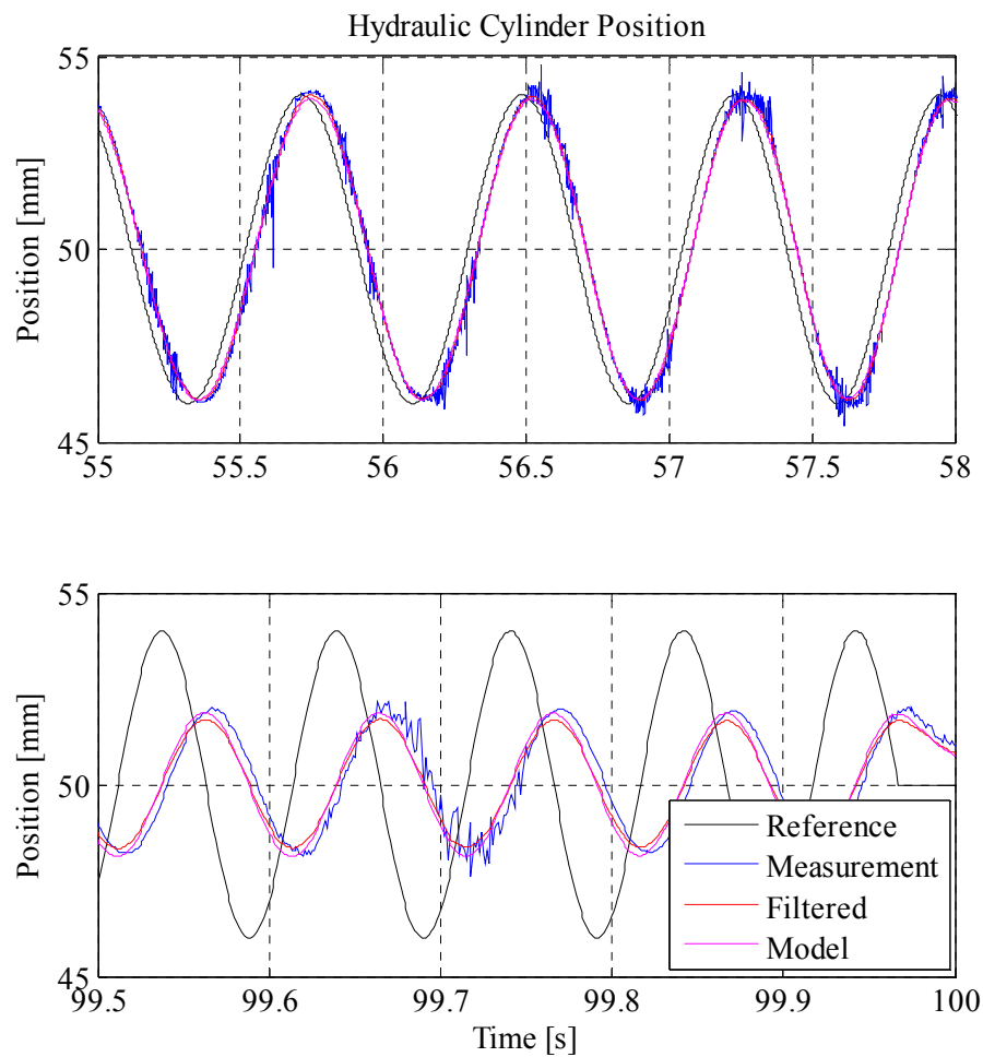
Figure 5-18 Detailed View of Position Response of Pump Controlled System
