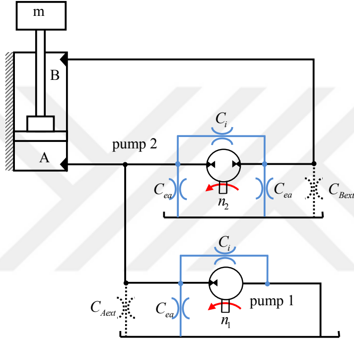
Figure 3-14 Representation of the Hydraulic Pump Leakages with Additional External Leakages
