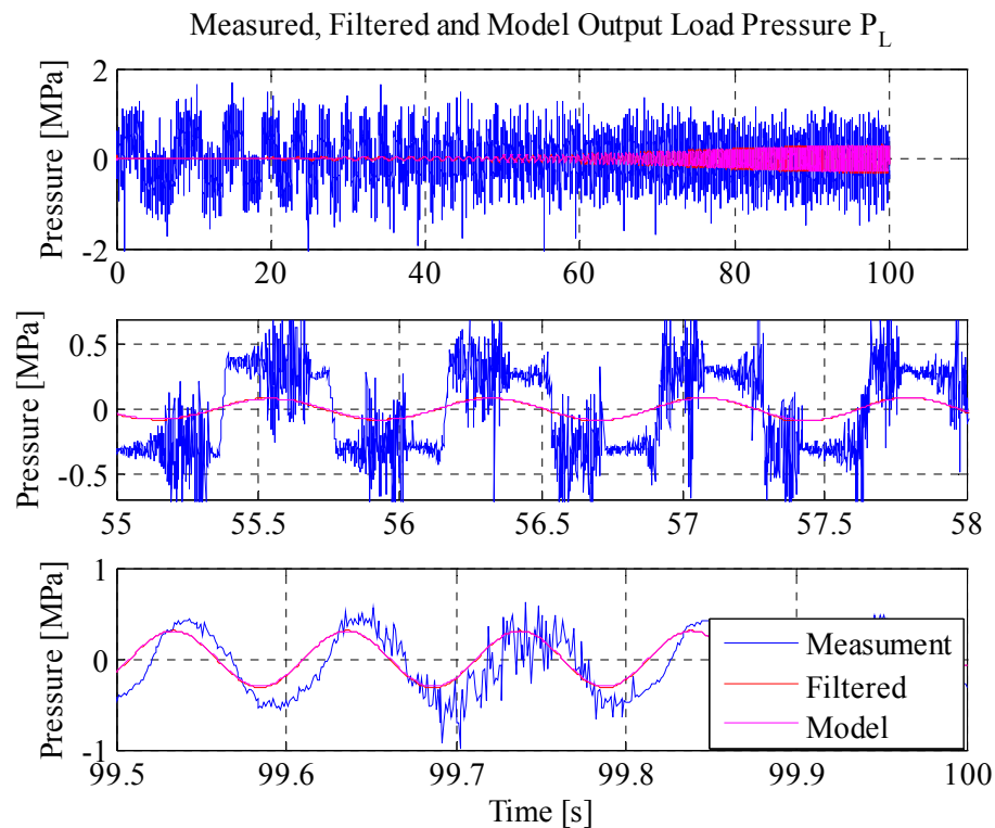
Figure 5-22 Load Pressure
