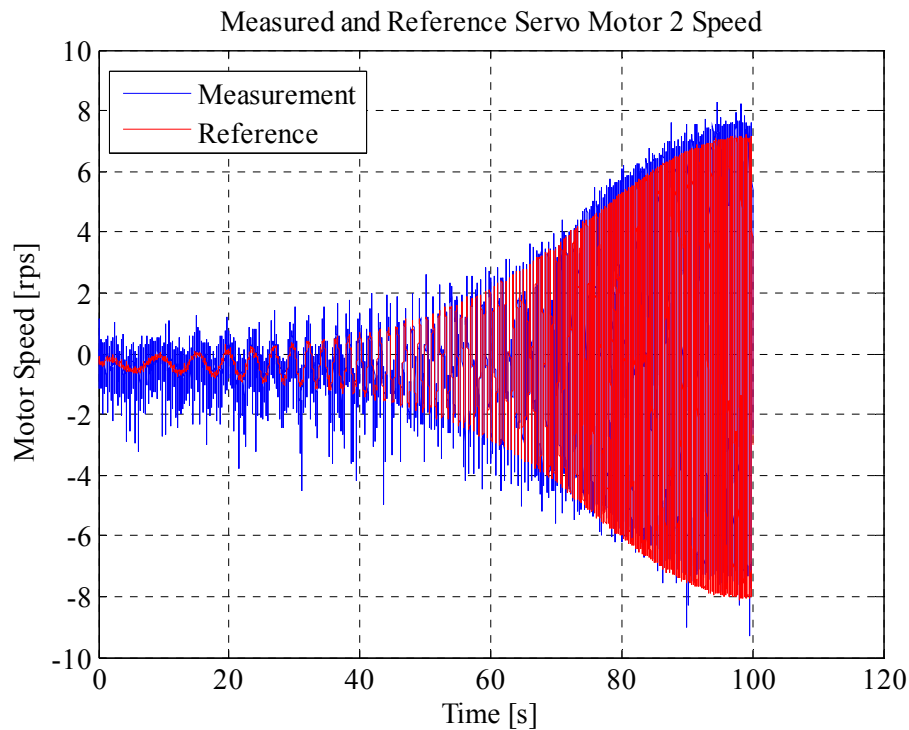
Figure 5-21 Servomotor Response
