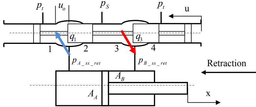
Figure 3-20 Schematic Representation of the Valve Spool Opening for Retraction
