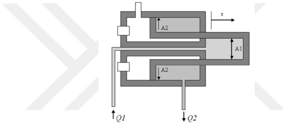
Figure 2-11 Single Rod Symmetric Linear Actuator [25]
