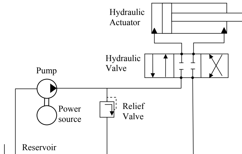
Figure 2-1 Conventional Valve Controlled Hydraulic Circuit
