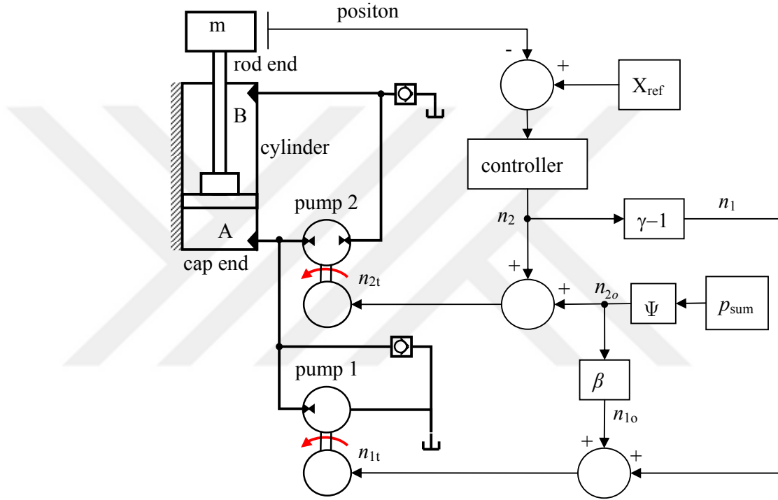
Figure 3-5 Variable Speed Pump Control Circuit
