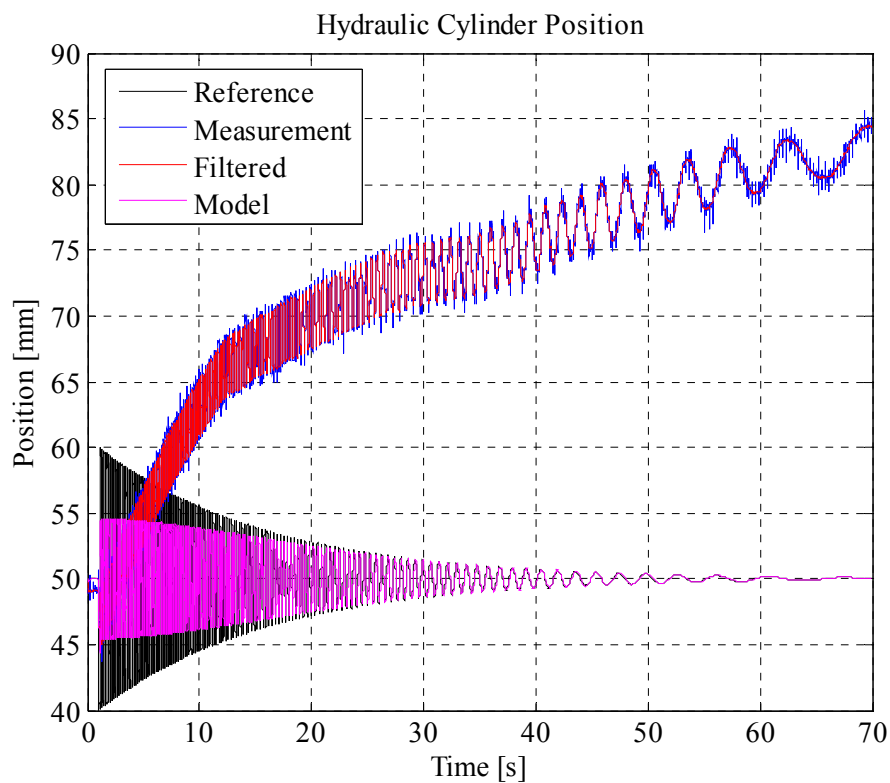
Figure 5-16 Hydraulic Cylinder Position in Open Loop Tests
