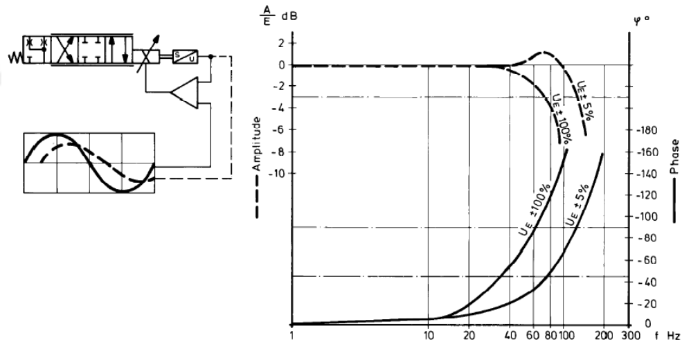
Figure 3-3 Servovalve Frequency Response Diagram [27]
