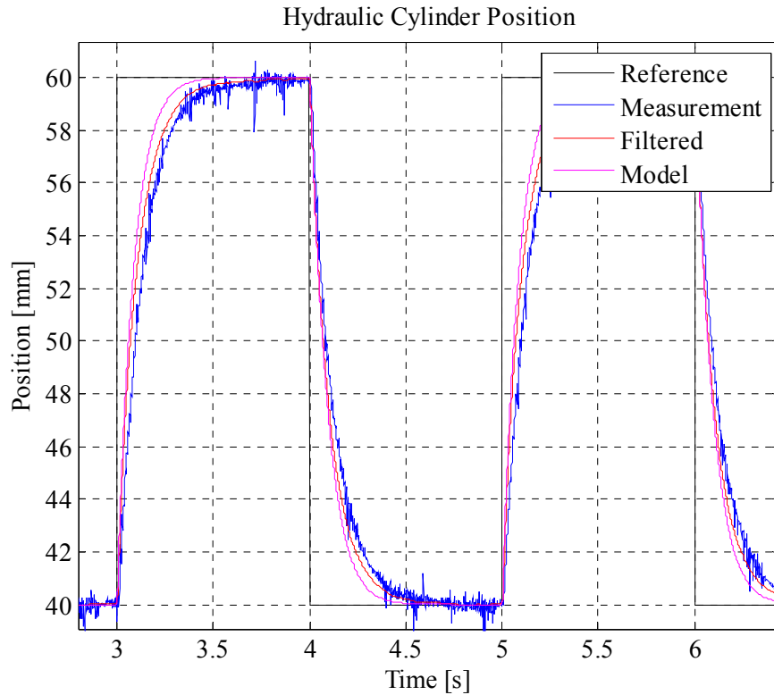
Figure 5-11 Step Response of the Valve Controlled System with Dominant Desired Closed Loop Pole Located at -2.2\pi rad/s
