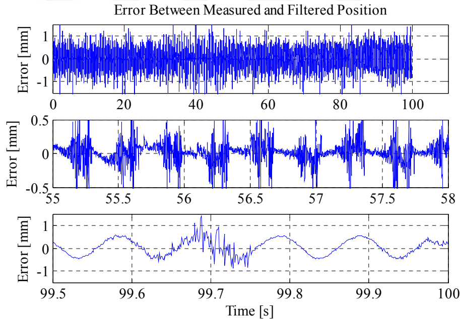
Figure 5-19 Error Between the Measured and Filtered Position Signal
