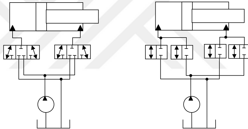
Figure 2-8 Individual Meter In Meter Out Valve Control System [24]
