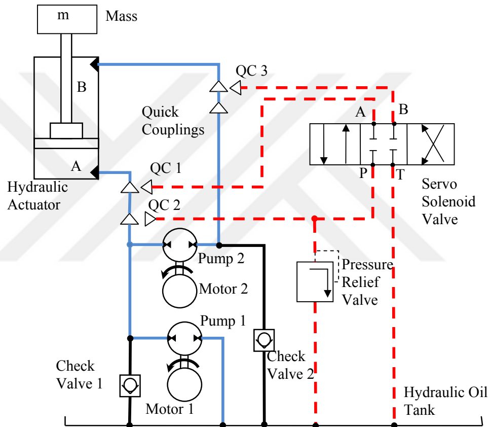
Figure 3-2 Schematic Diagram of the Experimental Test Set-Up
