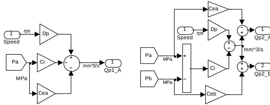
Figure 3-9 MATLAB Simulink Model of the Hydraulic Pump/Motor Unit
