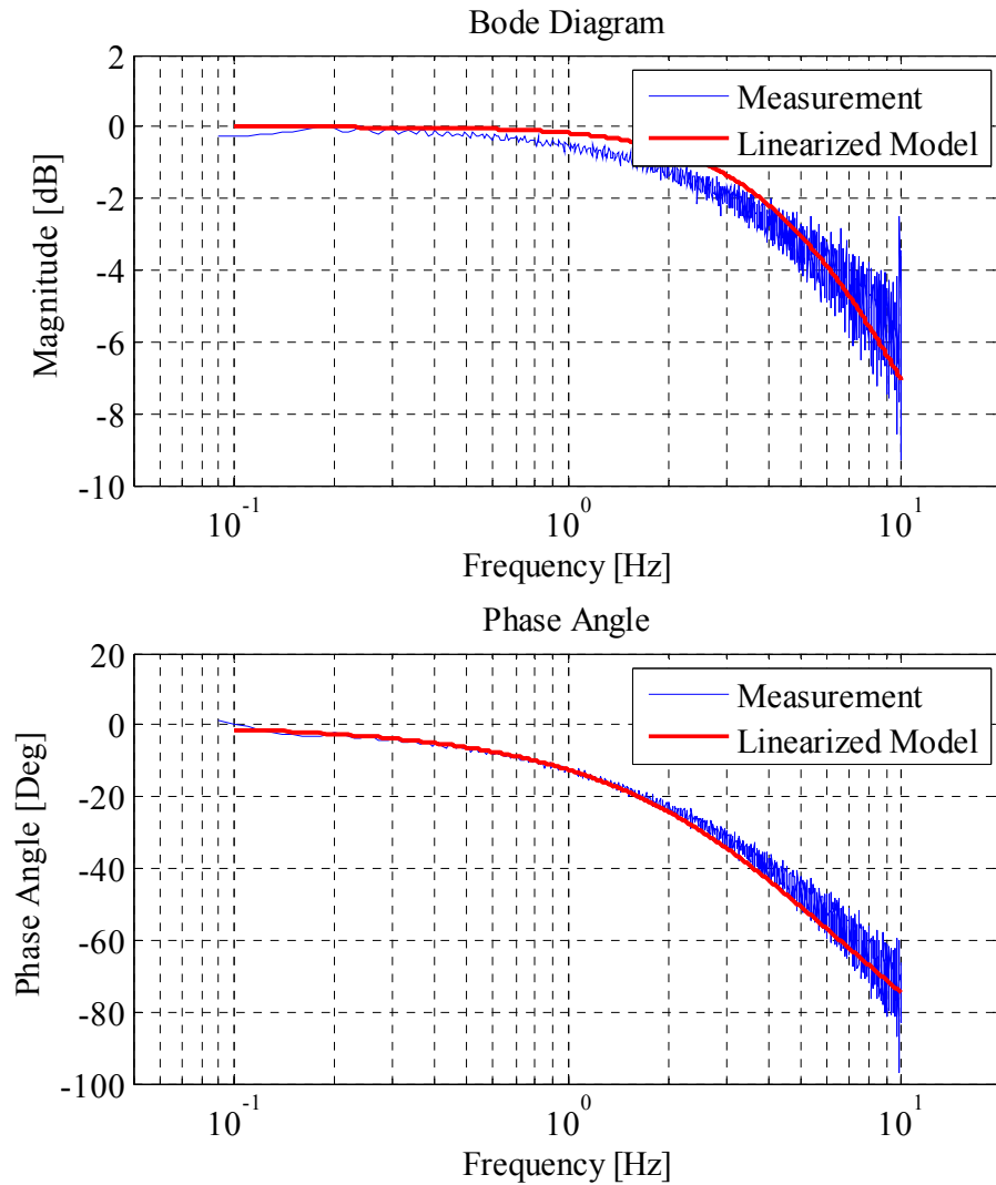
Figure 5-32 Experimental and Theoretical Frequency Response of Valve Controlled System with Desired Dominant Pole Located at -5.2\pi rad/s
