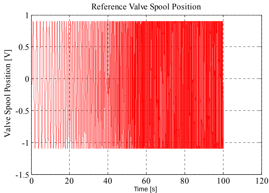
Figure 5-25 Test Signal for Valve Controlled System Open Loop Frequency Response
