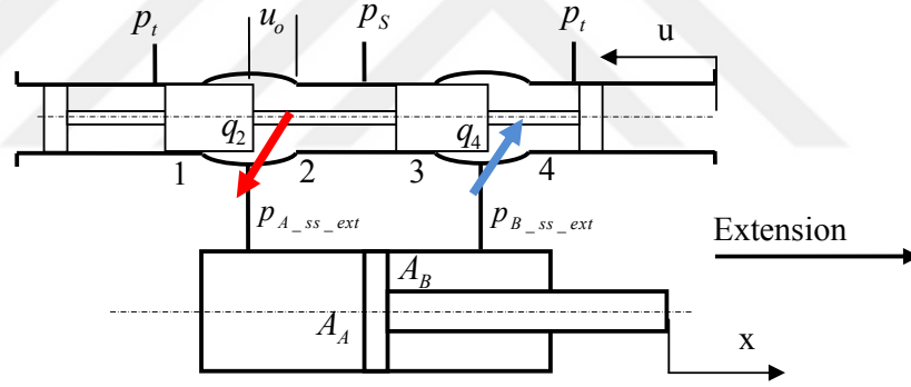
Figure 3-19 Schematic Representation of the Valve Spool Opening for Extension
