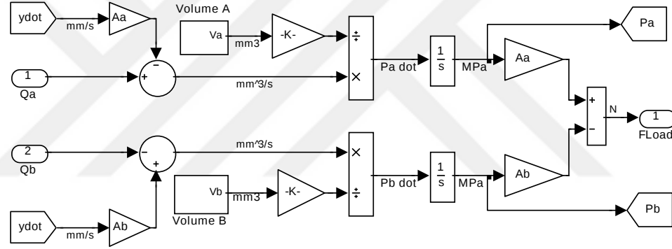
Figure 3-10 MATLAB Simulink Model of the Hydraulic Actuator
