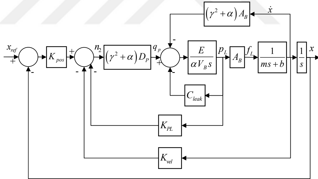
Figure 4-1 Block Diagram Representation of the Close Loop Pump Controlled System
