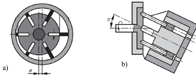
Figure 2-9 Variable Displacement Pumps a) Vane Pump, b) Piston Pump
