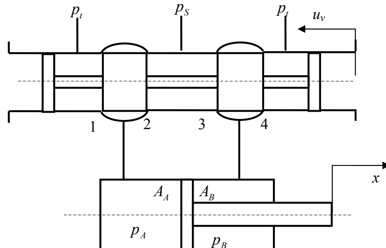
Figure 3-17 Schematic Representation of the Valve Controlled System
