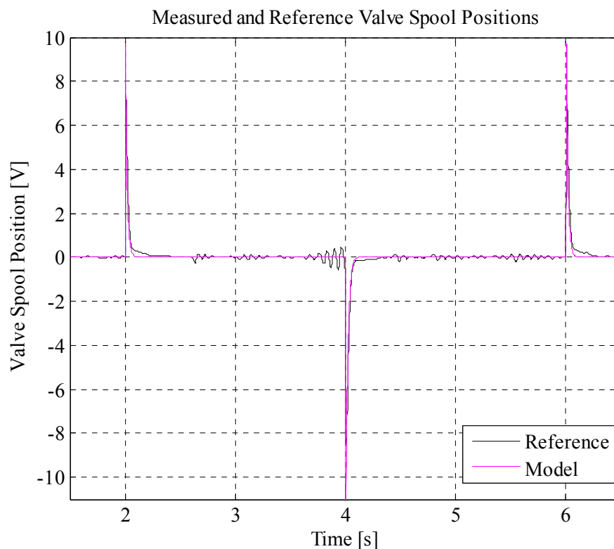
Figure 5-13 Real System Valve Spool Position Command and Simulink Model Spool Position Command
