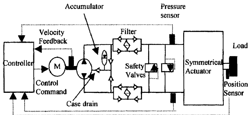
Figure 2-14 Electro Hydraulic Actuation System of Habibi and Goldenberg with Symmetric Actuator [3]
