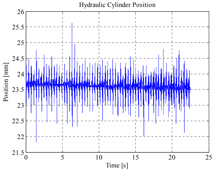
Figure 4-9 Position Transducer Measurement for Zero Reference Input
