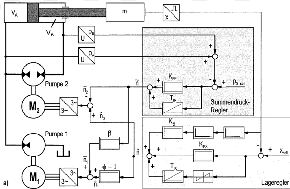
Figure 1-1 The Circuit Operation and Sum Pressure Principle [19]
