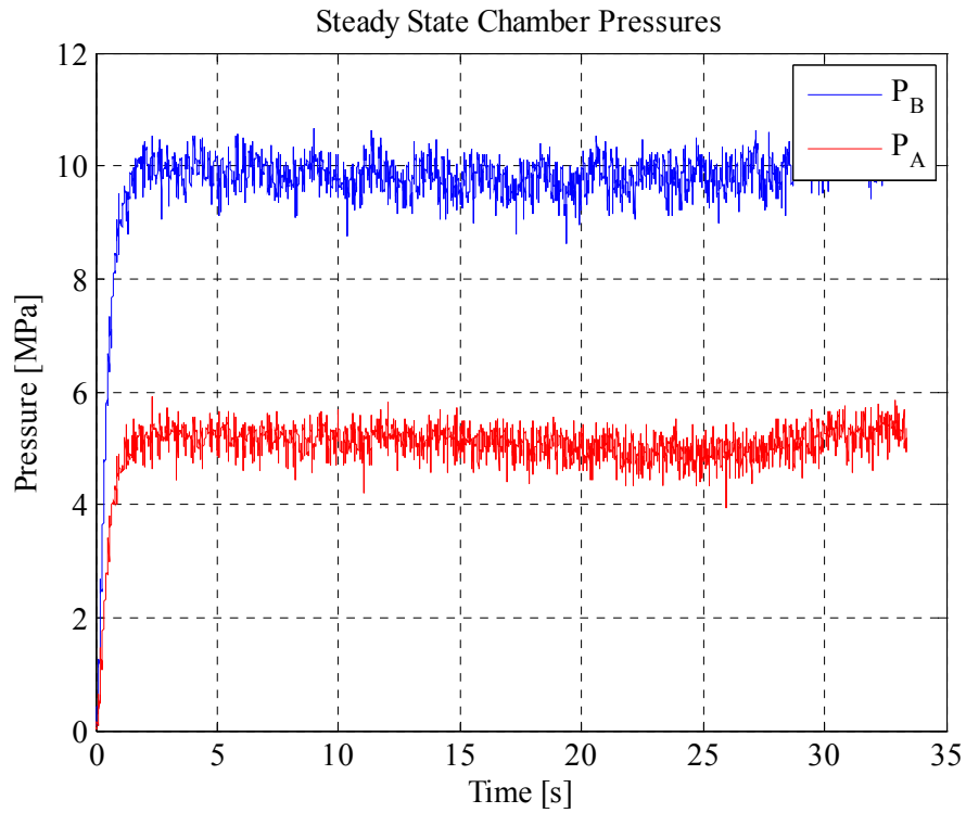
Figure 5-3 Steady State Chamber Pressures
