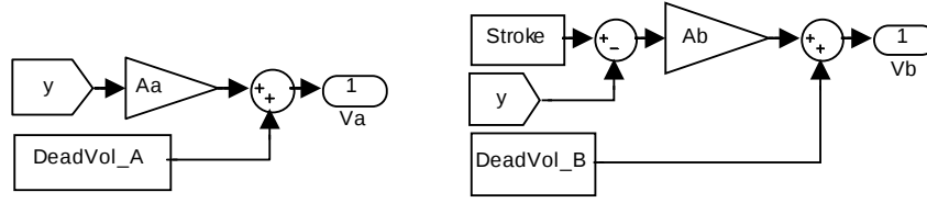
Figure 3-11 MATLAB Simulink Model of the Hydraulic Cylinder Chamber Volumes
