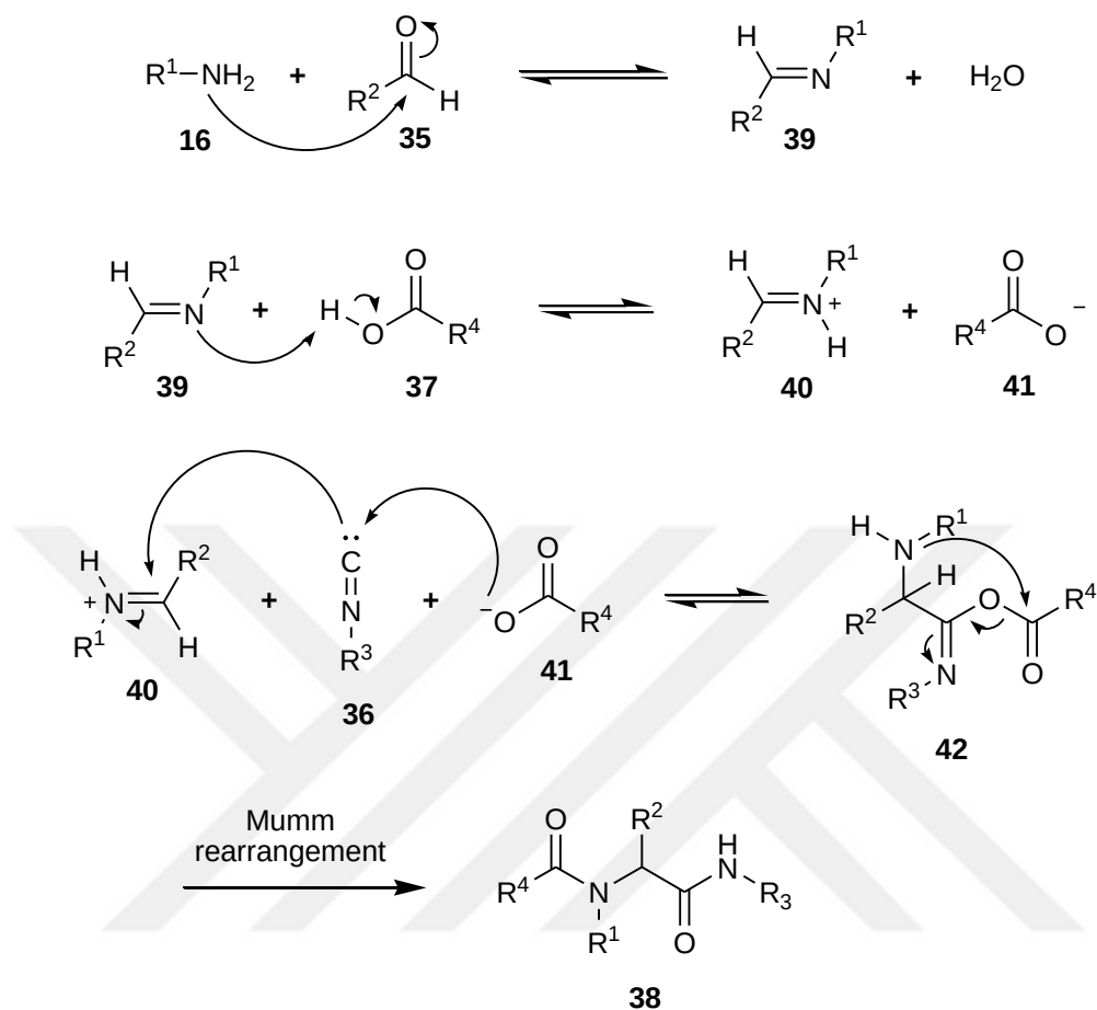
Scheme 10. Mechanism of the Ugi-4CR [40]
