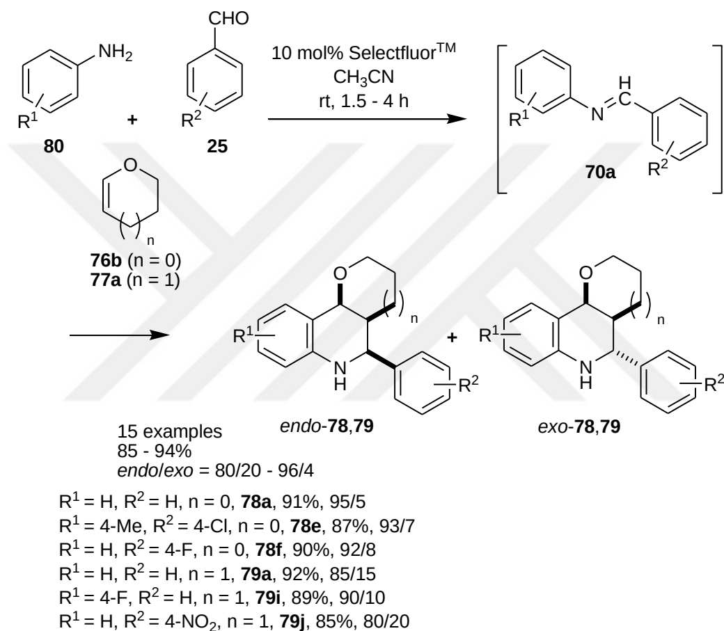
Scheme 31. Three component Povarov reaction in the presence of Selectfluor TM [65]
