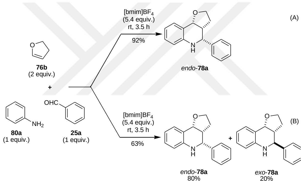
Scheme 46. Conflicting results for the Povarov reaction between 80a , 25a , and 76b . (A)
