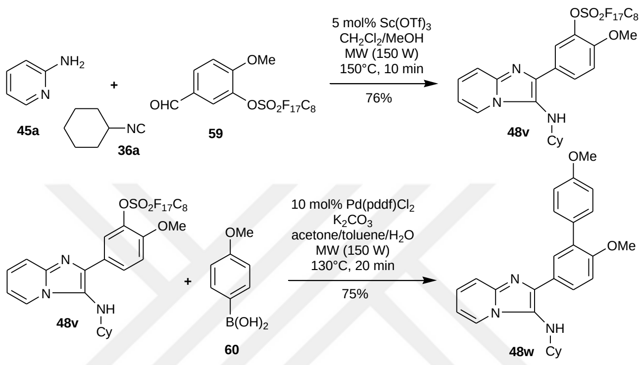
Scheme 20. Fluorous three component reaction and subsequent cross coupling reaction for the synthesis of the fused 3-aminoimidazole 48w [52]
