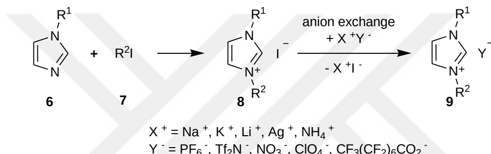
Scheme 1. Synthesis of 1,3-dialkylimidazolium salts 9 starting from 1-alkylimidazoles 6 [11]
