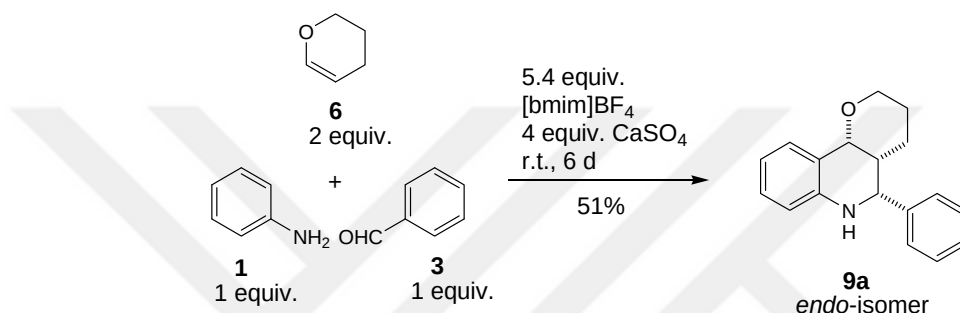
Scheme 3. [bmim]BF 4 promoted reaction between 1 , 3 and 2,3-dihydropyran ( 6 )
