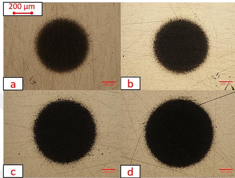
Figure 6-1 Optical microscopy images of the micro-abrasion wear scars for Ti-64 substrate after (a) 25, (b) 50, (c) 100, and (d) 200 ball revolution
