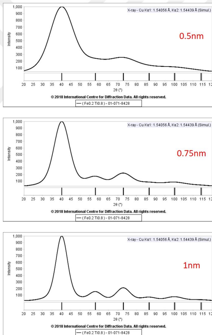
Figure 4-32 Simulated XRD profiles for \text{Ti}_{0.8}\text{Fe}_{0.2} for 0.5, 0.75 and 1 nm crystallite sizes
