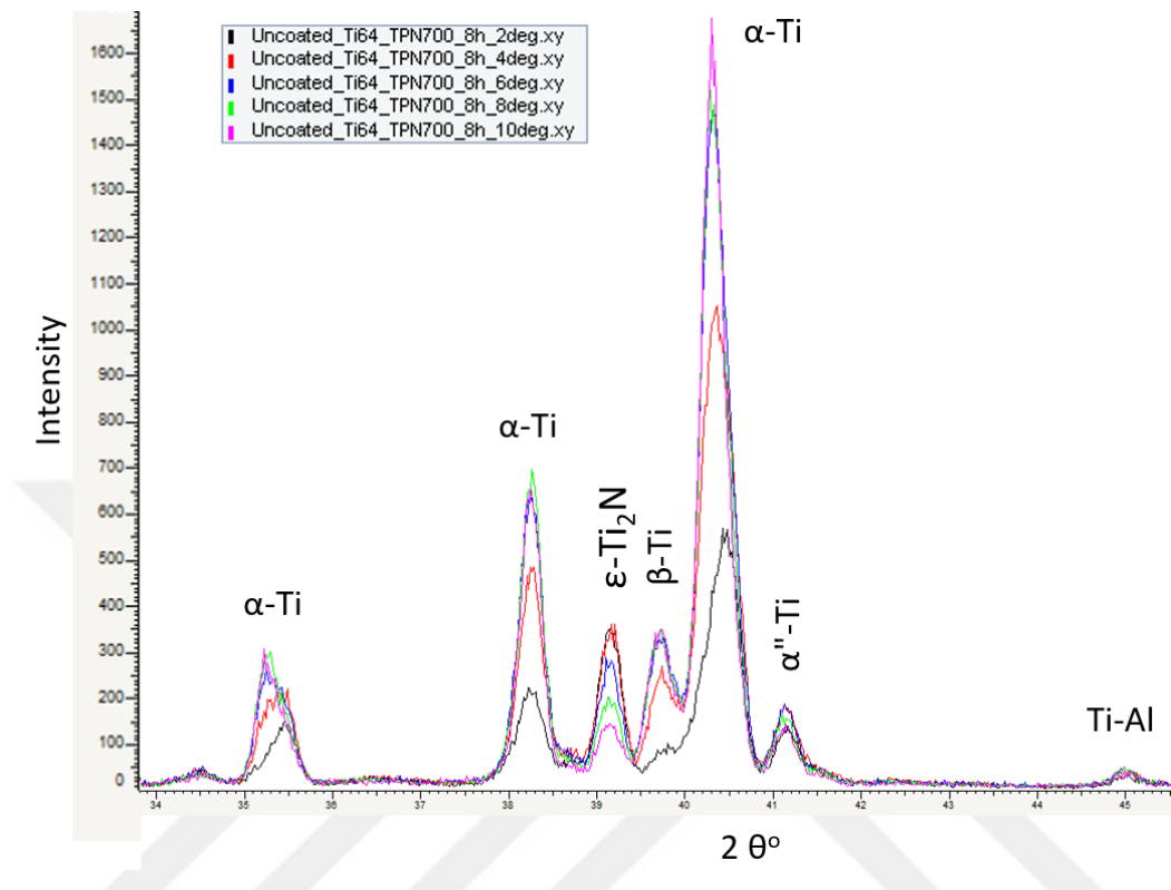
Figure 5-24 GAXRD (2° to 10° angle of incidence) diffraction patterns of uncoated Ti-64 substrate nitrided at 700°C for 8 hours
