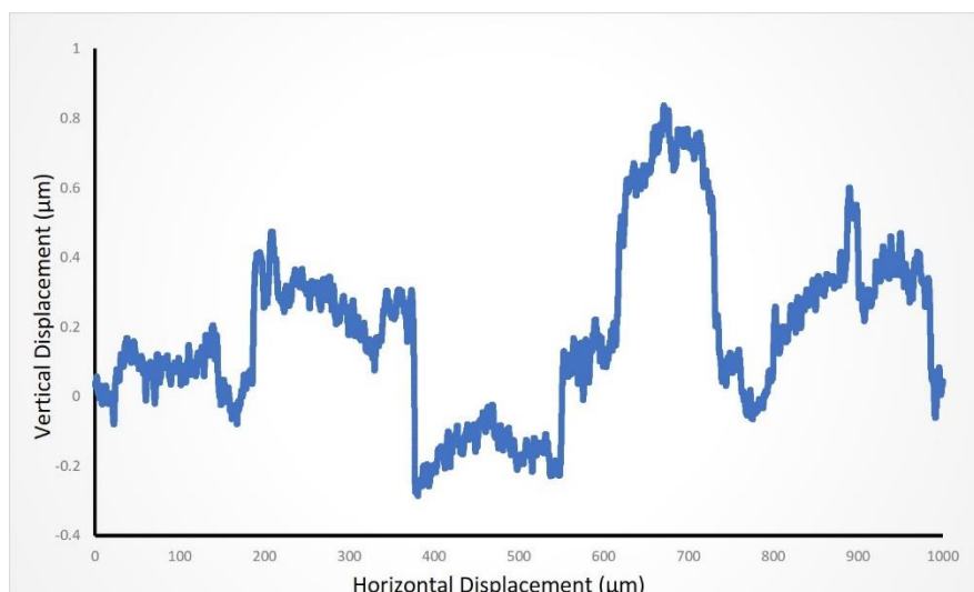
Figure 5-13 2D scan profile across the nitrided surface of the uncoated Ti-AVM sample
