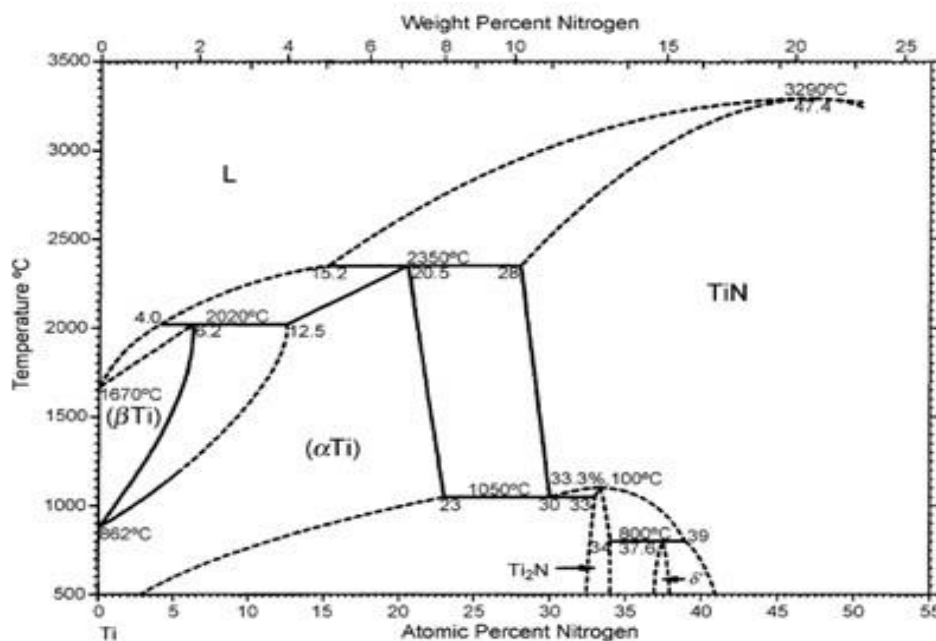
Figure 2-11 Ti-N phase diagram [56]
