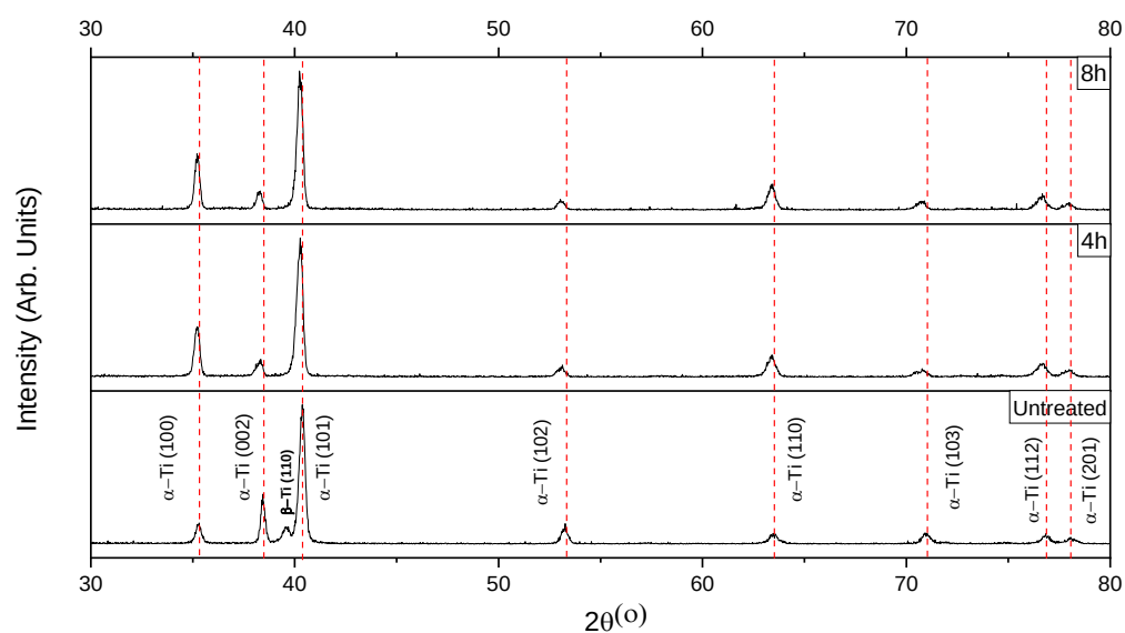
Figure 5-2 GAXRD ( 2^\circ angle of incidence) diffraction patterns of Ti-64 treated at 500°C for 4 and 8 hours
