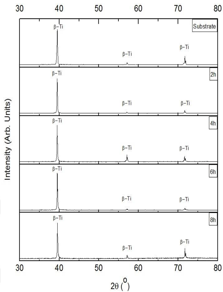
Figure 5-3 Theta-2theta diffraction patterns for untreated and nitrided Ti-AVM at 500°C
