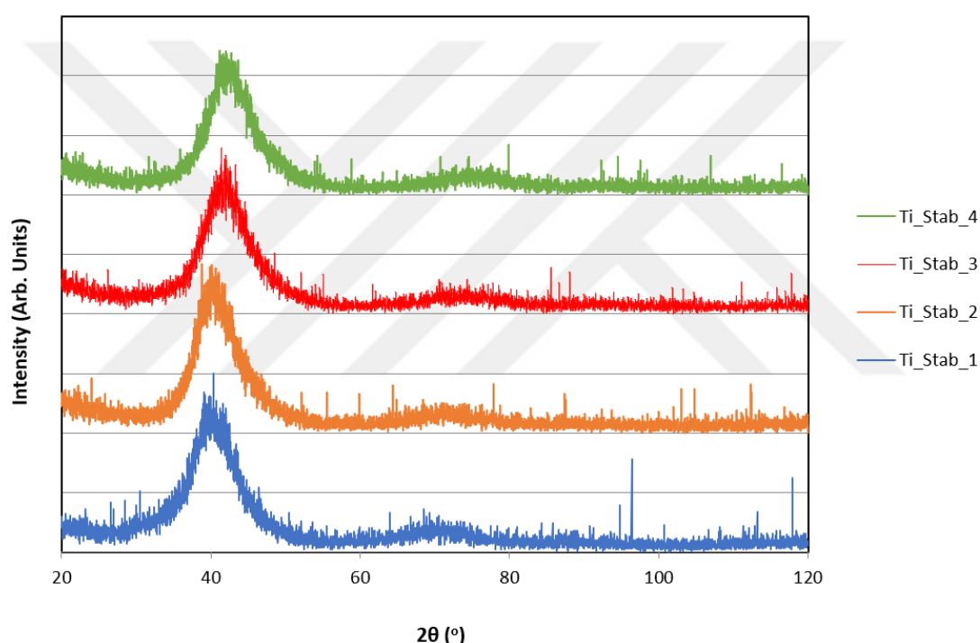
Figure 4-30 GAXRD (2° angle of incidence) diffraction patterns of the Ti-Stab alloy coatings
