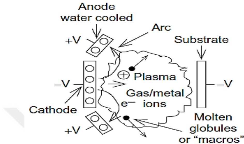
Figure 2-7 Components of Cathodic Arc Vapour Deposition System [31]
