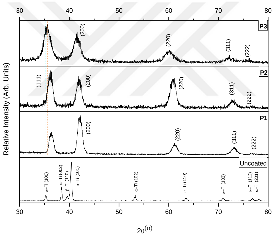
Figure 4-28 GAXRD (2° angle of incidence) diffraction patterns for Ti-Nb-N coatings on Ti-64 substrates
