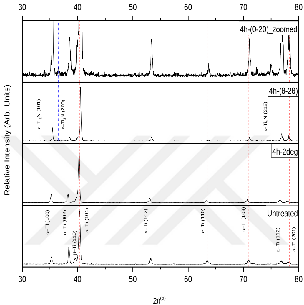
Figure 5-5 GAXRD ( 2^{\circ} angle of incidence) and Theta-2theta diffraction patterns of the uncoated Ti-64 substrate treated at 600°C for 4 hours (also includes \theta - 2\theta peaks as zoomed)
