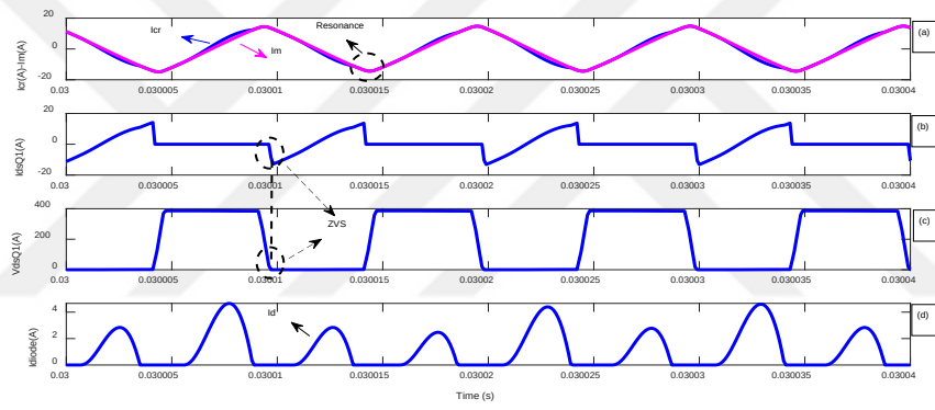
Figure 4.50 Icr and Im (a), IDSQ1 (b), VDSQ1 (c), Idiode (d), (5% load)
