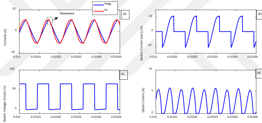
Figure 5.53 State 5, PV panel-side resonance capacitor and transformer magnetizing current ( I_{cr} - I_{m} ) (a) Switch current ( I_{sQ1} ) (b), Switch Voltage ( V_{sQ1} ) (c), Rectifier diode current (d)
