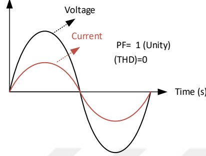
Figure 1.7 Voltage, current and THD relationship of power factor (Alam., 2017)
