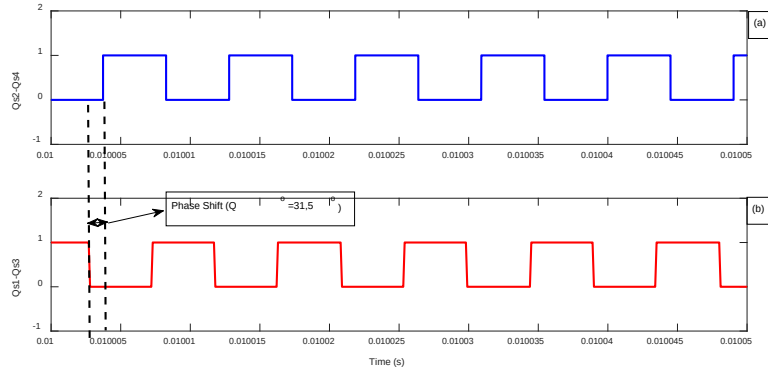
Figure 2.17 PHFB converter switching signals (Qs2-Qs4) (a), (Qs1-Qs3) (b)
