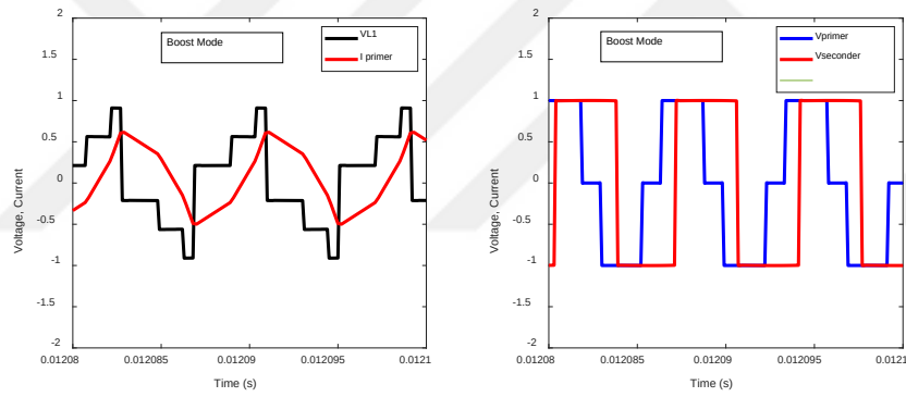
Figure 2.31 Current and voltage characteristics of transformer (boost mode)
