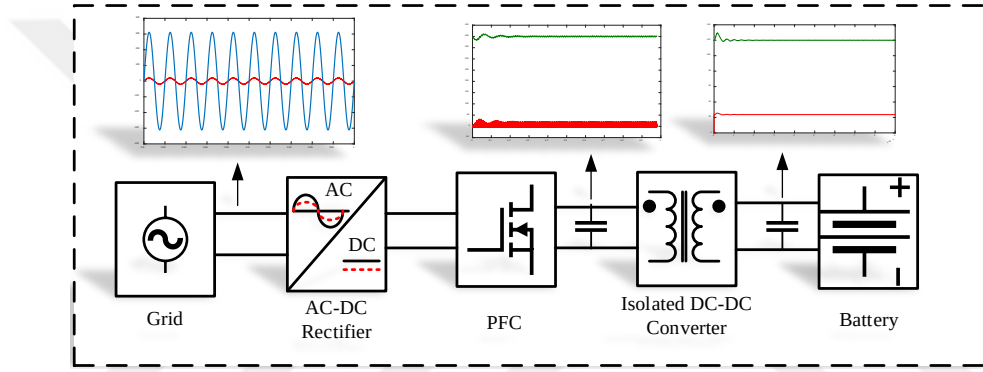
Figure 1.5 General structure of two-stage OBC.
