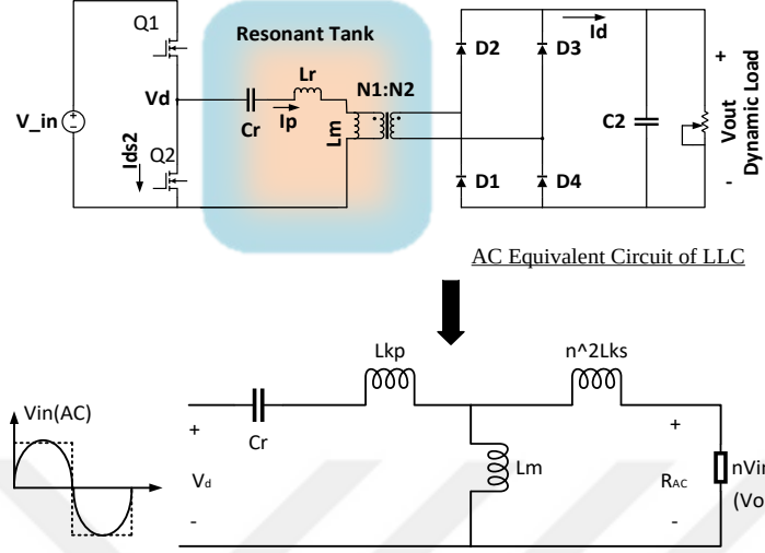
Figure 4.5 HLLC resonant converter and equivalent circuit.
