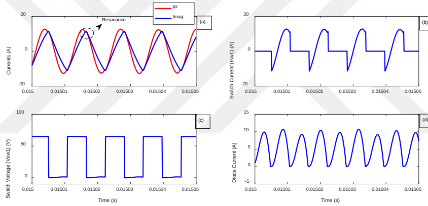
Figure 5.46 State 4, PV panel-side resonance capacitor and transformer magnetizing current (Icr-Im) (a) Switch current (IsQ1) (b), Switch voltage (VsQ1) (c), Rectifier diode current (d)
