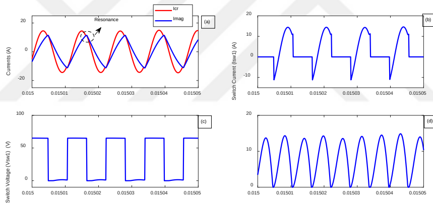
Figure 5.39 State 3, PV panel-side resonant capacitor and transformer magnetizing current (Icr-Im) (a) Switch current (IsQ1) (b), Switch voltage (VsQ1) (c), Rectifier diode current (d)
