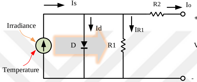
Figure 5.2 Single diode equivalent circuit of the solar cell.
