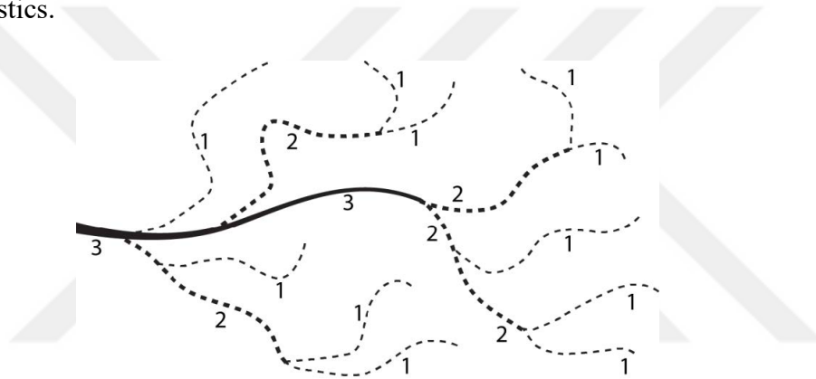
Figure 2.1. Strahler's Stream Order [Source: Strahler (1952)]
