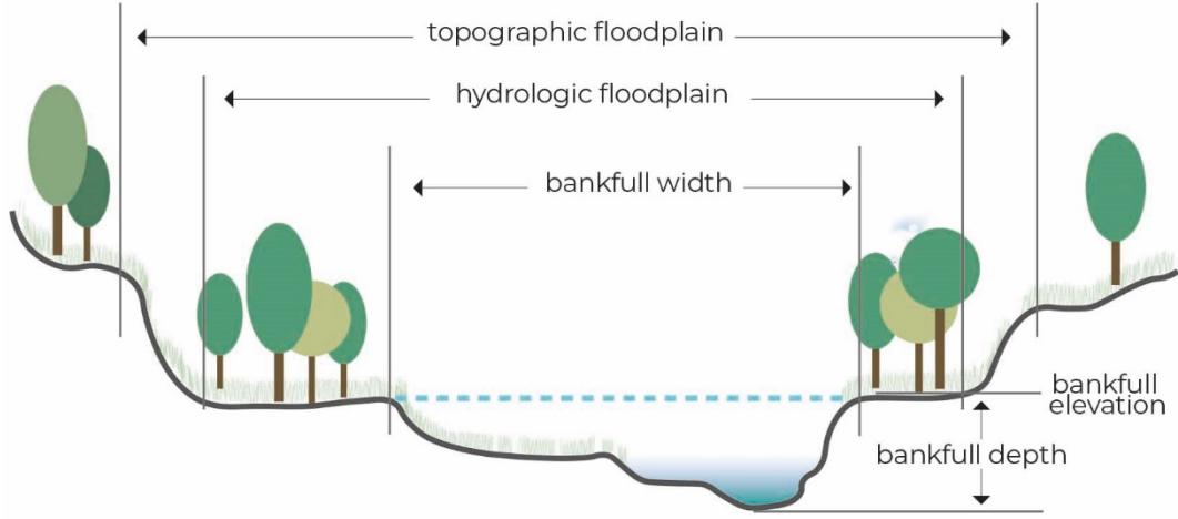
Figure 2.3. Bankfull discharge
