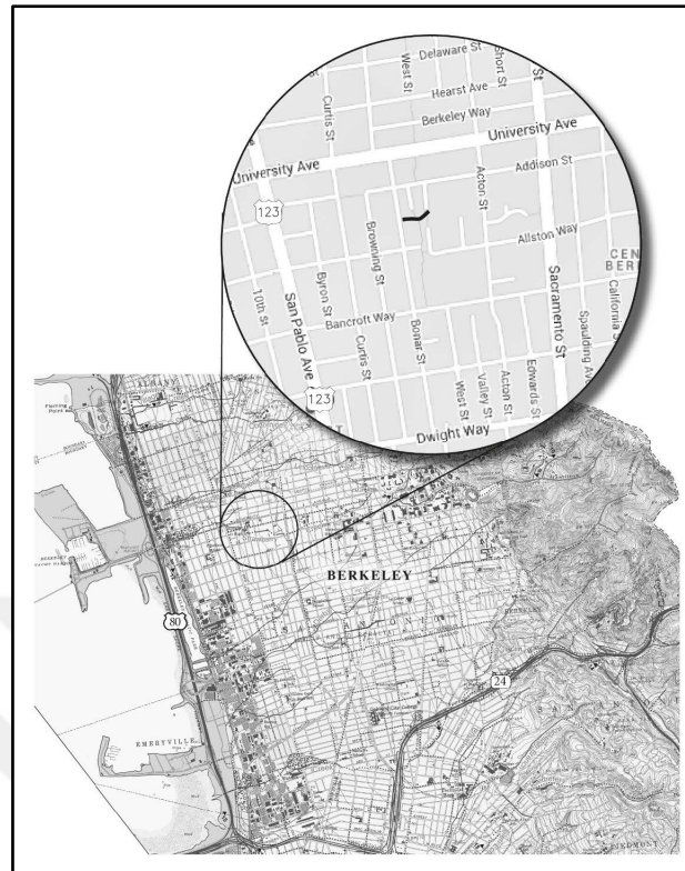
Figure 3.2. The Creek flows from Strawberry Canyon in the Berkeley Hills to San Francisco Bay [Source: Riley, L. A. (2016)]
