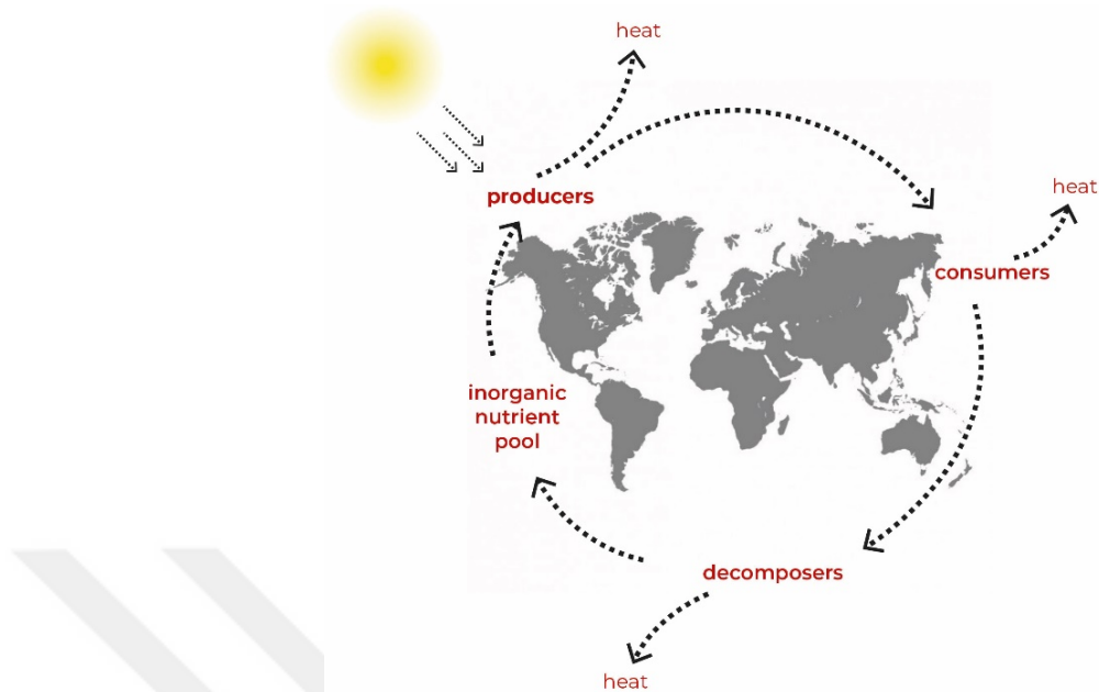
Figure 2.5. The flow of energy lost in the unusable form of heat and chemical nutrients continues as a biogeochemical cycle. (Reproduced from khanacademy.org , accessed November 2020)
