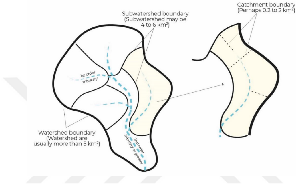
Figure 2.2. Watershed scale: Watershed, Subwatershed, and Catchment
